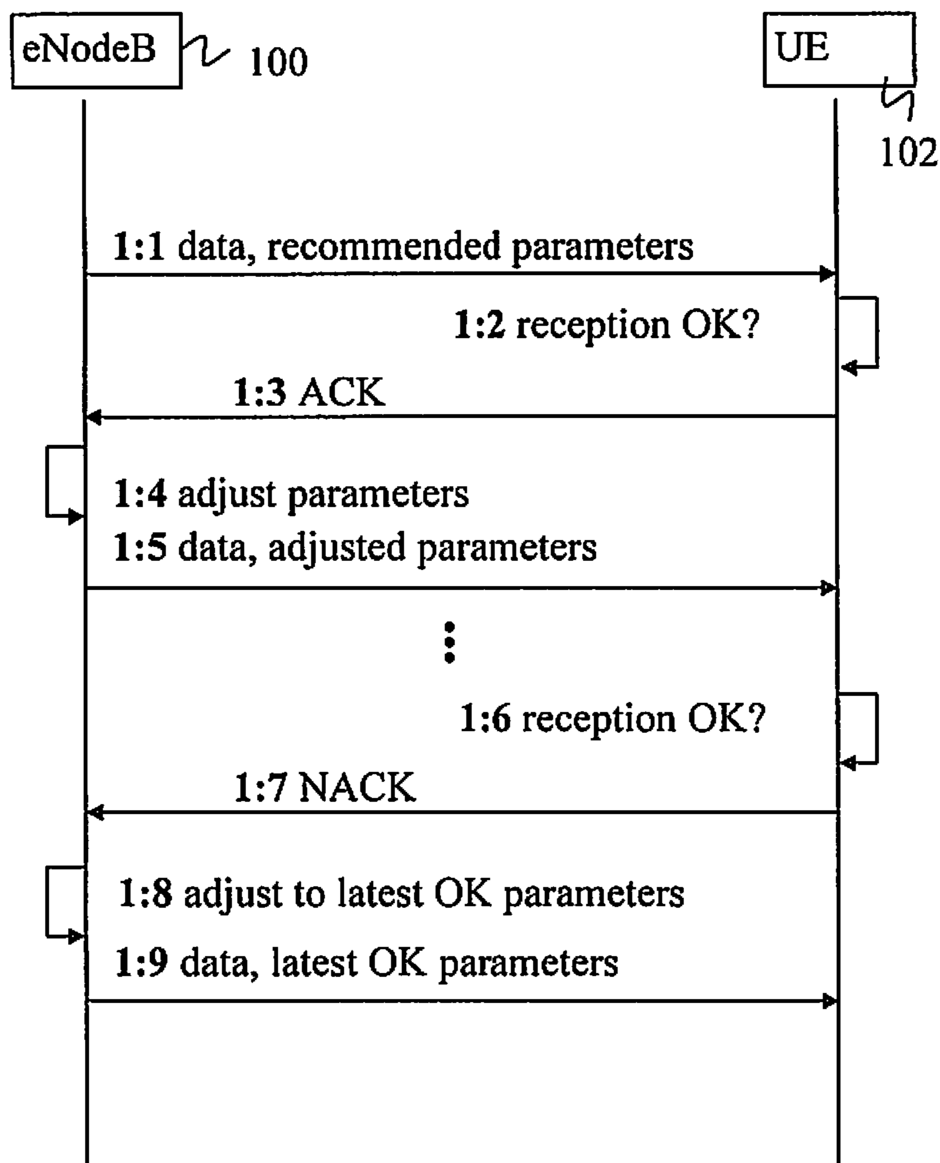
Figure 1 (prior art)
