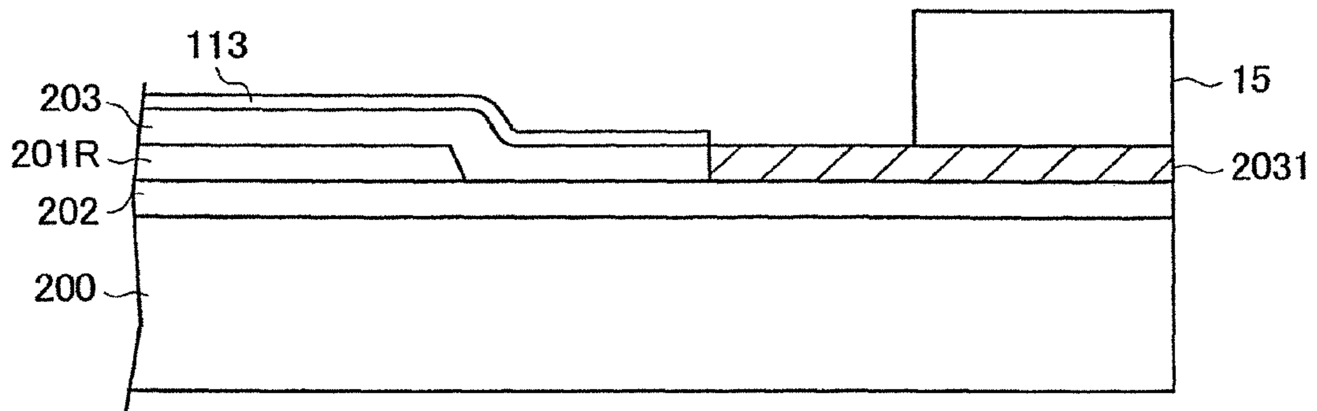
FIG. 16 PRIOR ART
