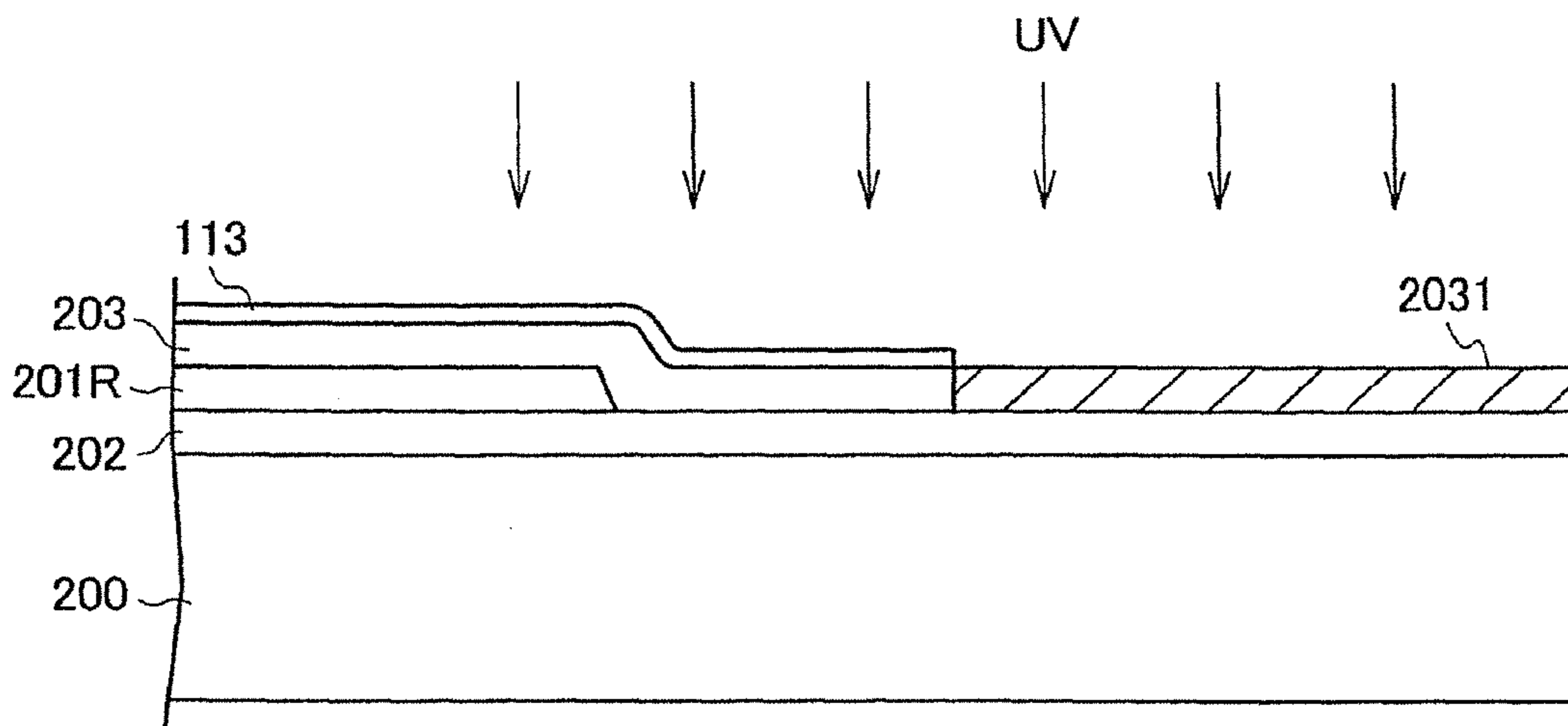
FIG. 15 PRIOR ART
