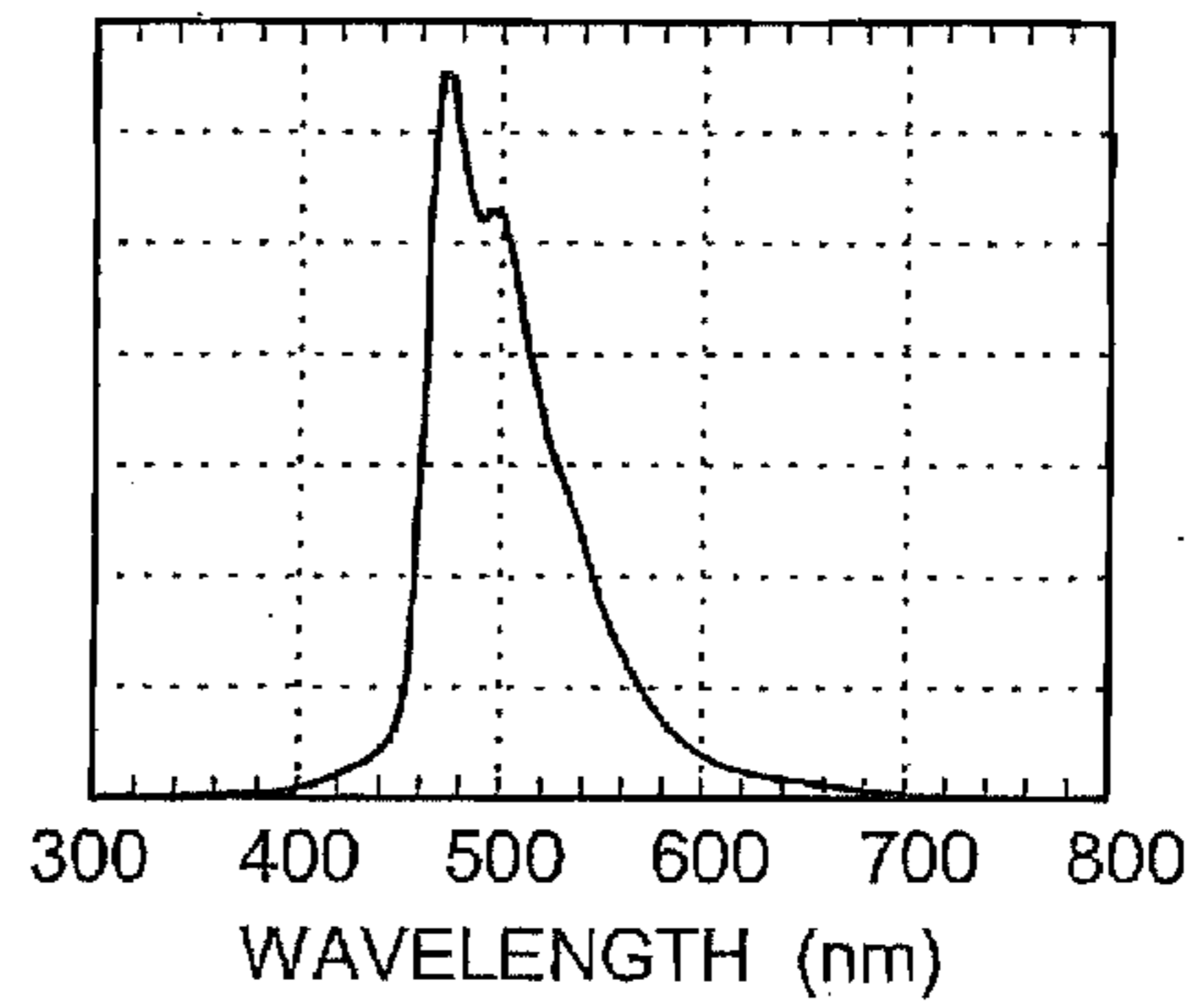
FIG. 8D LIGHT EMISSION SPECTRUM
