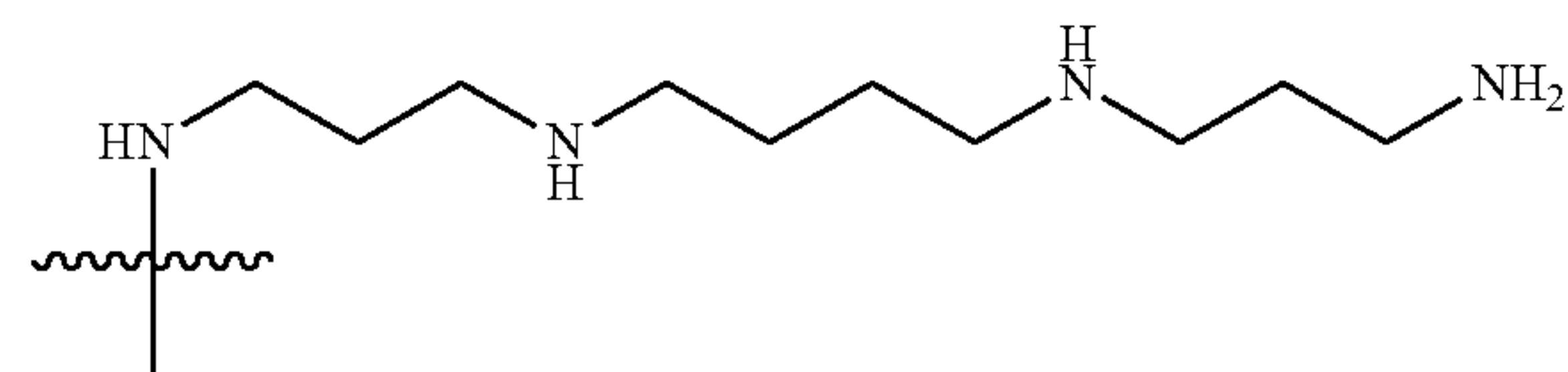
Spermine
