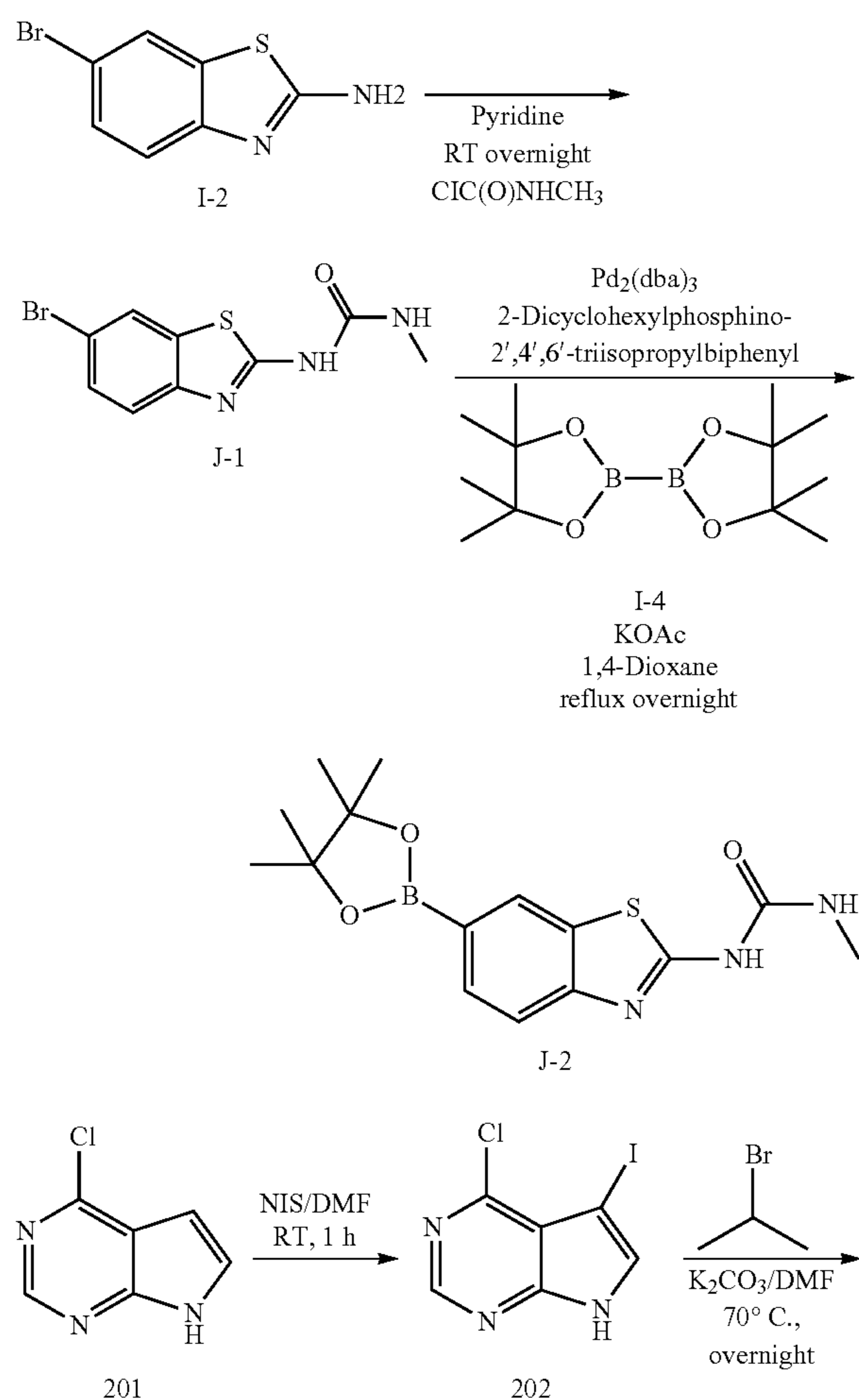
Scheme 3. The synthesis of 1-(6-(4-amino-7-isopropyl-7H-pyrrolo[2,3-d]pyrimidin-5-yl)benzo[d]thiazol-2-yl)-3-methylurea
