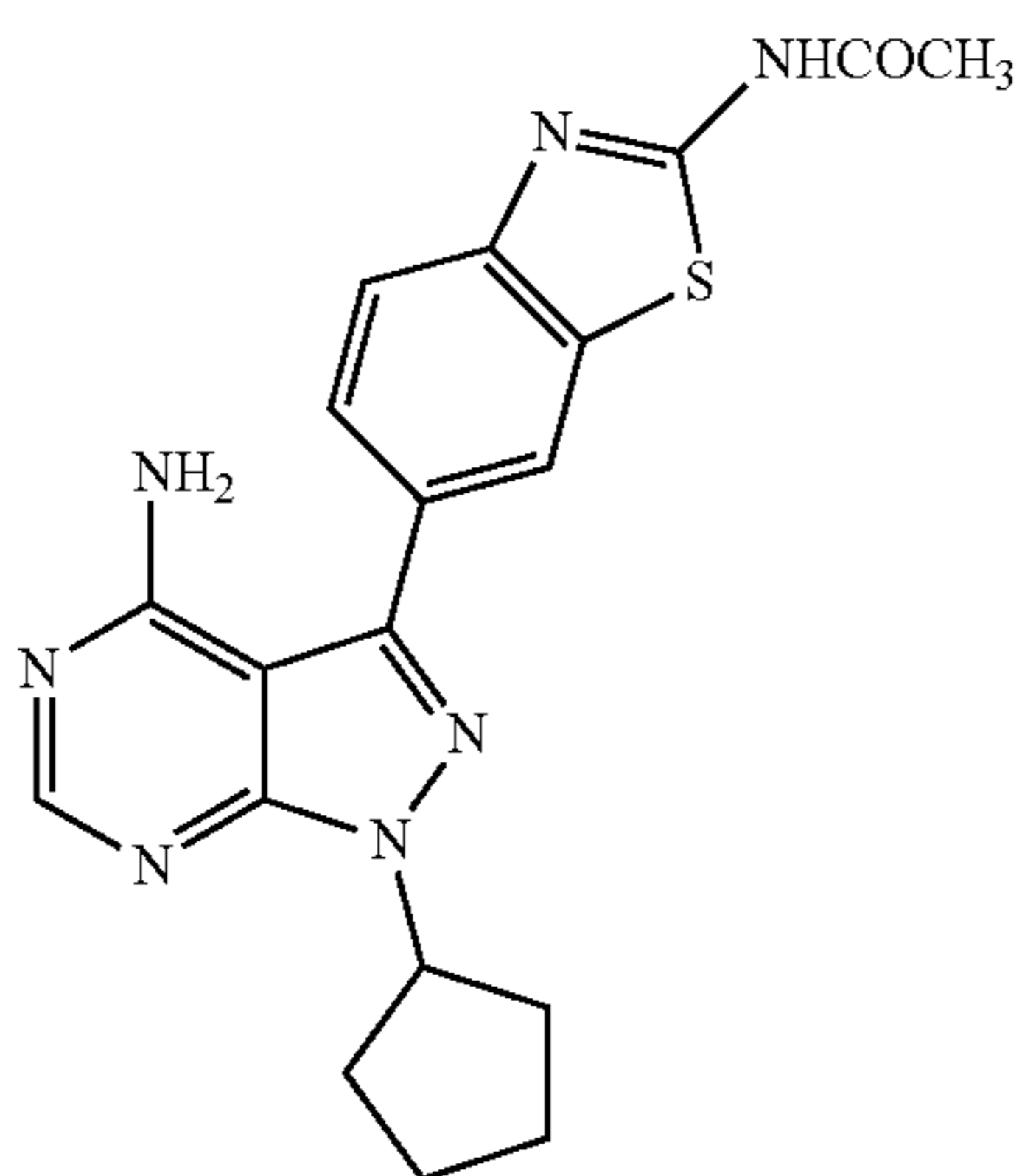
Compound 4
