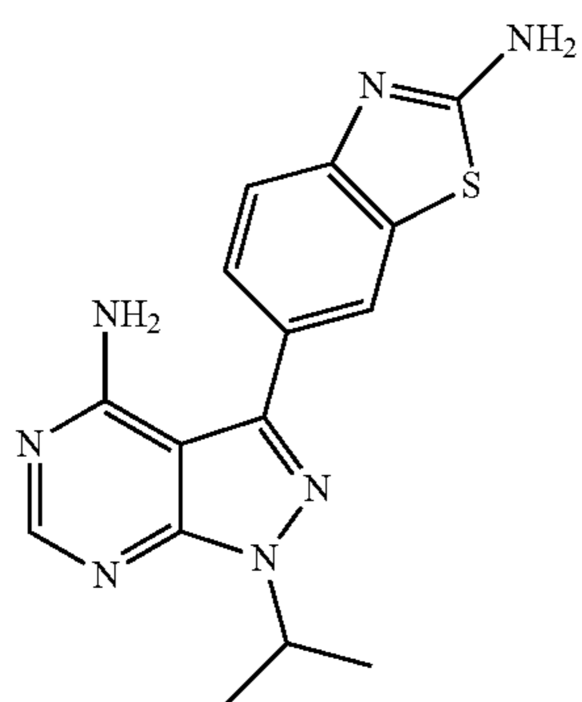
Compound 3
