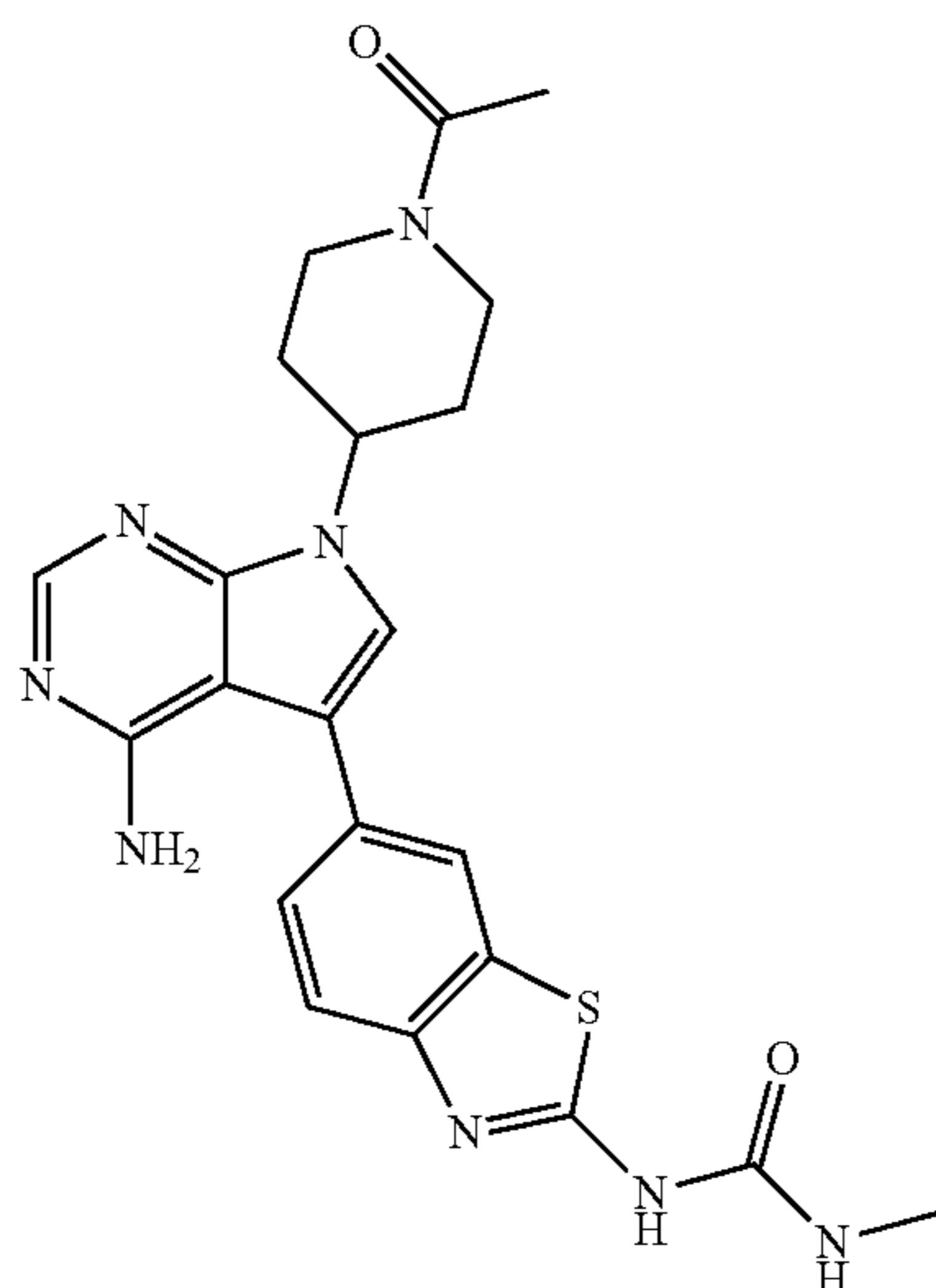
Compound 23
