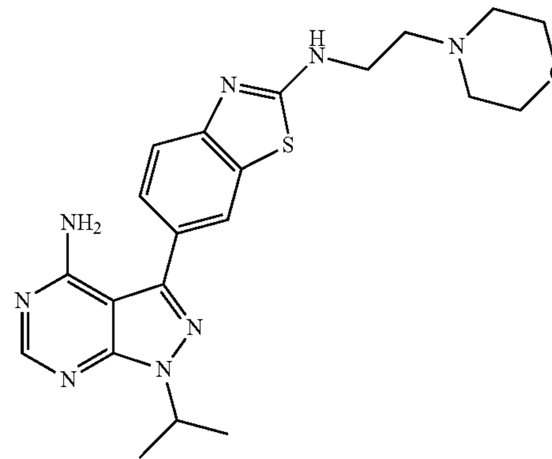
Compound 13
