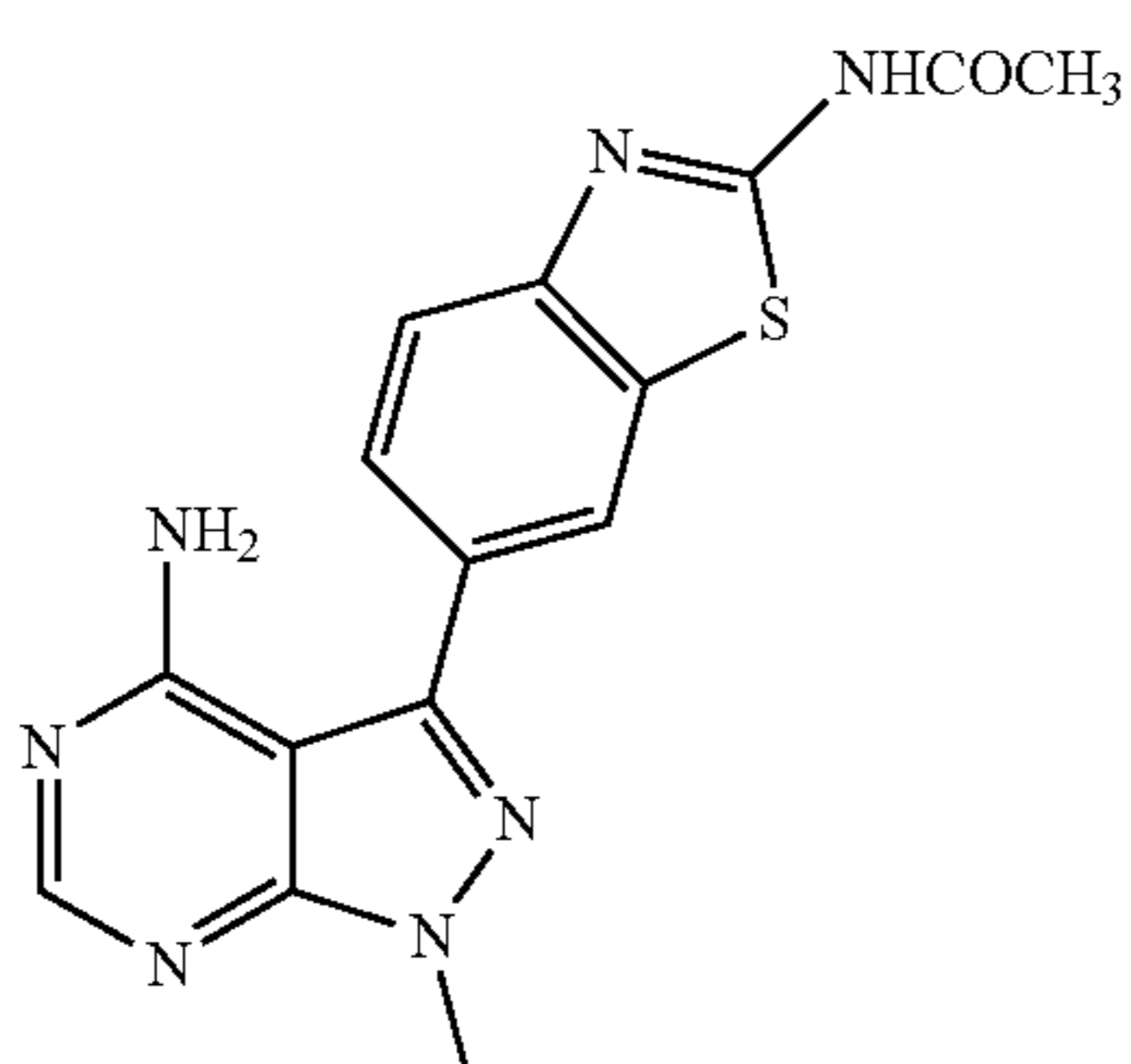
Compound 6
