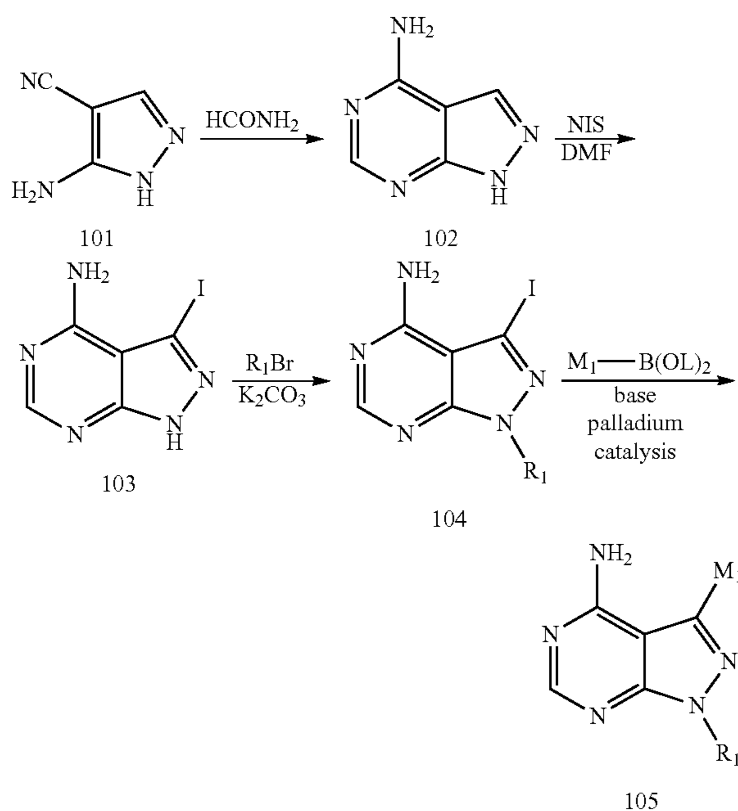
Scheme 1: Synthesis of pyrazolopyrimidine compounds of the invention.
