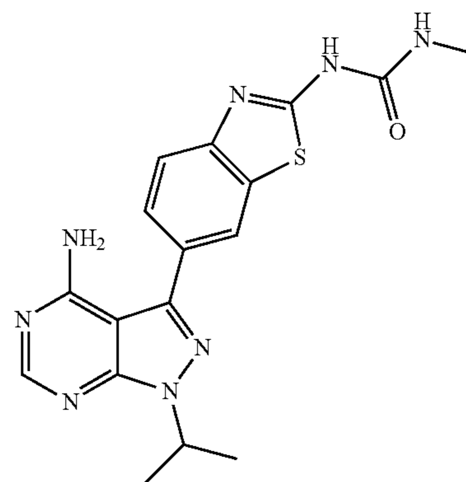
Compound 20
