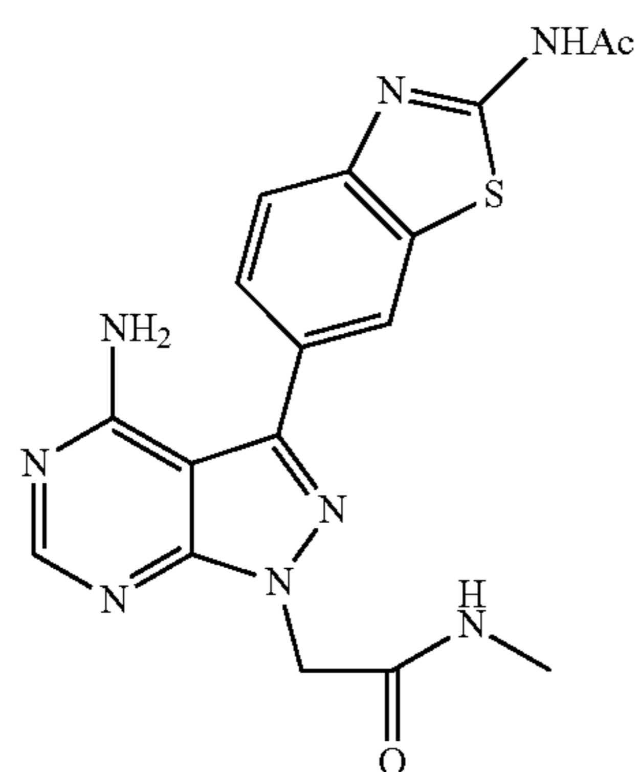
Compound 18
