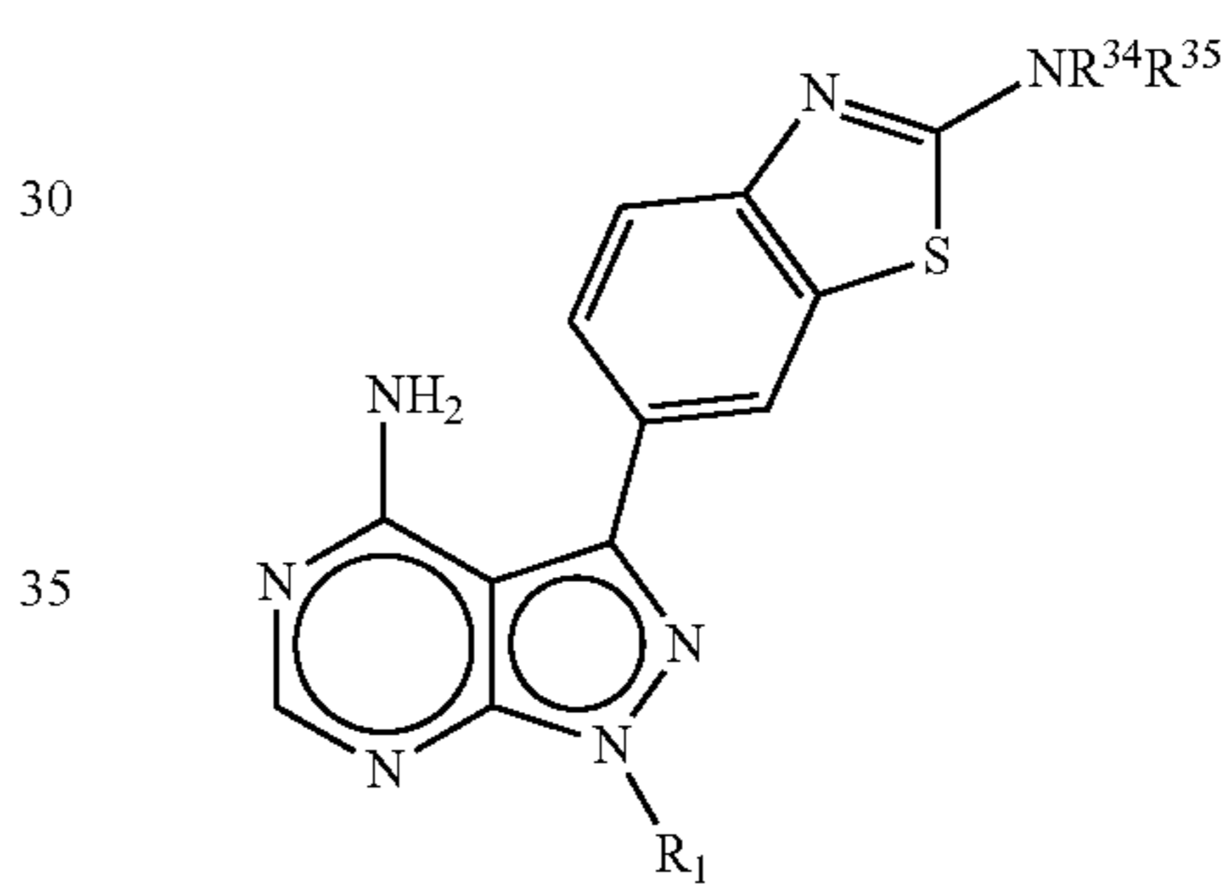
Formula XI-2
