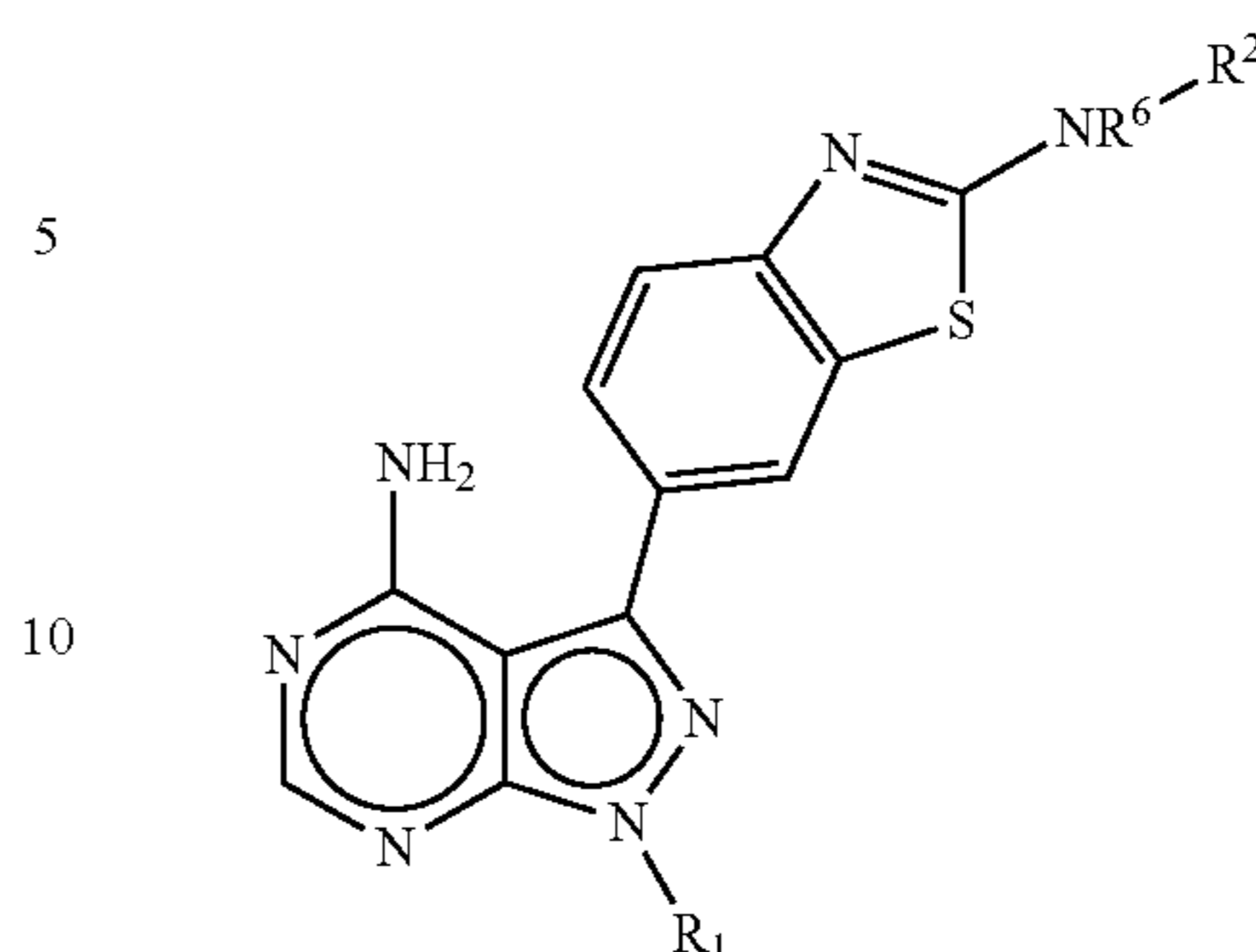
Formula XI-1
