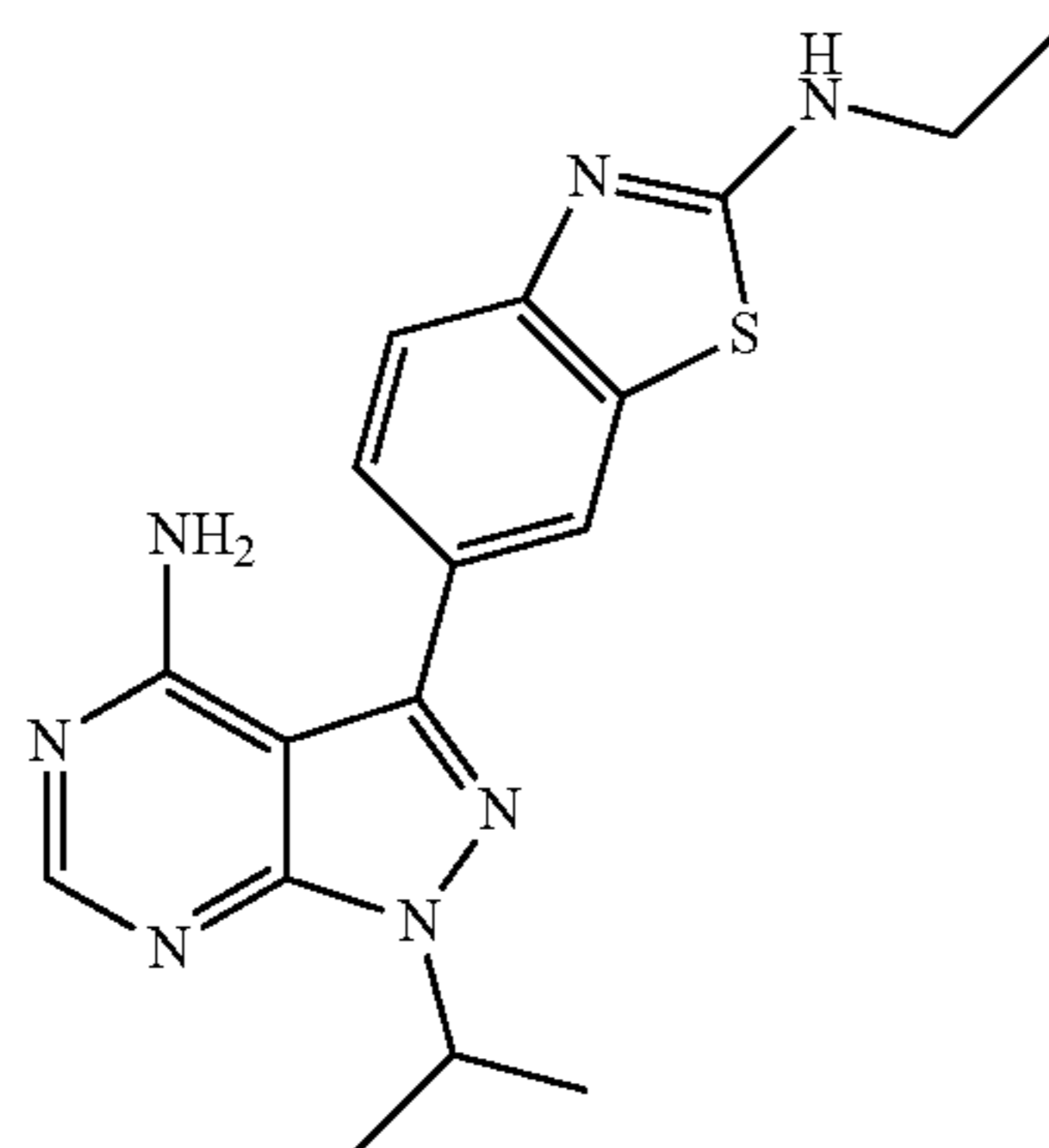
Compound 12
