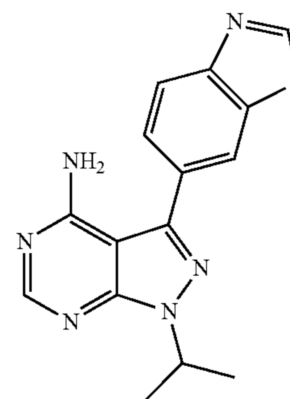
Compound 2
