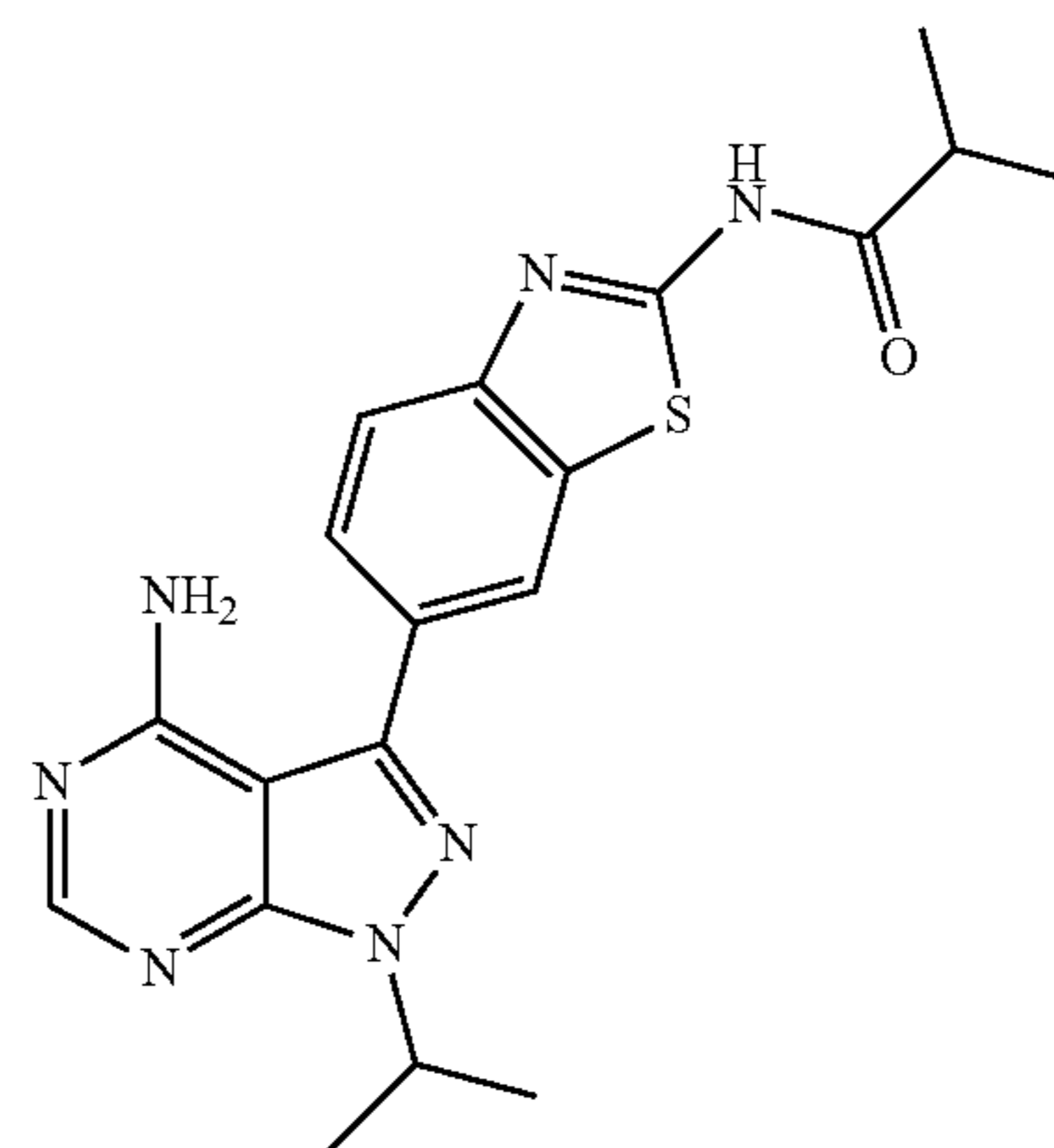
Compound 7
