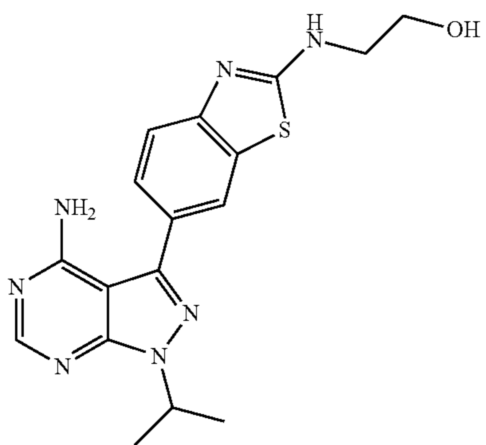
Compound 16
