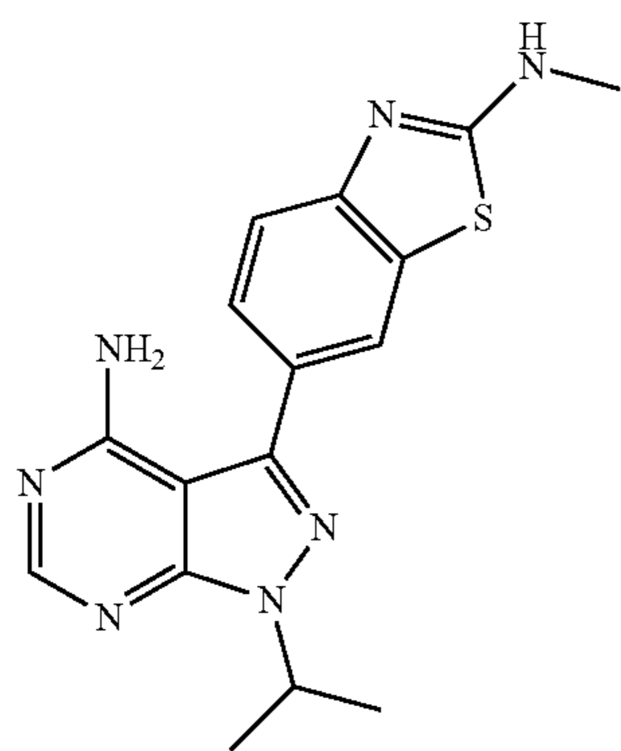
Compound 11
