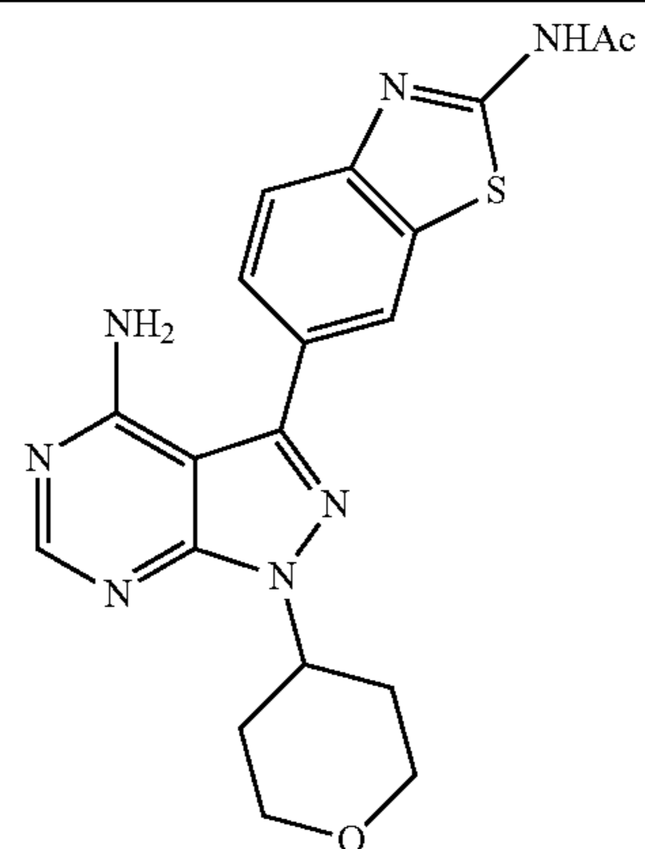
Compound 19
