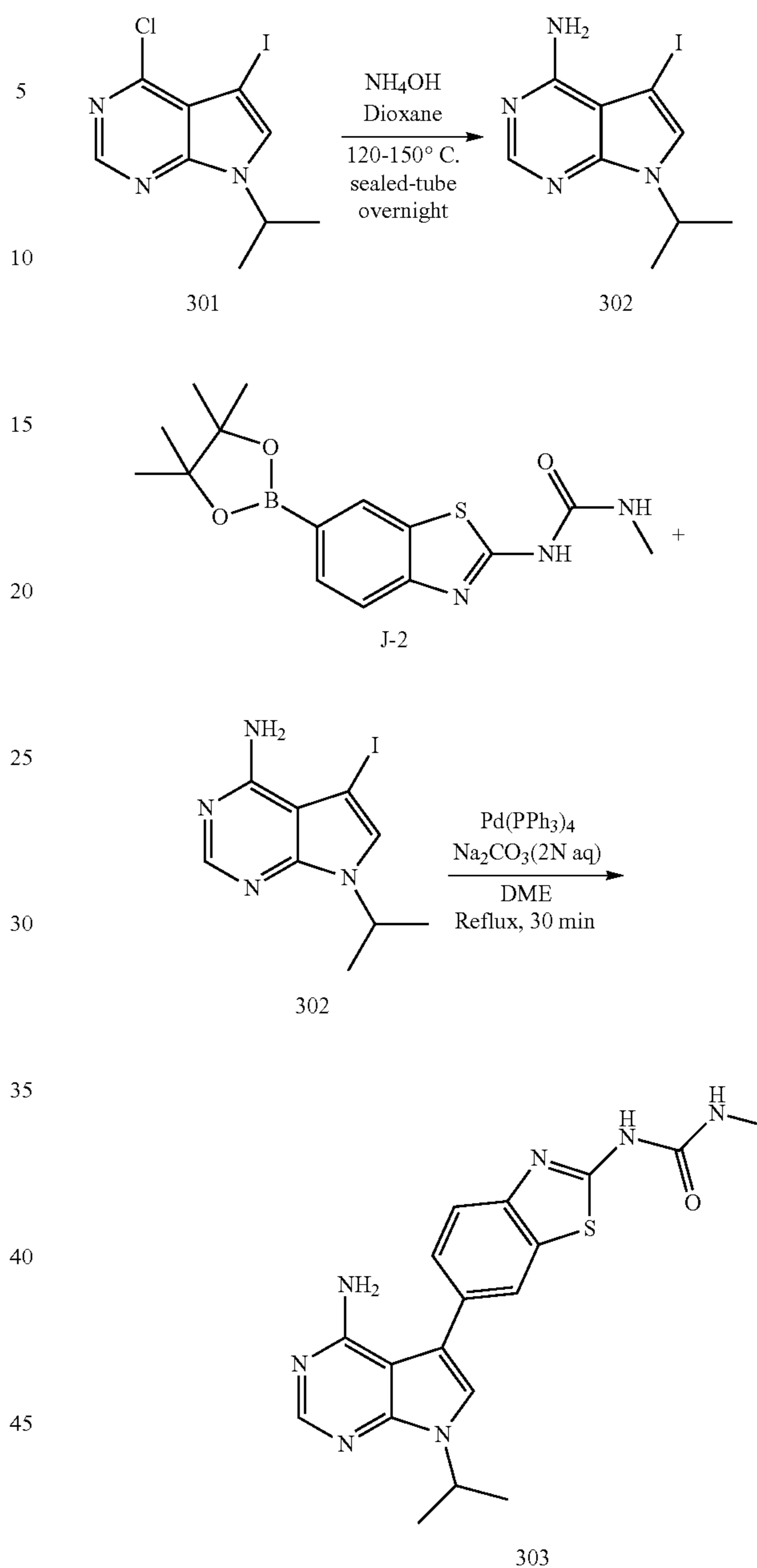
Scheme 3. The synthesis of 1-(6-(4-amino-7-isopropyl-7H-pyrrolo[2,3-d]pyrimidin-5-yl)benzo[d]thiazol-2-yl)-3-methylurea
