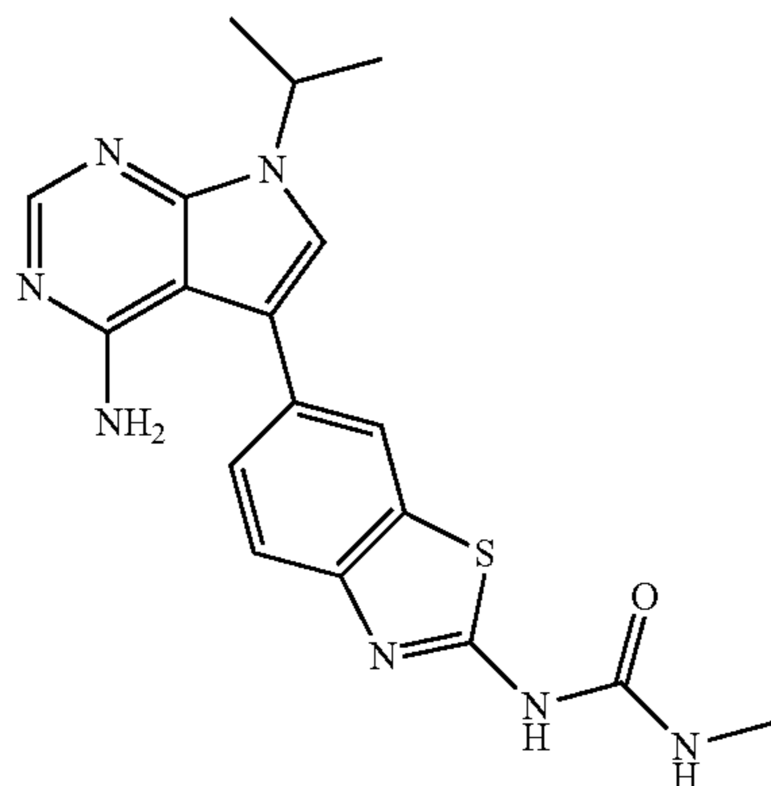
Compound 22
