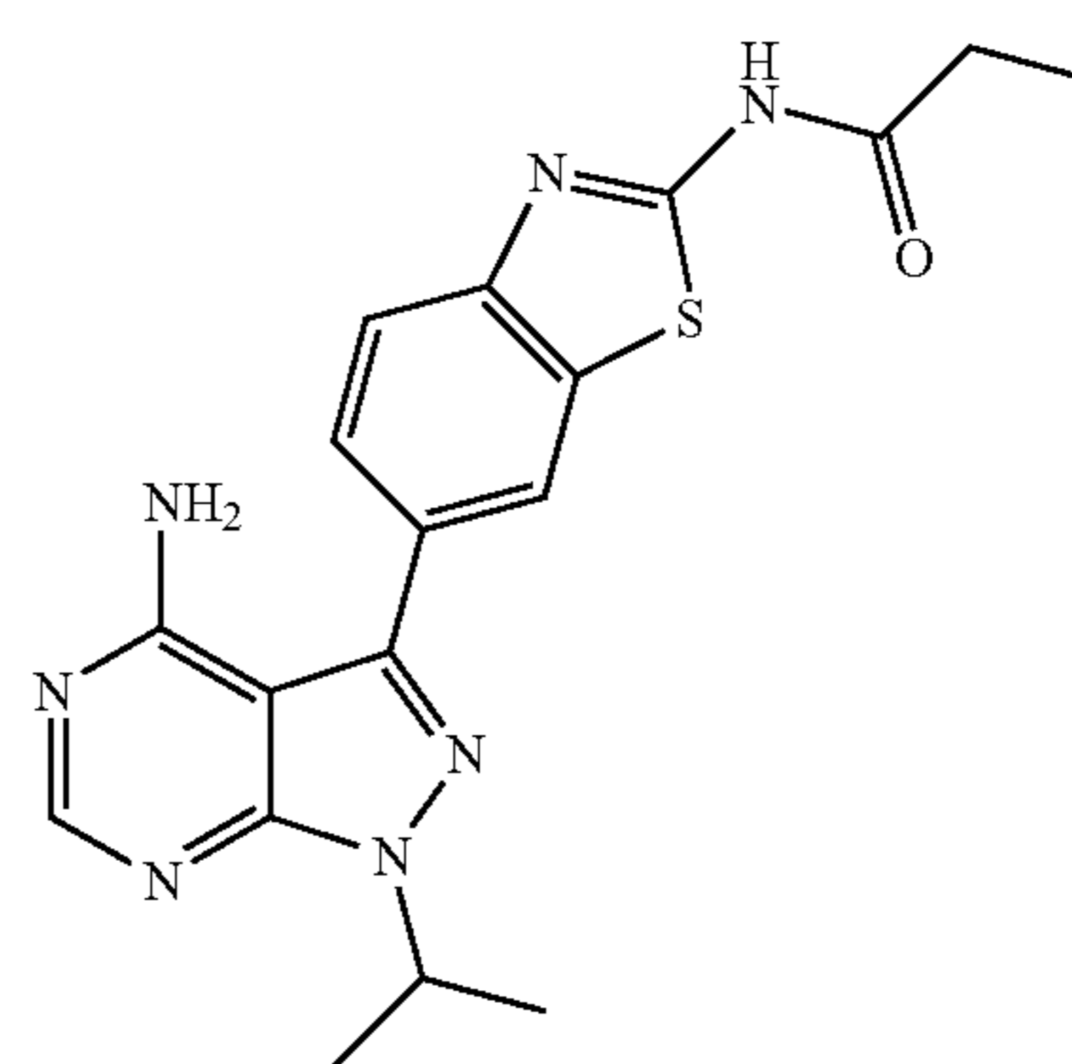
Compound 9
