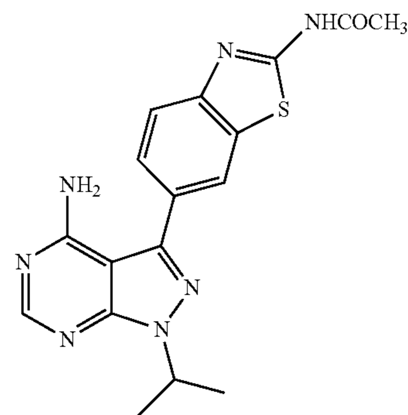
Compound 1
