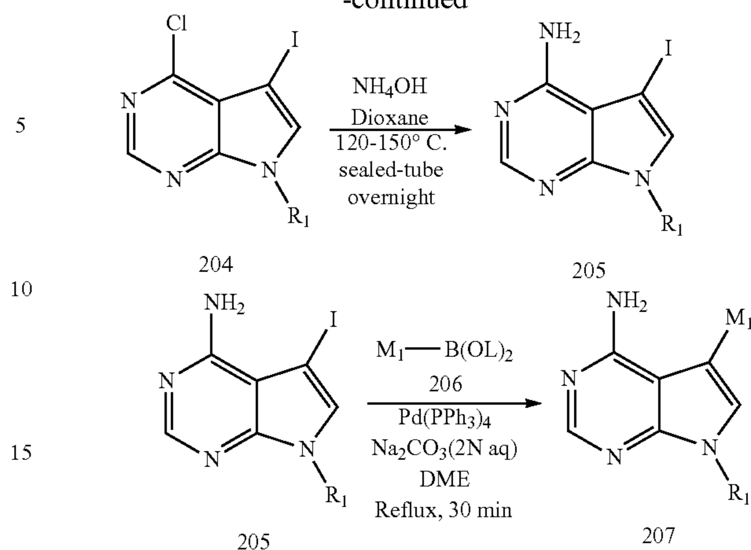
Scheme 1: Synthesis of pyrazolopyrimidine compounds of the invention.
