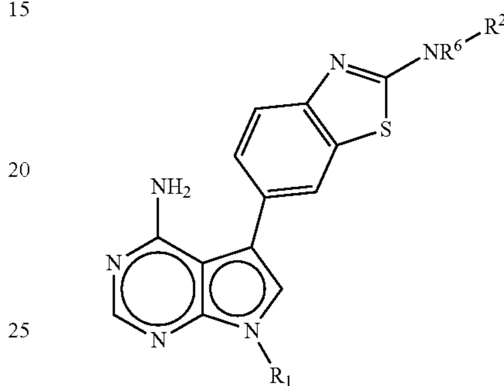
Formula XII-1
