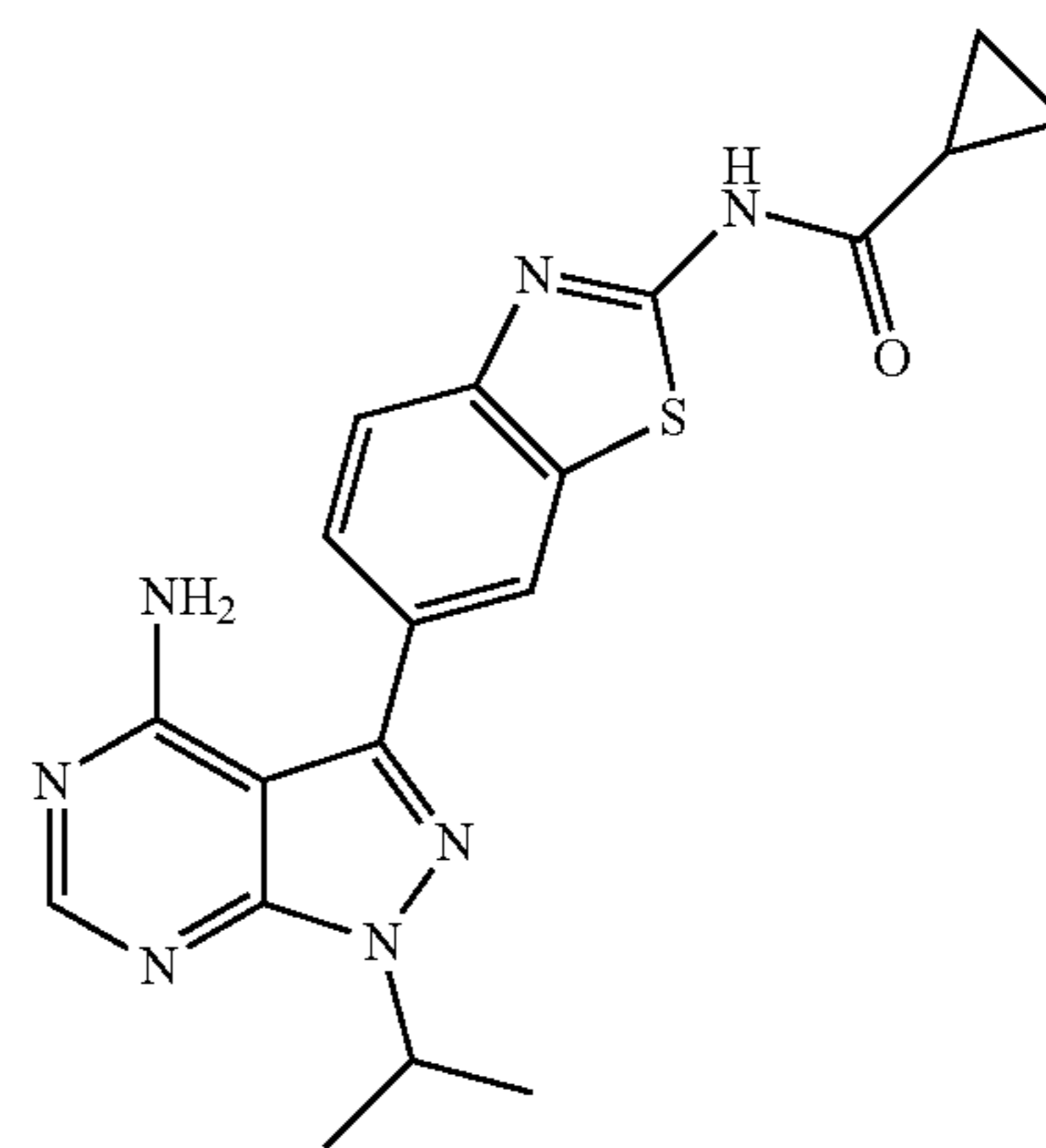
Compound 8
