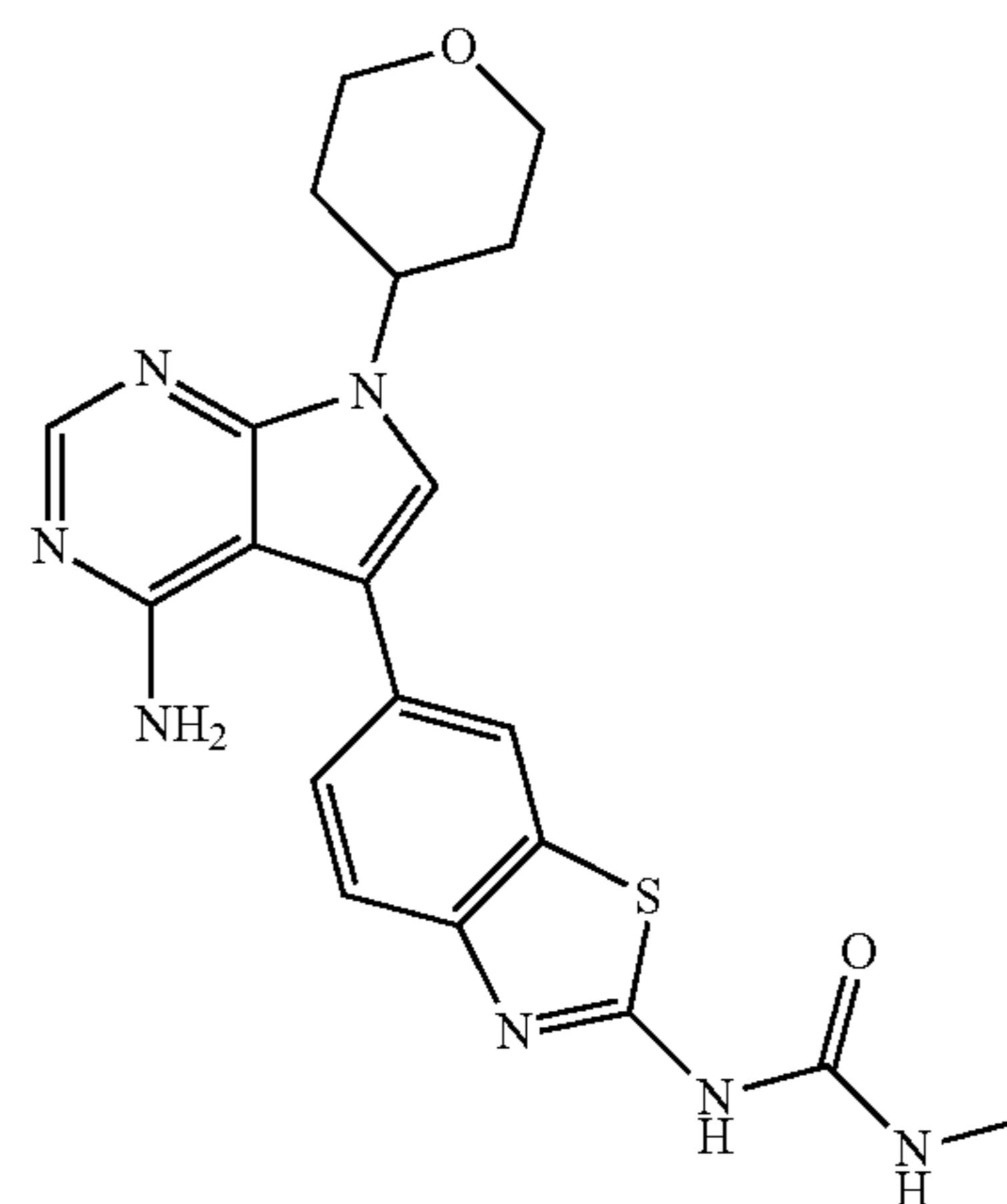
Compound 21
