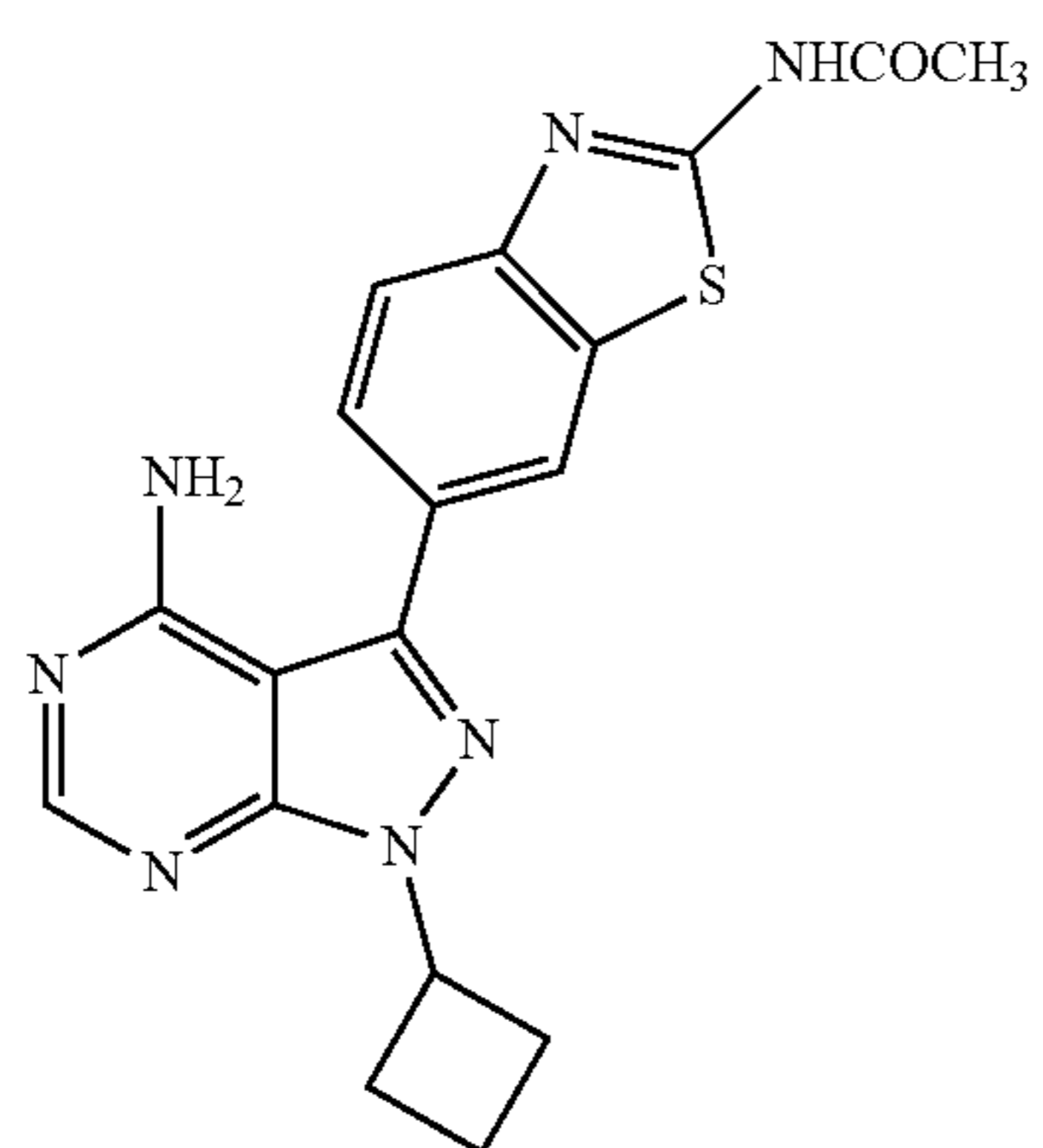
Compound 10
