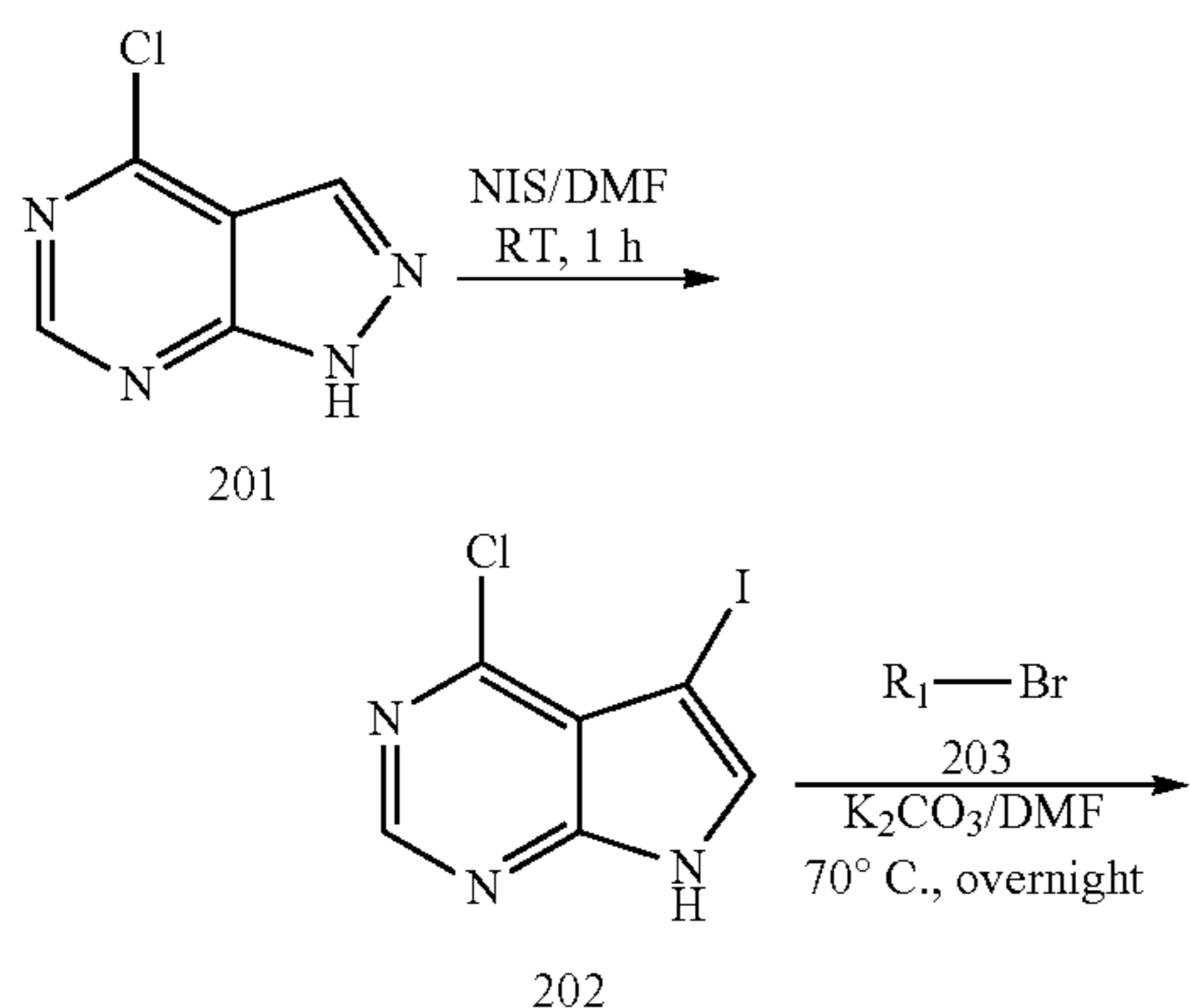
Scheme 2: Synthesis of pyrrolopyrimidine compounds of the invention
