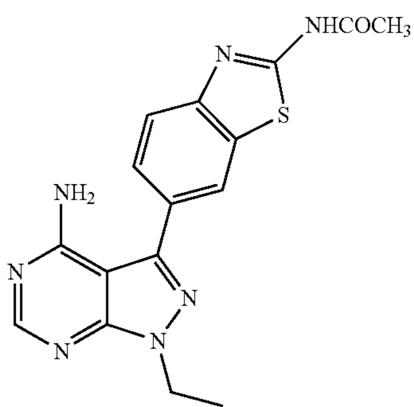
Compound 5
