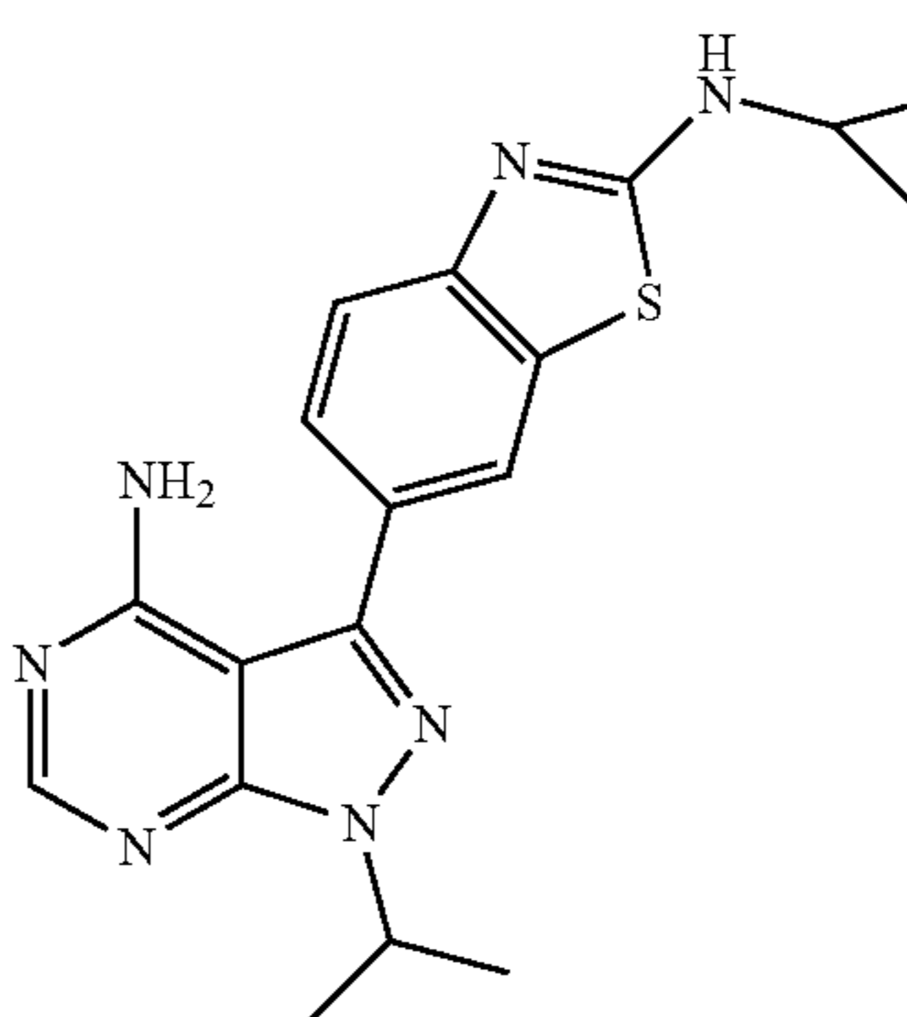
Compound 15
