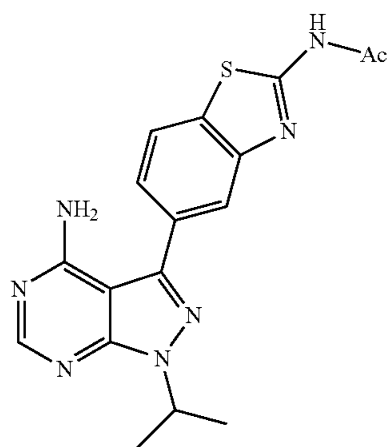
Compound 17
