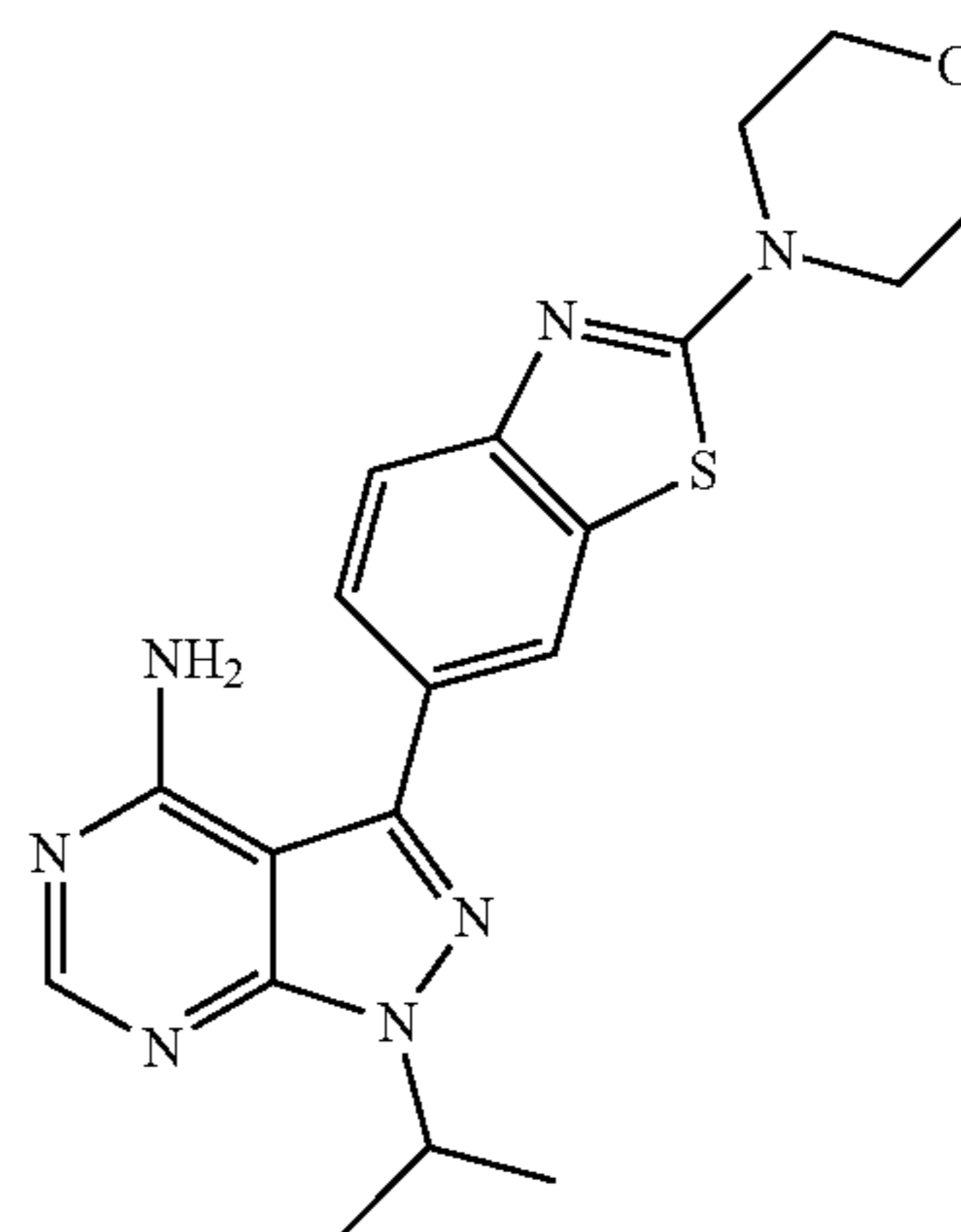
Compound 14
