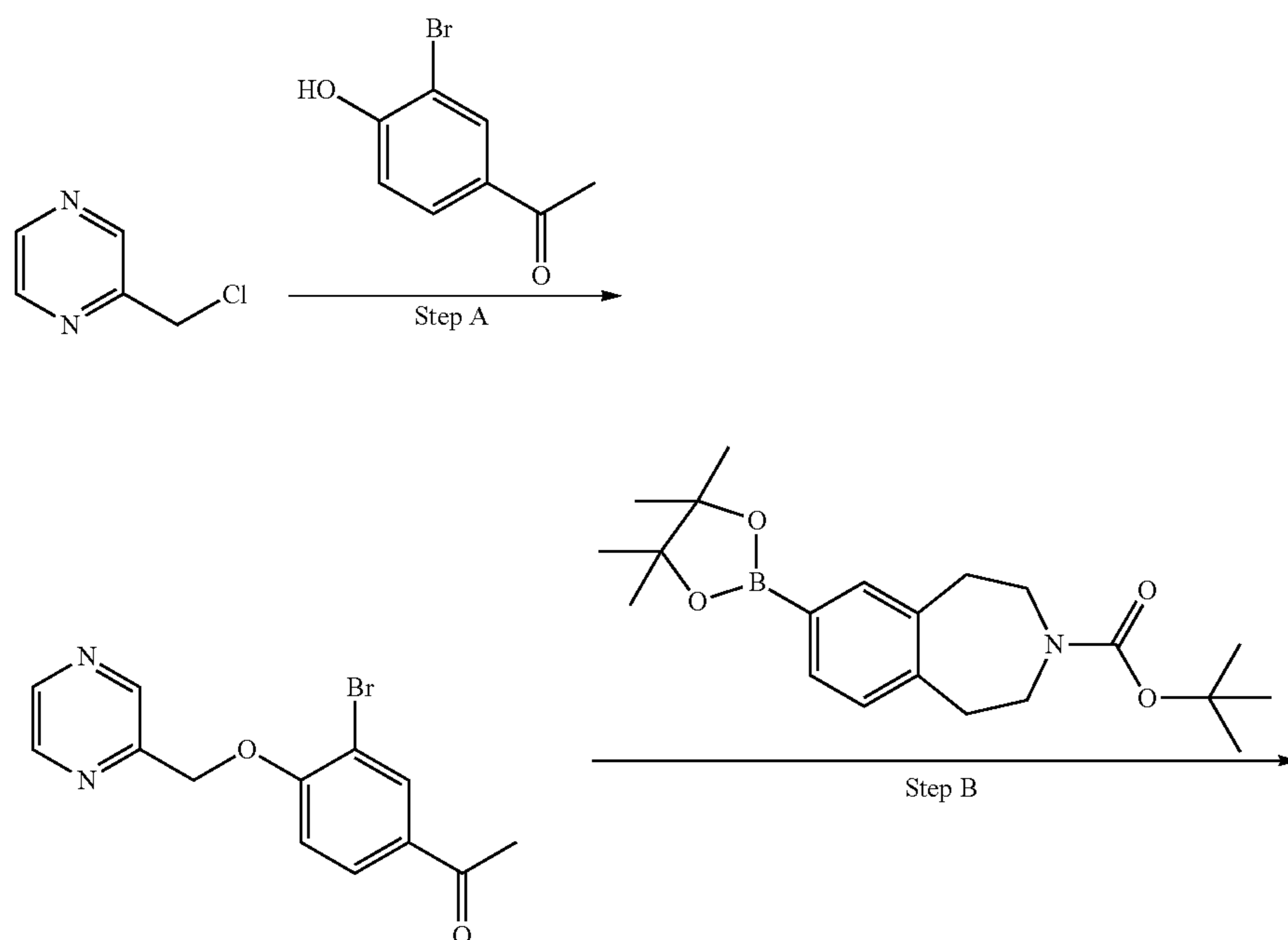
Scheme 3:
