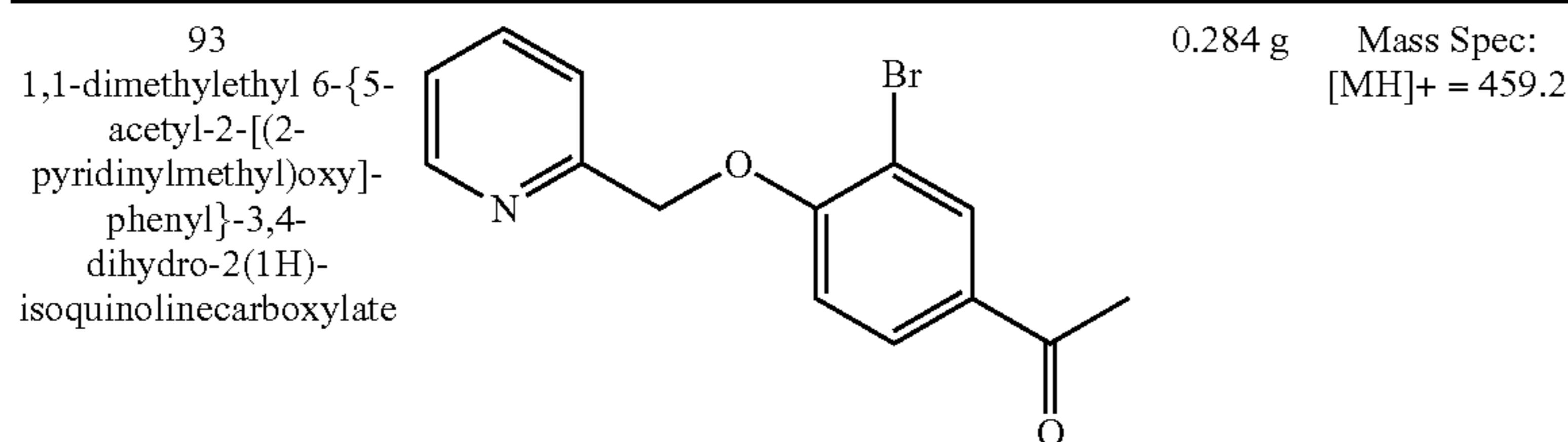
Intermediate 60, 2-bromo-5-[(phenylmethyl)oxy]pyridine
