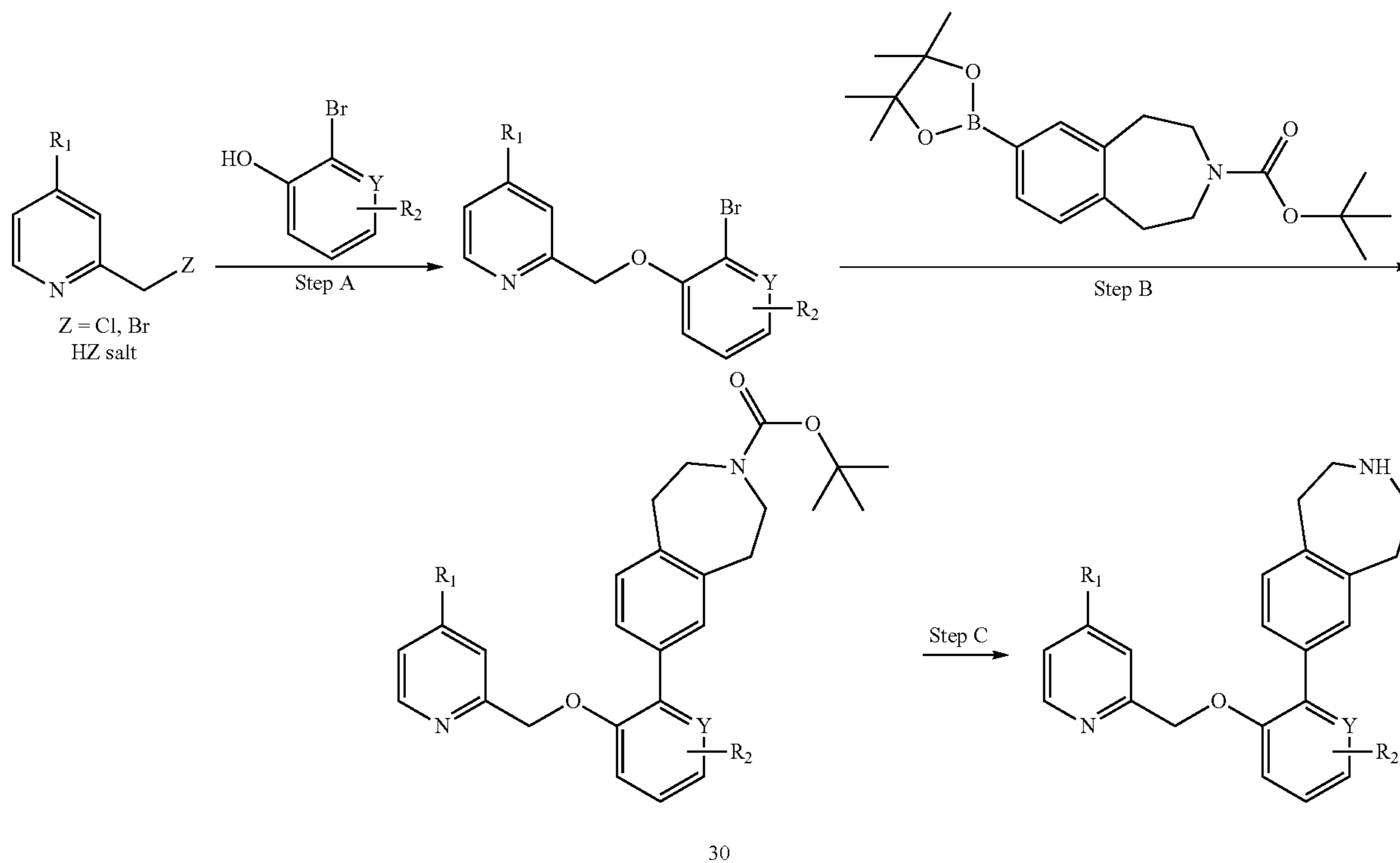
Scheme 2:
