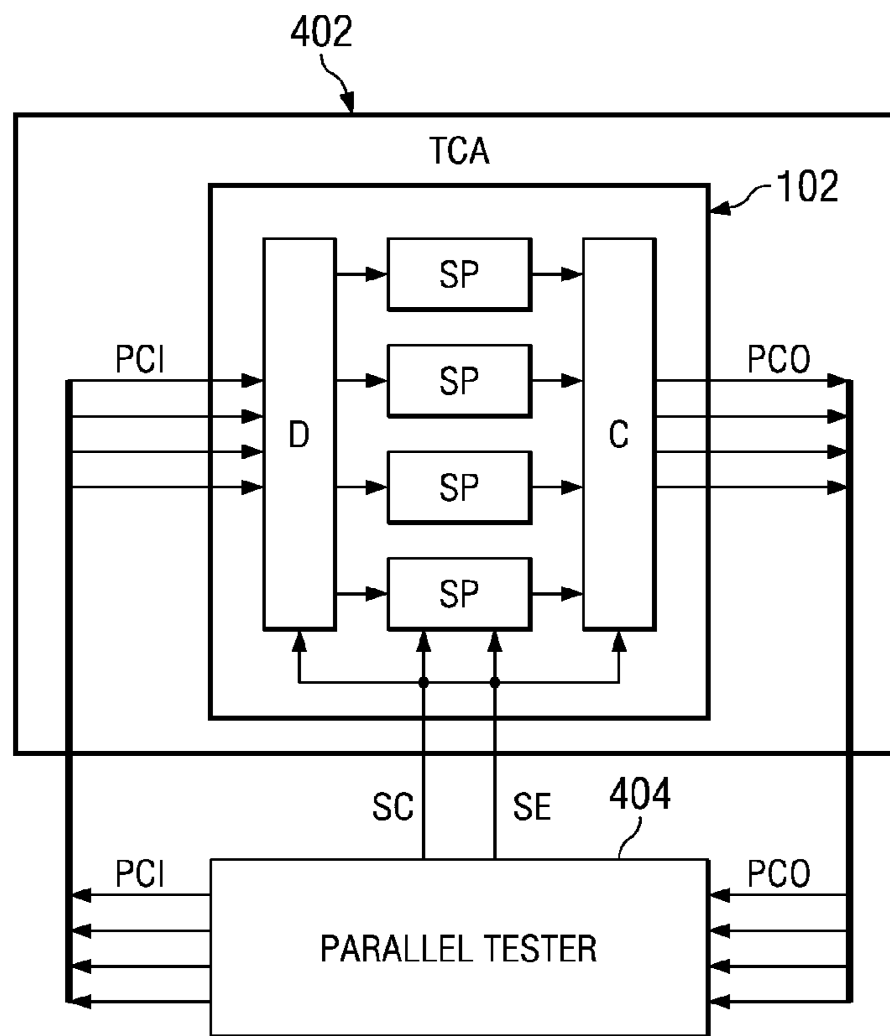
FIG. 4 (PRIOR ART)
