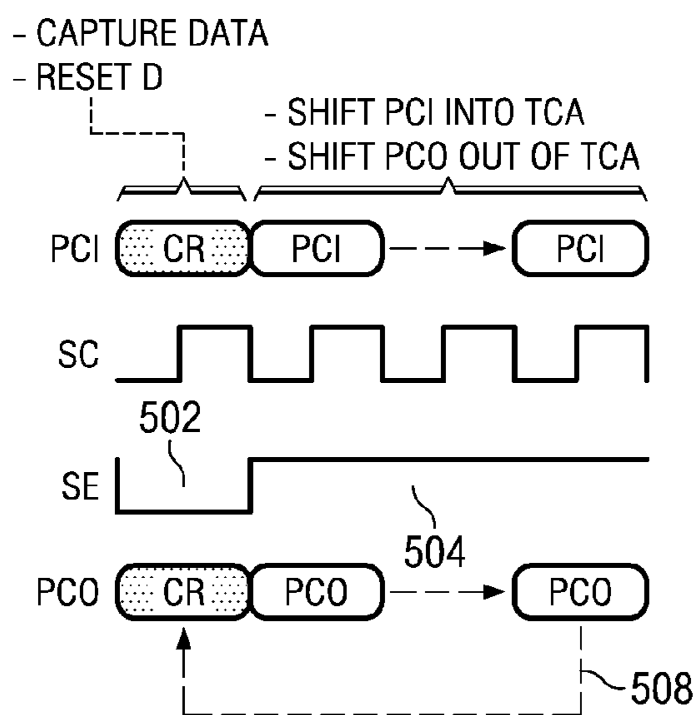
FIG. 5 (PRIOR ART)
