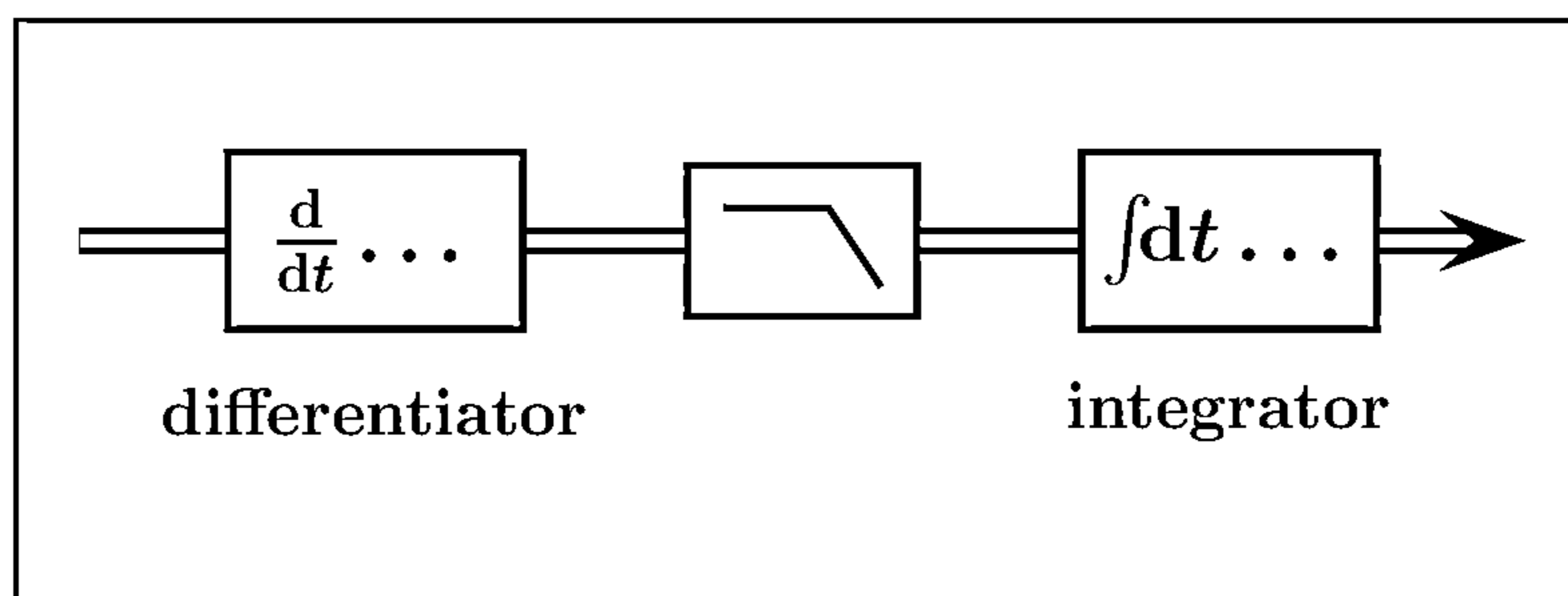
Equivalent linear lowpass filter
