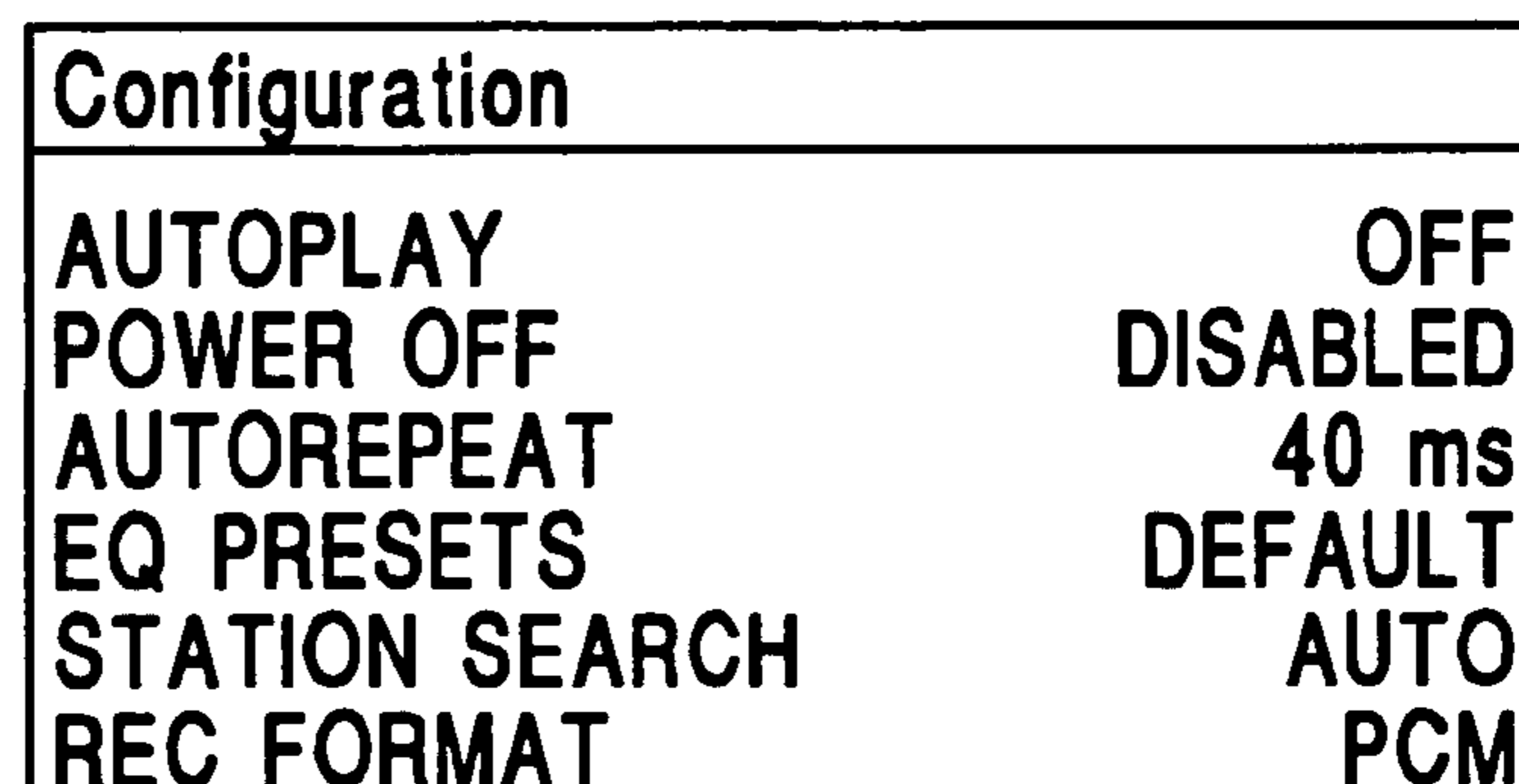
Configuration Screen
