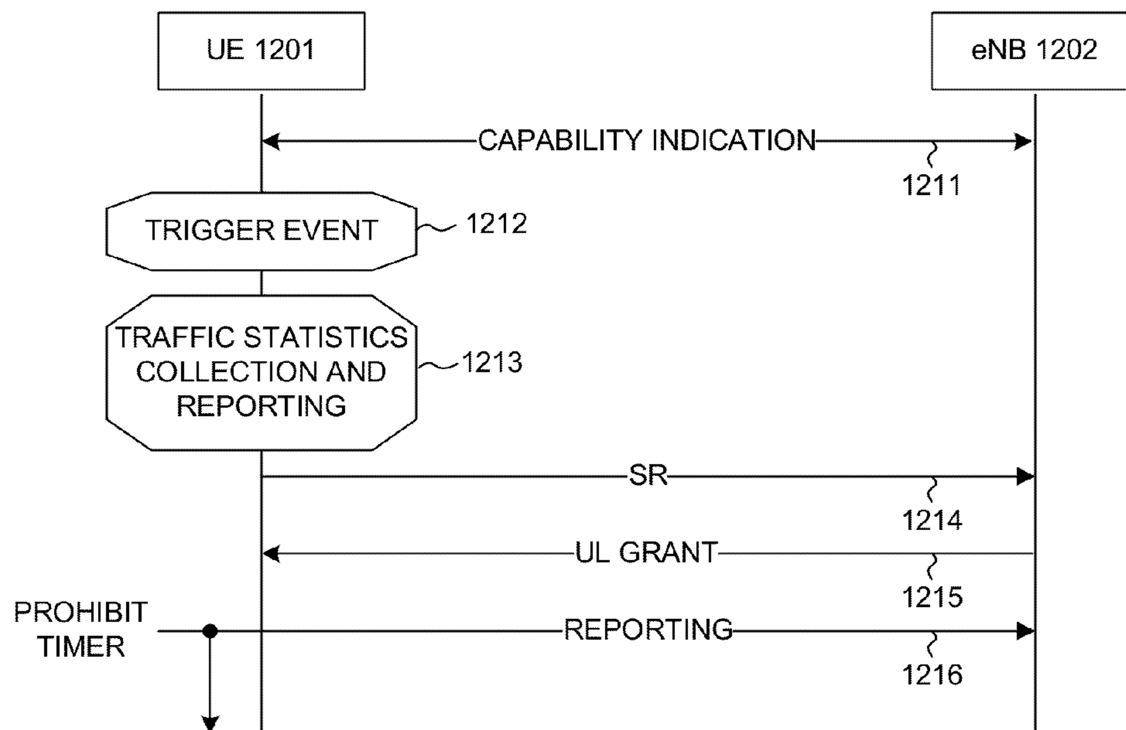
UE-ORIENTED TRAFFIC STATISTICS FIG. 12
