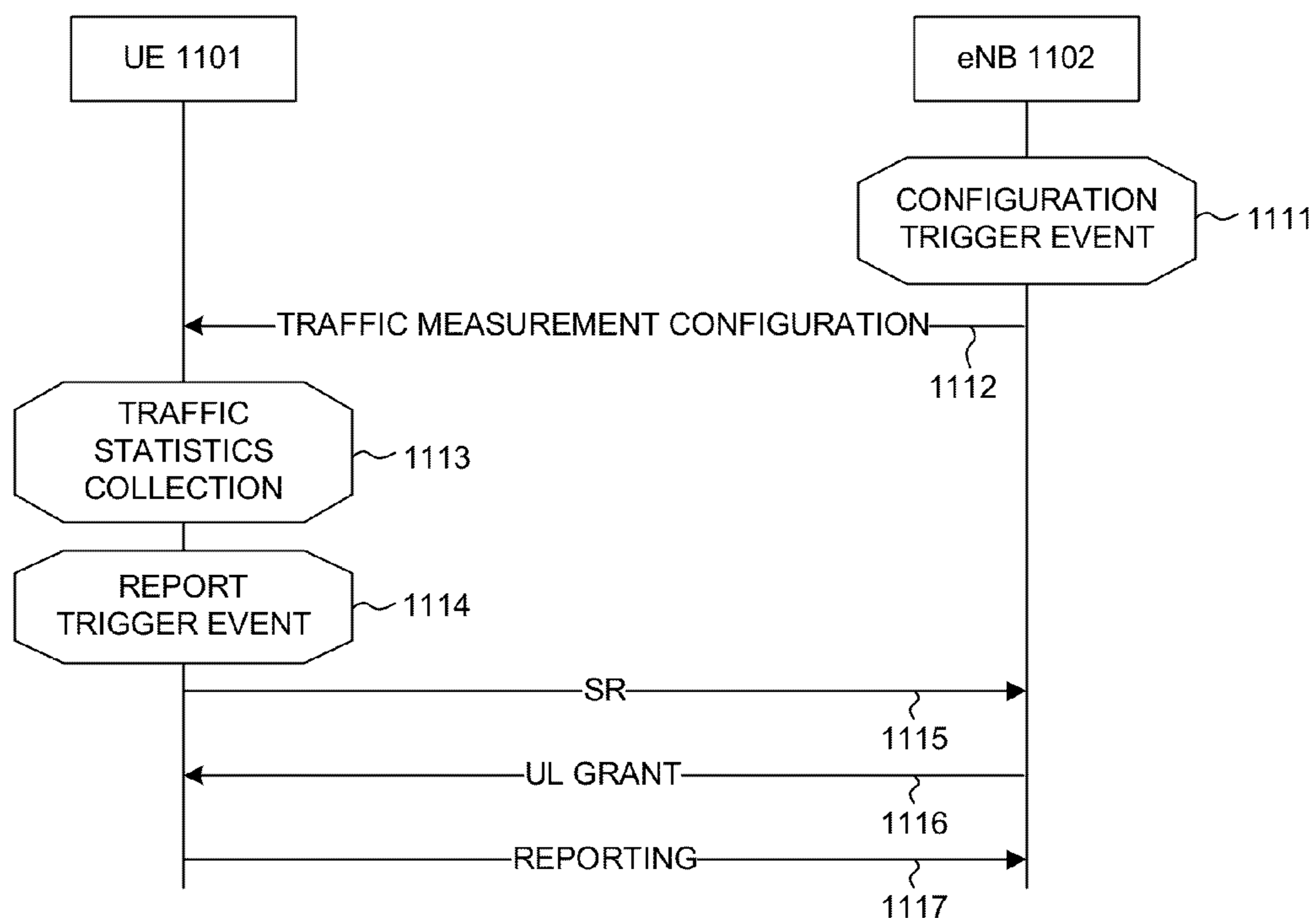
ENB-ORIENTED TRAFFIC STATISTICS #2 FIG. 11
