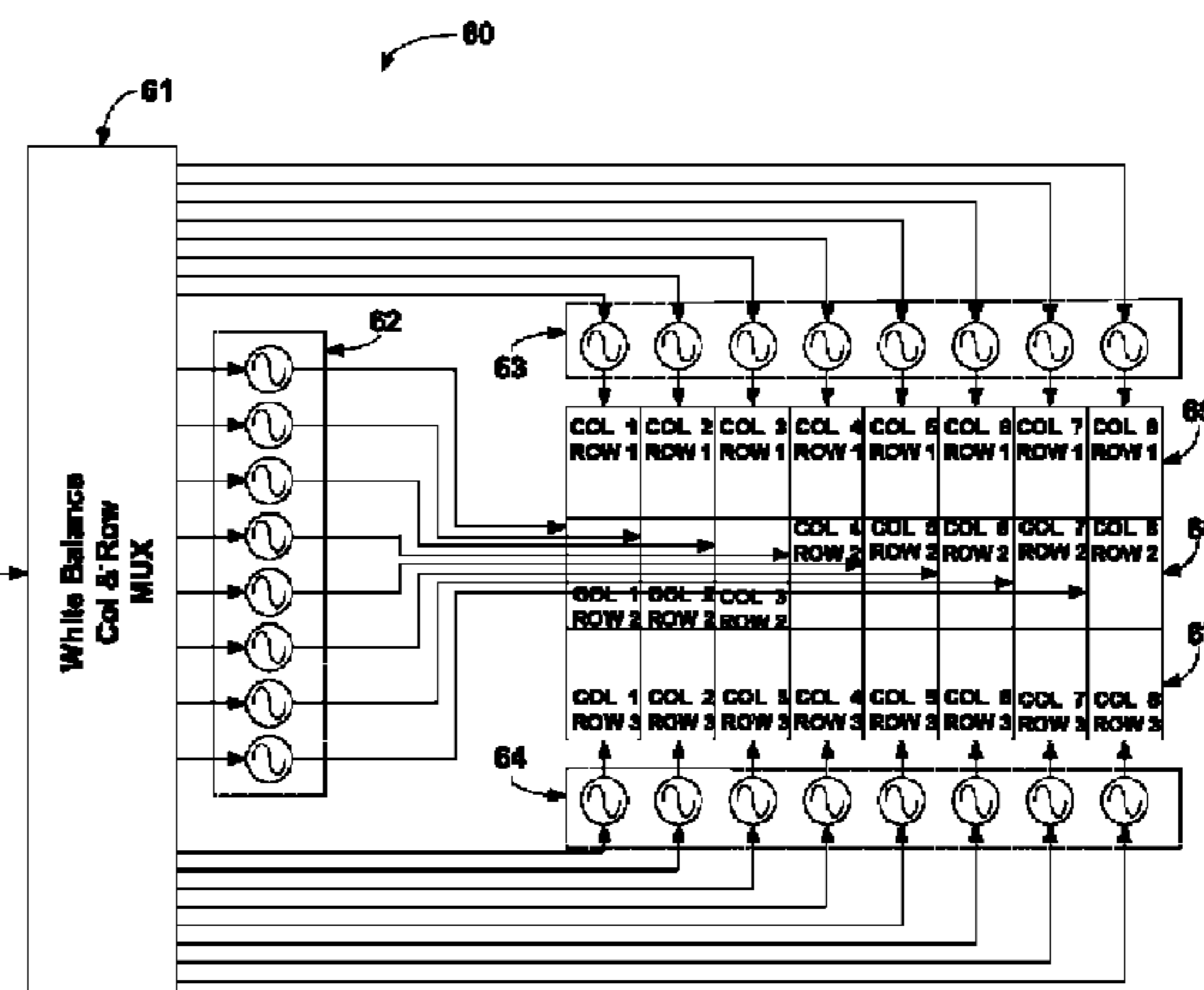
FIPEL Zone Dimming Color Balance Panel Back View
