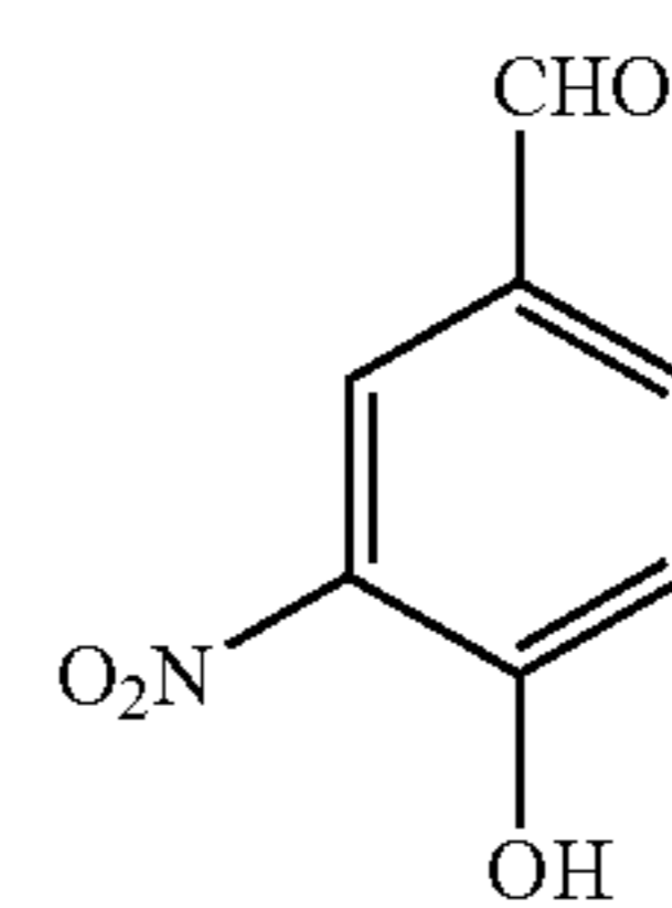
4-Hydroxy-3-Nitrobenzaldehyde (NHBA)
