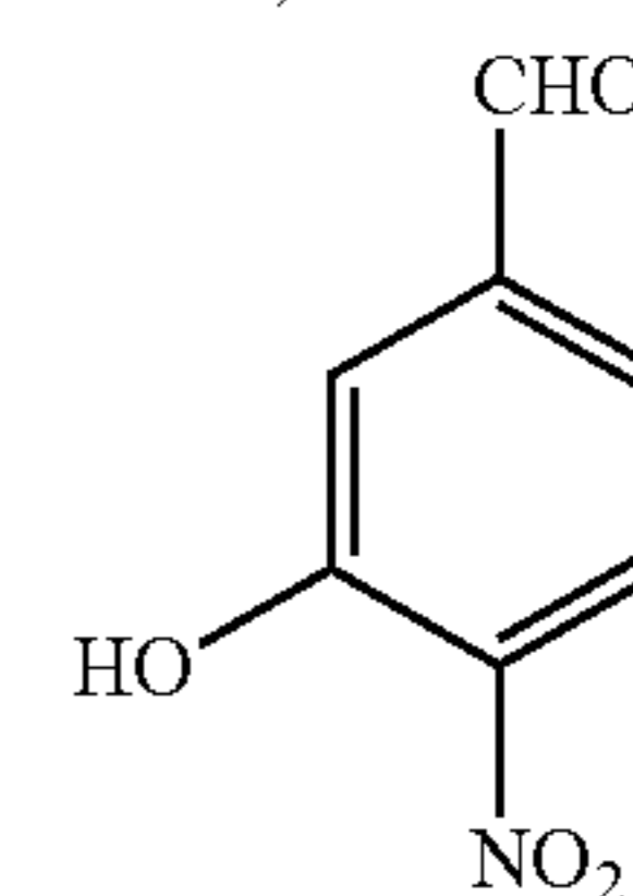
3-Hydroxy-4-Nitrobenzaldehyde (HNBA)
