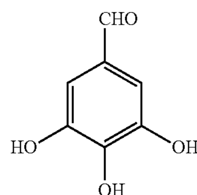
3,4,5-Trihydroxybenzaldehyde (THB—CHO)
