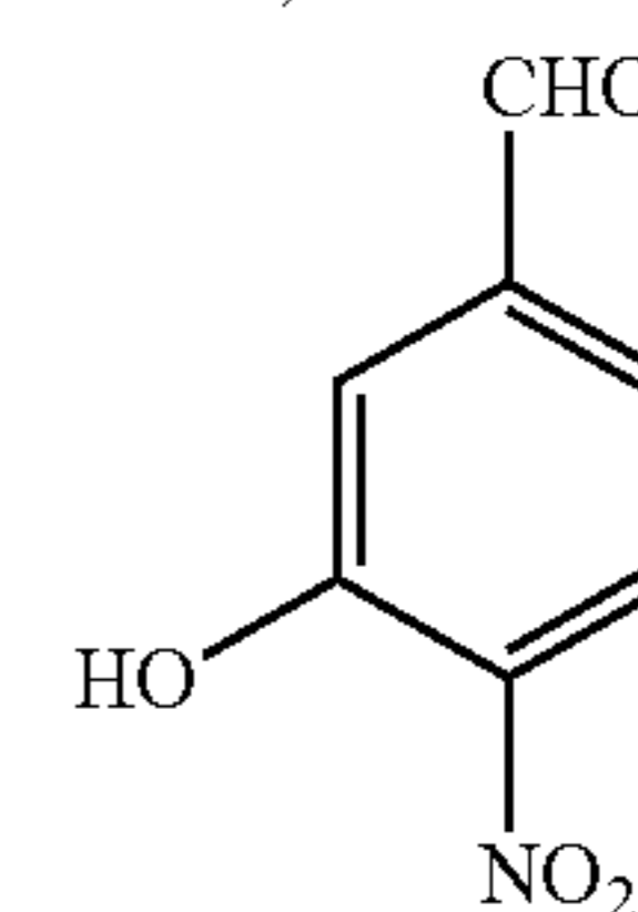
3-Hydroxy-4-Nitrobenzaldehyde (HNBA)
