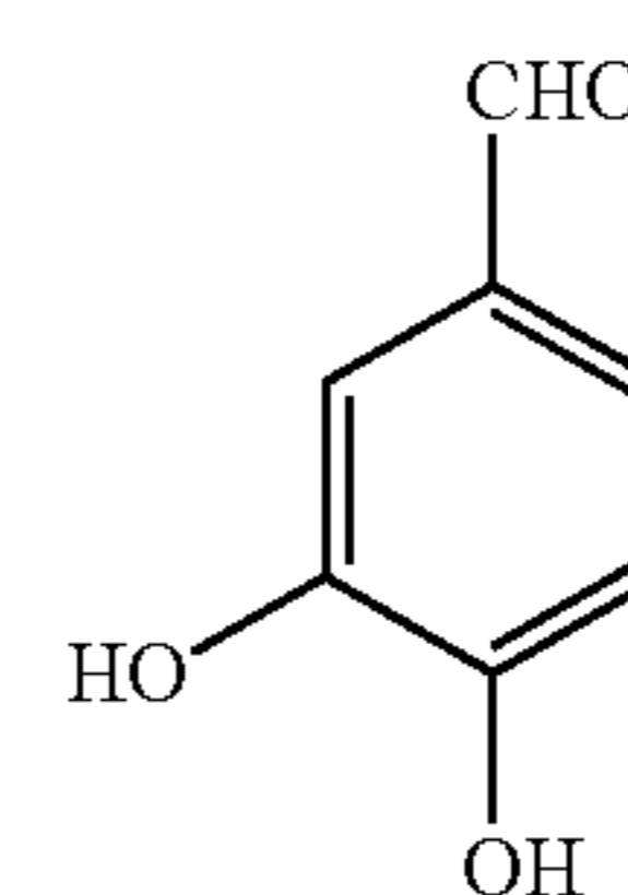
3,4-Dihydroxybenzaldehyde (DHB—CHO)
