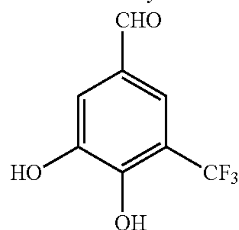
3,4-Dihydroxy-5-(trifluoromethyl)benzaldehyde
