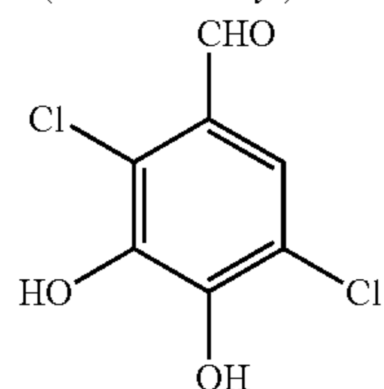
2,5-Dichloro-3,4-dihydroxybenzaldehyde
