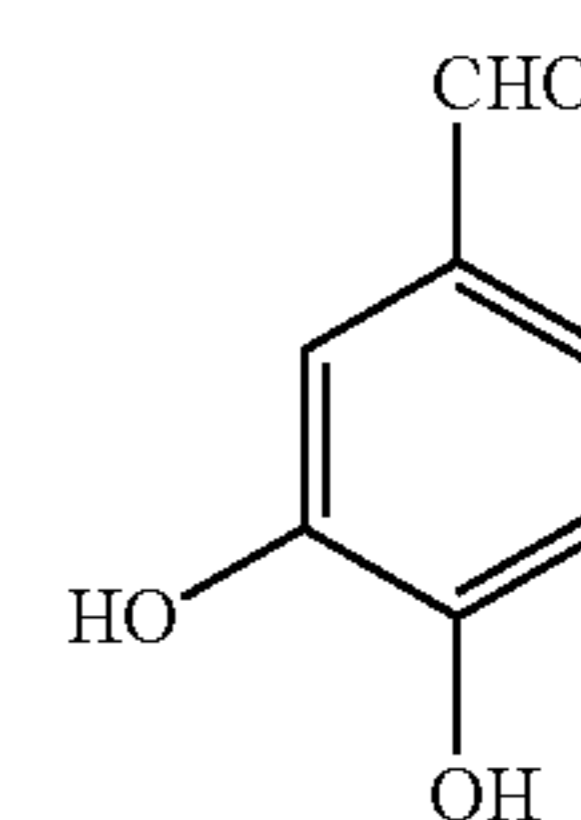
3,4-Dihydroxybenzaldehyde (DHB—CHO)
