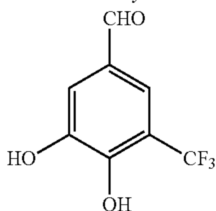
3,4-Dihydroxy-5-(trifluoromethyl)benzaldehyde
