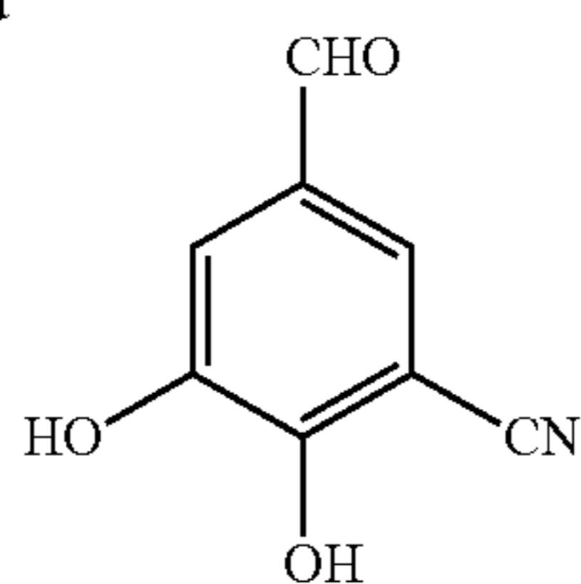
5-Formyl-2,3-dihydroxybenzonitrile
