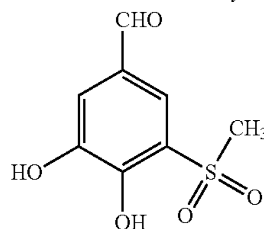
3,4-Dihydroxy-5-(methylsulfonyl)benzaldehyde
