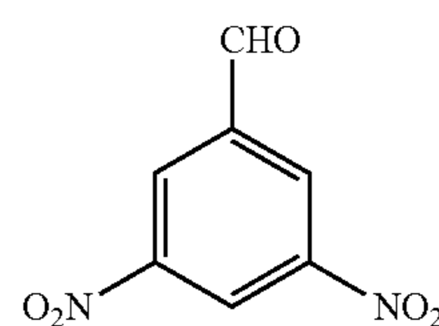
3,5-Dinitrobenzaldehyde
