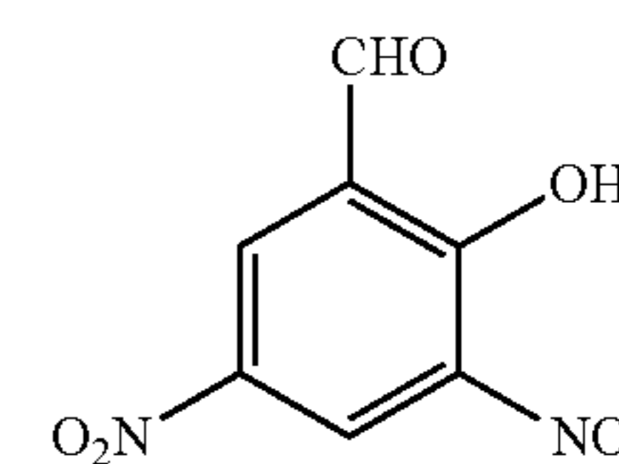
3,5-Dinitrosalicylaldehyde (DNSA)
