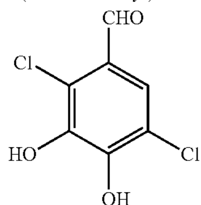
2,5-Dichloro-3,4-dihydroxybenzaldehyde
