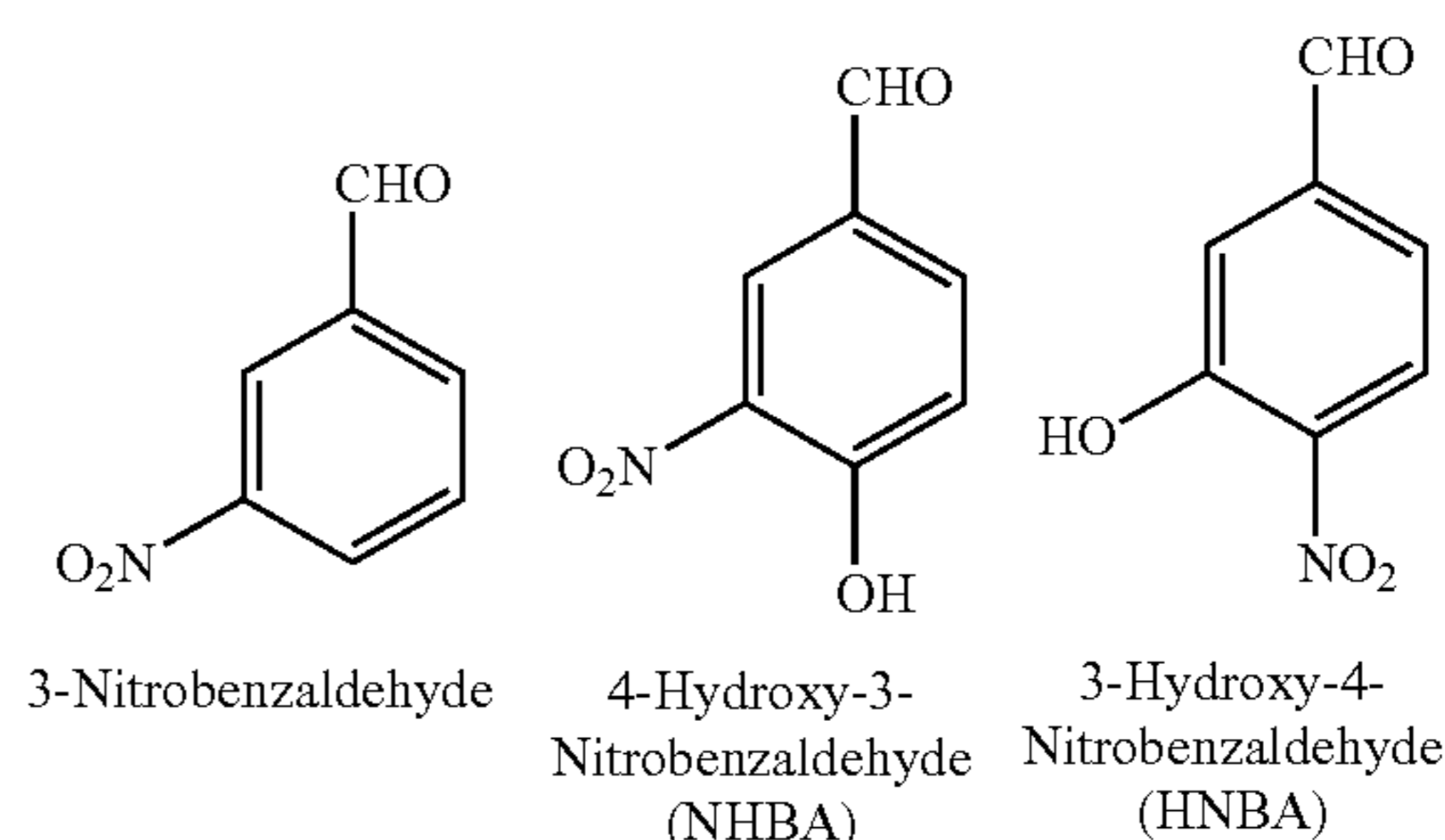
Scheme 2:
