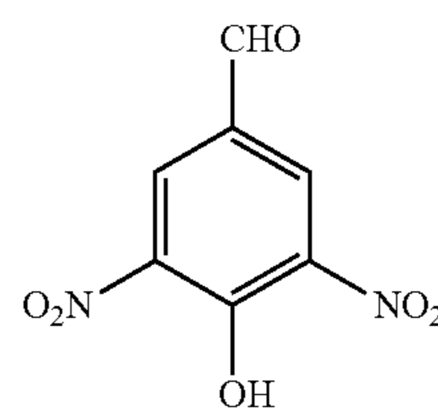
4-Hydroxy-3,5-Dinitrobenzaldehyde (DNHBA)
