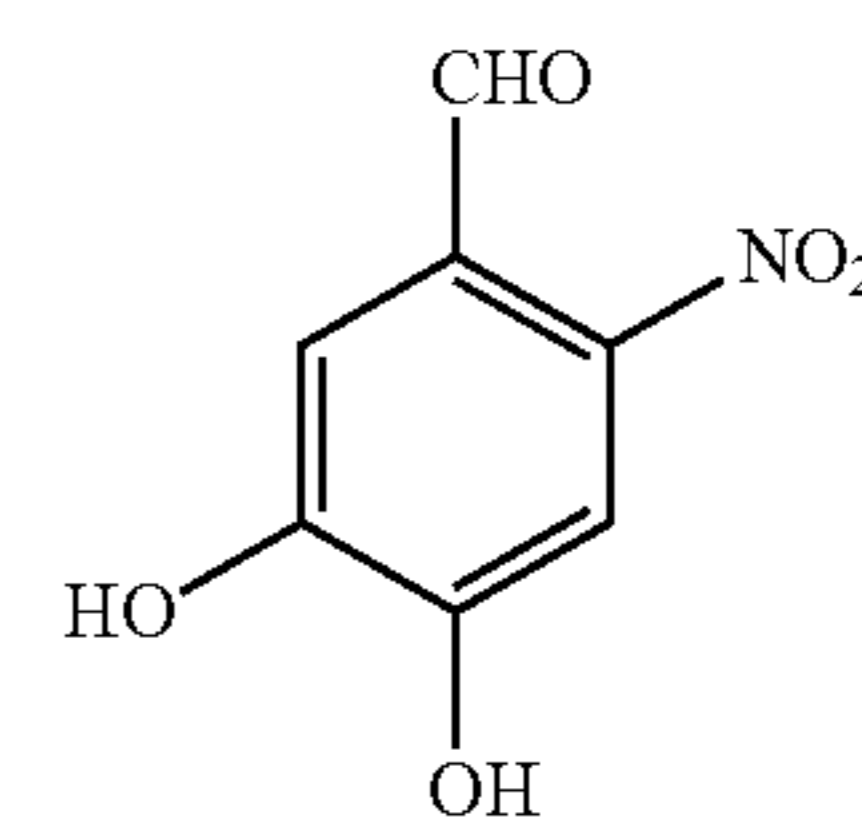
3,4-Dihydroxy-6-nitrobenzaldehyde (DH6NB)
