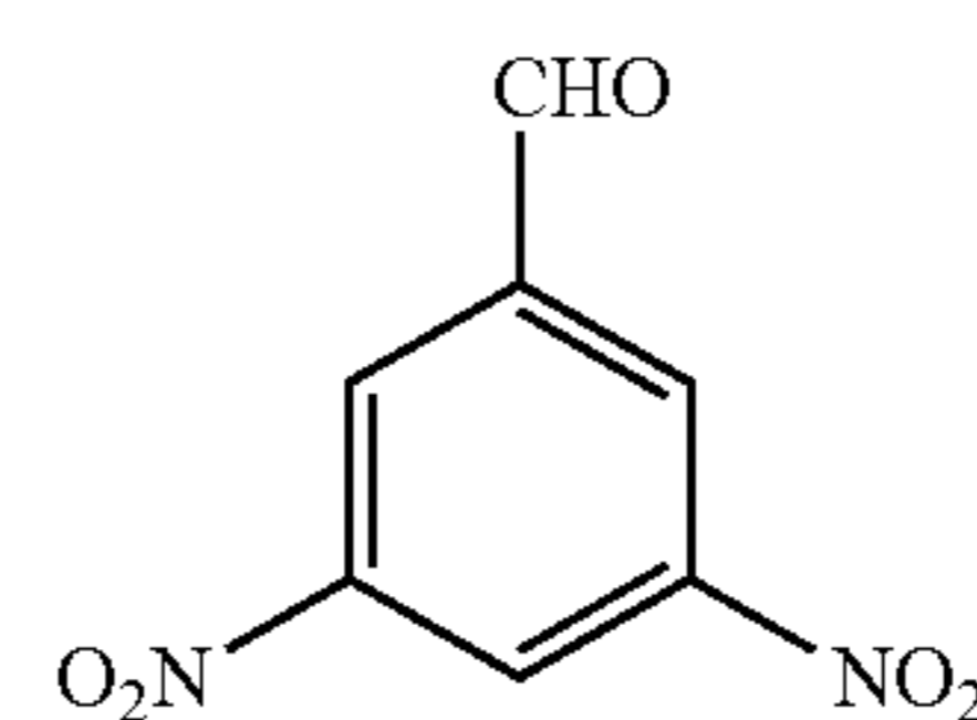
3,5-Dinitrobenzaldehyde
