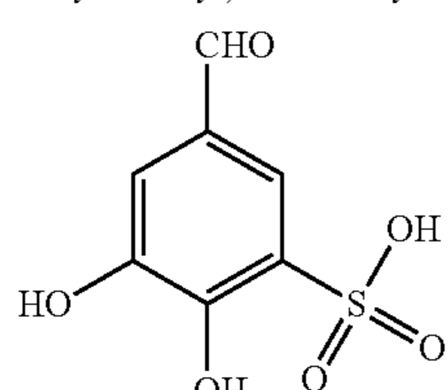
5-formyl-2,3-dihydroxybenzenesulfonic acid
