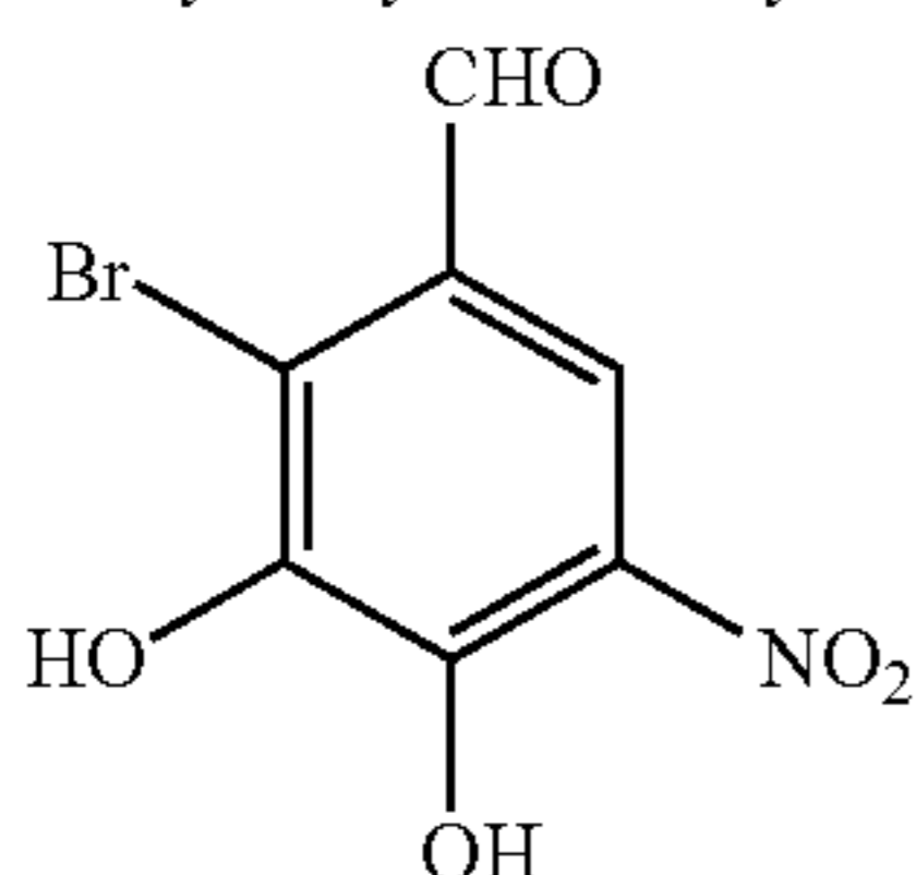
2-Bromo-3,4-dihydroxy-5-nitrobenzaldehyde
