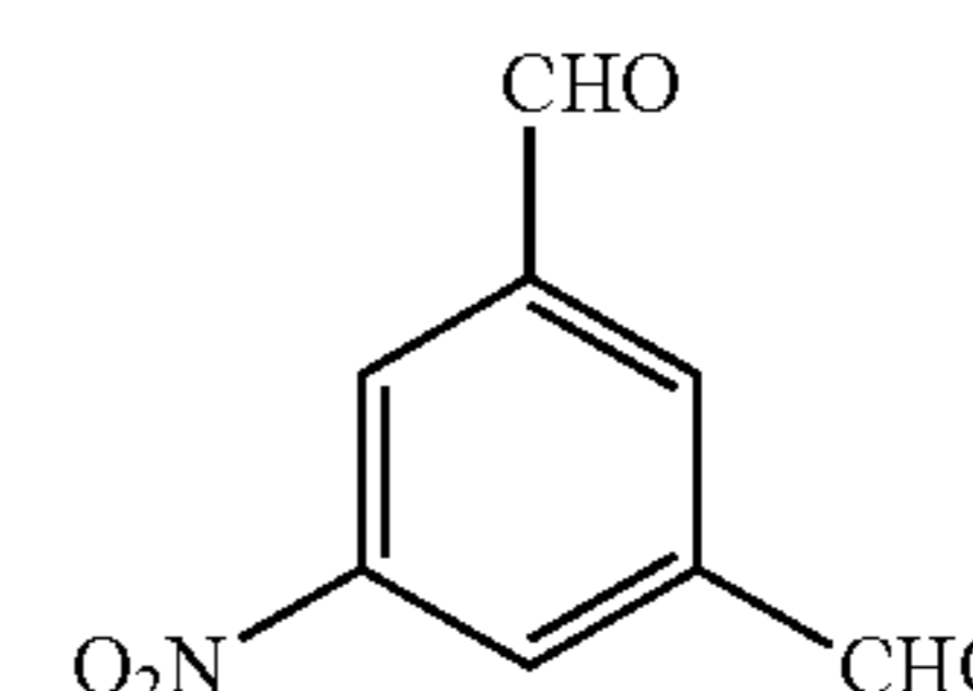
3-Nitro-m-Phthalaldehyde
