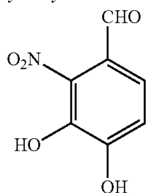
3,4-Dihydroxy-2-nitrobenzaldehyde
