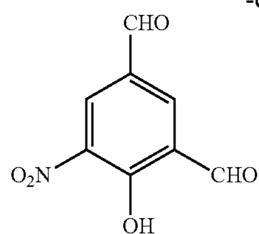
4-Hydroxy-3-Nitro-m-Phthalaldehyde
