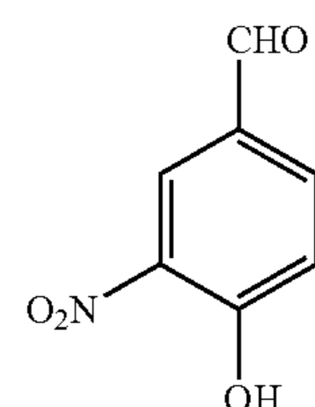
4-Hydroxy-3-Nitrobenzaldehyde (NHBA)
