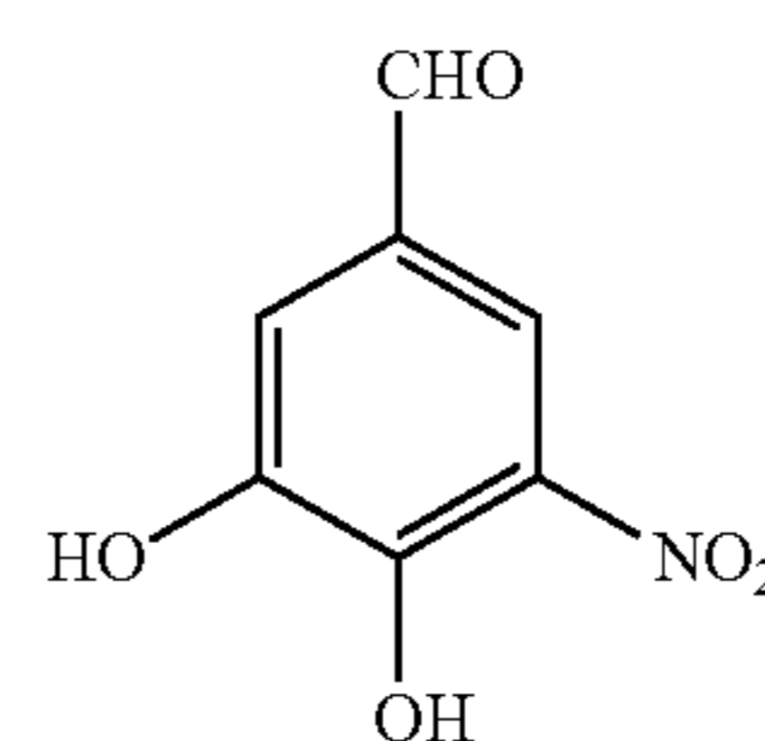
3,4-Dihydroxy-5-nitrobenzaldehyde (DHNB)
