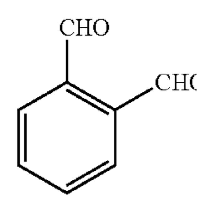
Phthalaldehyde
