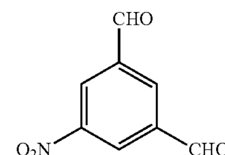
3-Nitro-m-Phthalaldehyde
