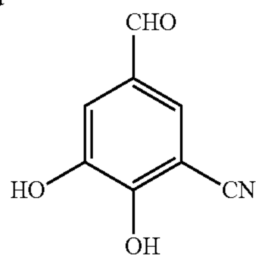
5-Formyl-2,3-dihydroxybenzonitrile
