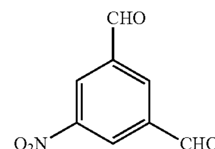
3-Nitro-m-Phthalaldehyde
