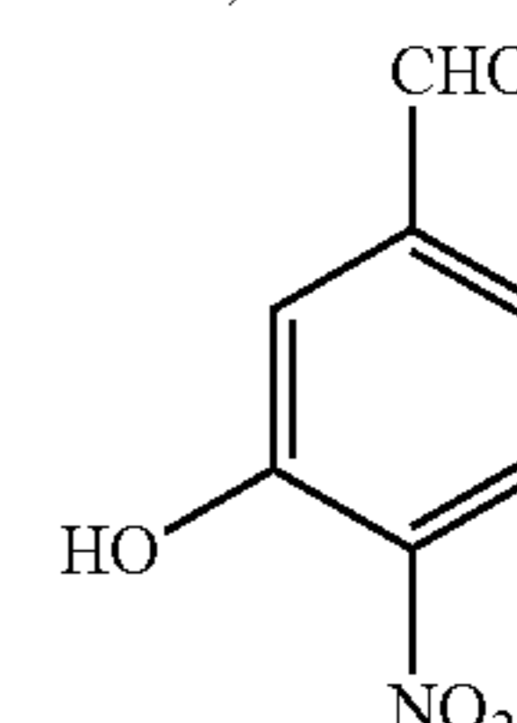
3-Hydroxy-4-Nitrobenzaldehyde (HNBA)
