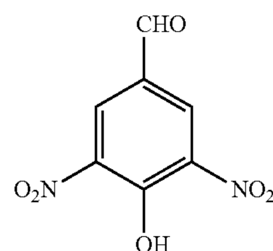
4-Hydroxy-3,5-Dinitrobenzaldehyde (DNHBA)
