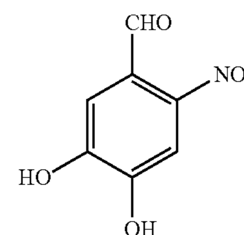
3,4-Dihydroxy-6-nitrobenzaldehyde (DH6NB)
