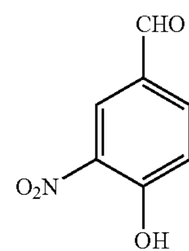
4-Hydroxy-3-Nitrobenzaldehyde (NHBA)
