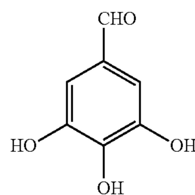
3,4,5-Trihydroxybenzaldehyde (THB—CHO)
