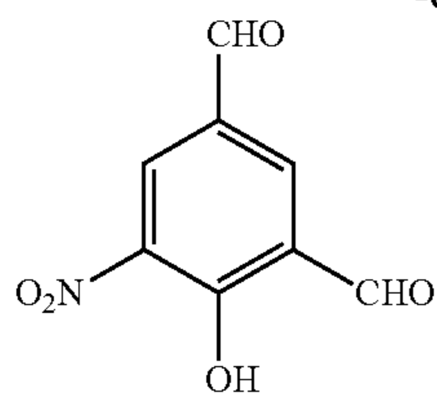
4-Hydroxy-3-Nitro-m-Phthalaldehyde
