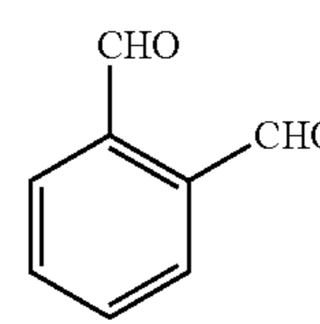
Phthalaldehyde
