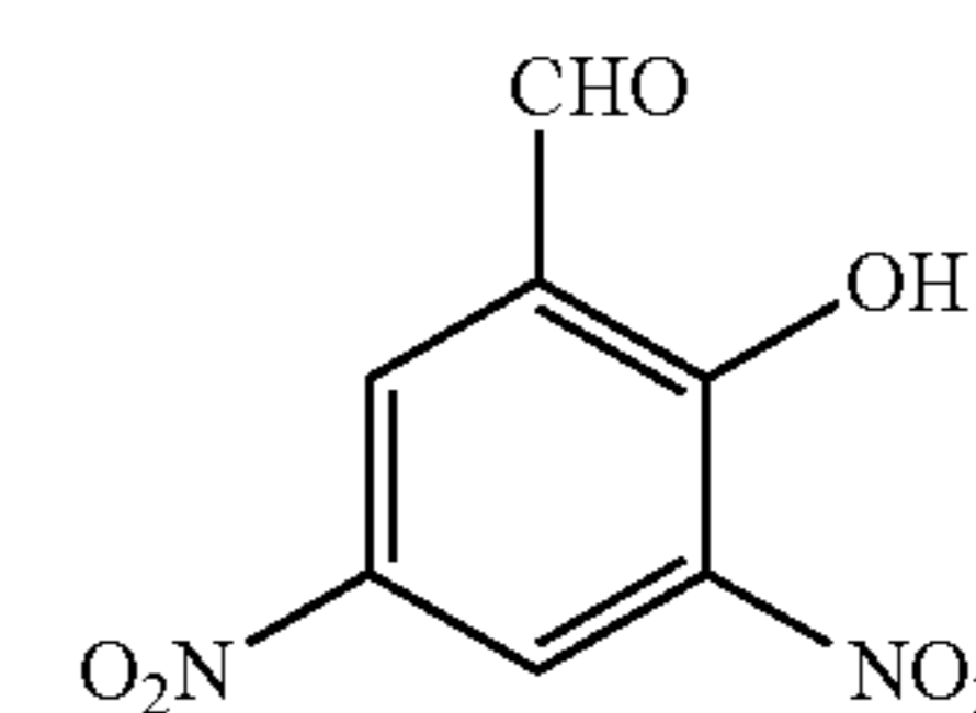
3,5-Dinitrosalicylaldehyde (DNSA)
