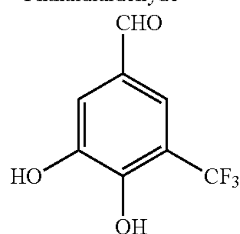
3,4-Dihydroxy-5-(trifluoromethyl)benzaldehyde
