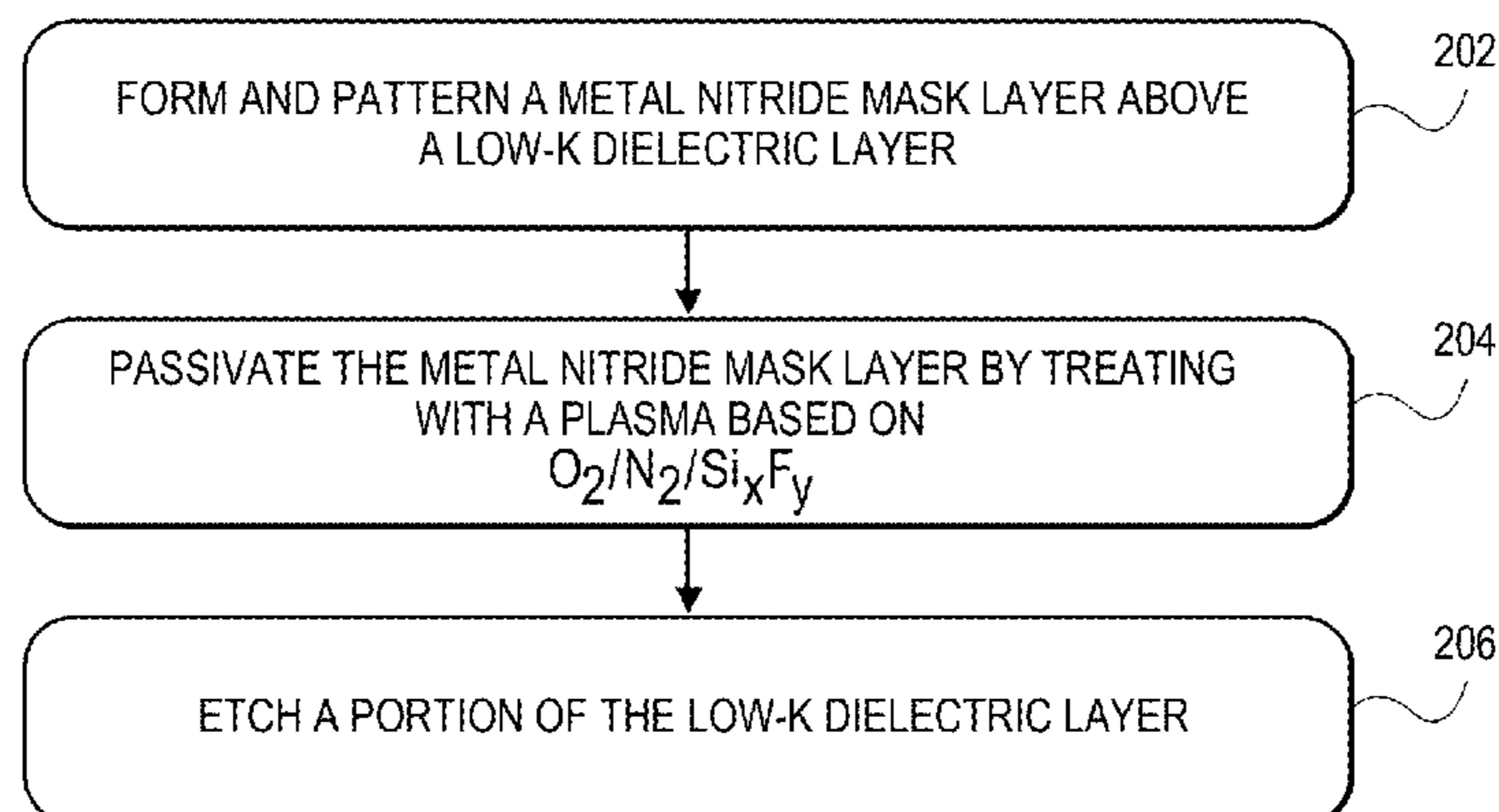
FLOWCHART 200
