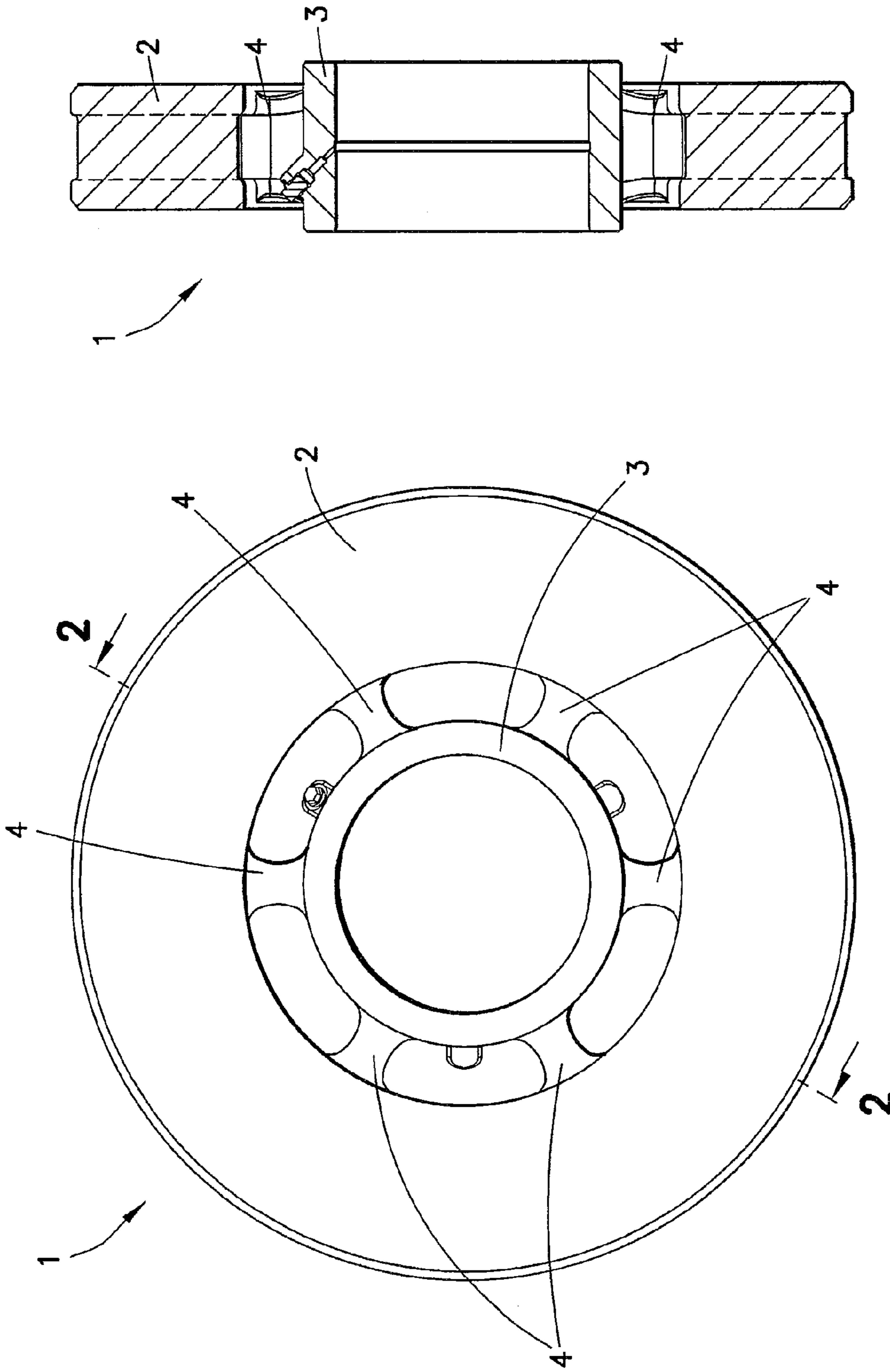
FIG. 2 PRIOR ART
