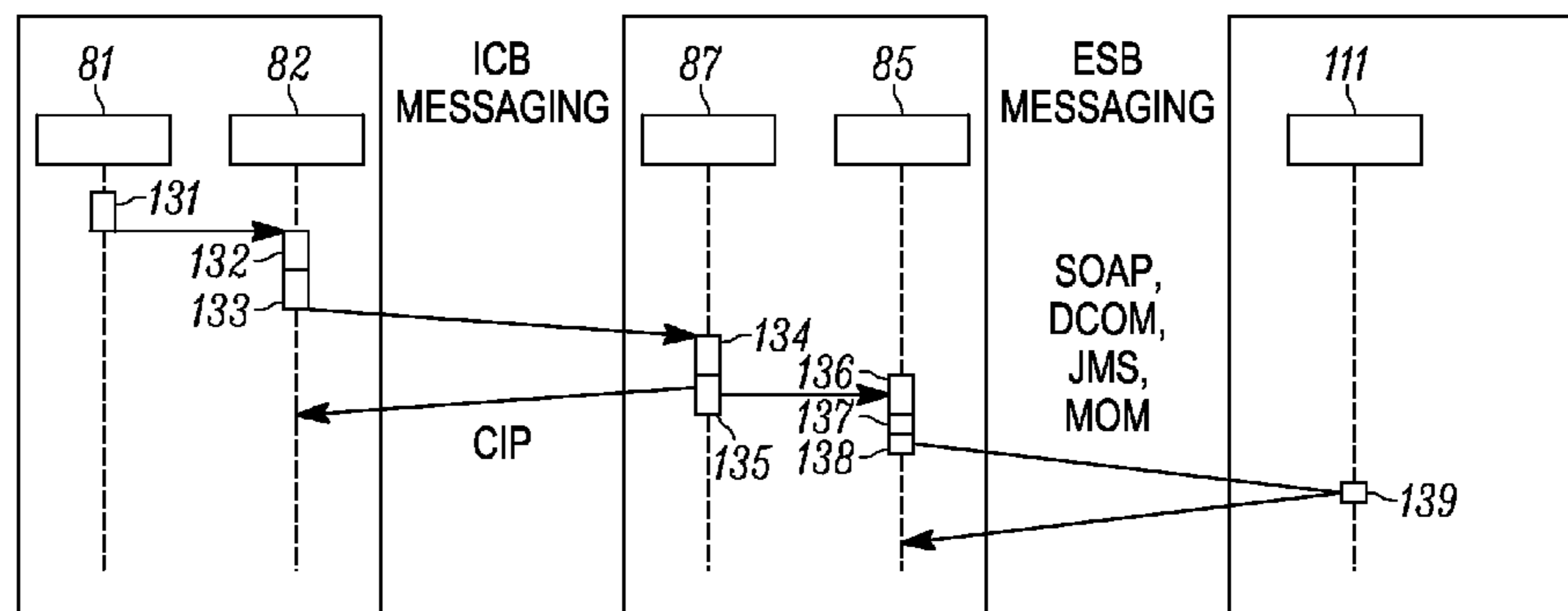
Controller to Enterprise Messaging Pattern
