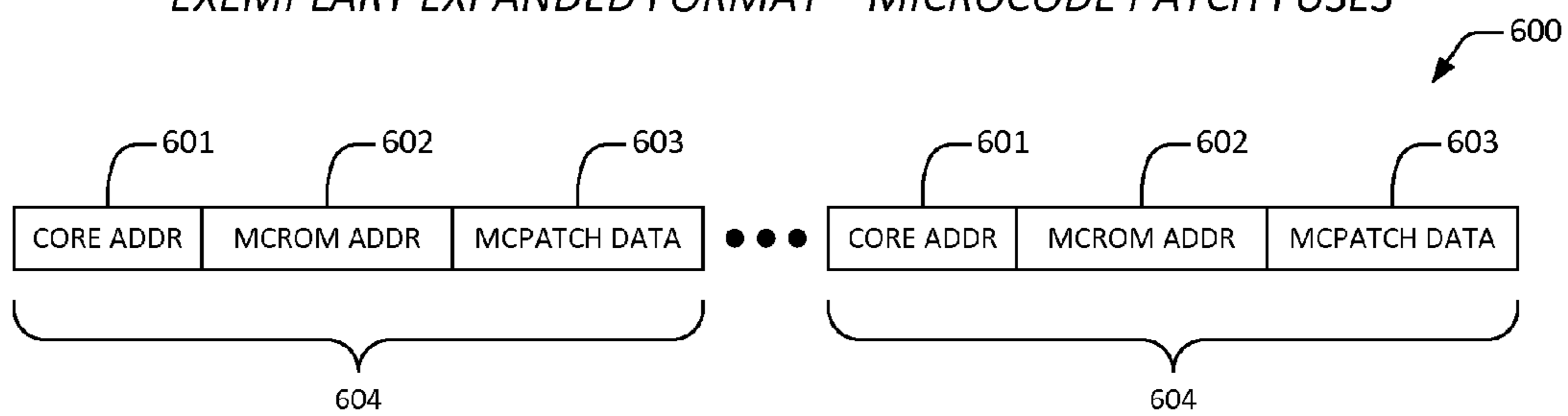
EXEMPLARY EXPANDED FORMAT – MICROCODE PATCH FUSES
