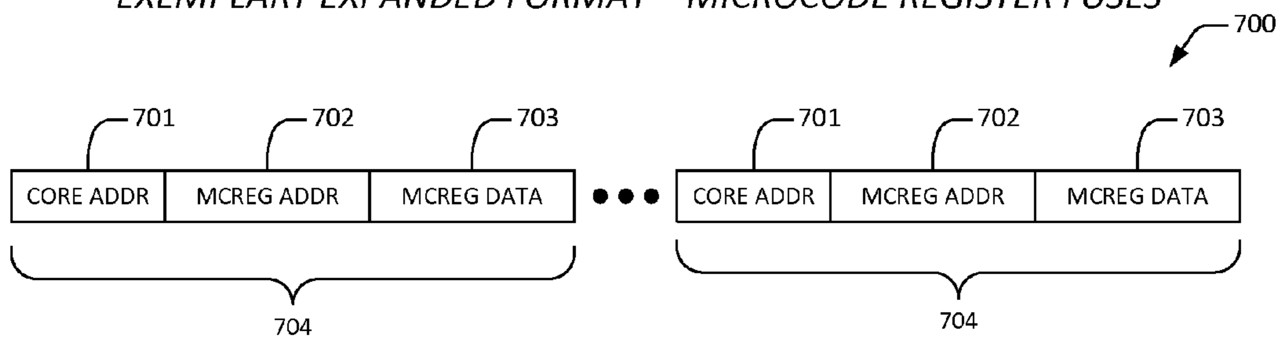
EXEMPLARY EXPANDED FORMAT – MICROCODE REGISTER FUSES
