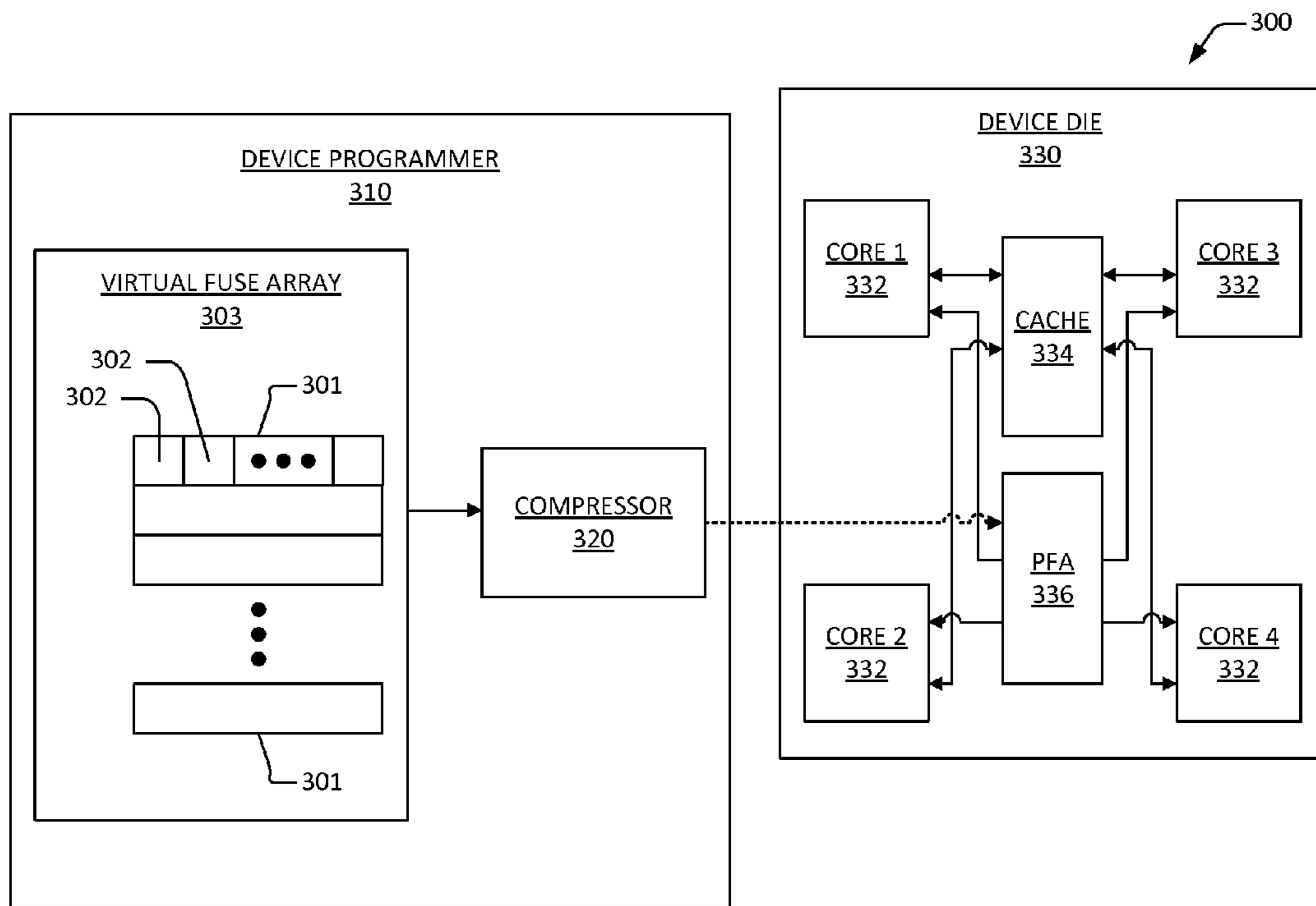
MICROPROCESSOR FUSE ARRAY COMPRESSION SYSTEM
