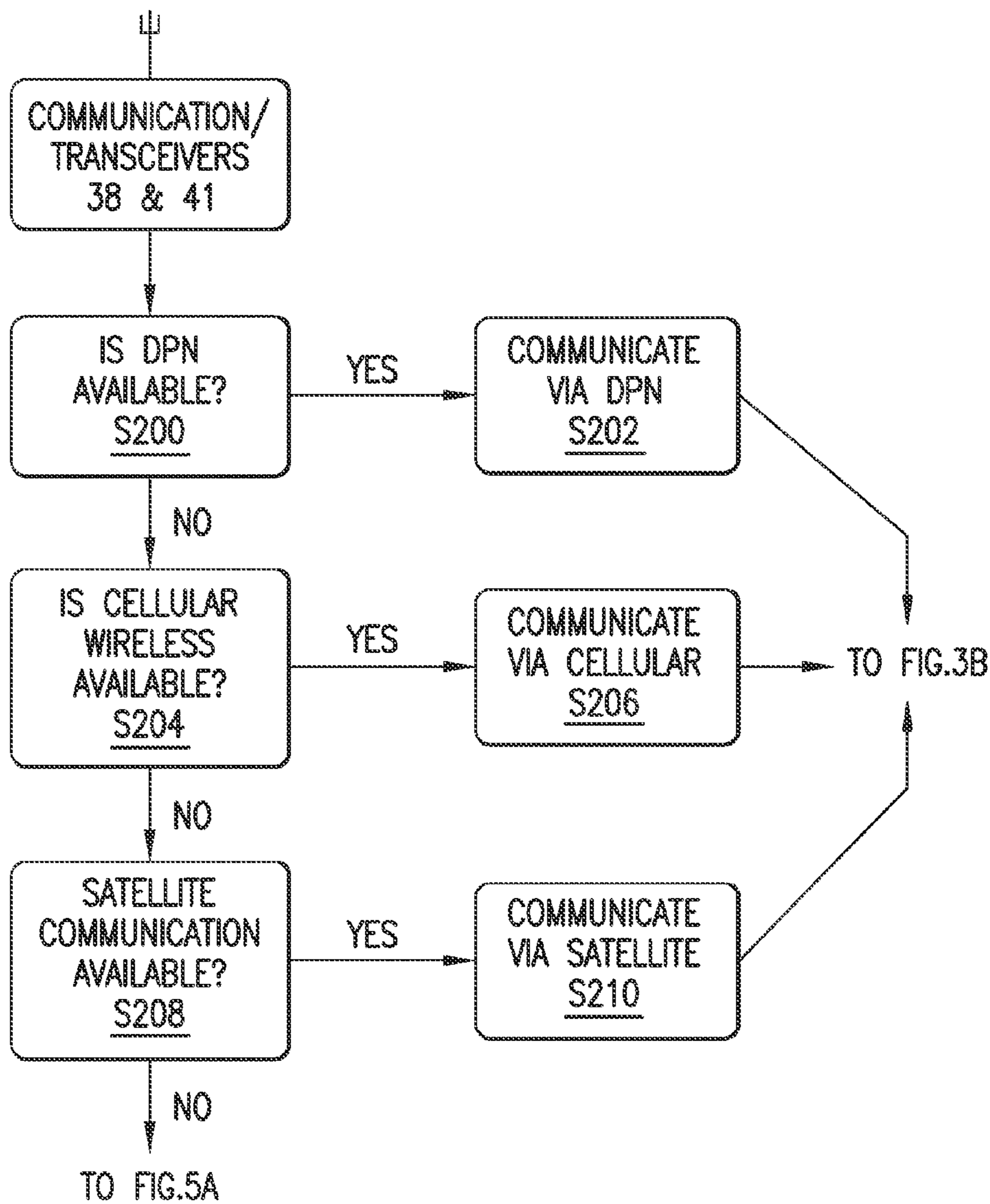
COMMUNICATION SUB-ROUTINE
