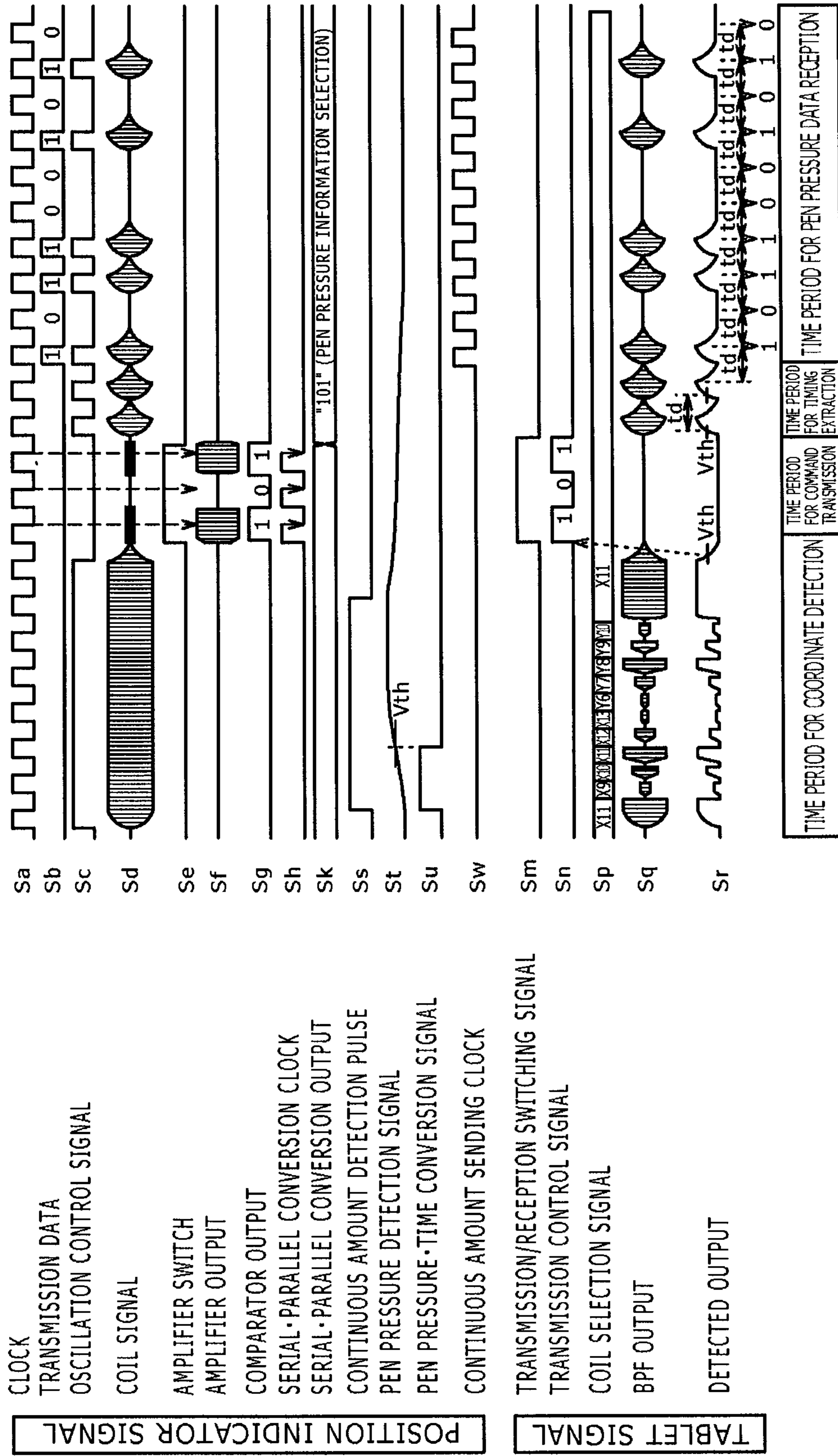
FIG. 6 OPERATION WHEN COMMAND "101" IS TRANSMITTED
