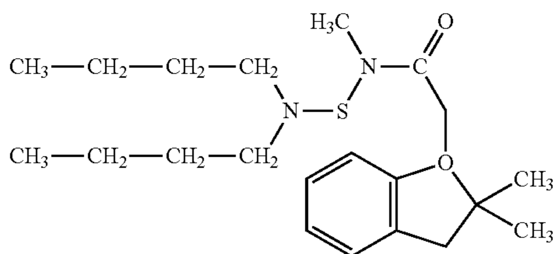
Carbosulfan
