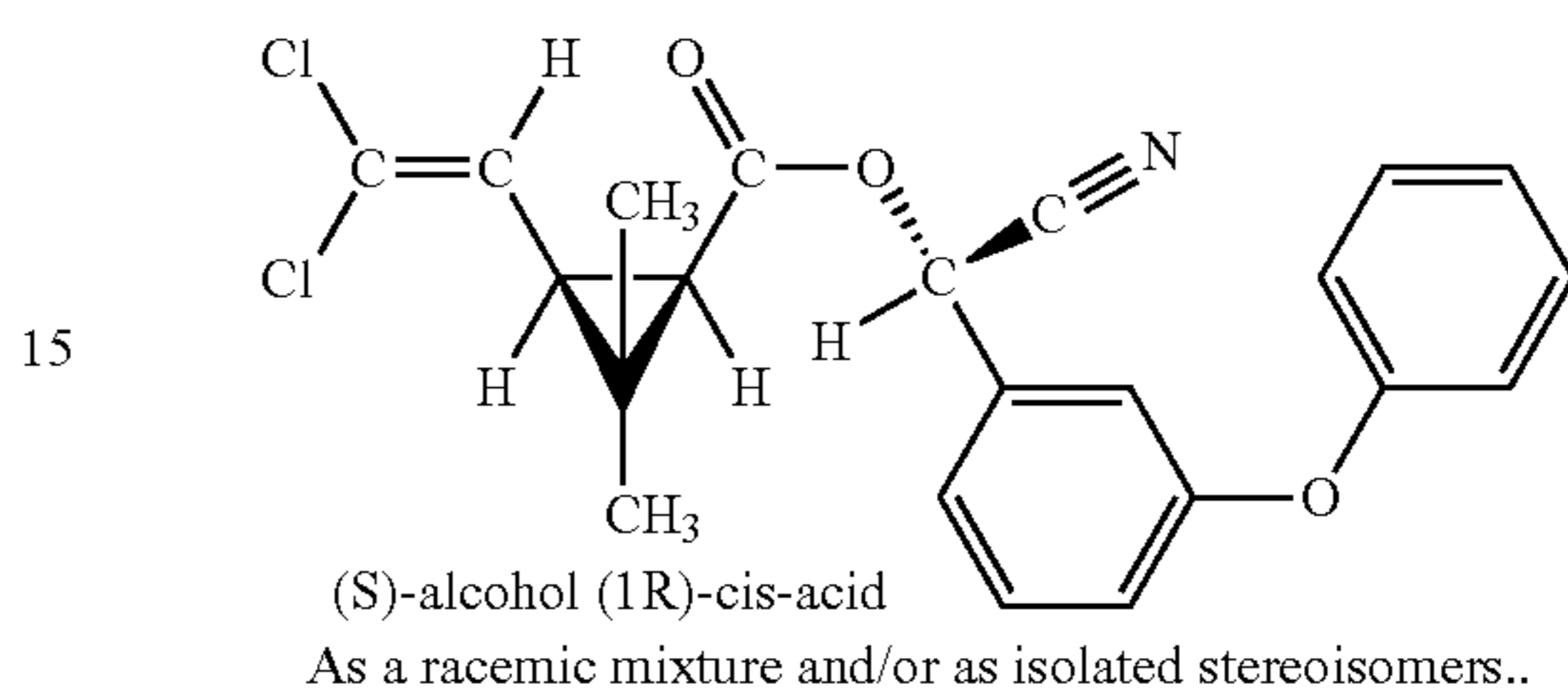
alpha-cypermethrin
