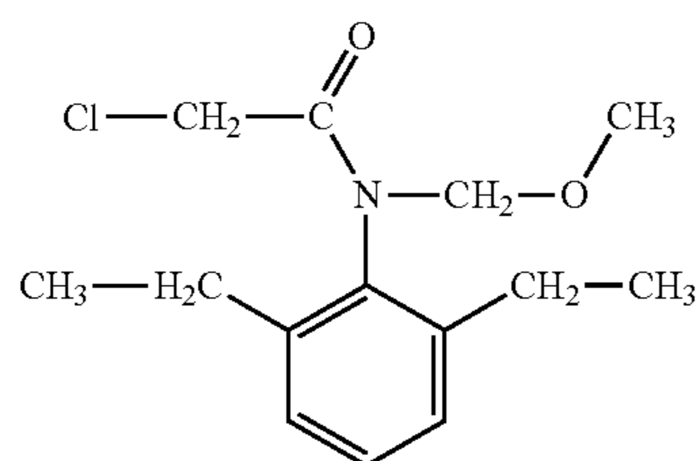
Alachlor
