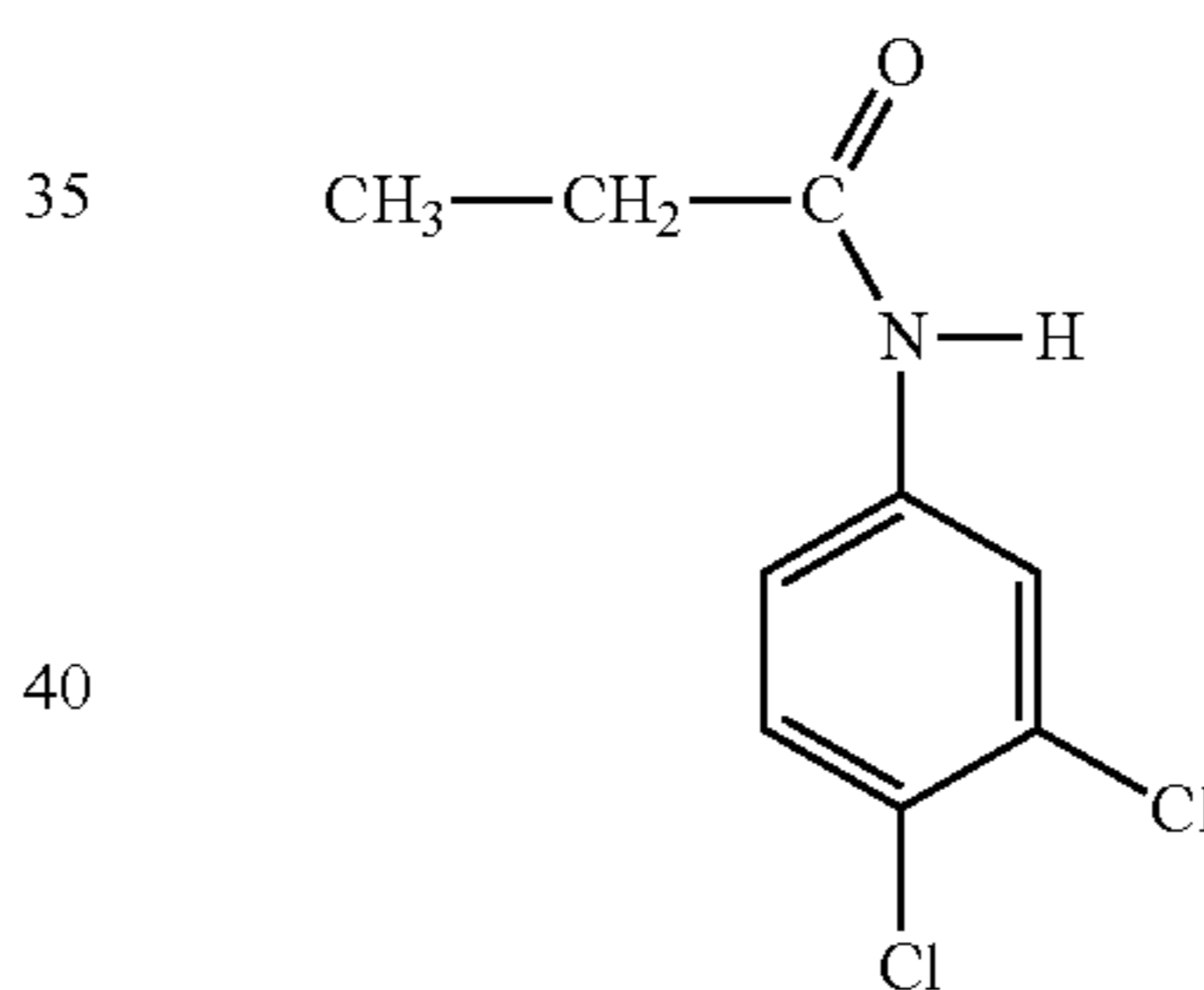
Propanil
