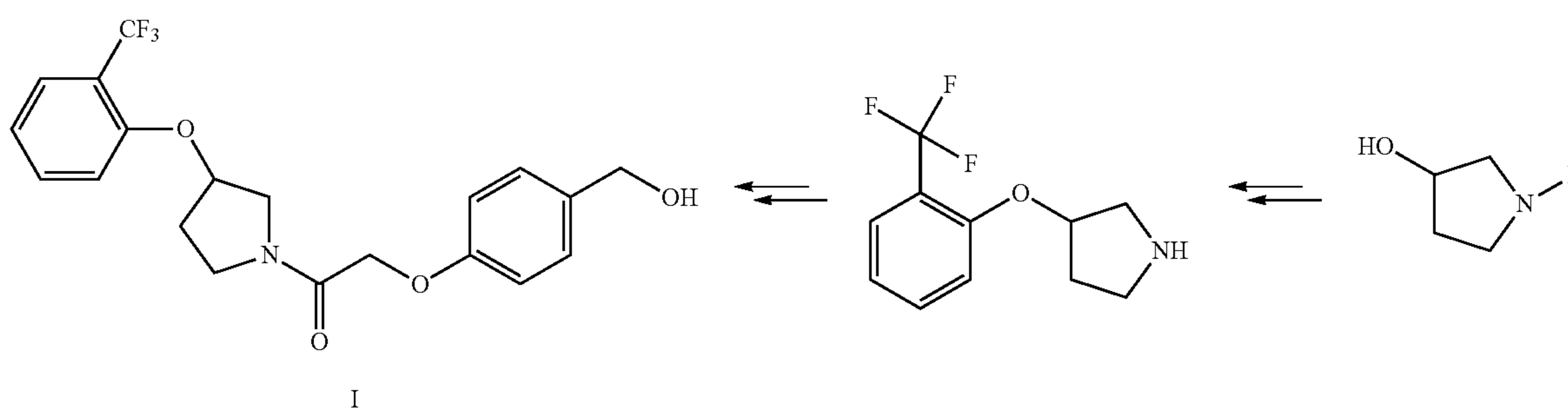
Scheme IV
