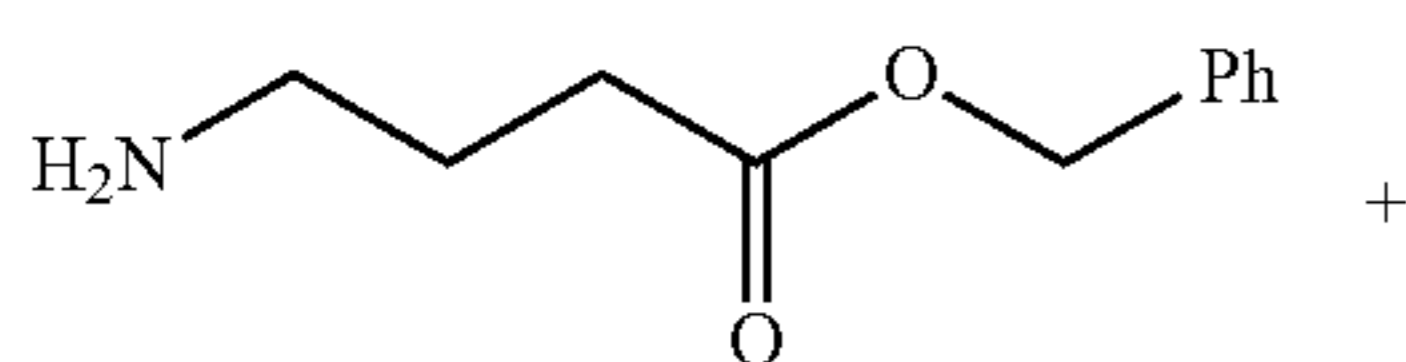
Scheme 4. Synthesis of locking module.
