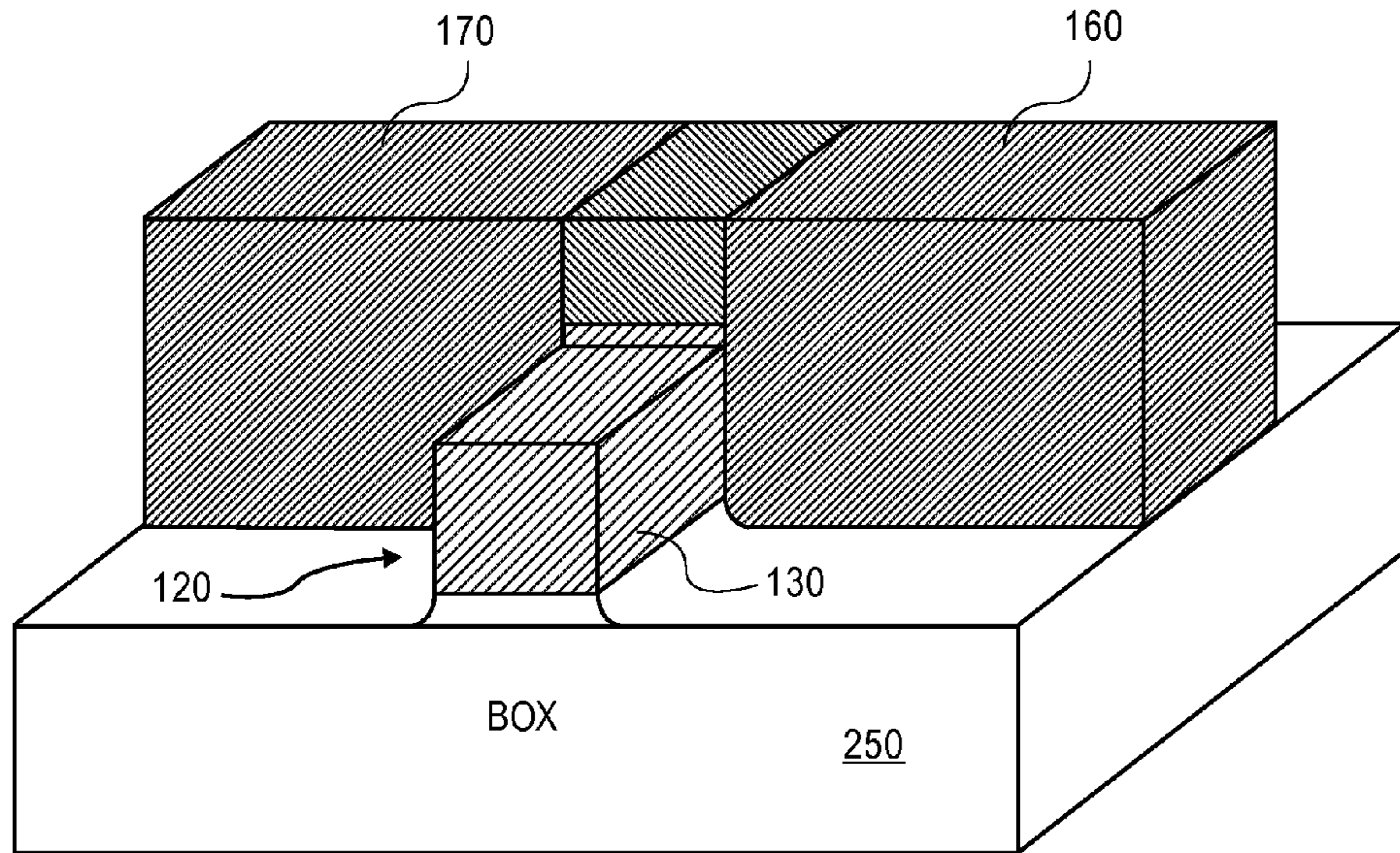
FIG. 2 (PRIOR ART)
