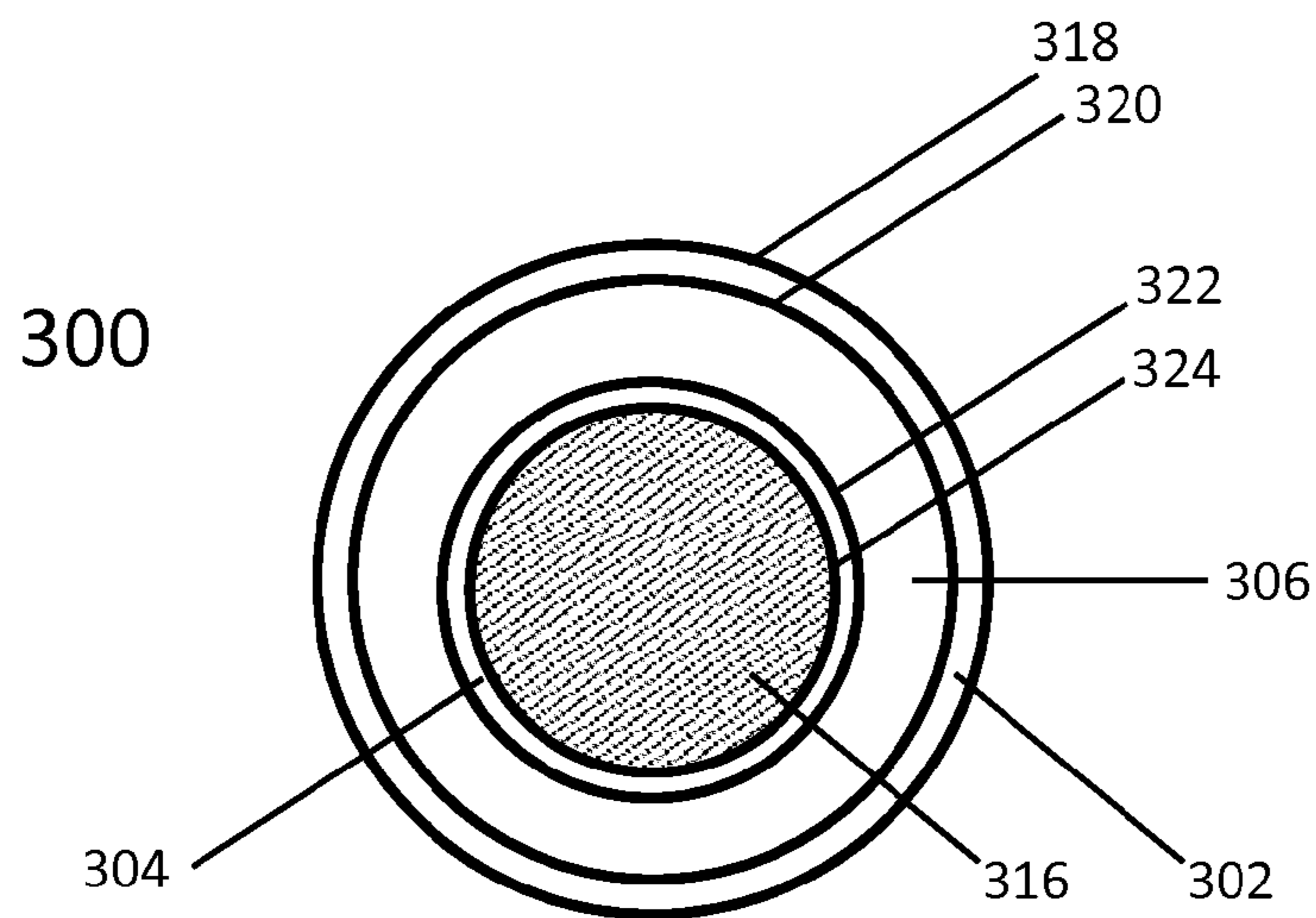
Cross-sectional view
