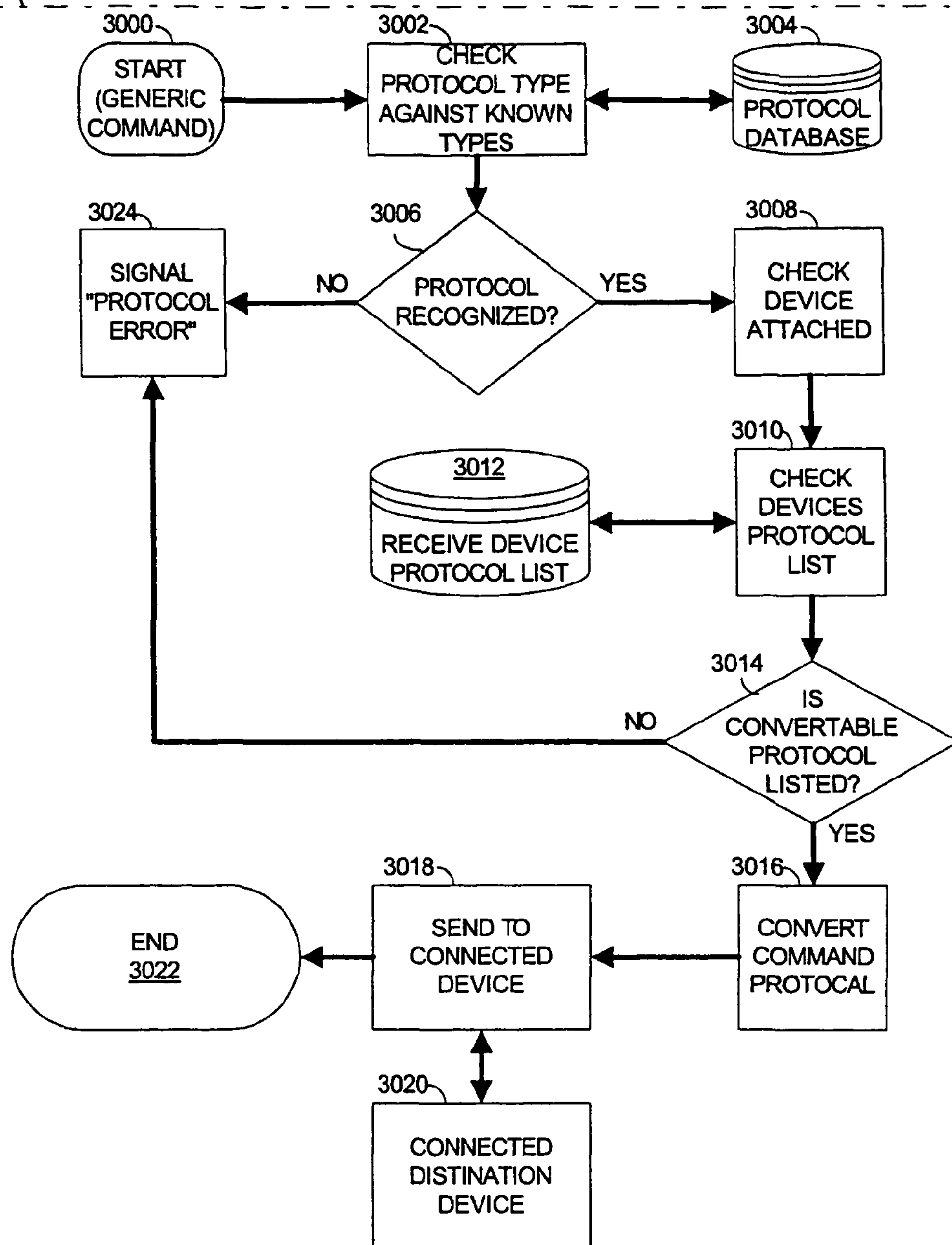
906 STANDARDIAZTION/CONVERSION SOFTWARE FIG. 30
