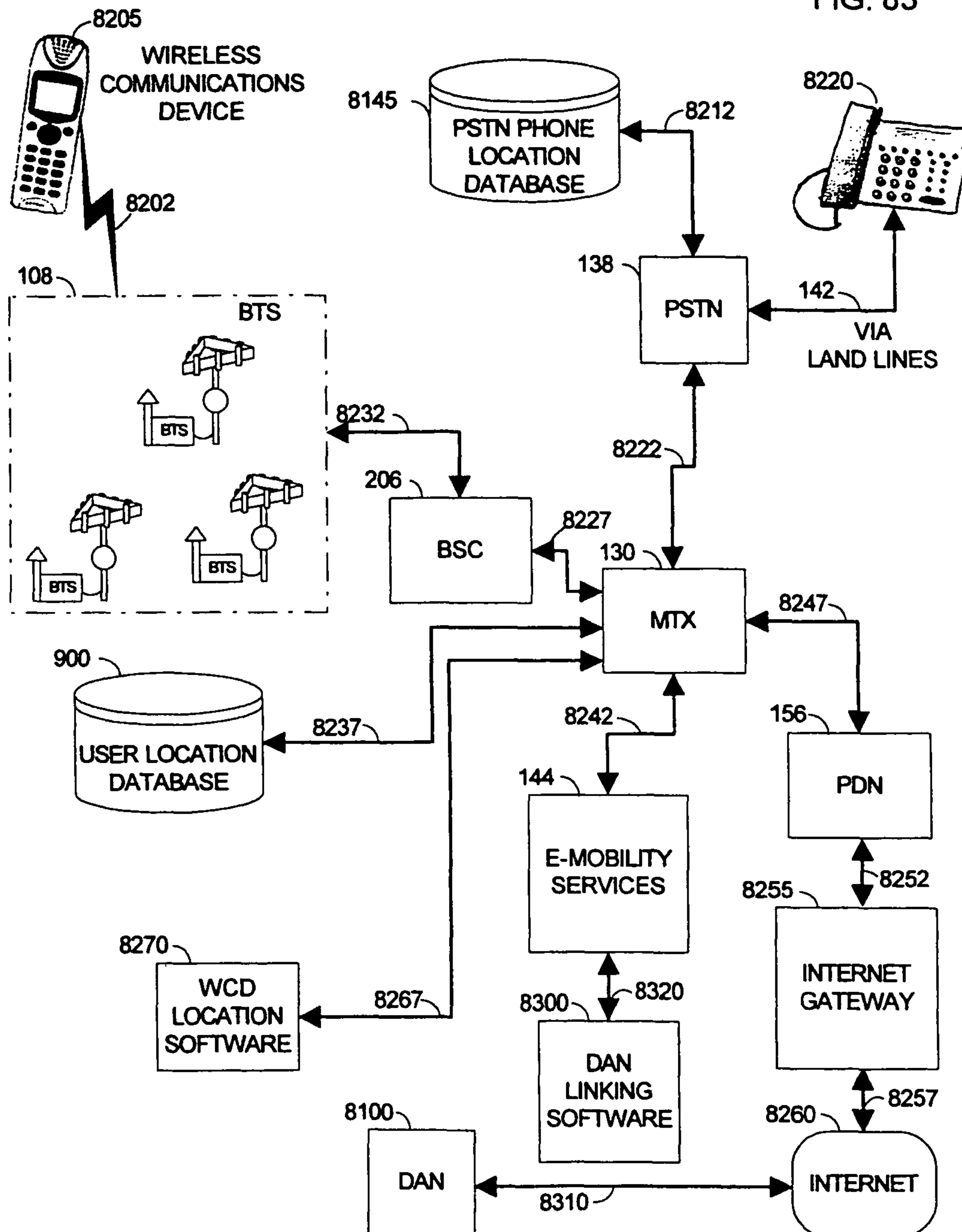
PRIMARY EMBODIMENT'S ALTERNATE LOCATION ON A TYPICAL 2/3G CELLULAR NETWORK
