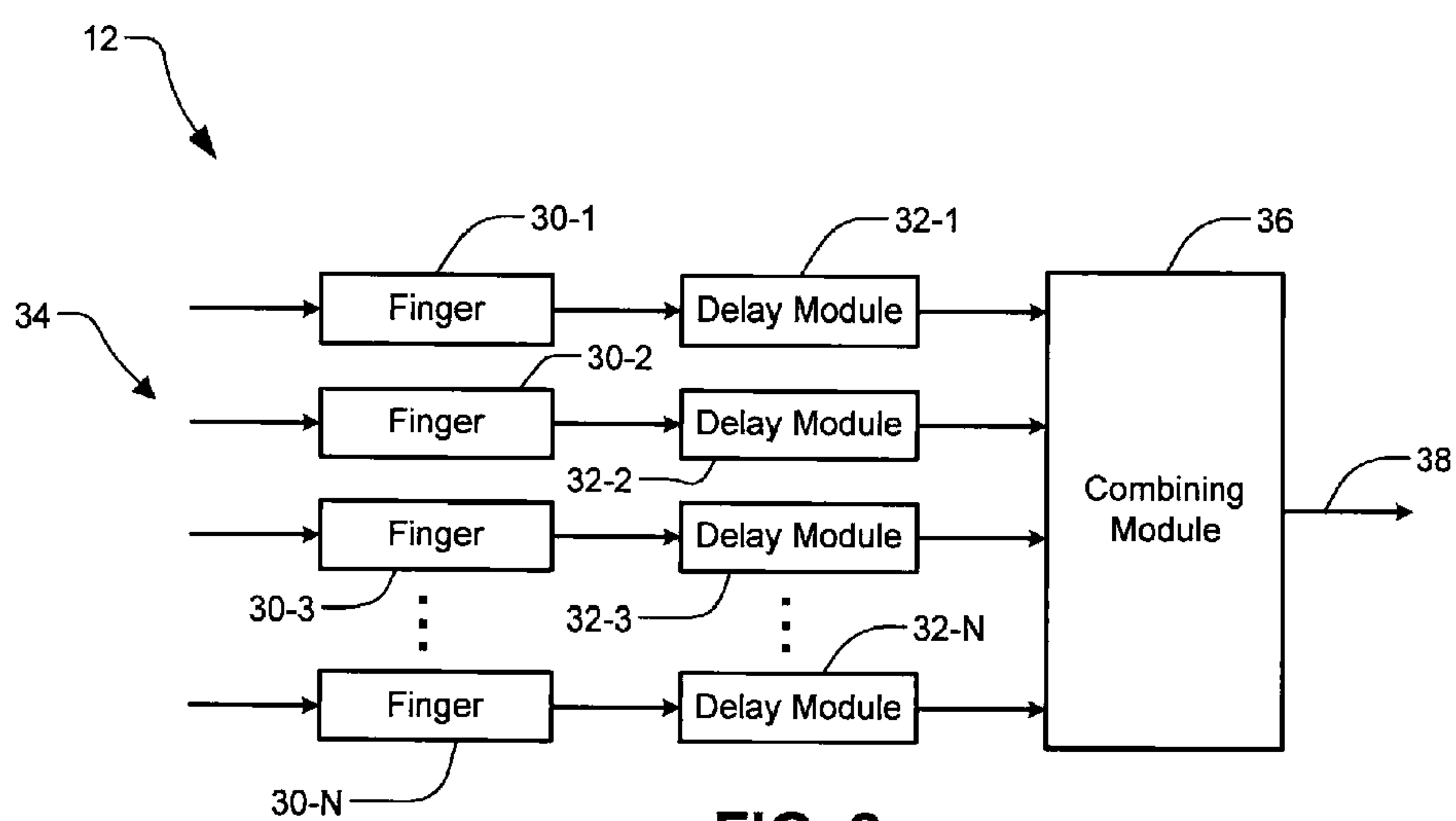
FIG. 2 Prior Art
