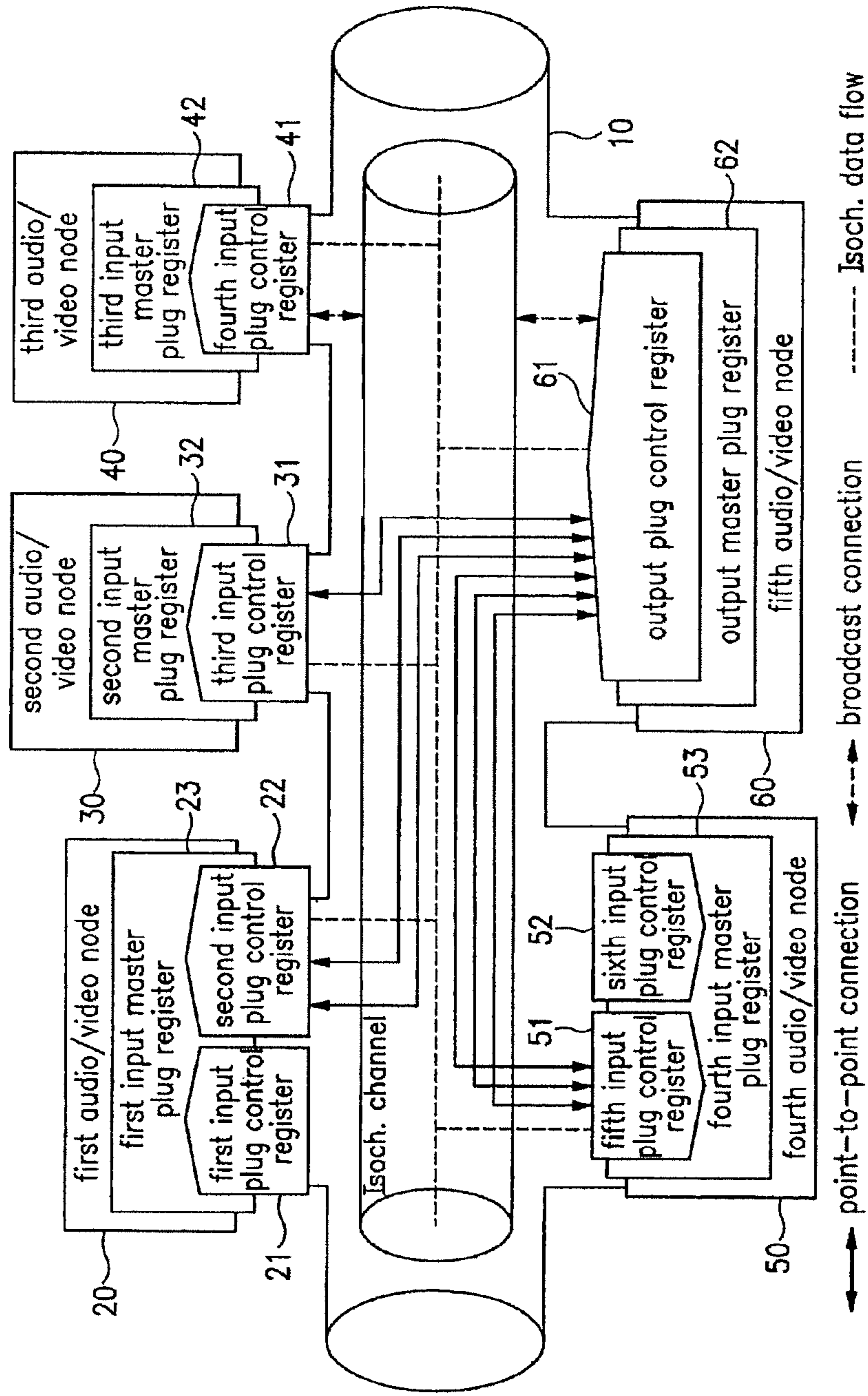
FIG. 1 Related Art
