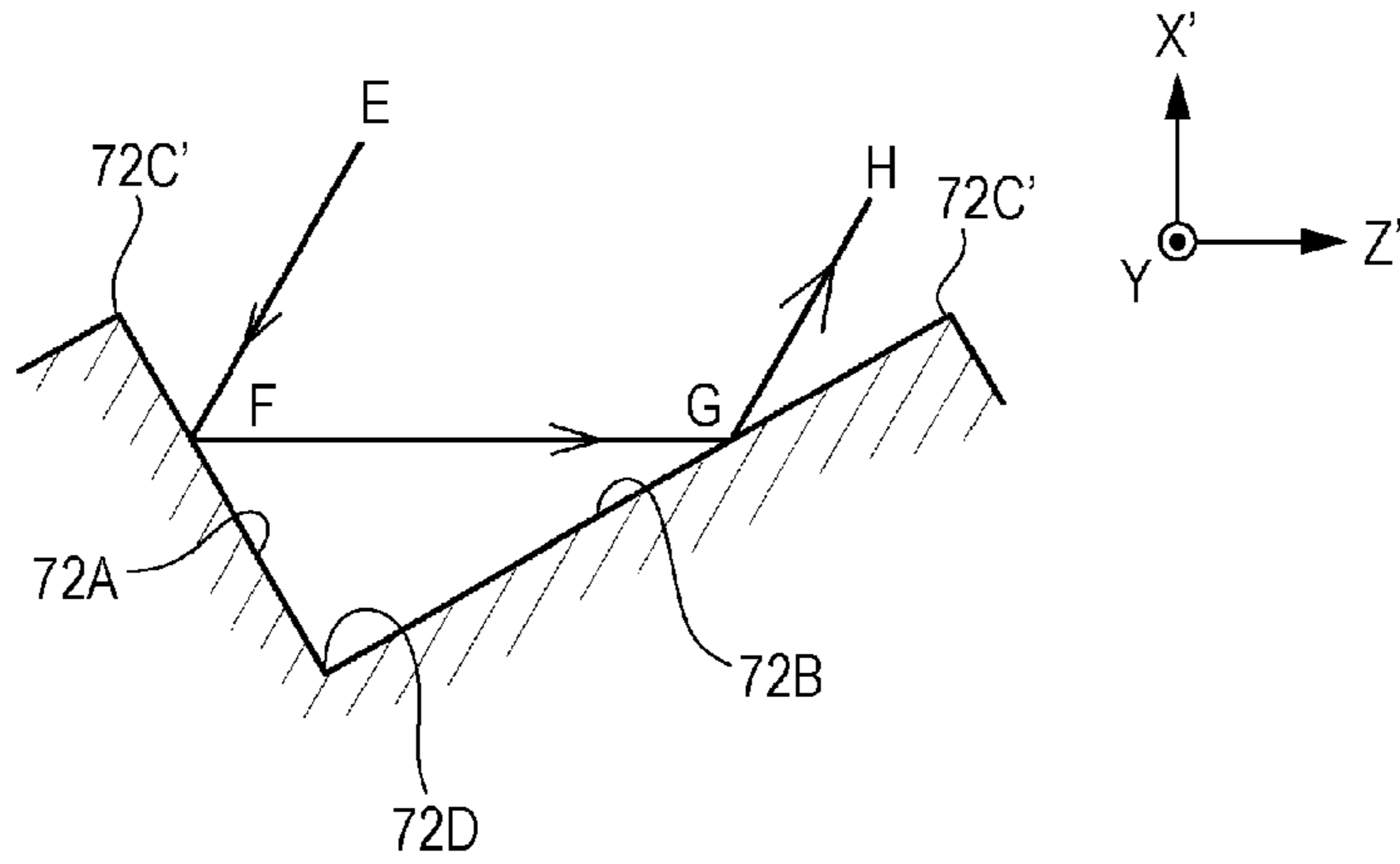
FIG. 4A [SECOND A IMAGINARY PLANE]
