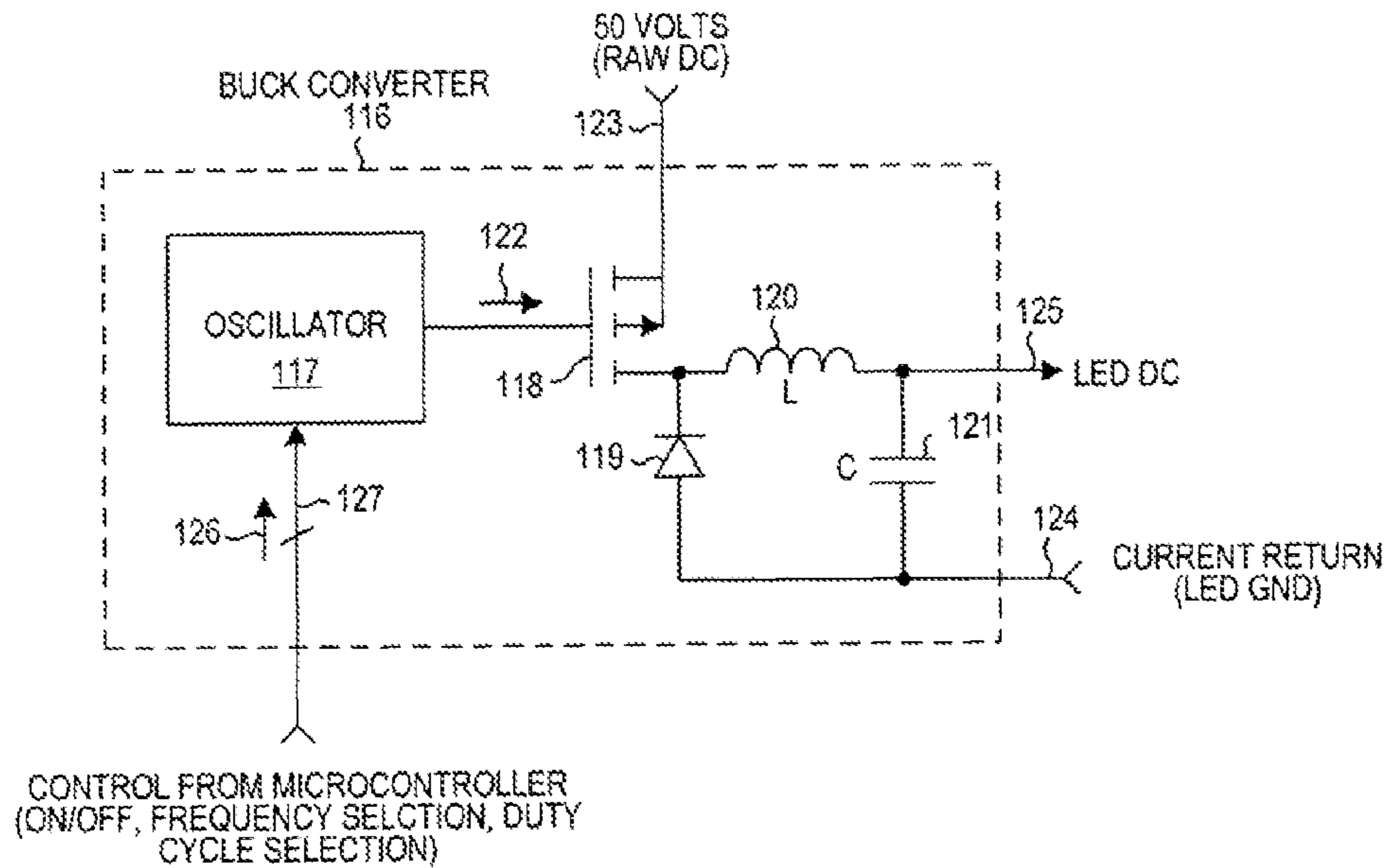
BUCK CONVERTER
