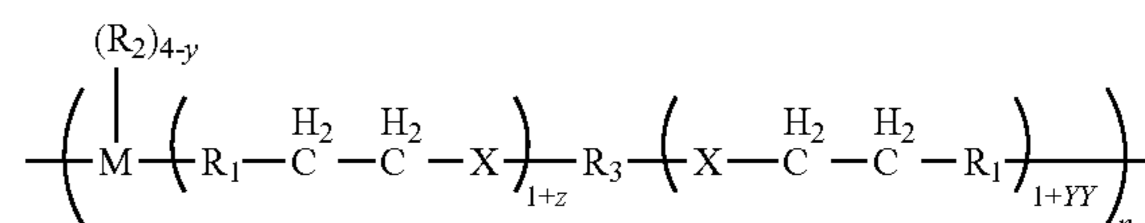
Structure (I)
