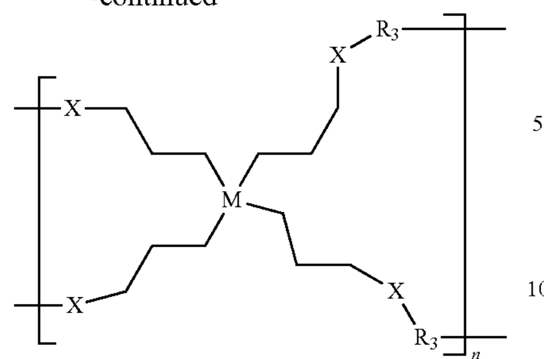
Structure (XXVI)
