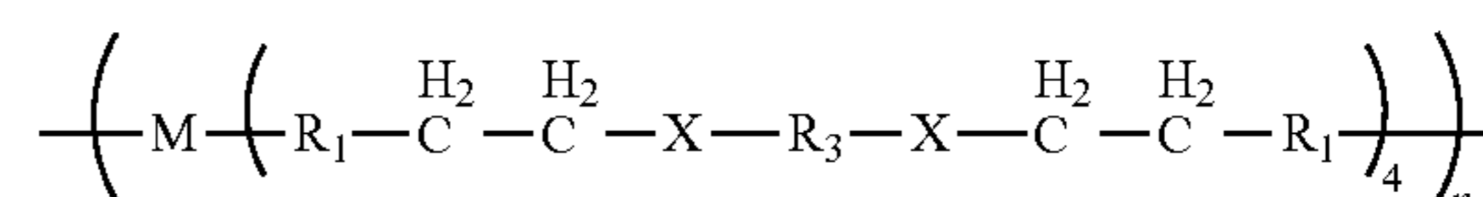
Structure (IIa)
