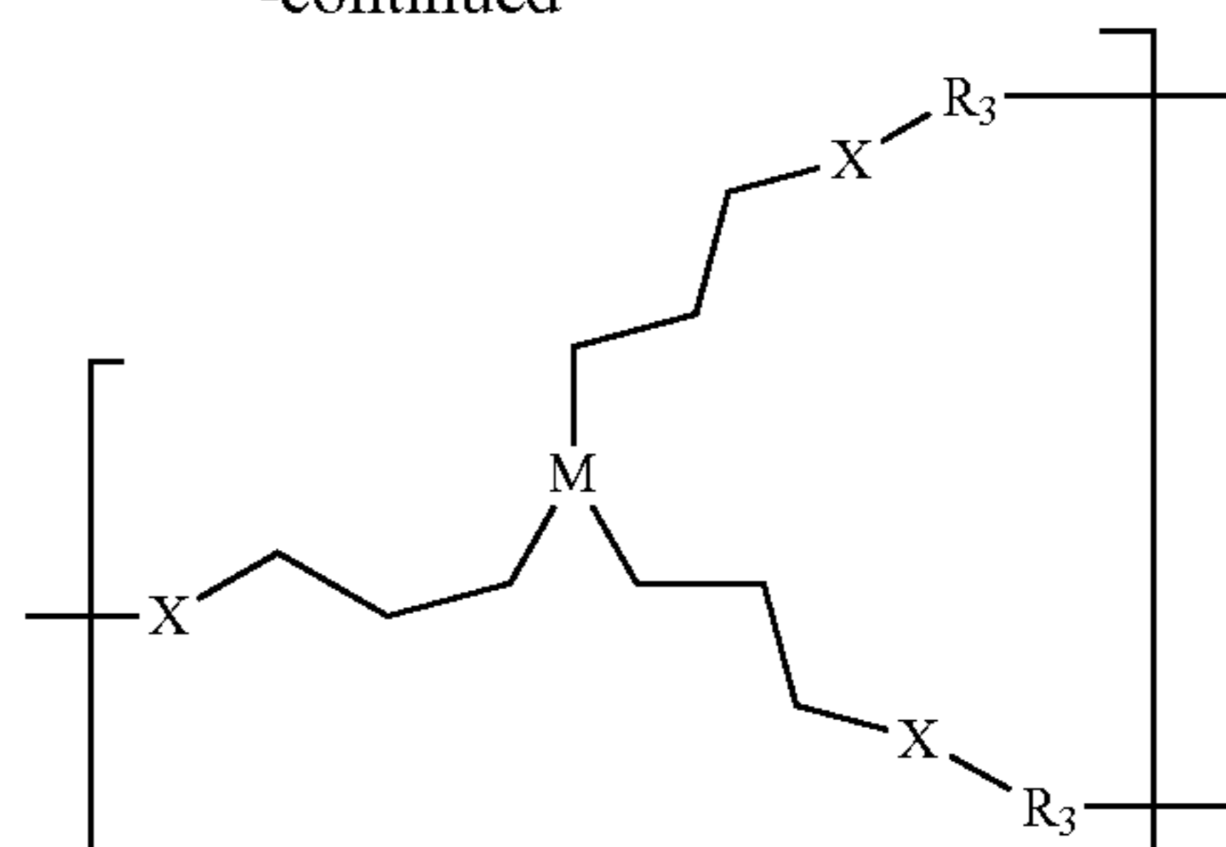
Structure (XXVIII)
