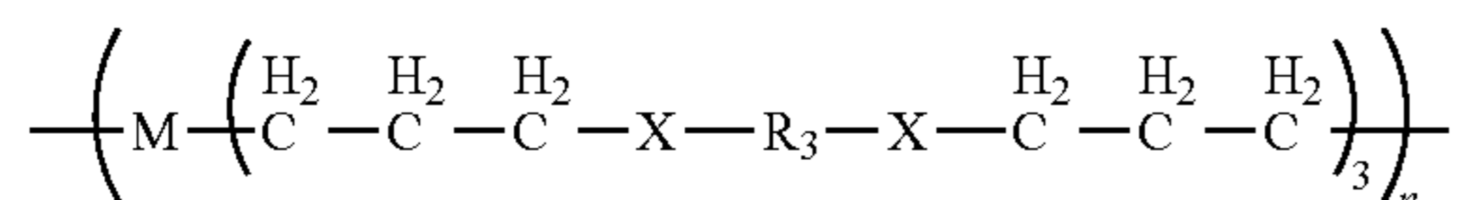
Structure (IIIc)
