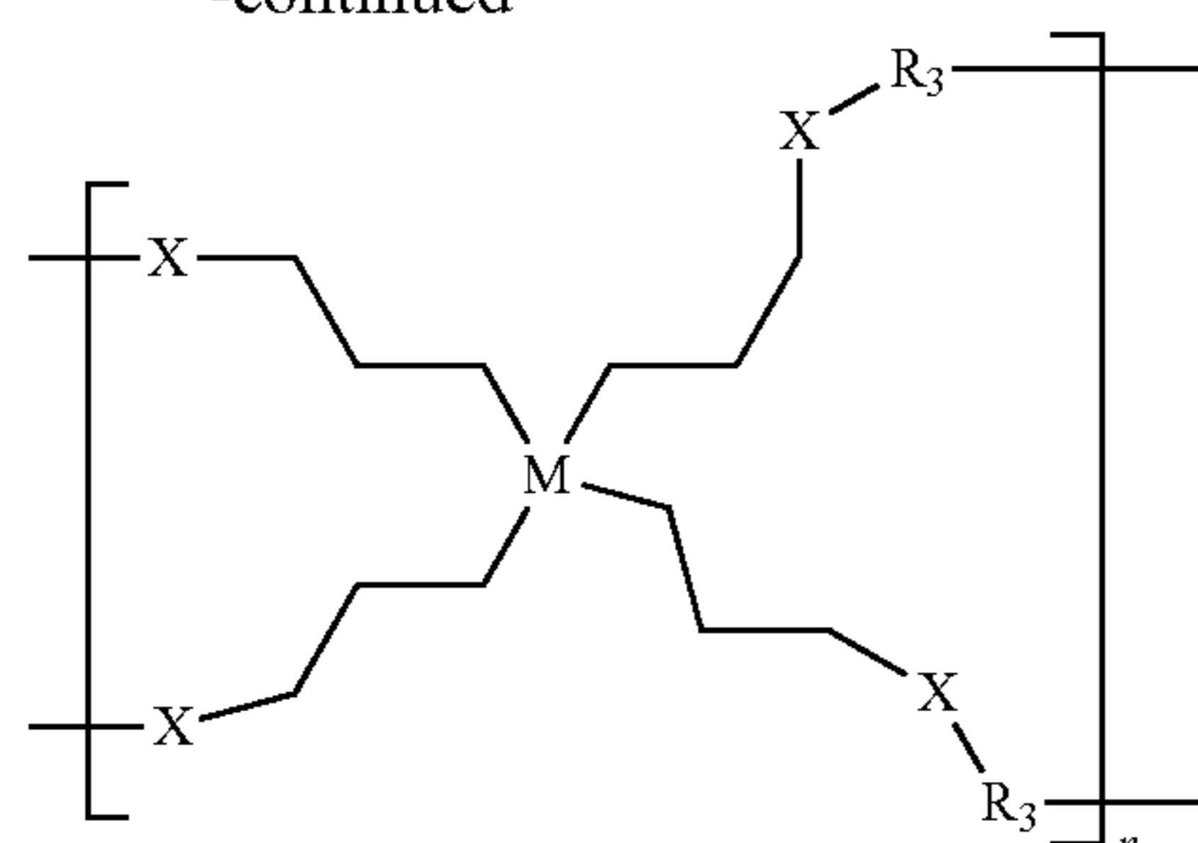
Structure (XXVI)
