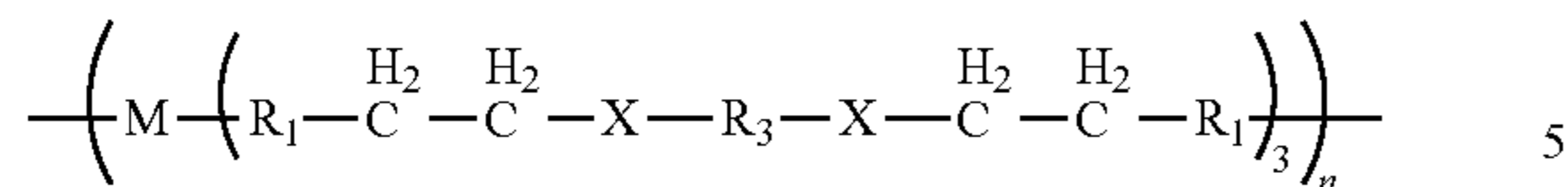
Structure (IIIa)
