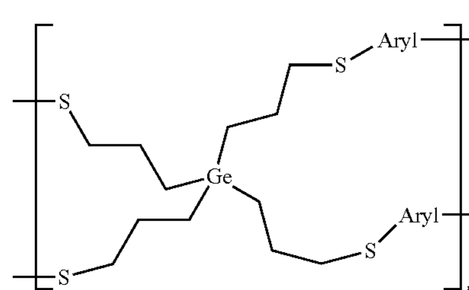
Structure (IVh)
