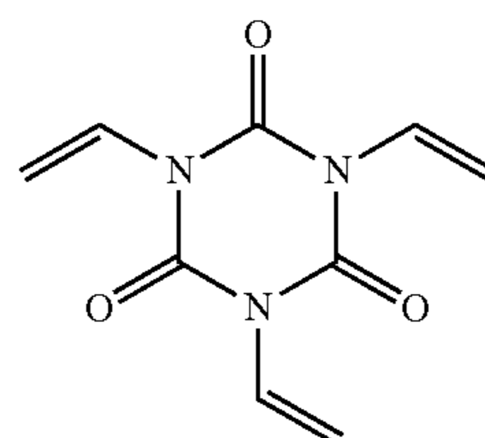
Structure (IX) 20
