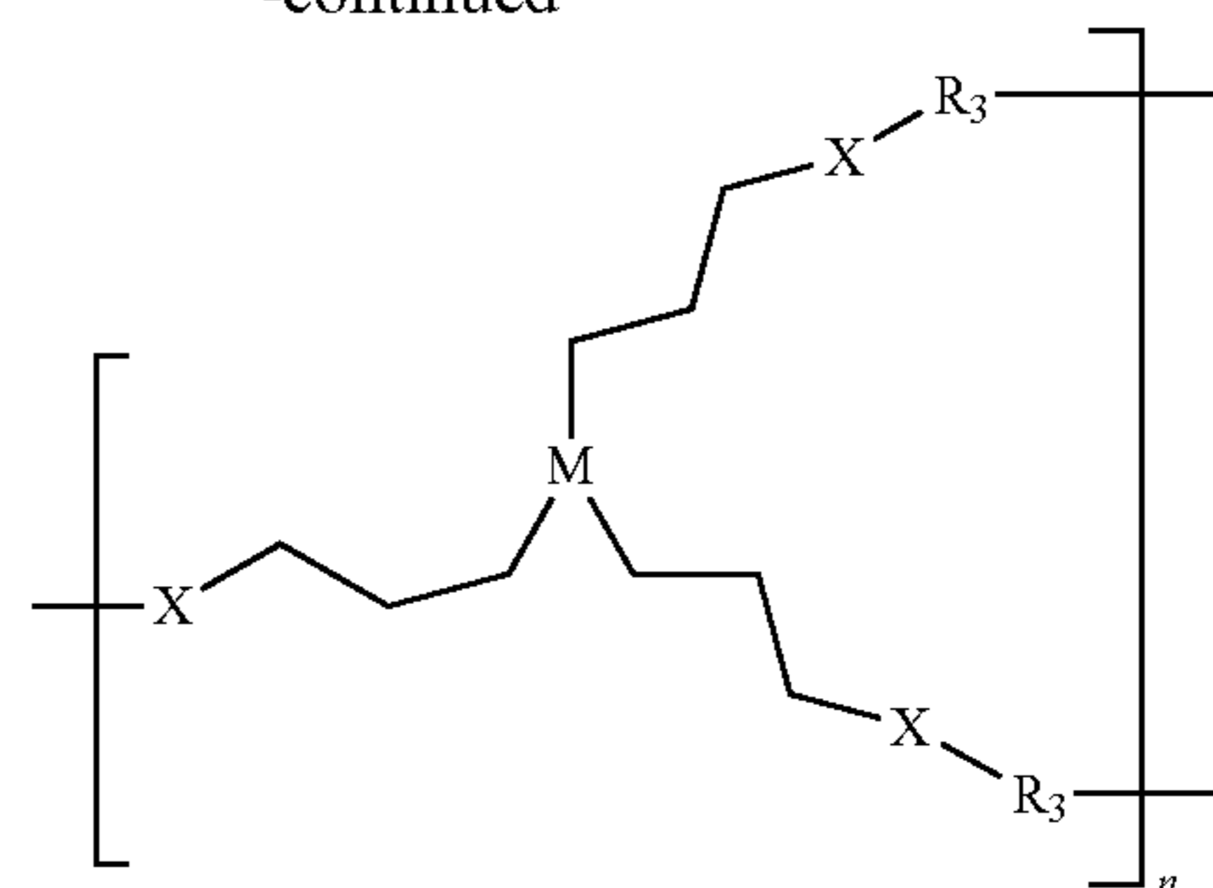
Structure (XXVIII)
