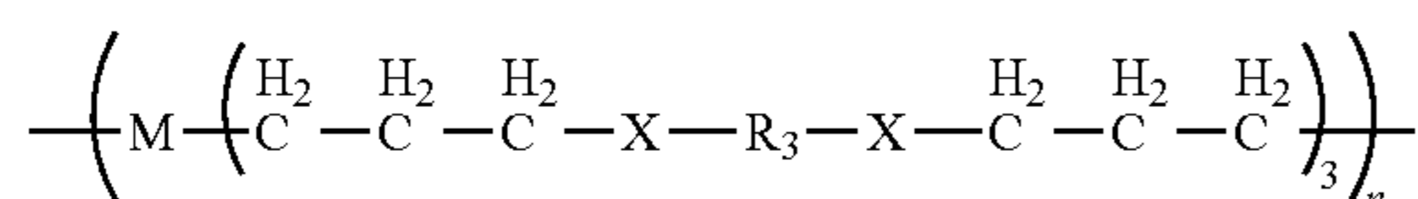
Structure (IIIc)
