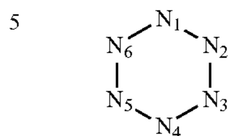
Structure (V)
