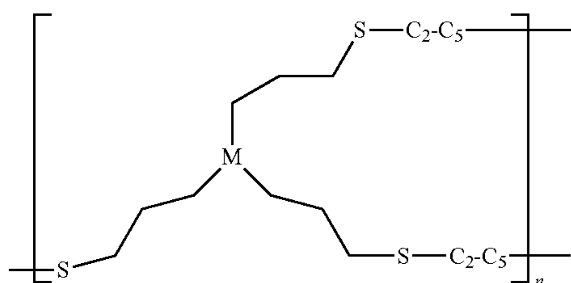
Structure (IVk)
