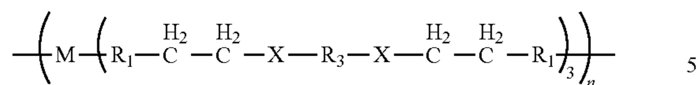
Structure (IIIa)
