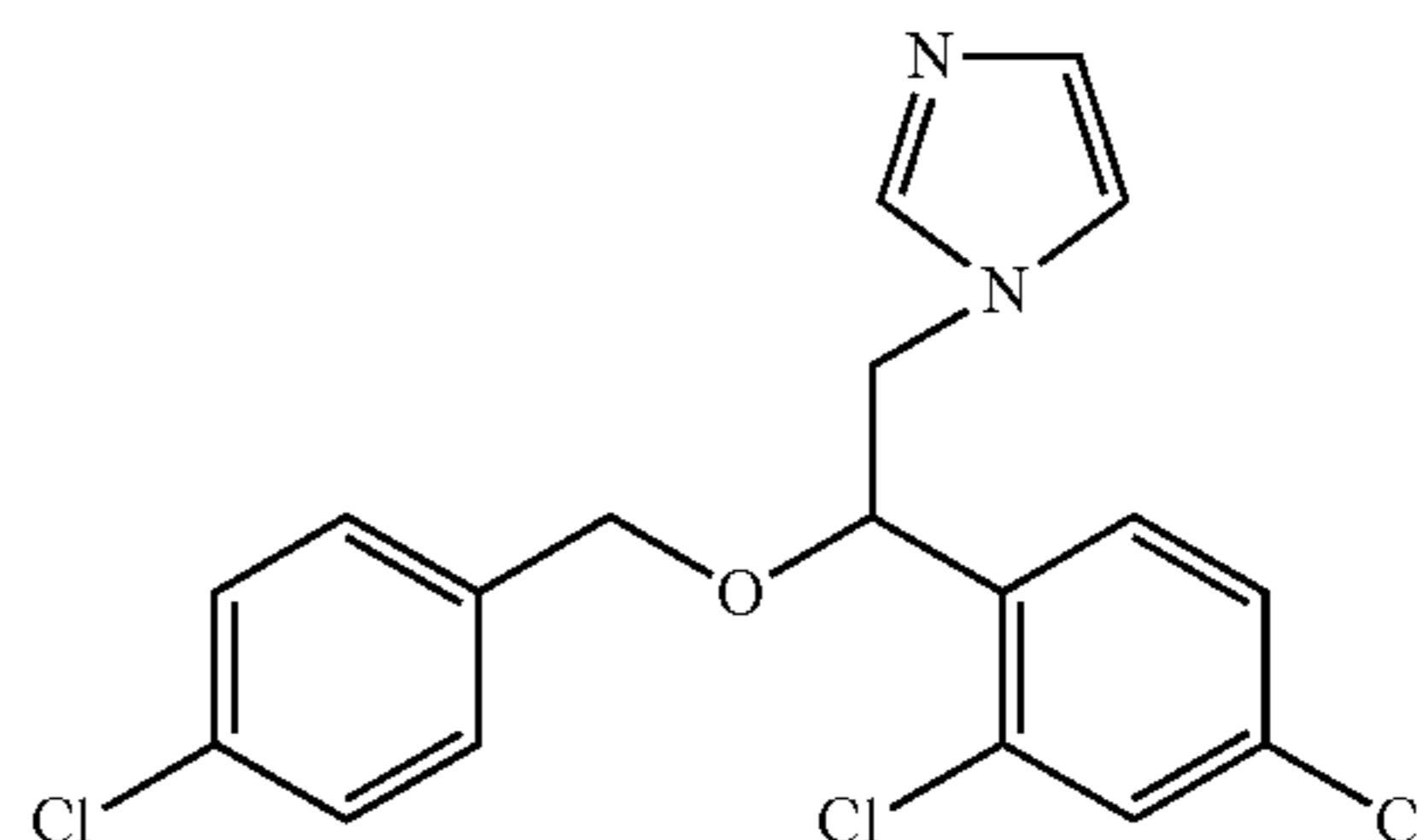
Econazole
