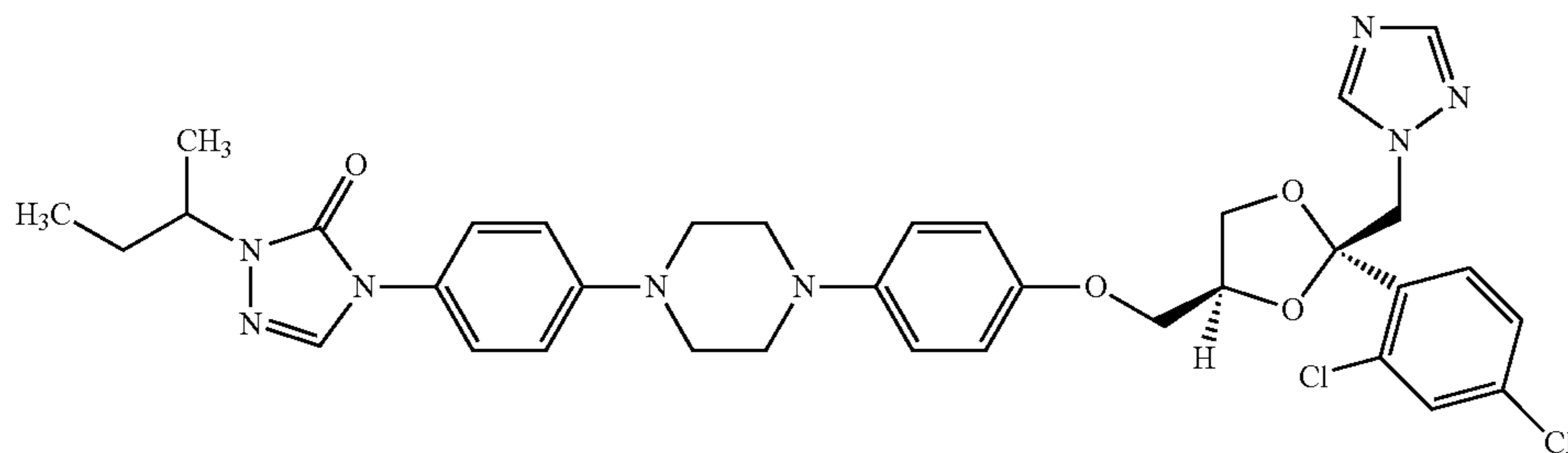
Itraconazole
