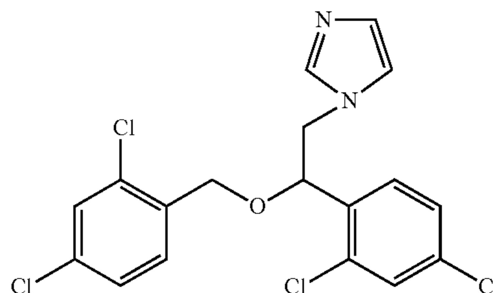
Miconazole
