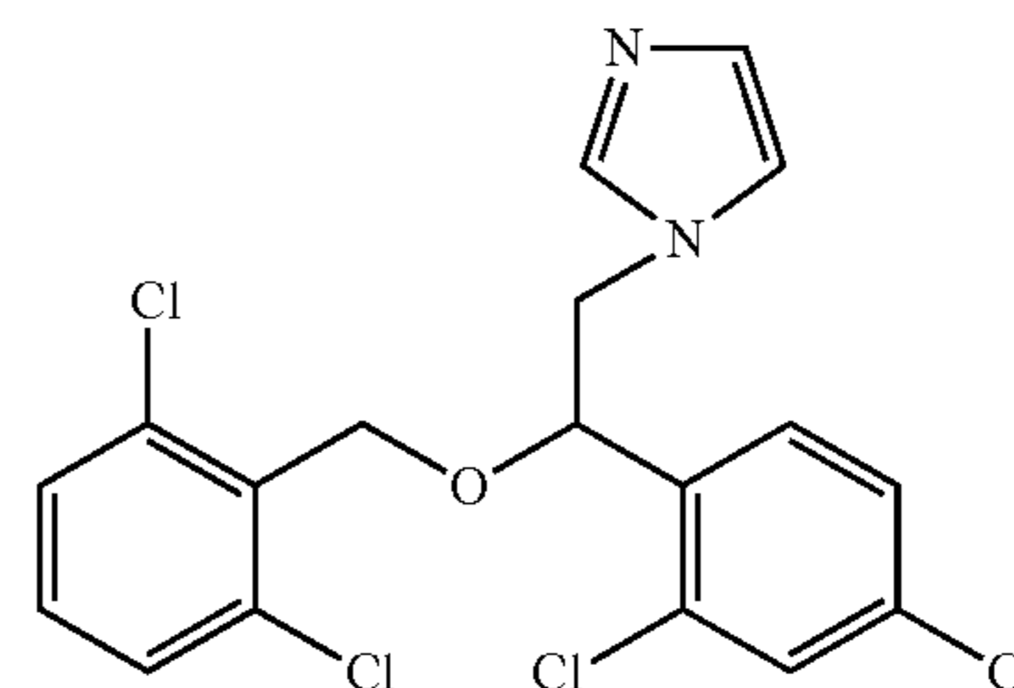
Isoconazole
