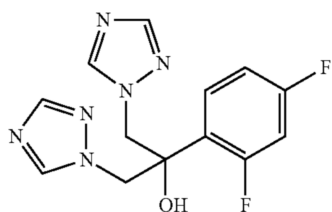
Fluconazole
