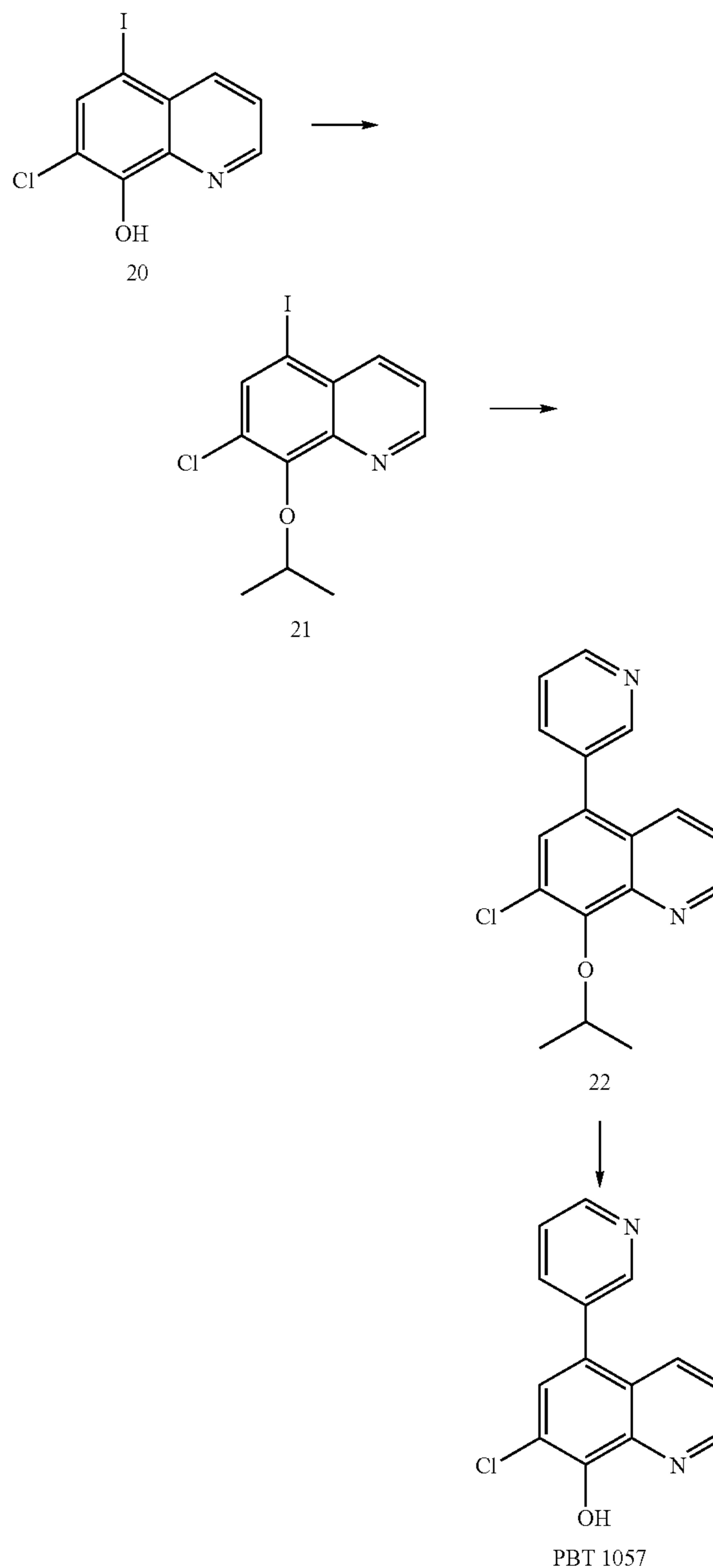
Scheme 17
