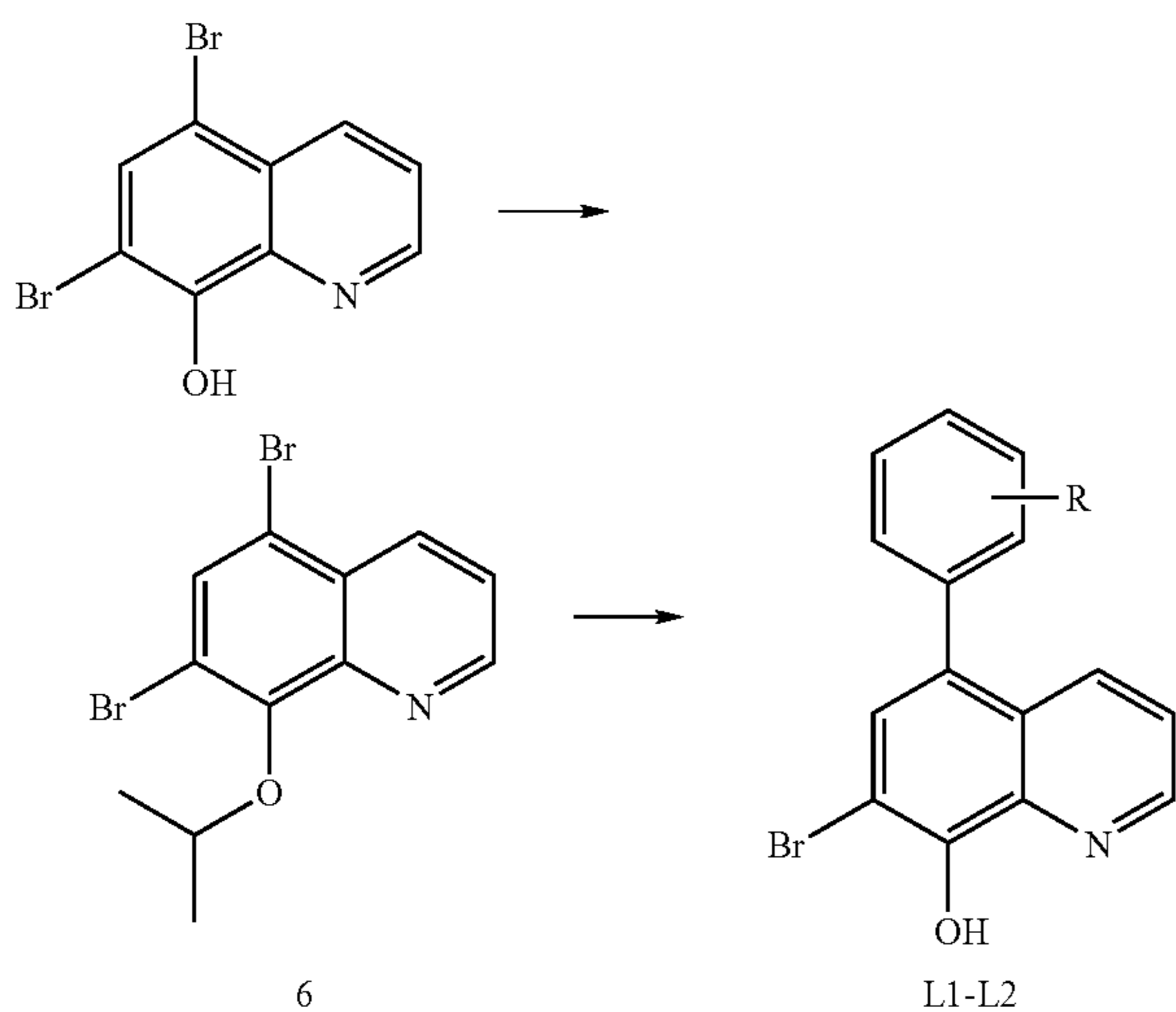
Scheme 9
