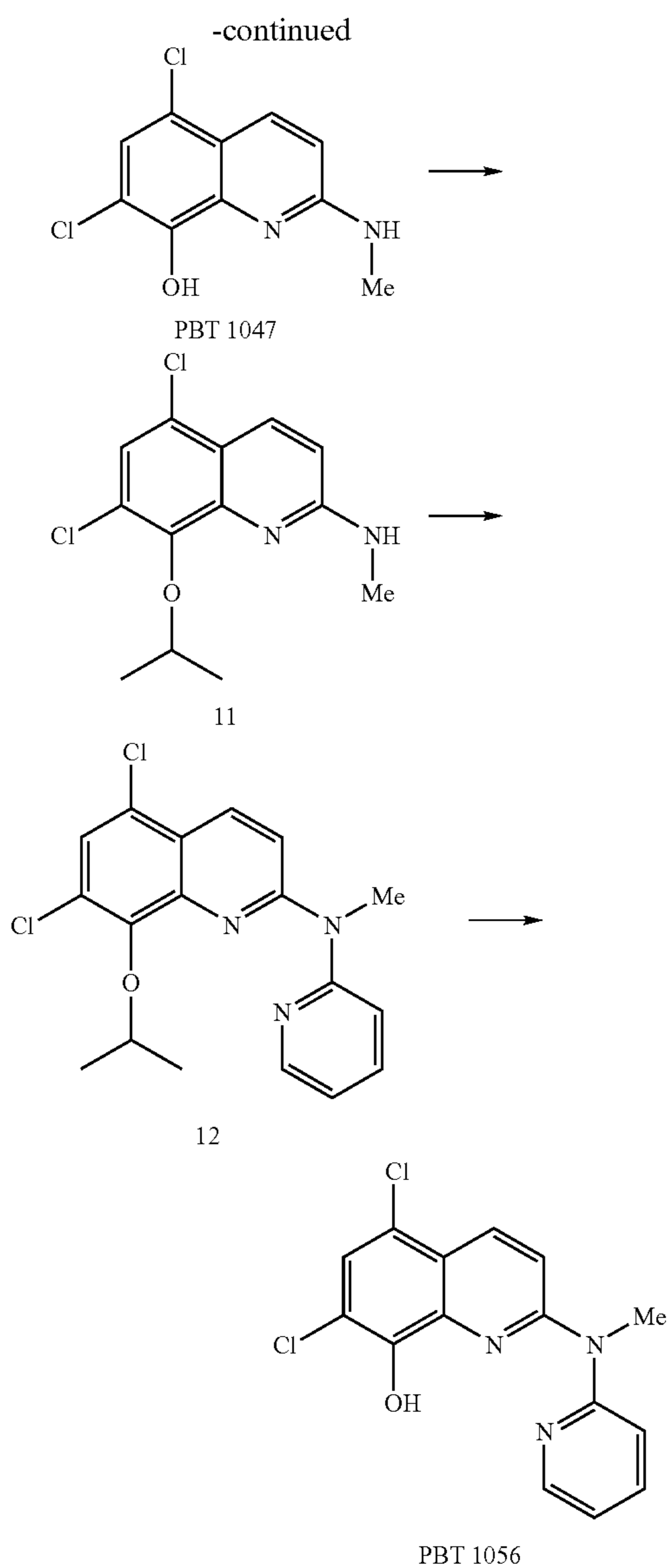
5,7-Dichloro-2-methylamino-8-hydroxyquinoline (PBT 1047)
