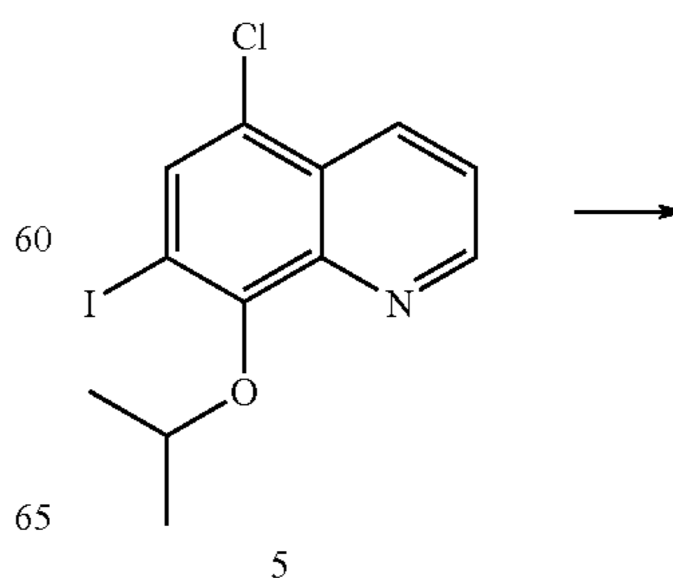
Scheme 11
