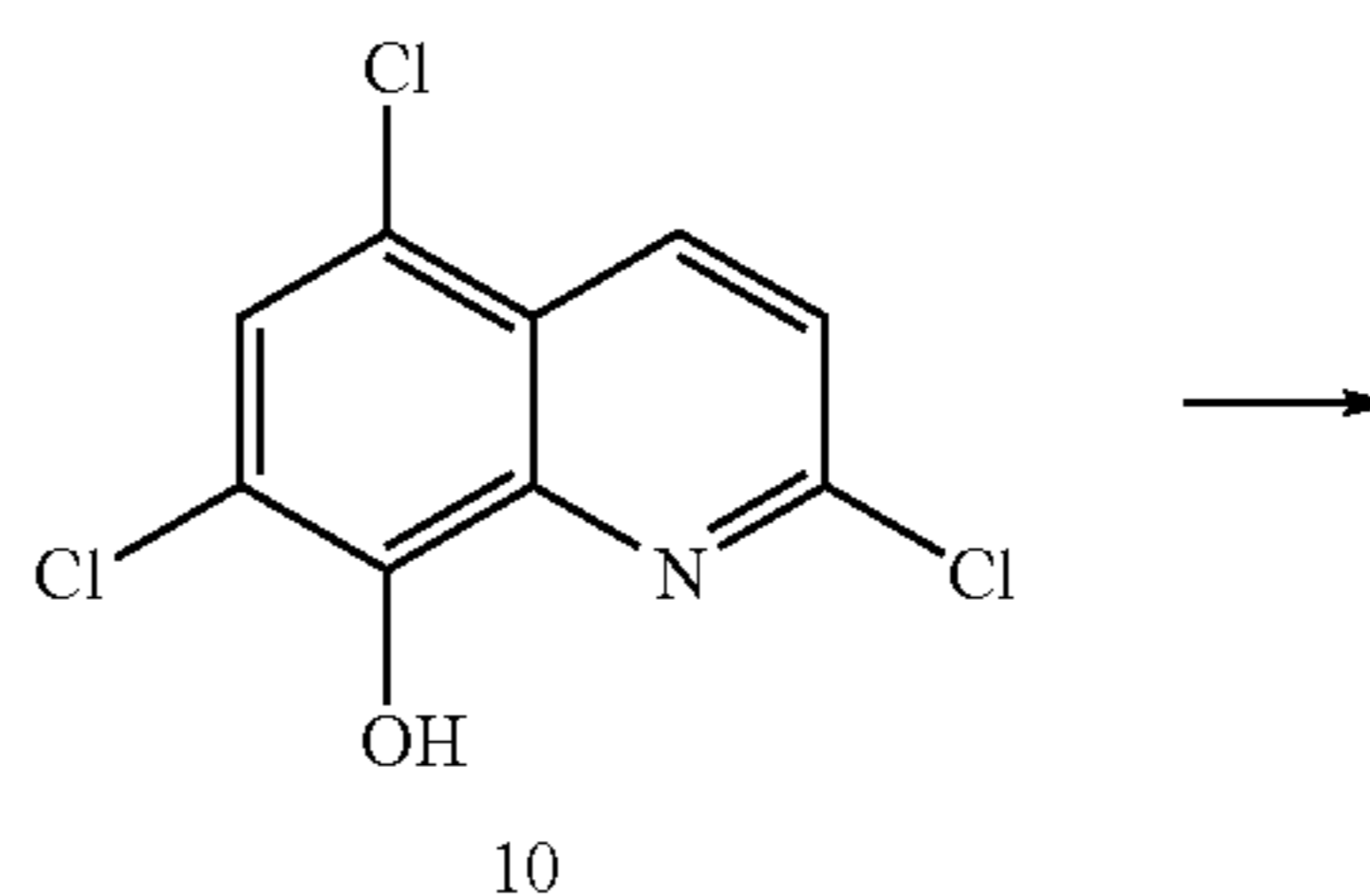
Scheme 14
