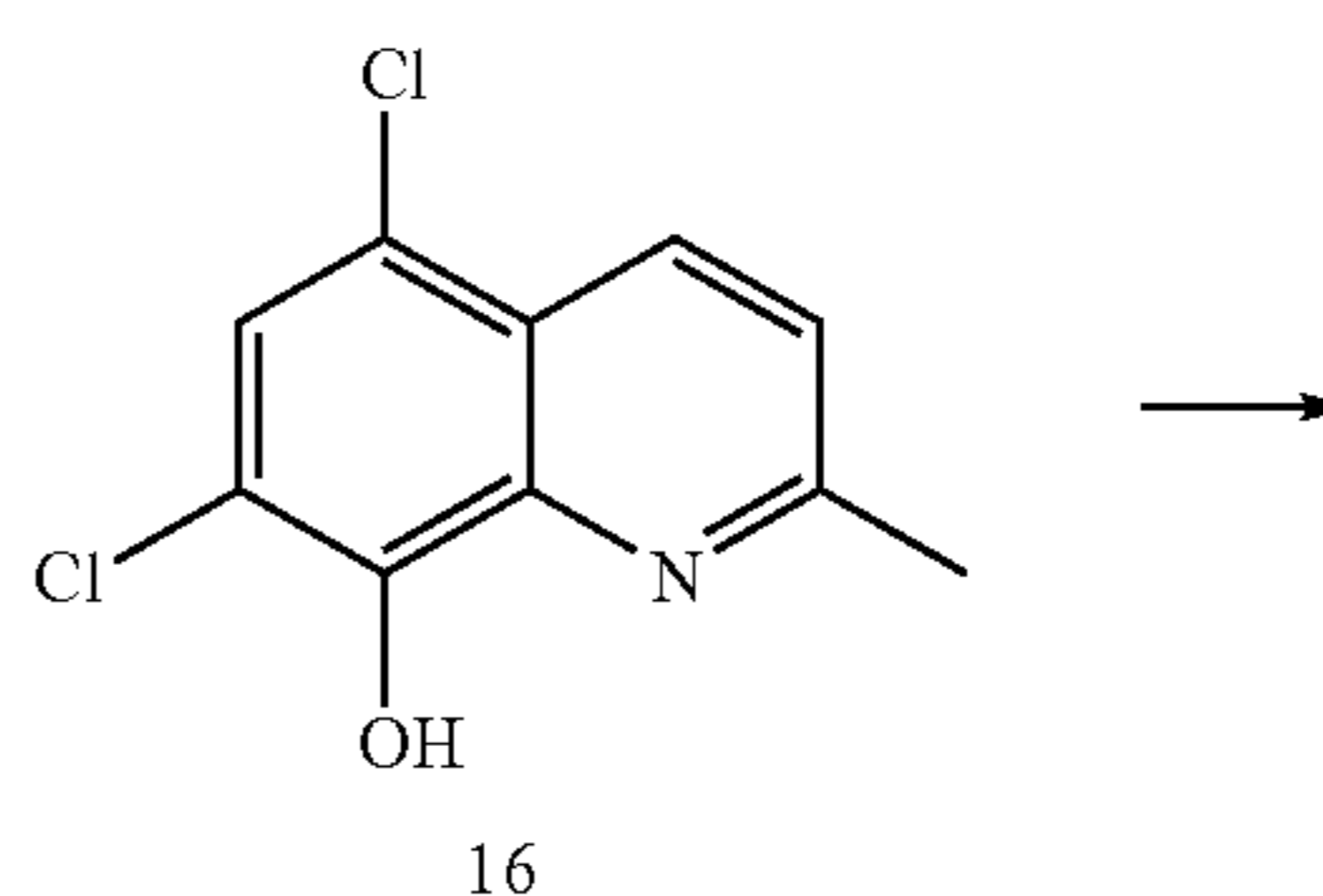
Scheme 15
