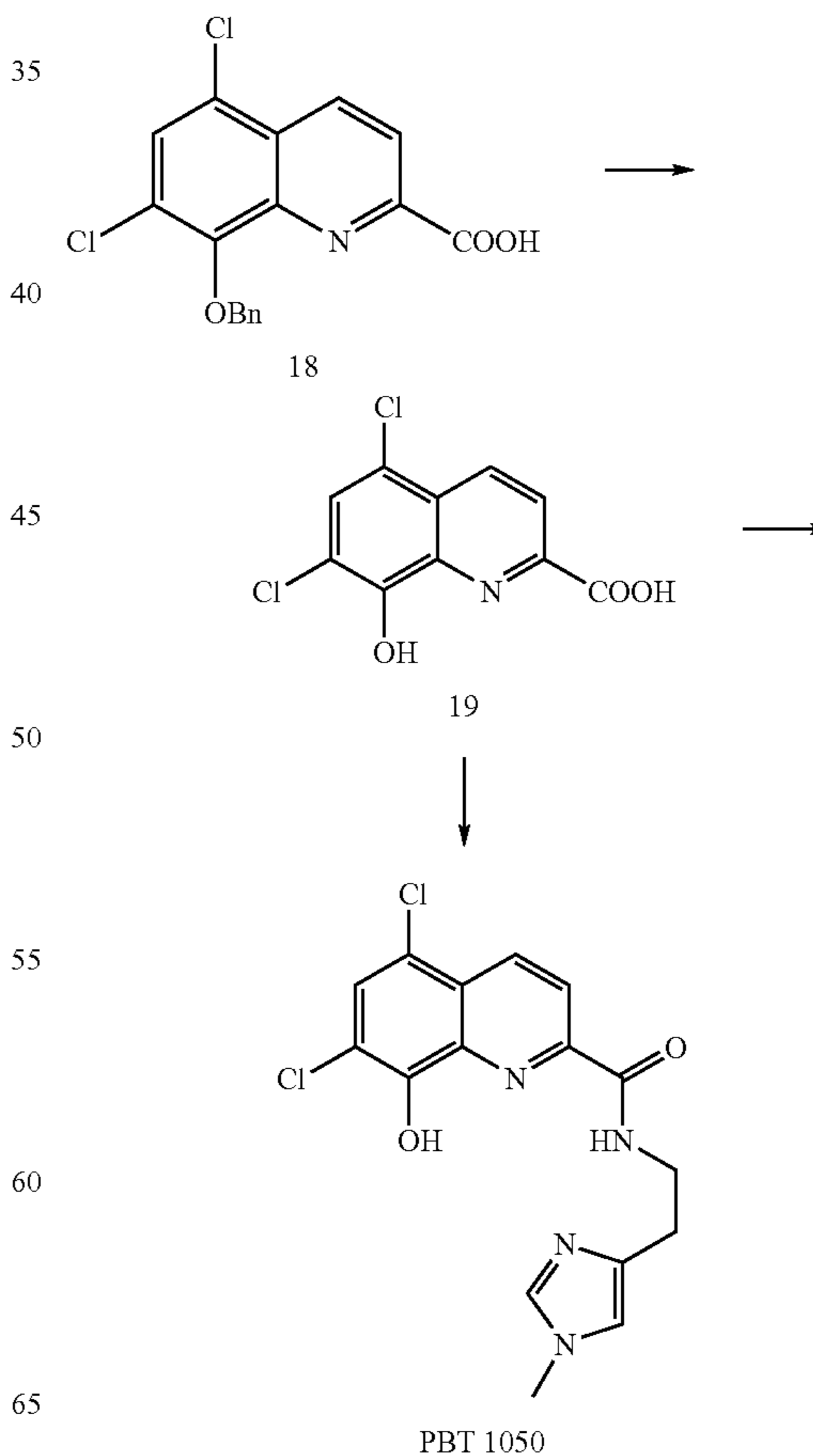
Scheme 16
