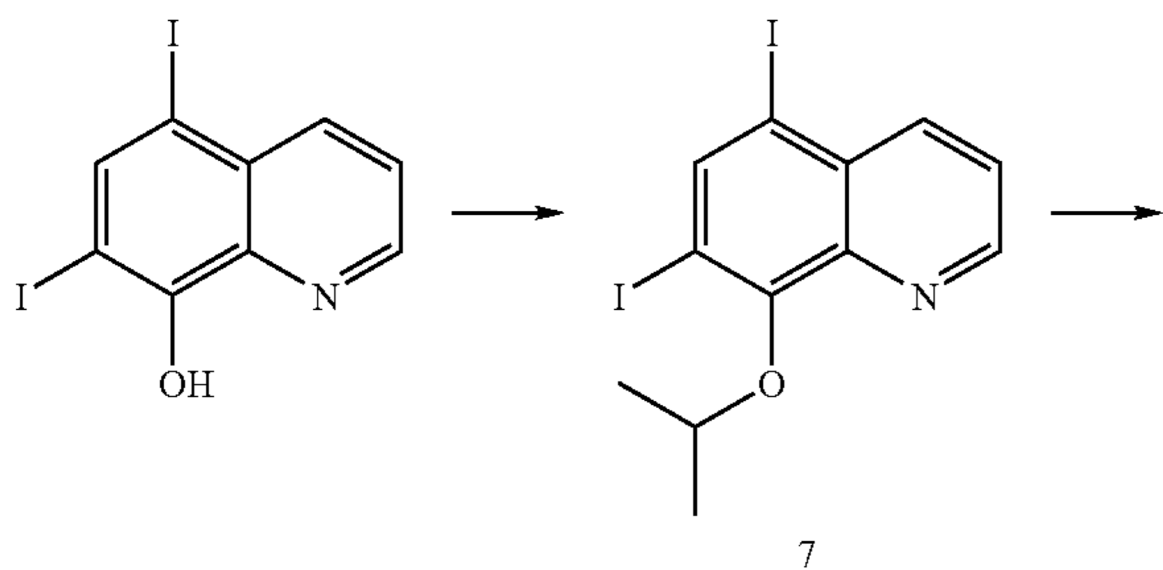
Scheme 10
