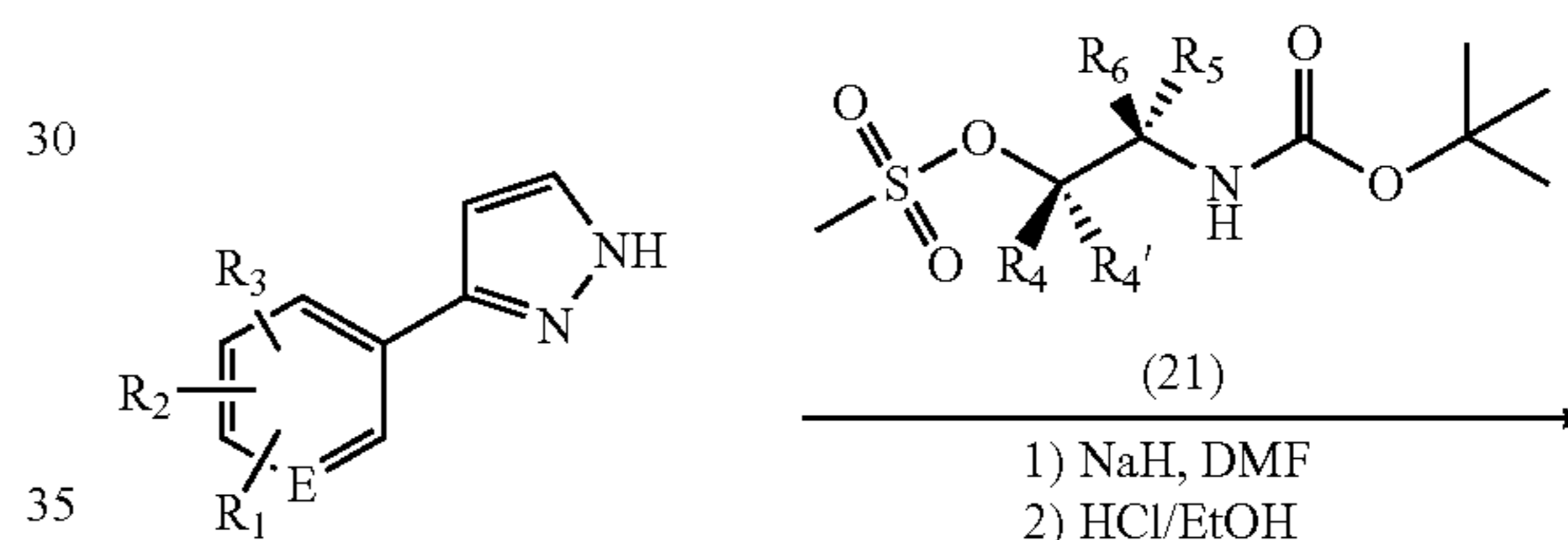
Scheme 5
