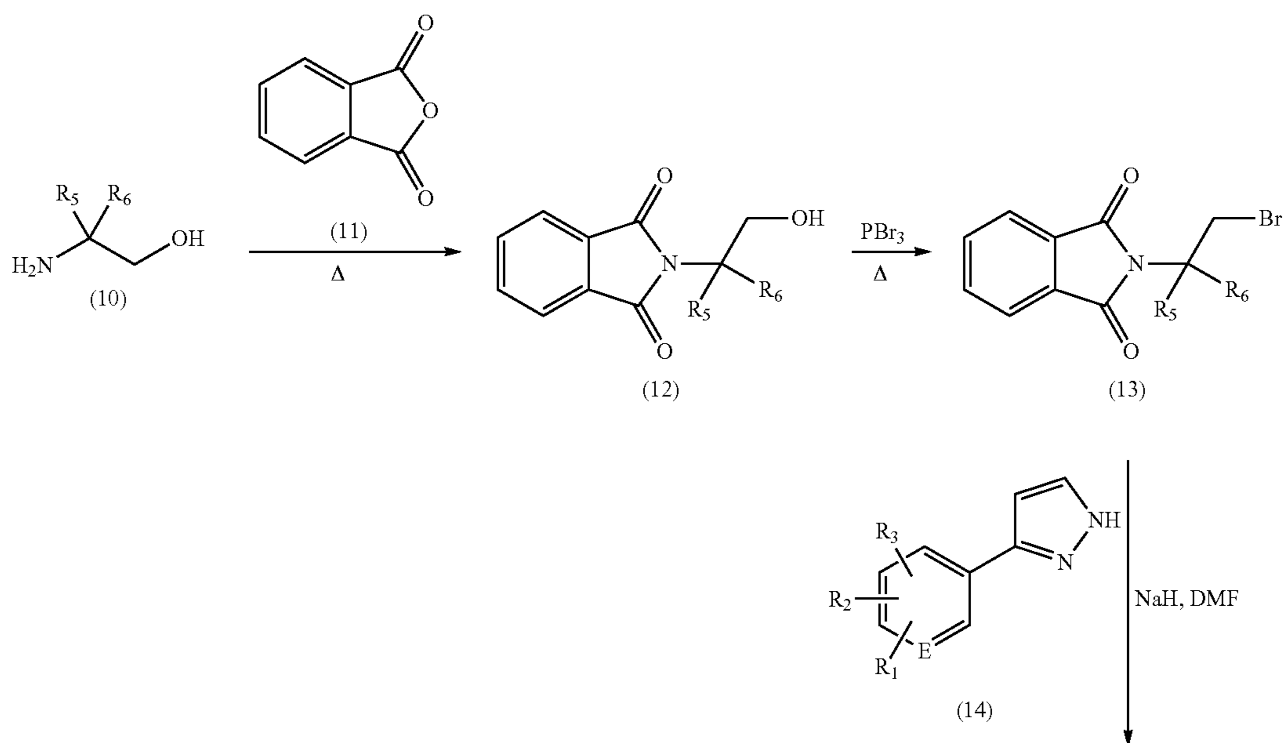
Scheme 3
