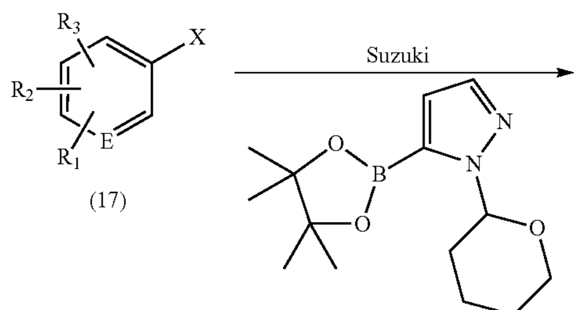
Scheme 4
