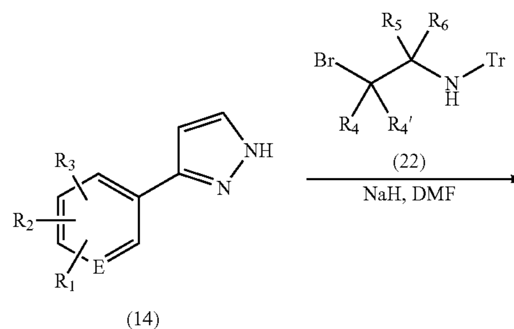
Scheme 6
