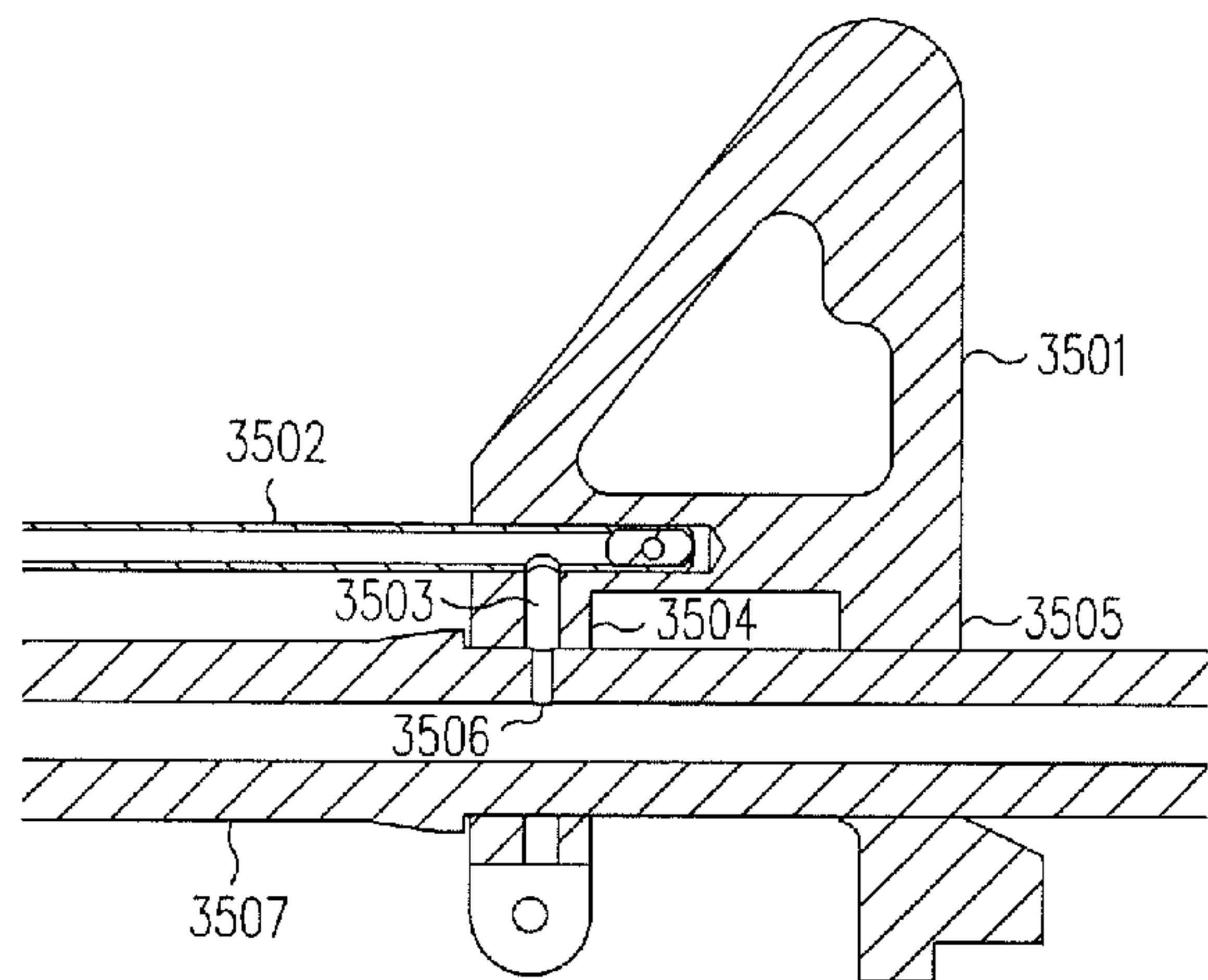
FIG. 35 (PRIOR ART)
