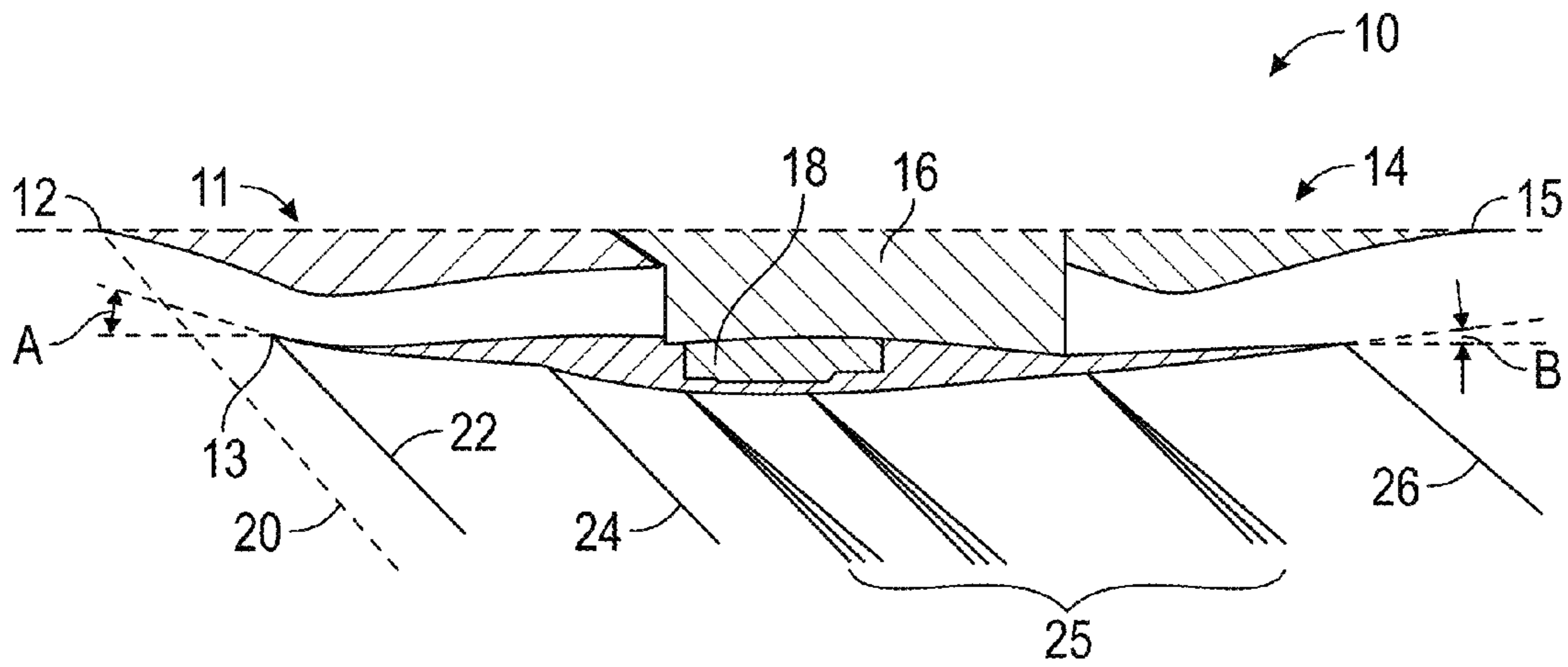
FIG. 2 (Prior Art)
