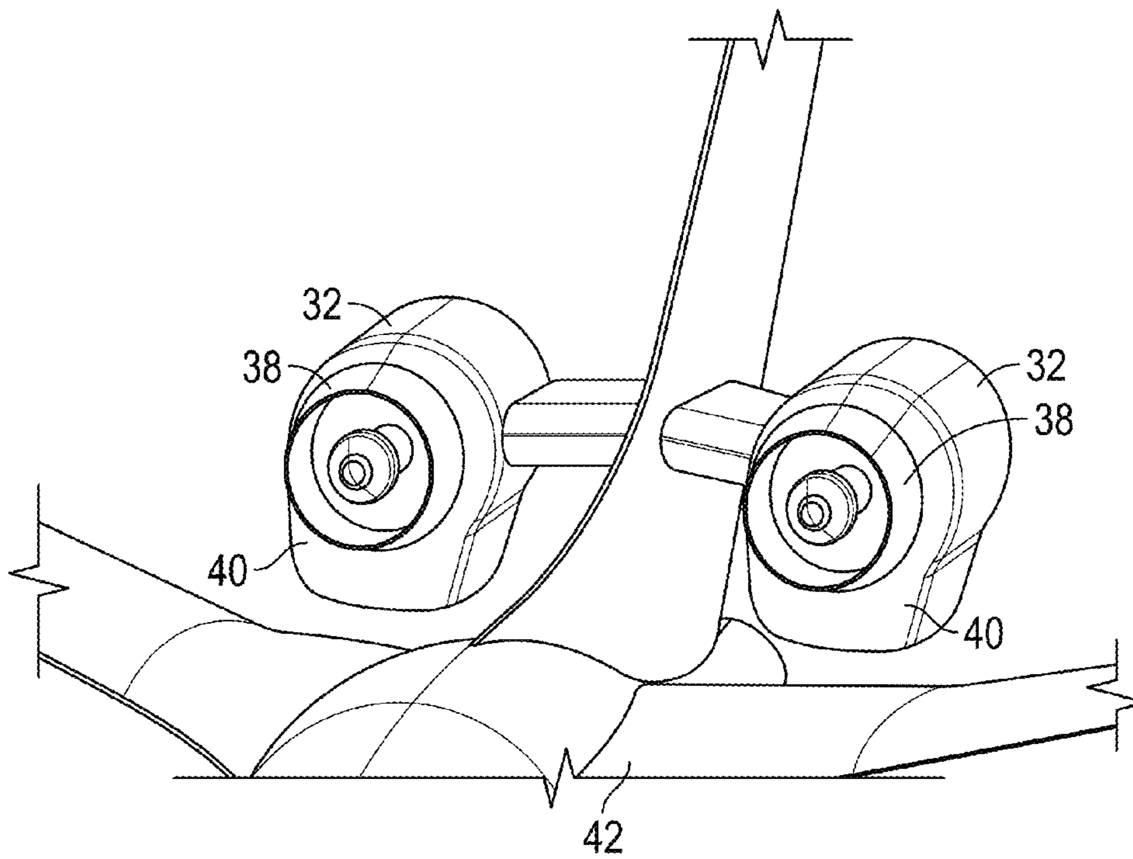
FIG. 4 (Prior Art)
