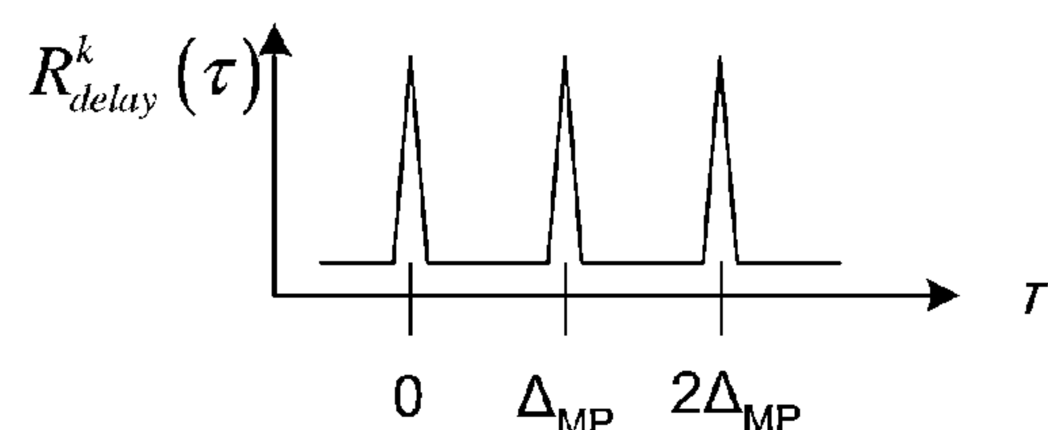
Delay-based autocorrelation of (three-path) multipath signal y(t)
