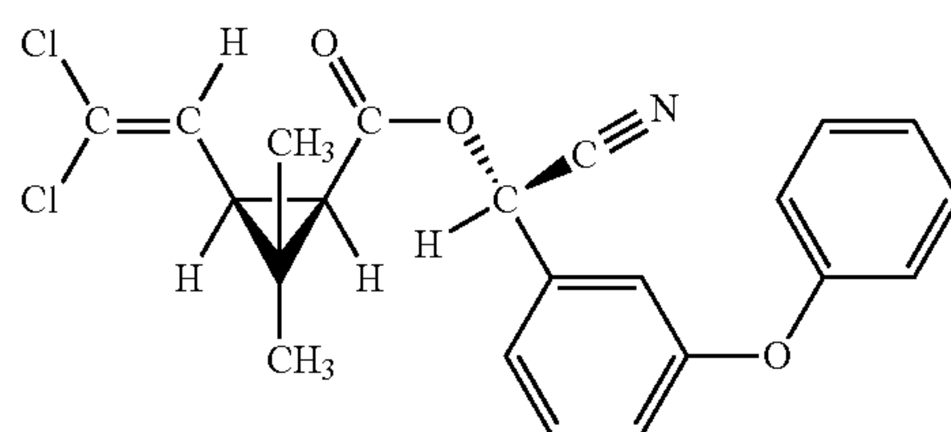
(S)-alcohol (1R)-cis-acid
