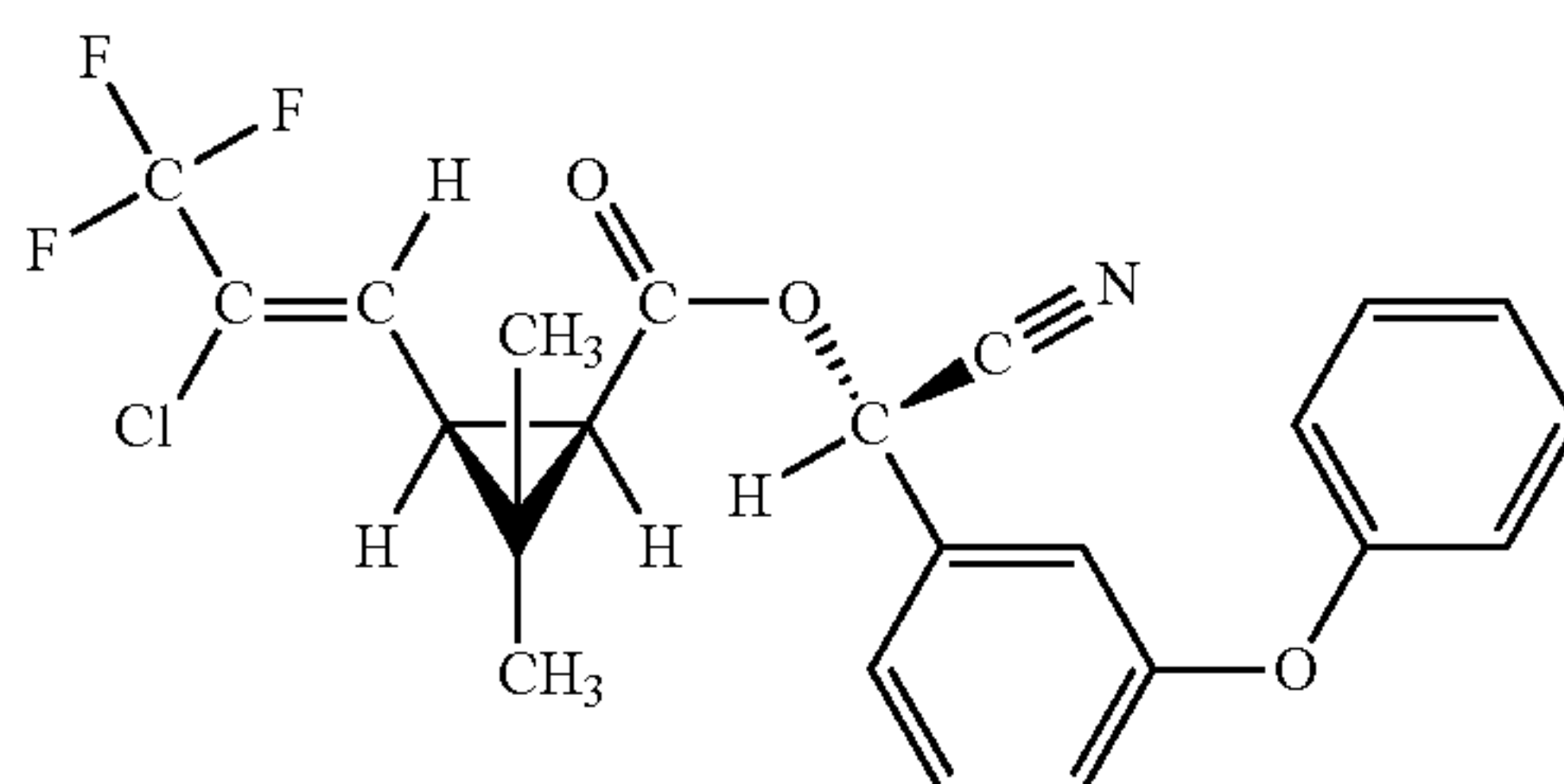
(S)-alcohol (Z)-(1R)-cis-acid
