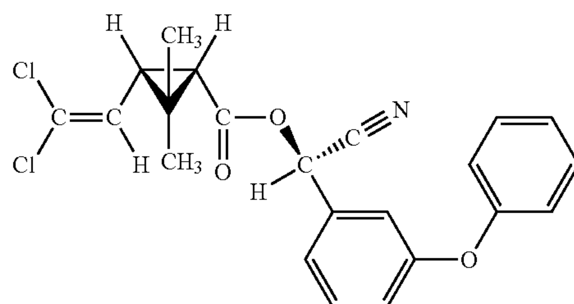
(R)-alcohol (1s)-cis-acid
