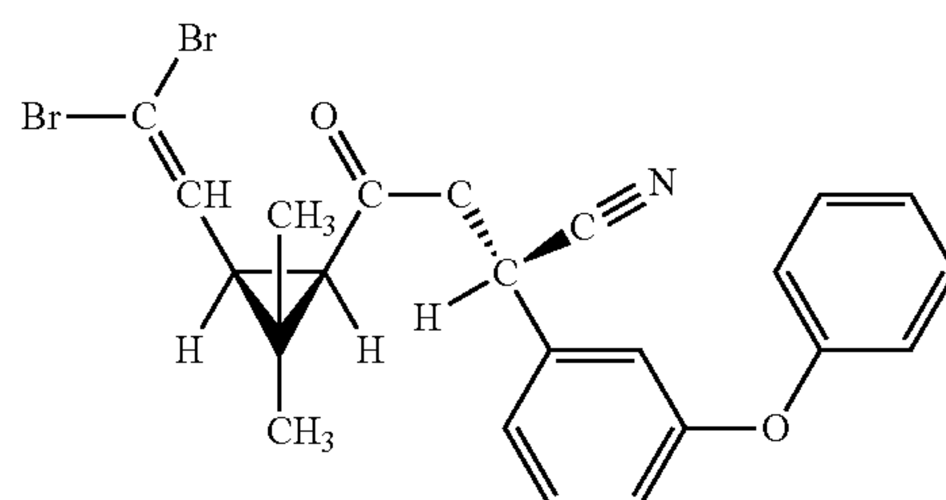
(S)-alcohol (1R)-cis-acid
