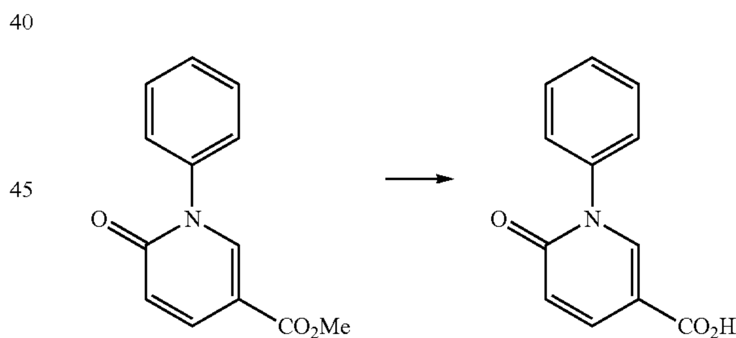
6-Oxo-1-phenyl-1,6-dihydropyridine-3-carboxylic acid
