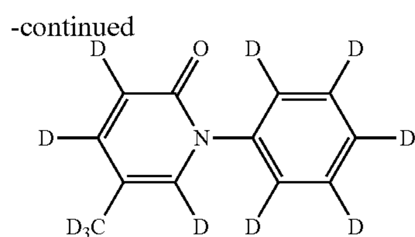
d 11 -5-Methyl-1-phenyl-1H-pyridin-2-one
