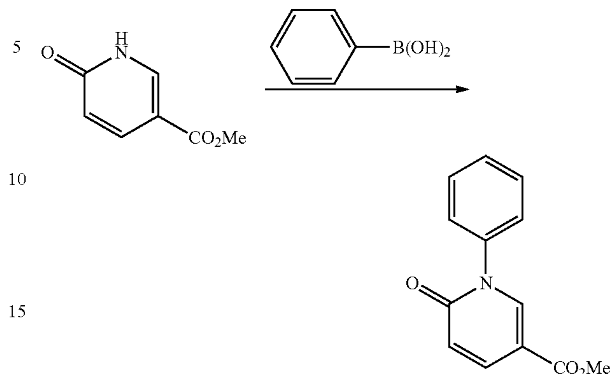
Methyl-6-oxo-1-phenyl-1,6-dihydropyridine-3-carboxylate
