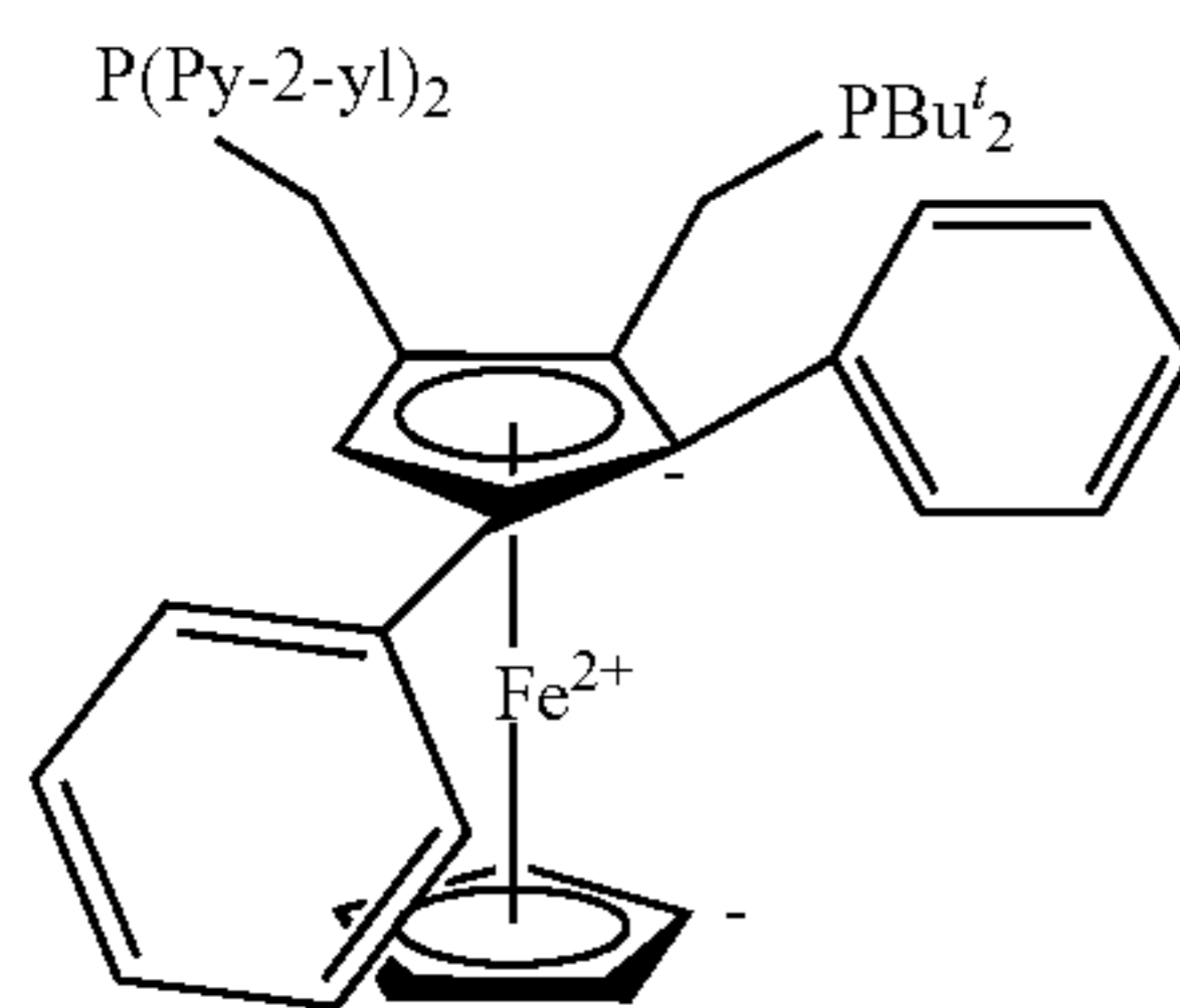
1-(di-t-butylphosphinomethyl)-2-(di-pyridin-2-ylphosphinomethyl)-4,5-diphenyl ferrocene;
