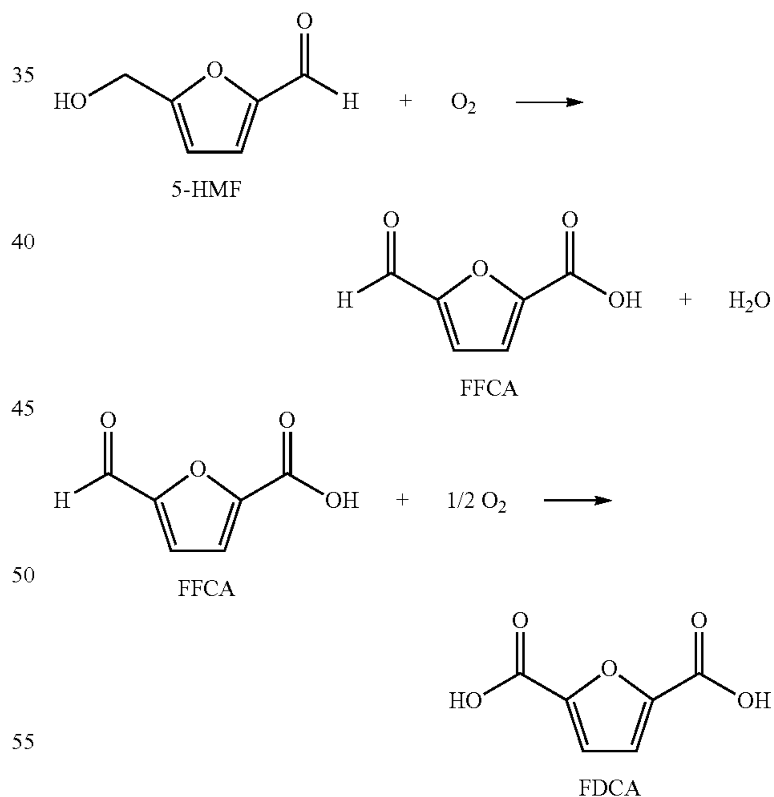
5-methylfurfural
