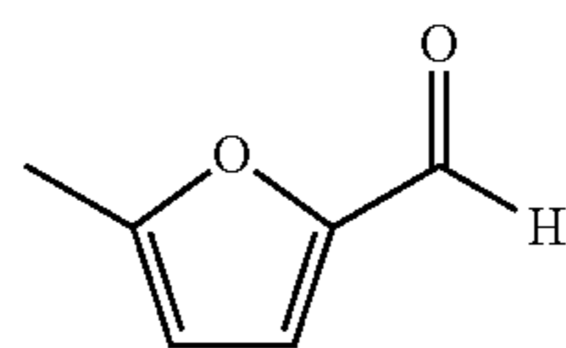
5-methylfurfural
