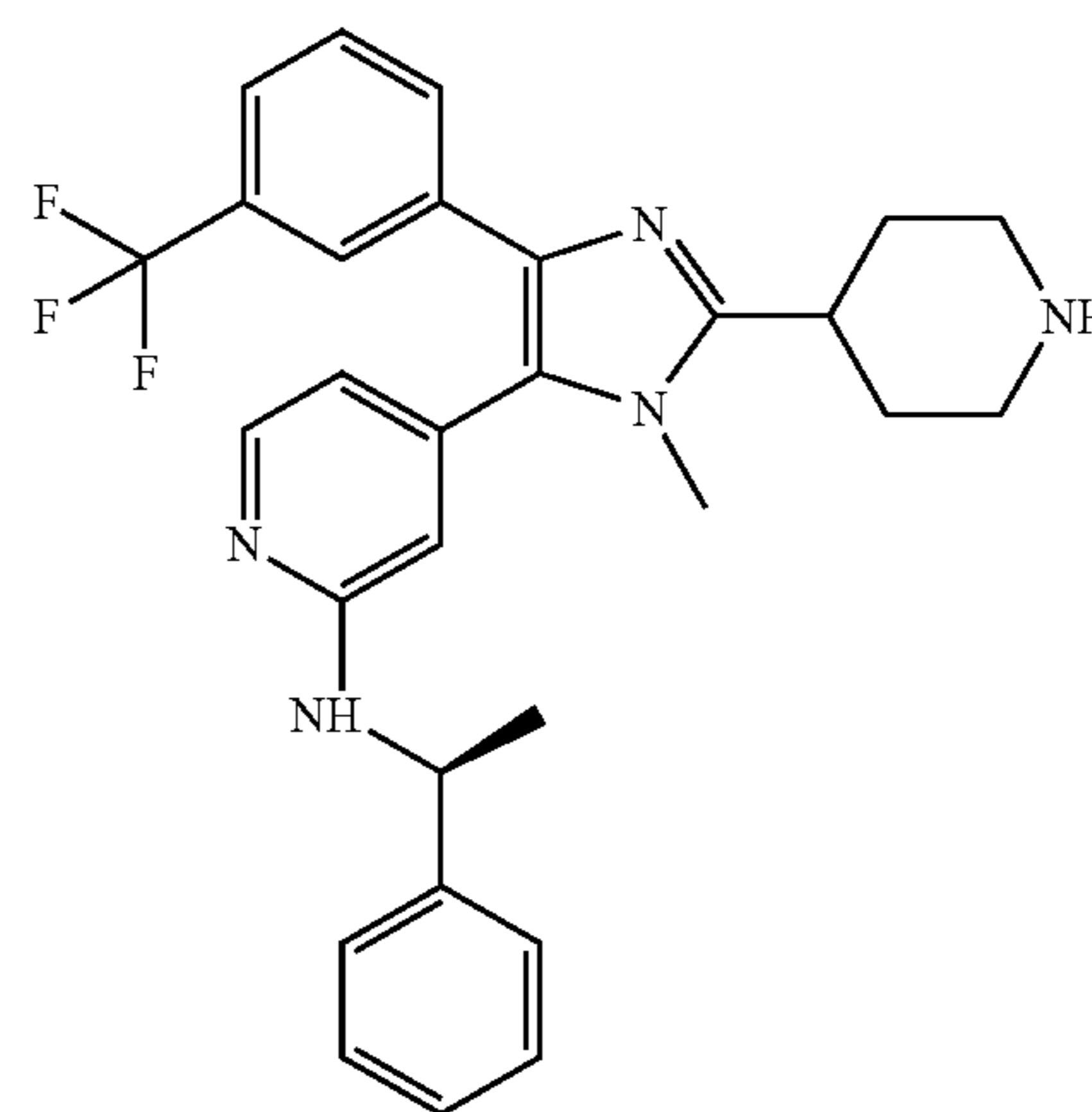
2 X = N; SB 203580 3 X = CH; L-167307
