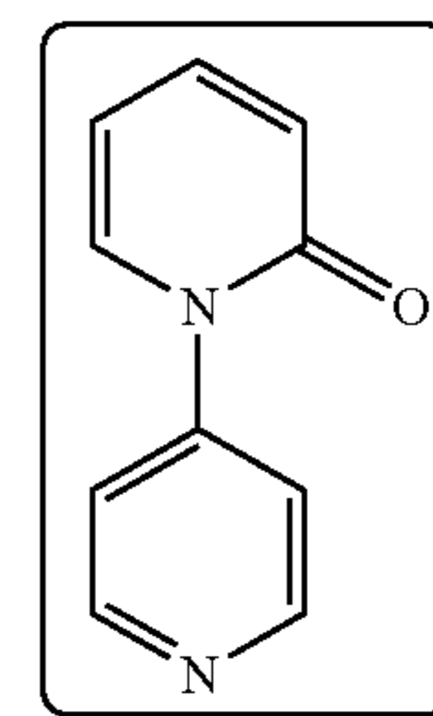
Ullmann Condensation
