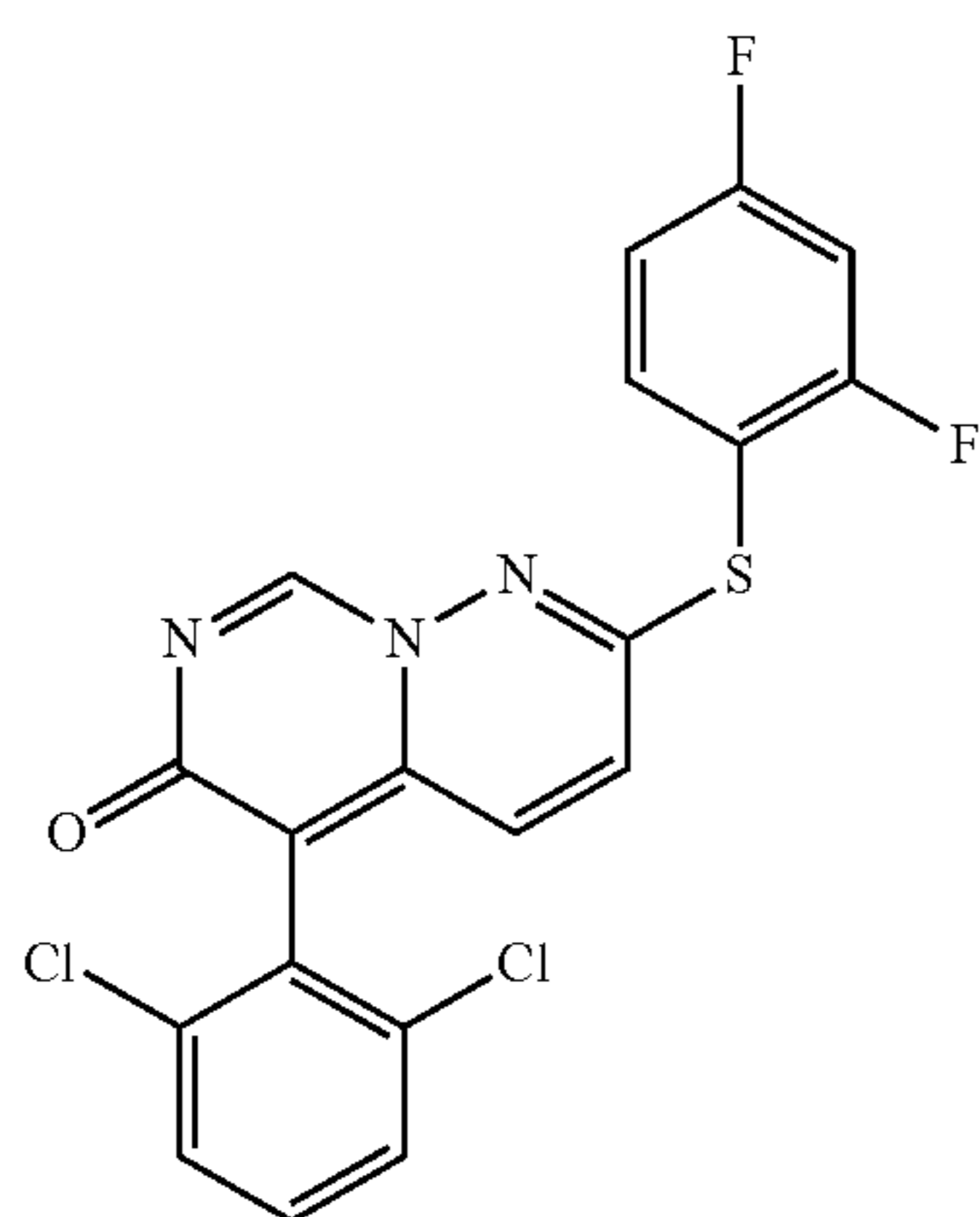
VX-745
