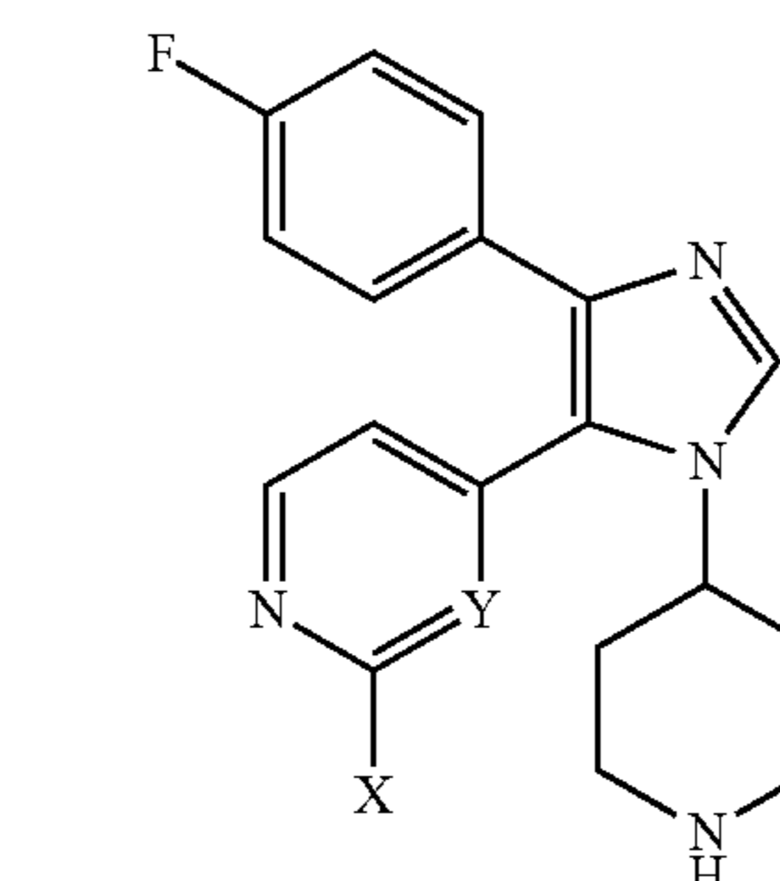
6 X = H, Y = CH; HEP 689 (SB 235699) 7 X = HN 2 , Y = N; SB 220025
