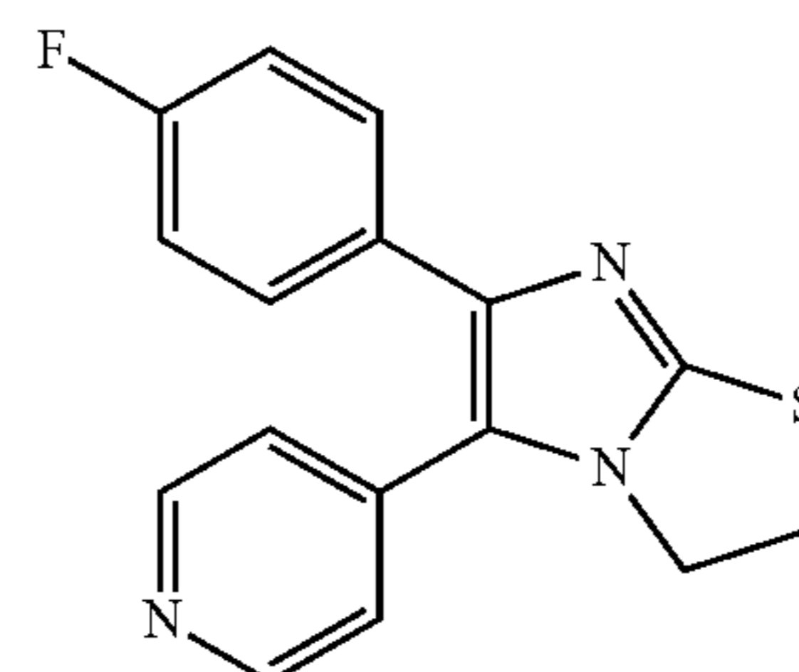
SKF 86002
