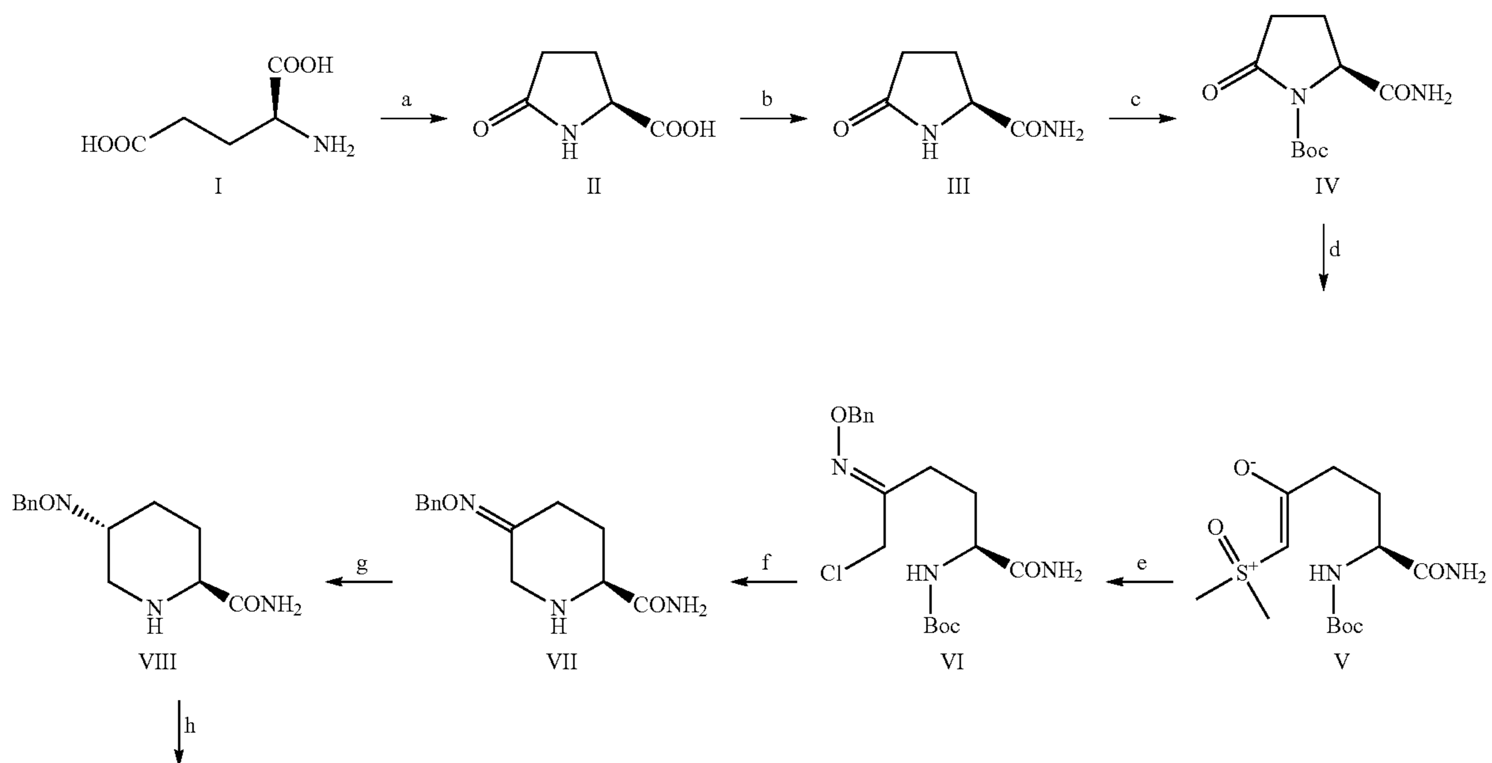
Scheme 3
