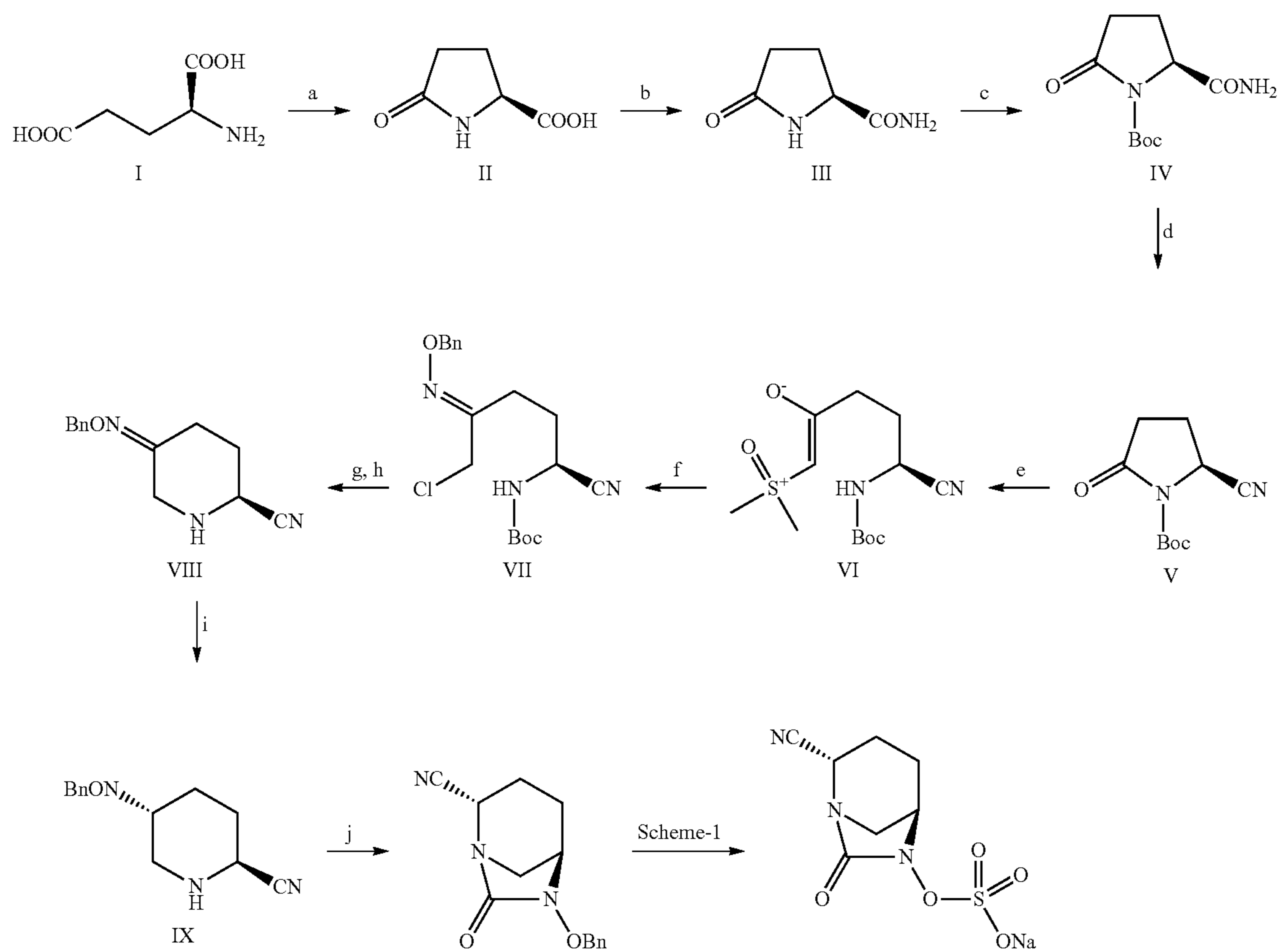
Scheme 2
