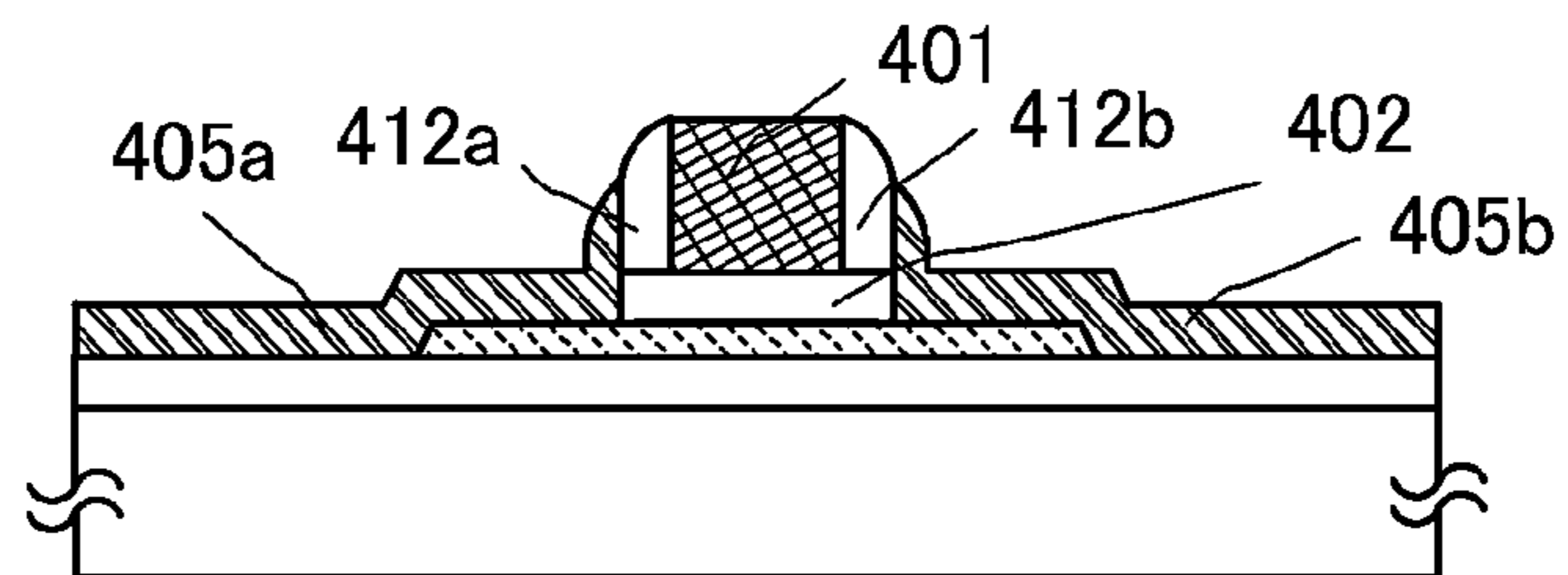
FIG. 2D
