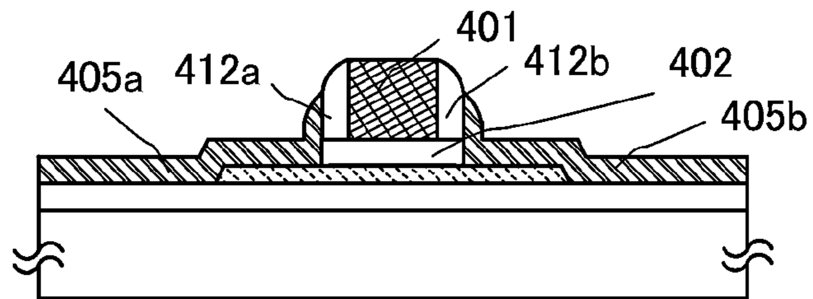
FIG. 1D
