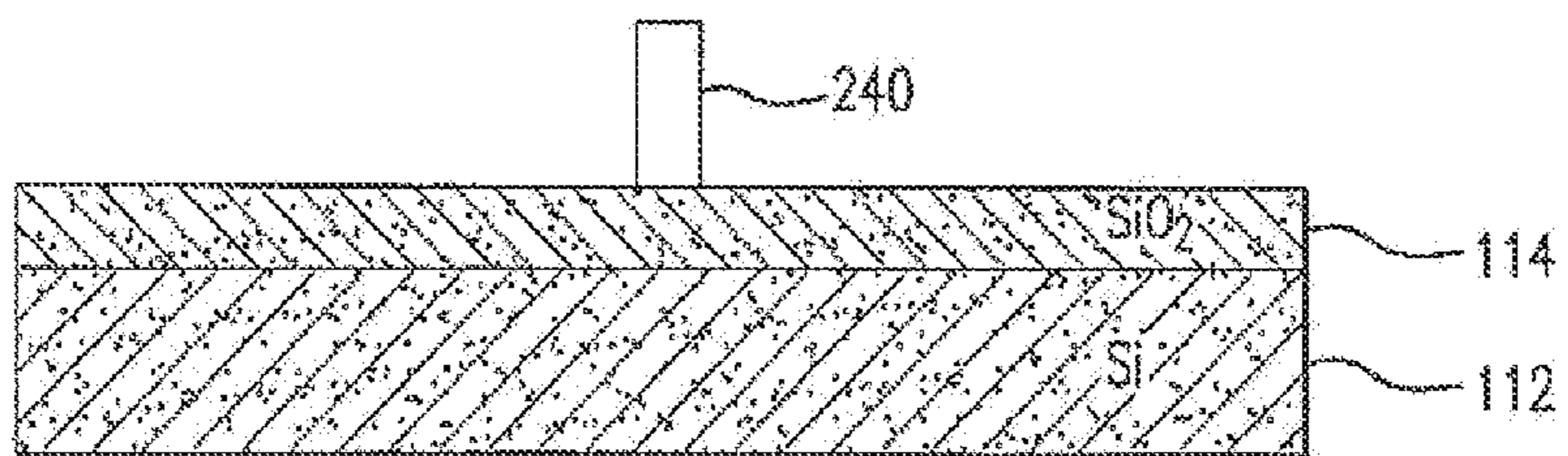
Grow Nanotube
