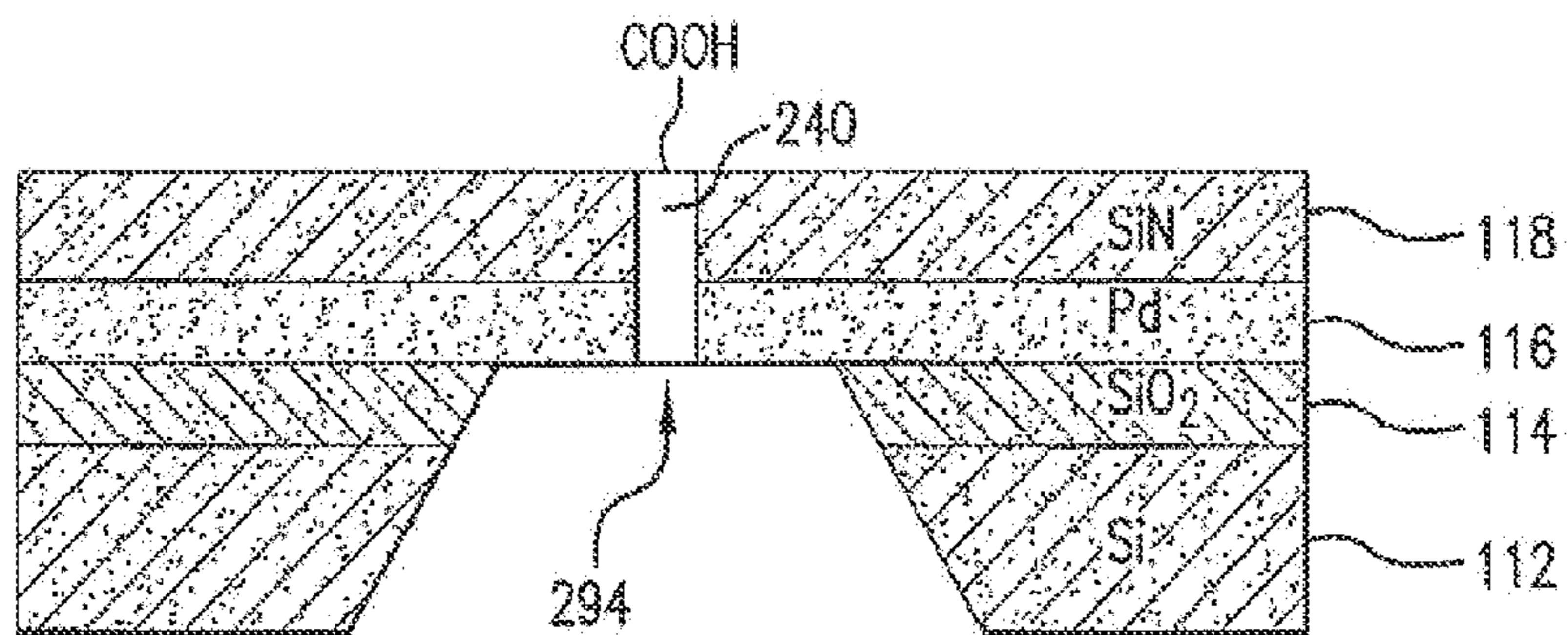
Etch Window on Back Side
