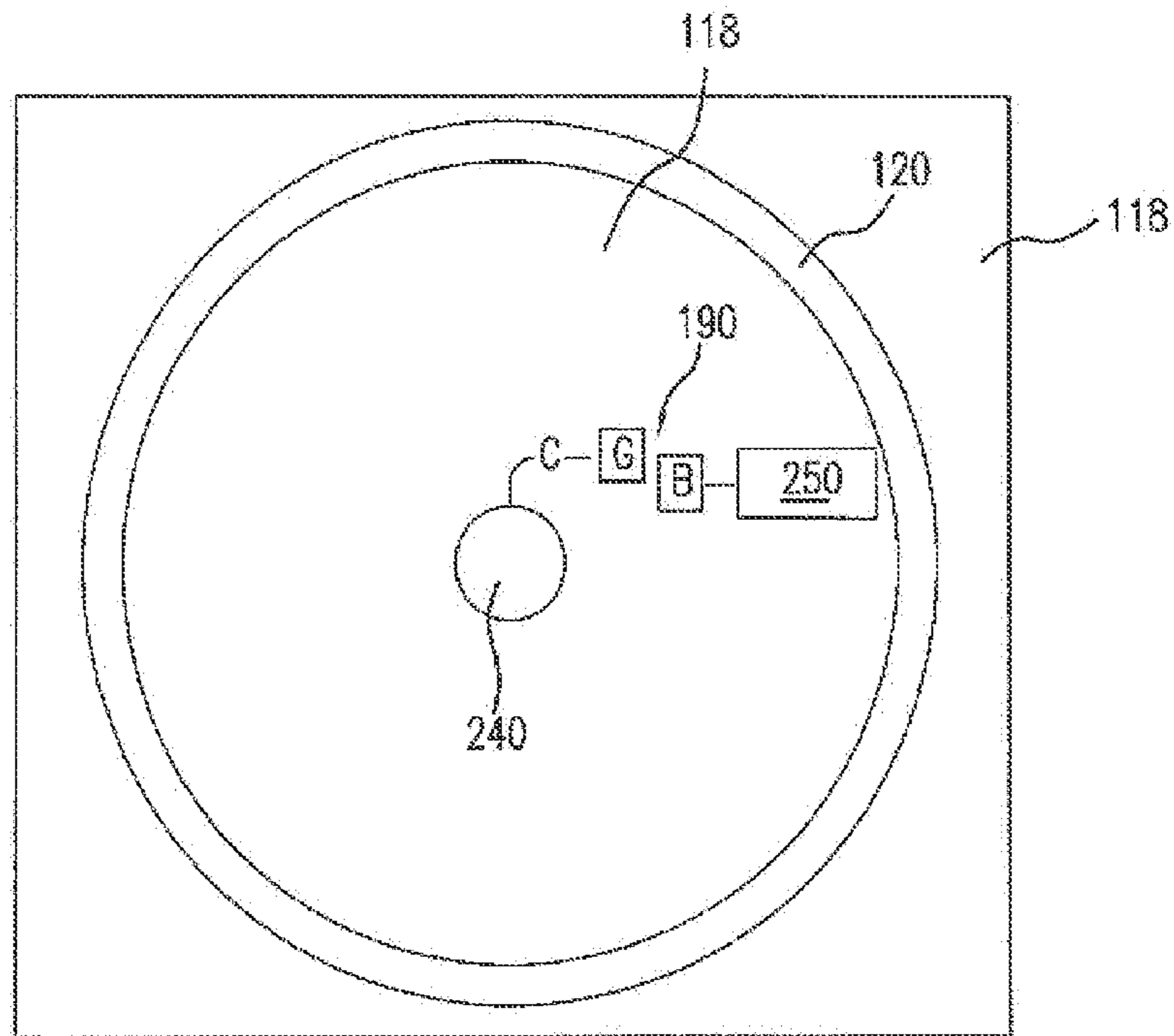
Top View of FIG. 2L After Removal of Passivation Layer of removal of sacrificial nucleotide
