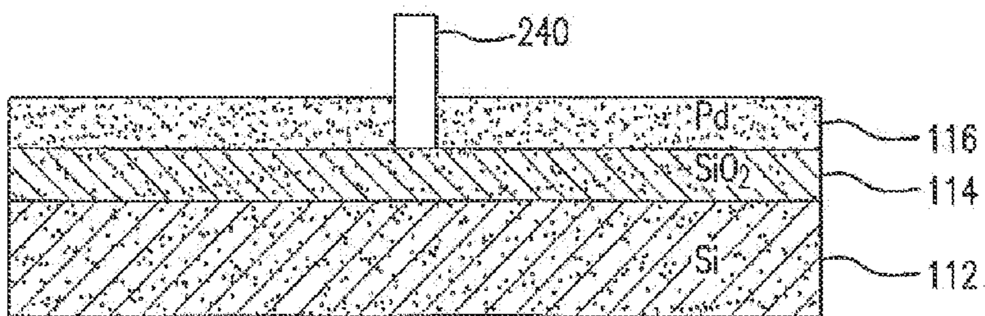
Deposit Pd
