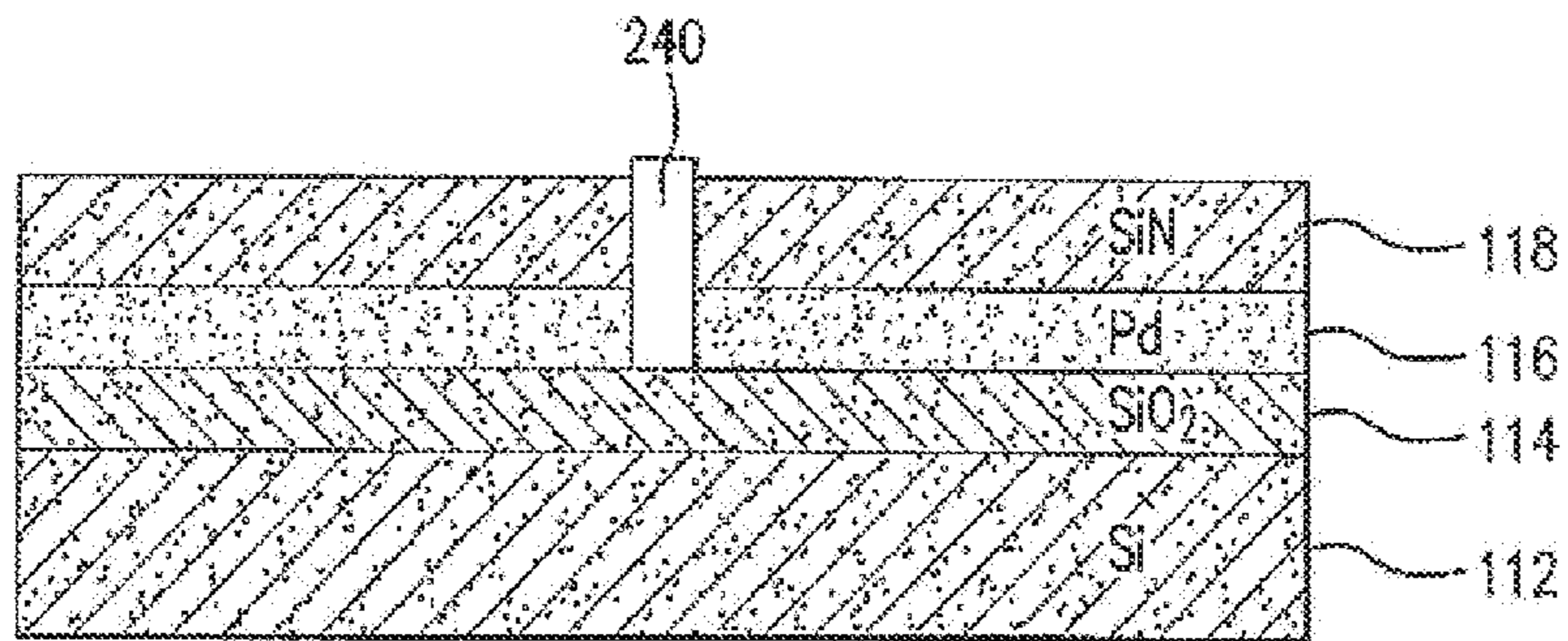
Deposit SiN FIG.2D
