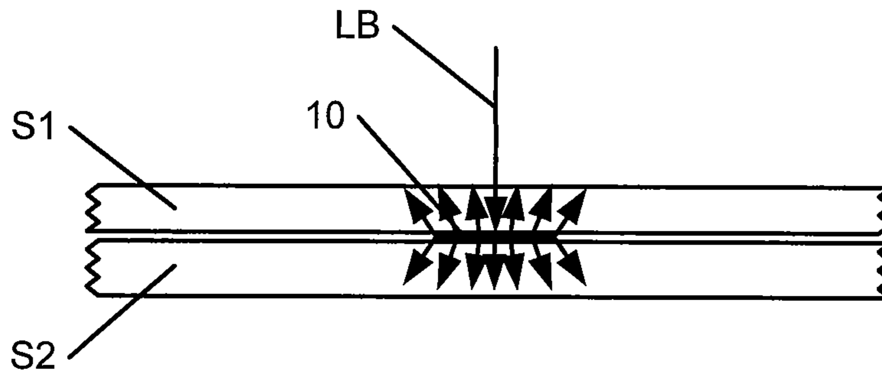
FIG. 1 (Prior Art)
