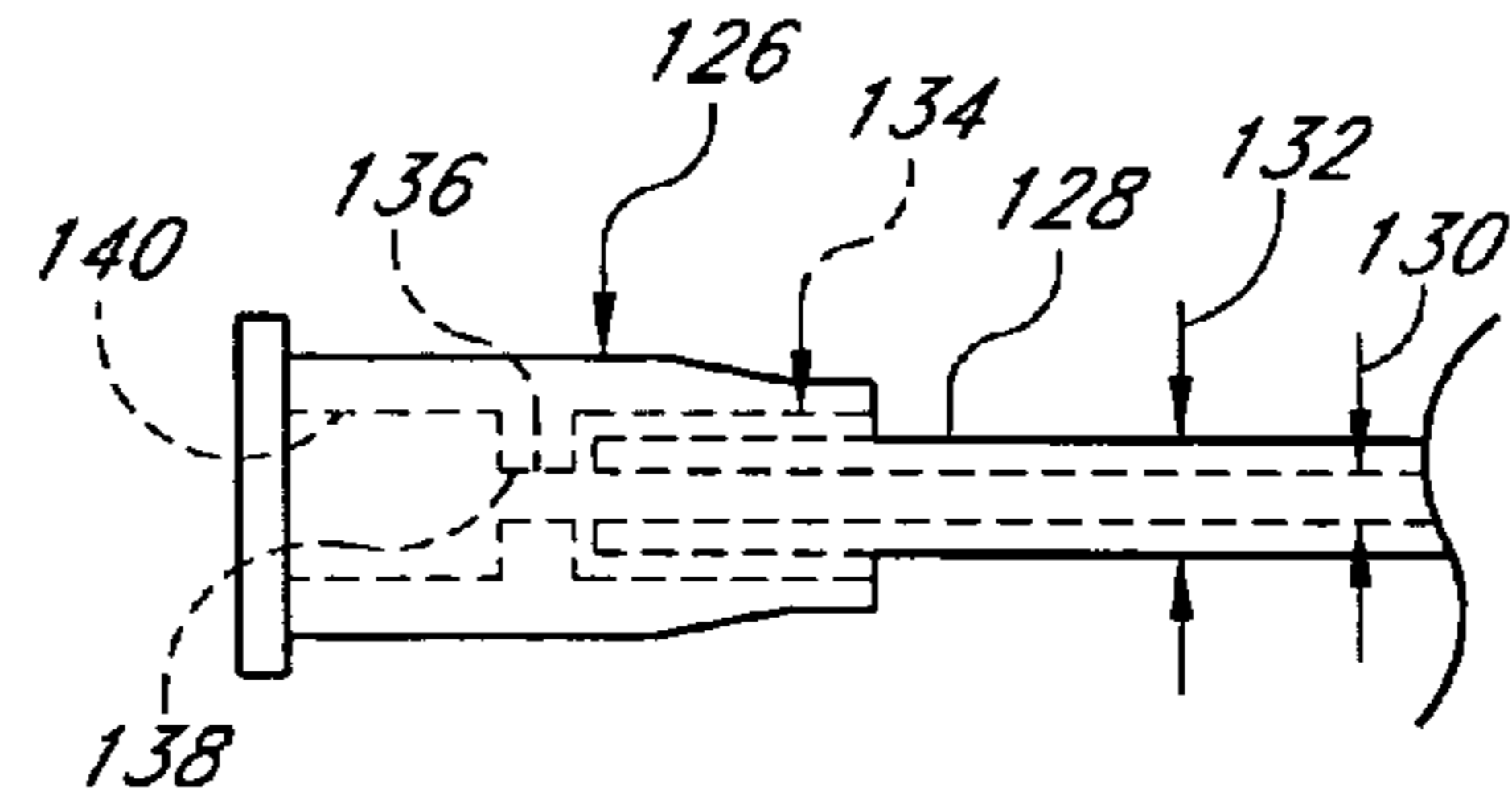
FIG. 15 (PRIOR ART)
