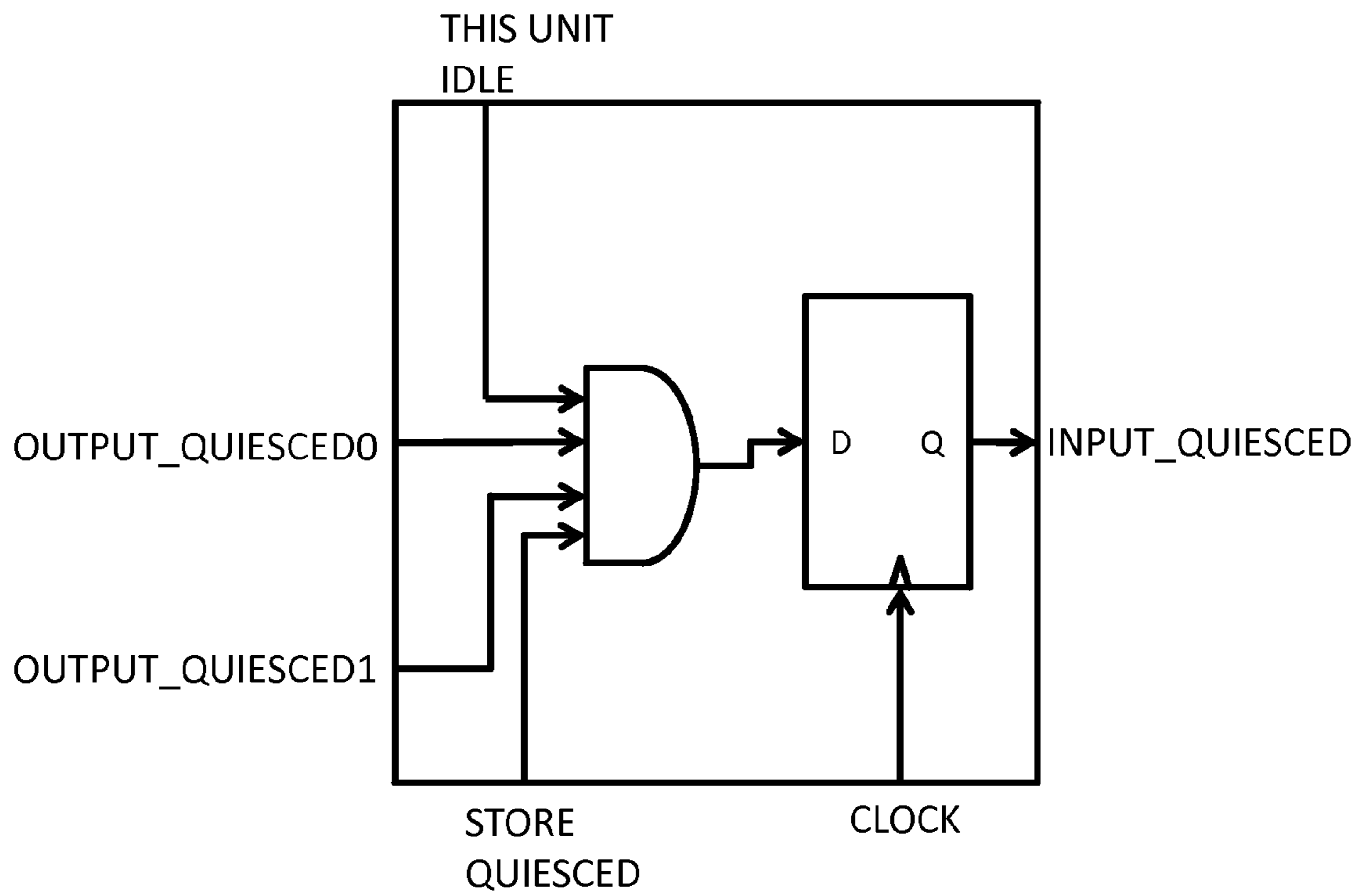
FIG 11 A quiescence circuit building block (Qunit)
