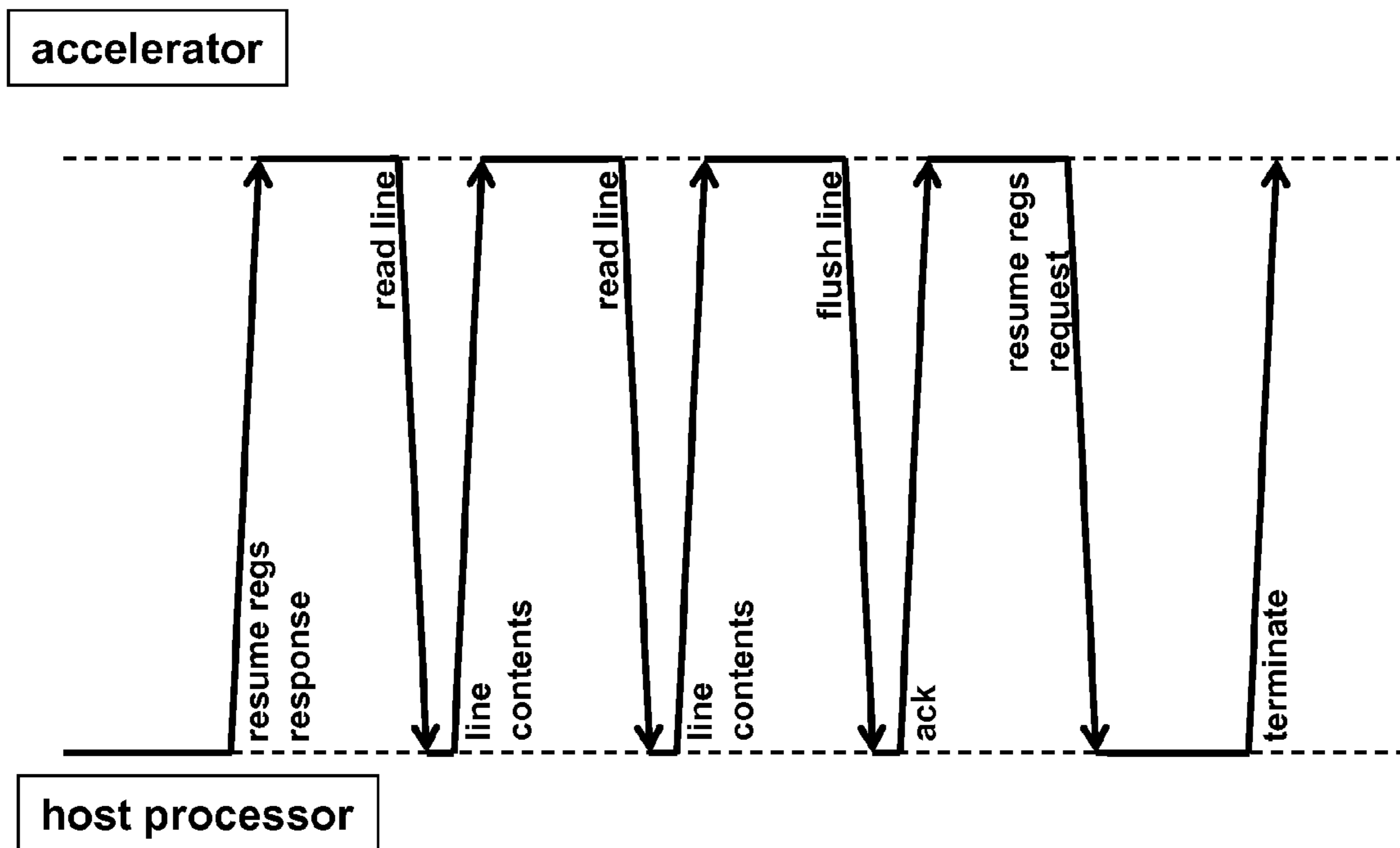
FIG 20 Example of Host-Accelerator communication protocol
