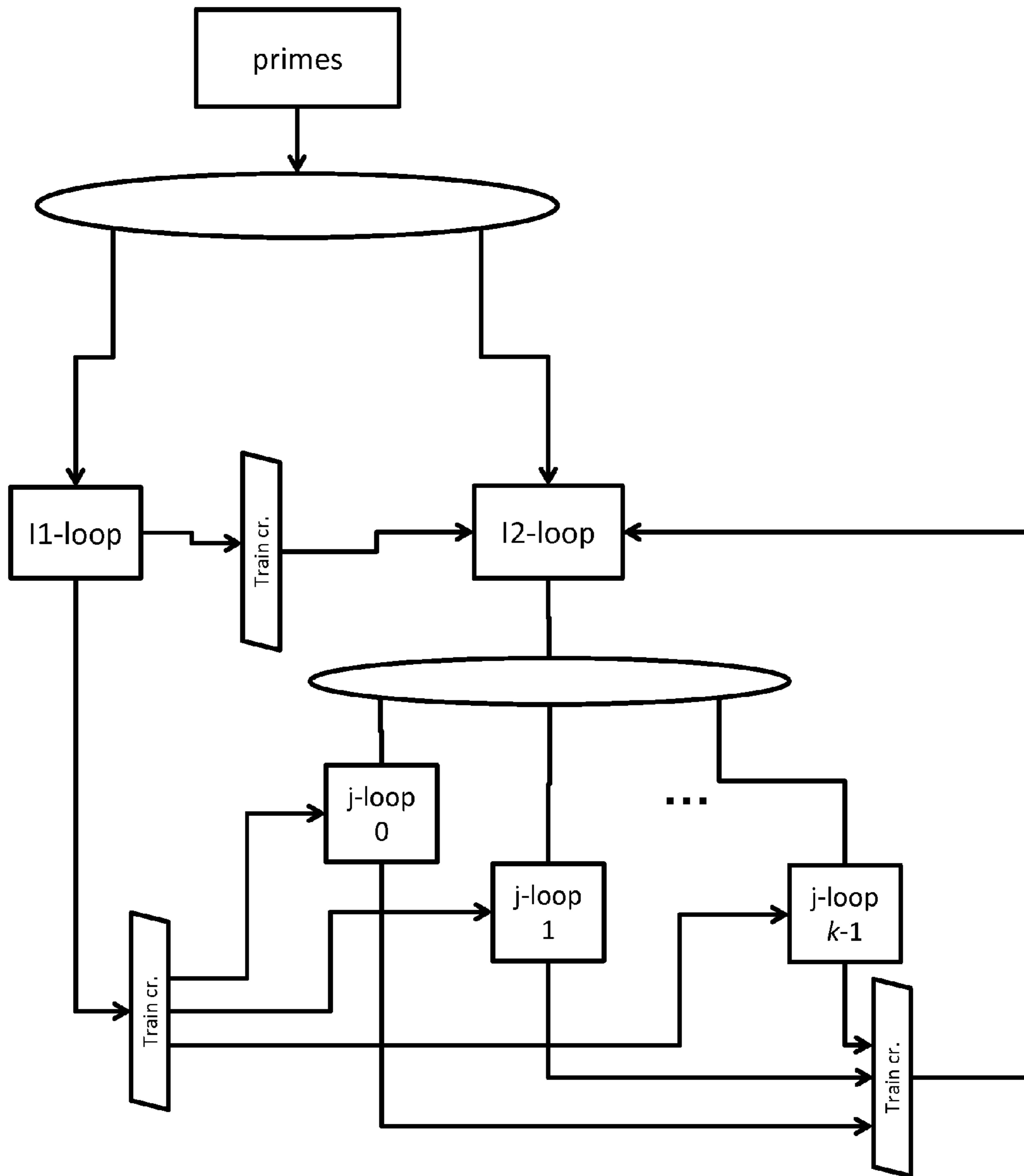
FIG 53 Hardware implementation of Eratosthenes's Sieve
