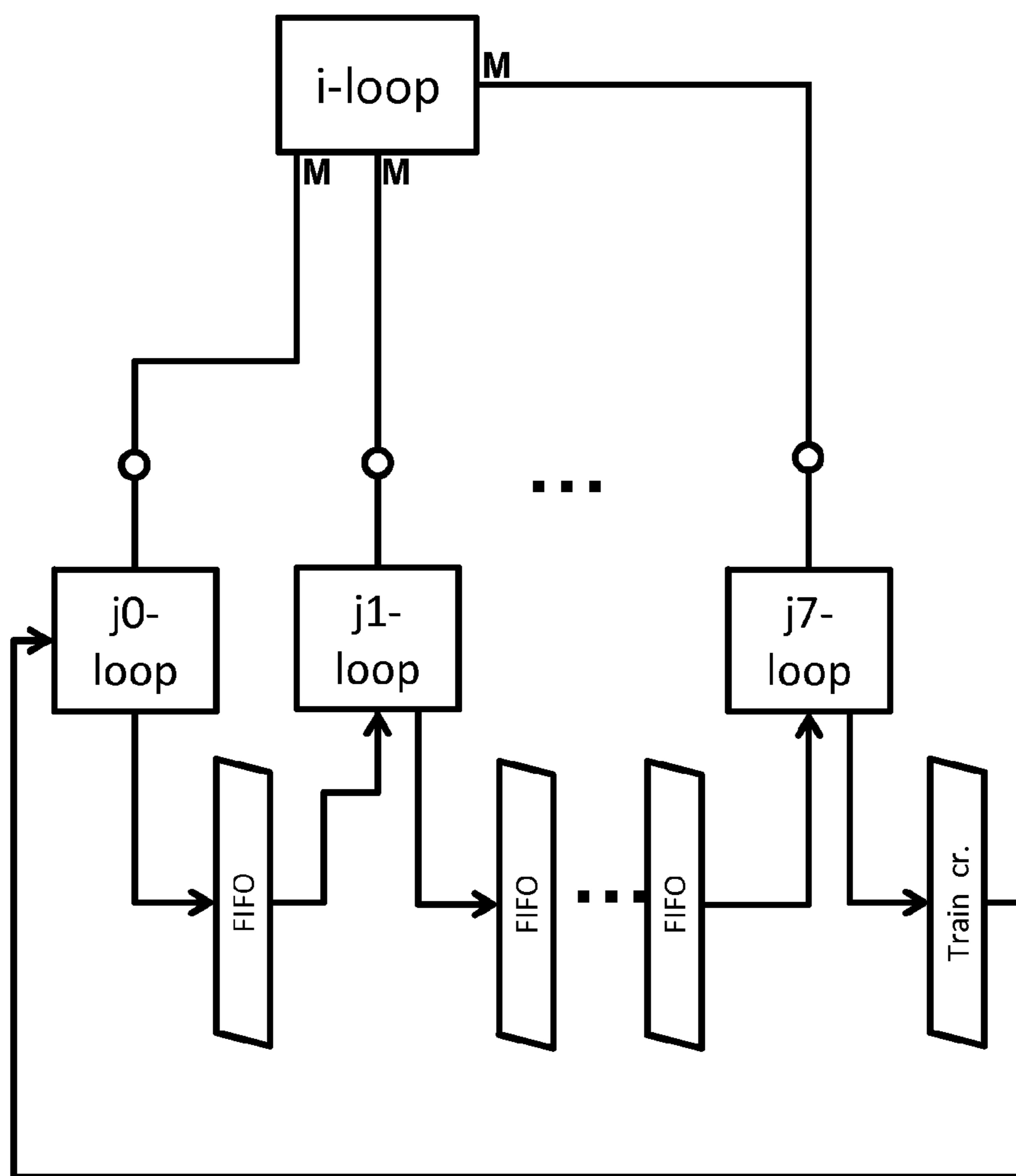
FIG 57 Cascaded filter implementation of bubble sort.
