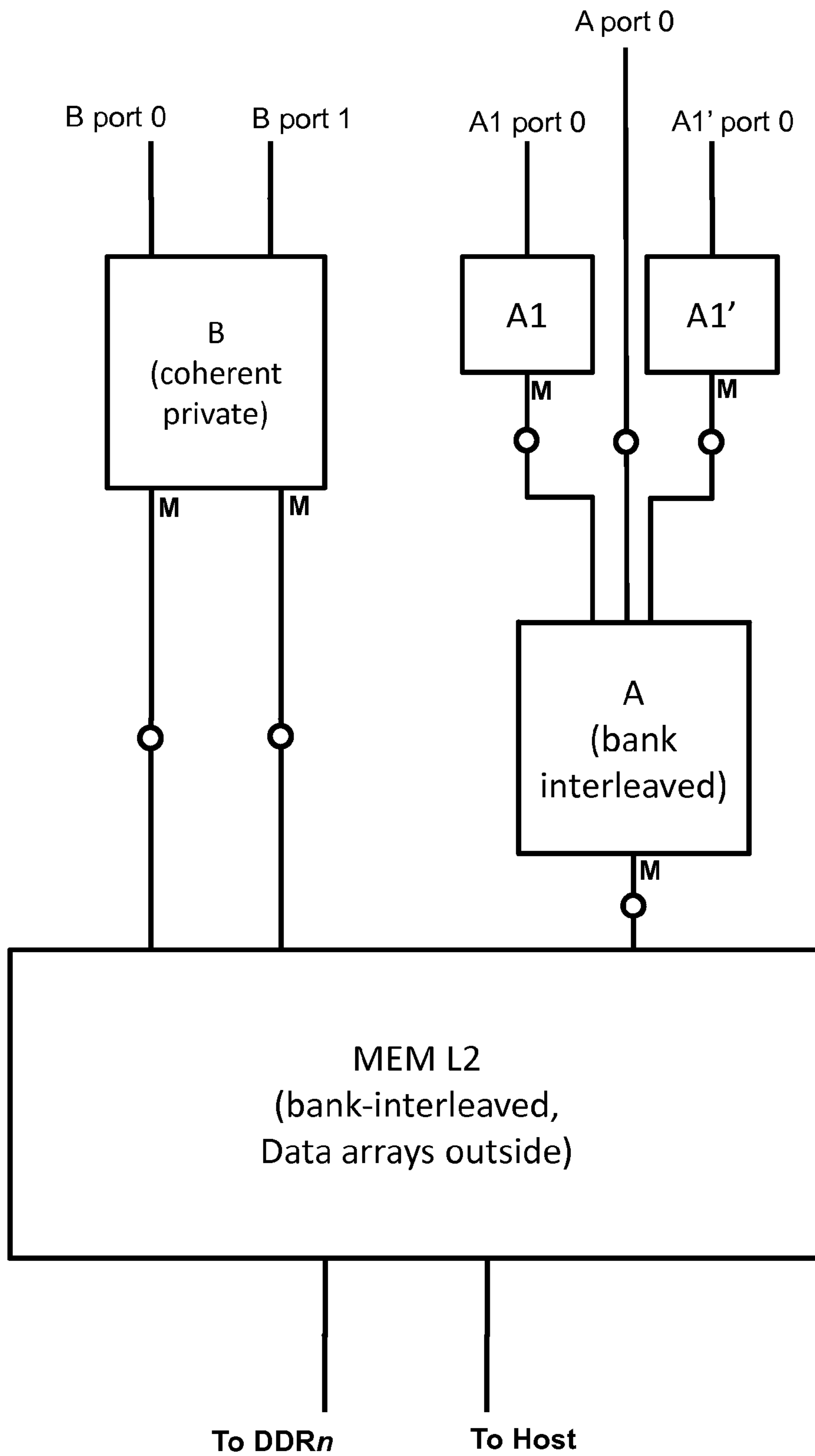
FIG 45 Implementation of memory hierarchy example
