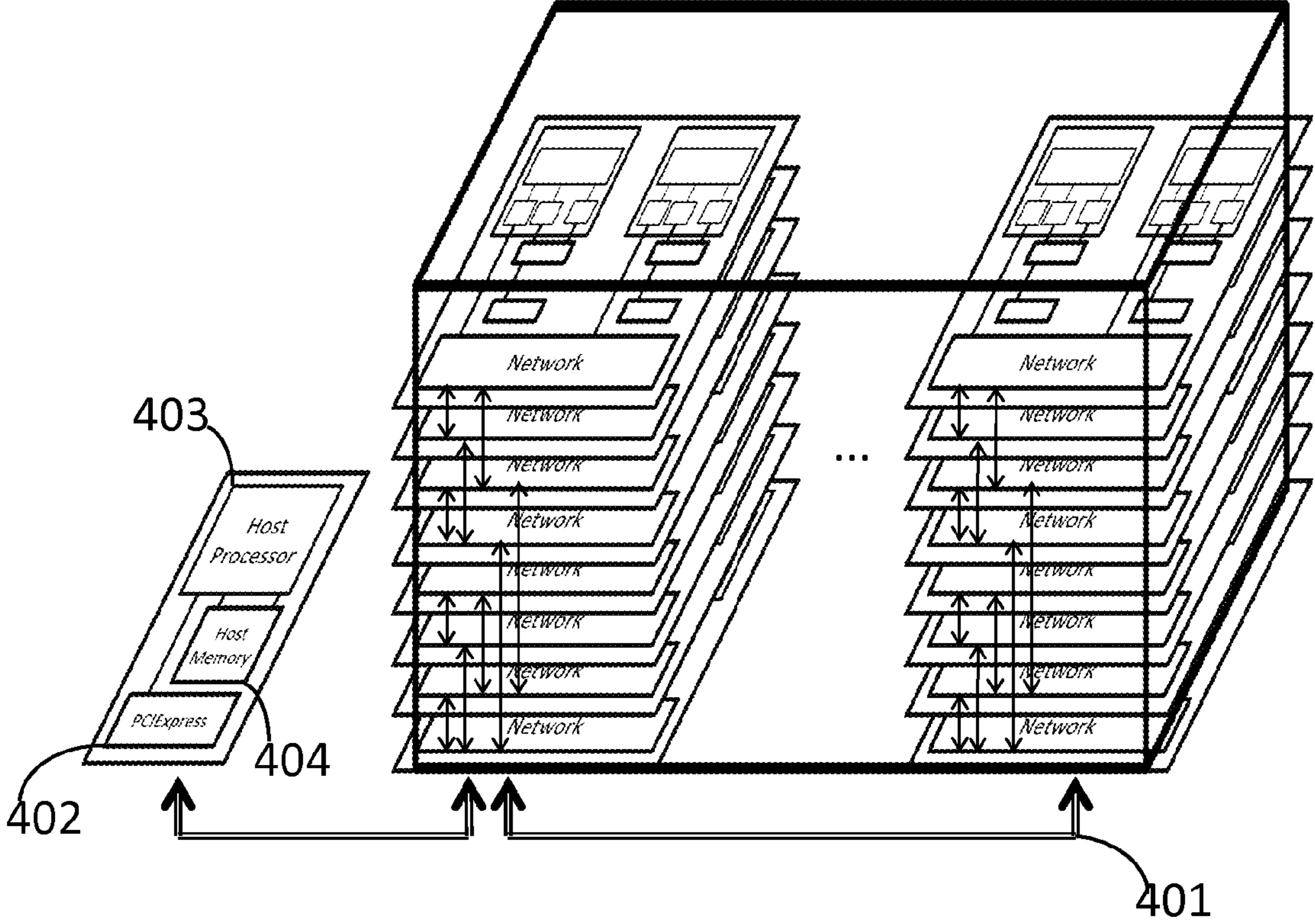
FIG 4 Supercomputer at the whole system level
