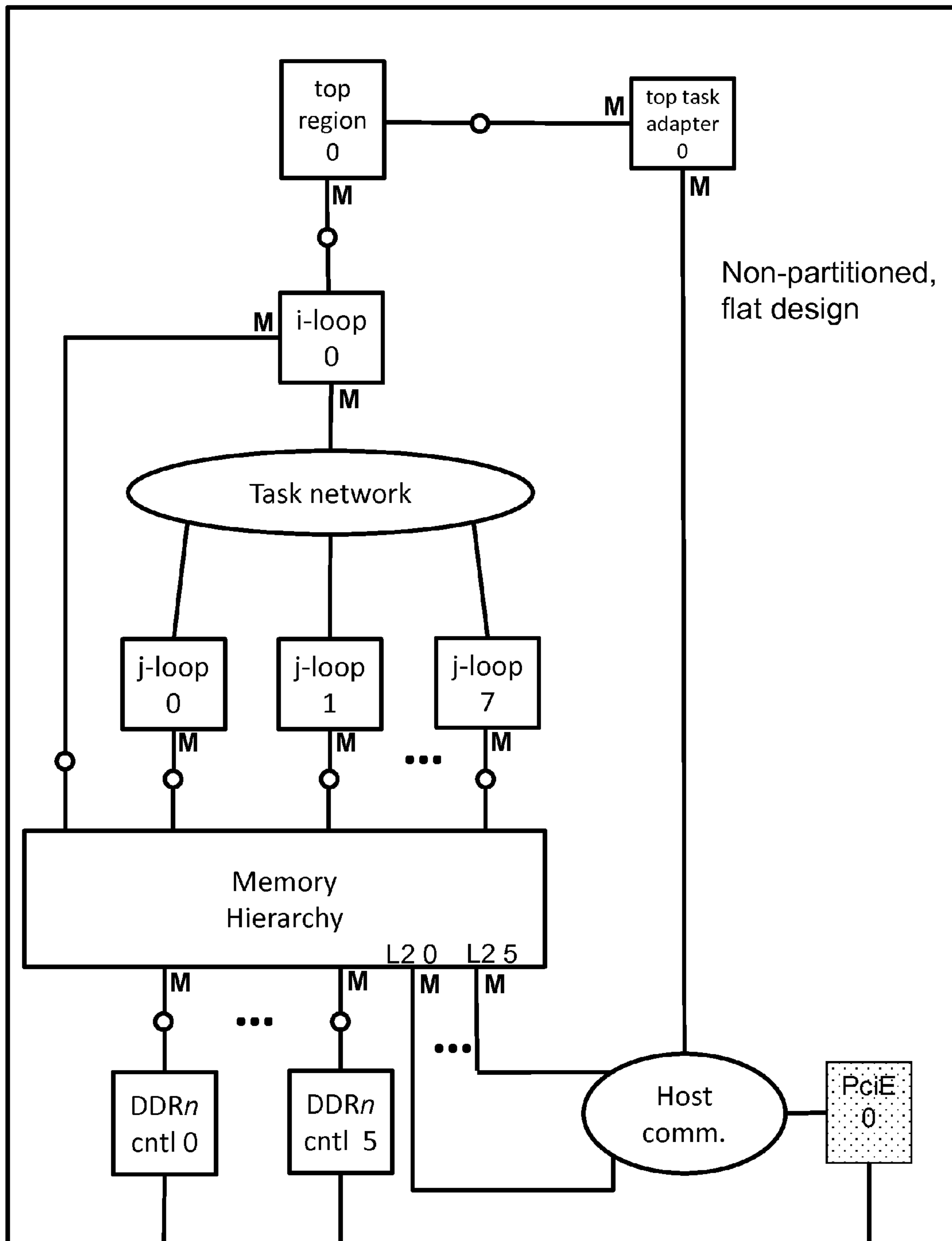
FIG 19 A flat design for RandomAccess
