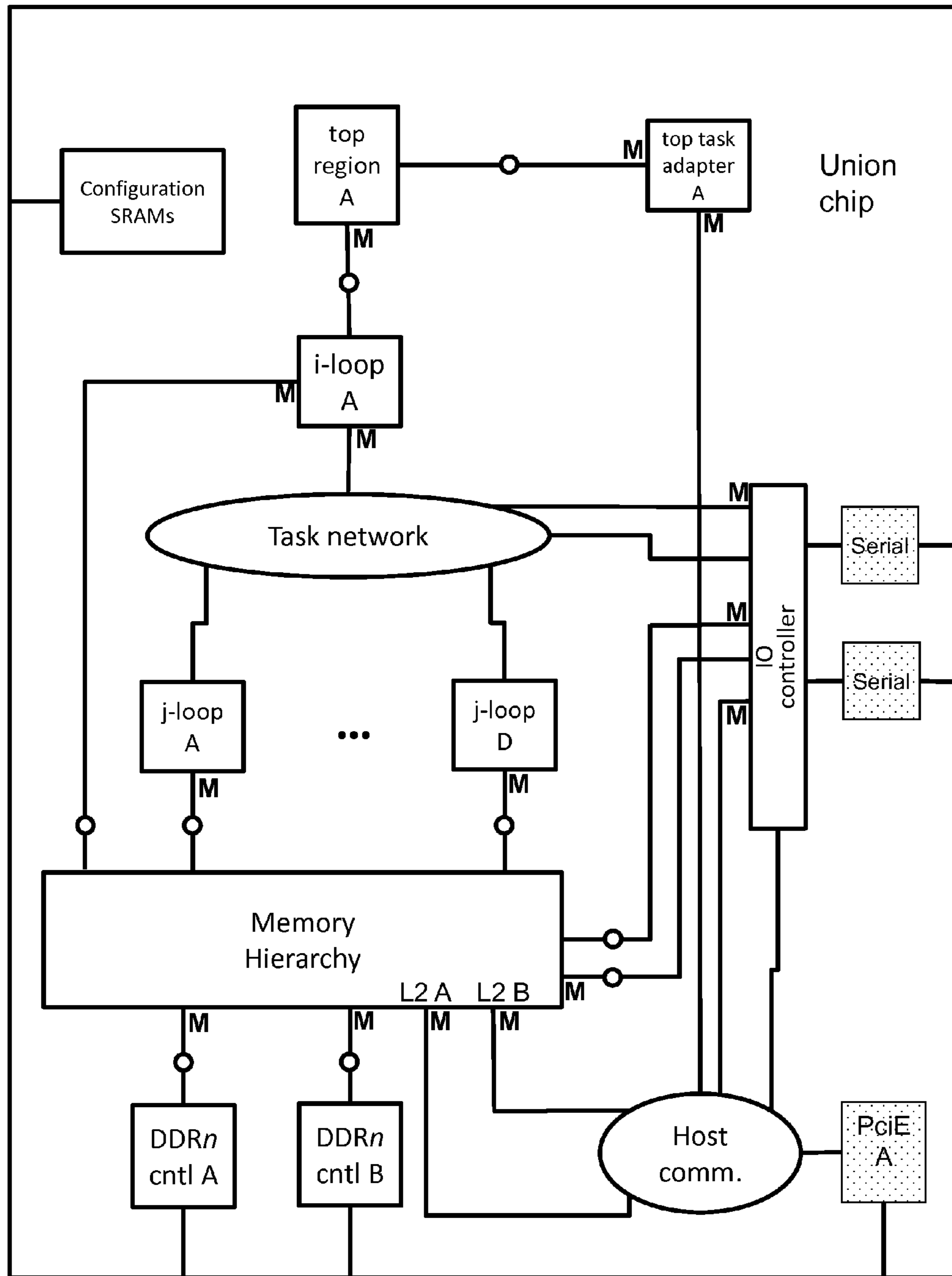
FIG 36 The Union Chip
