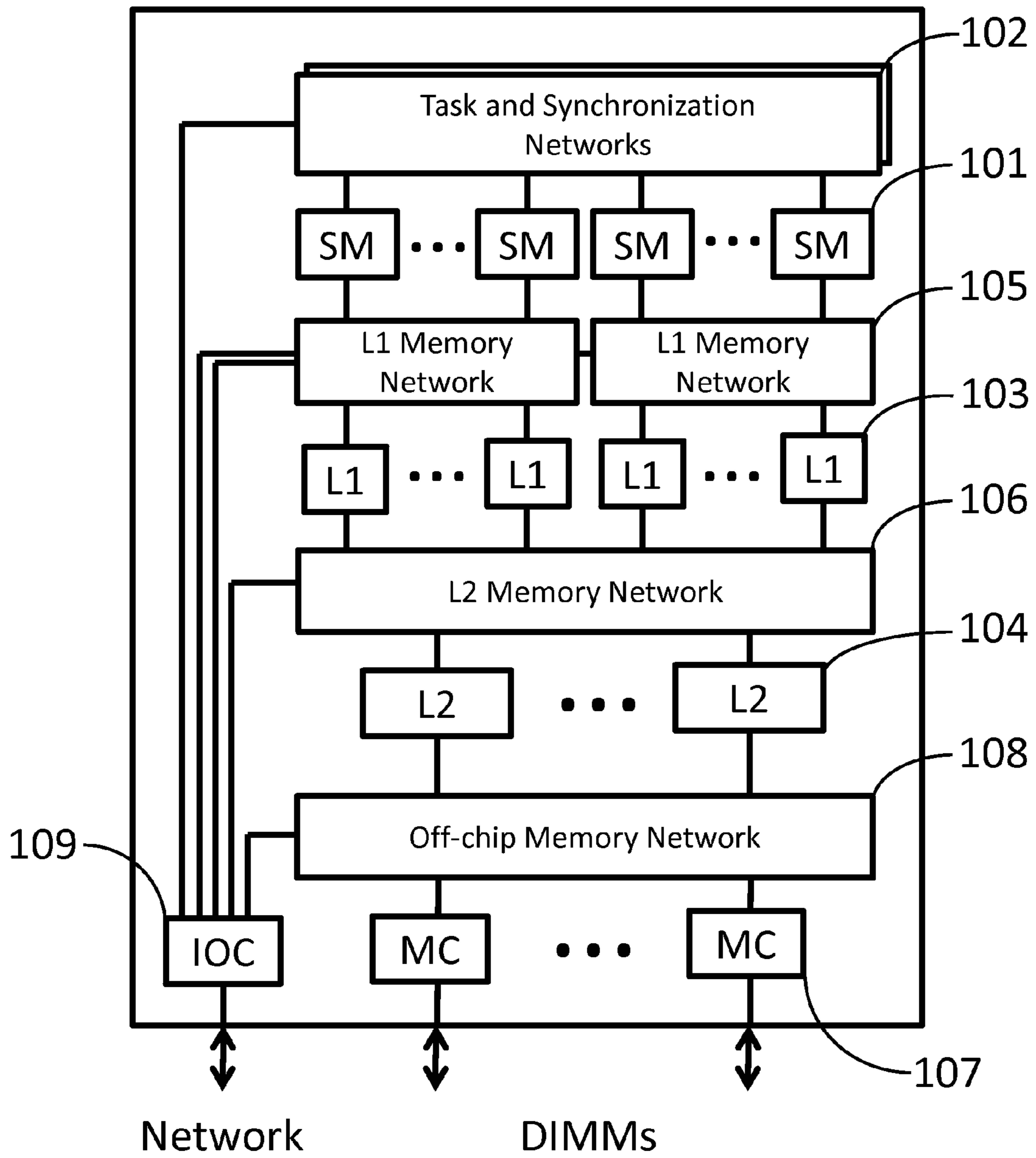
FIG 1 Supercomputer at the chip level
