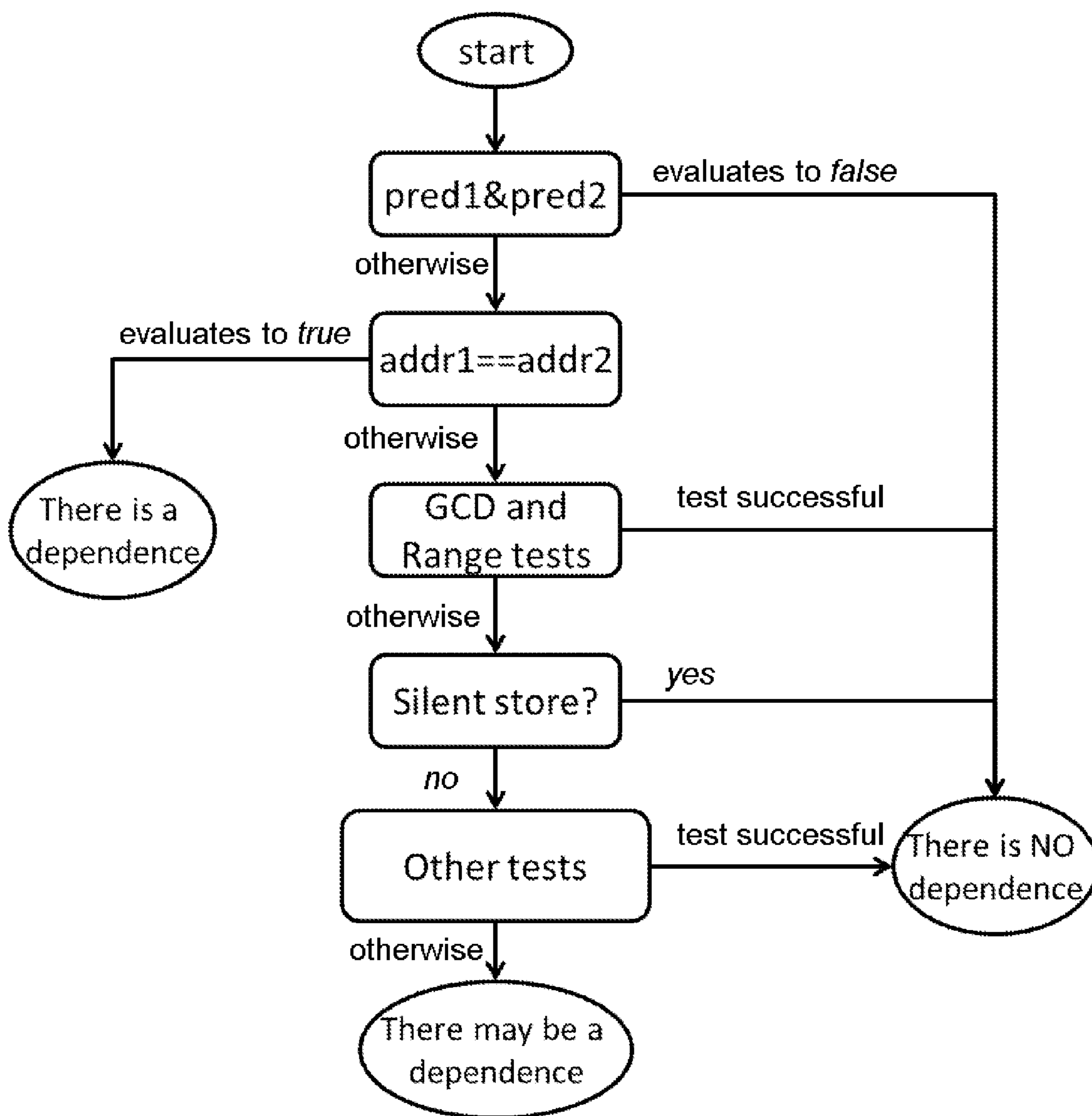
FIG 71 Algorithm for dependence analysis
