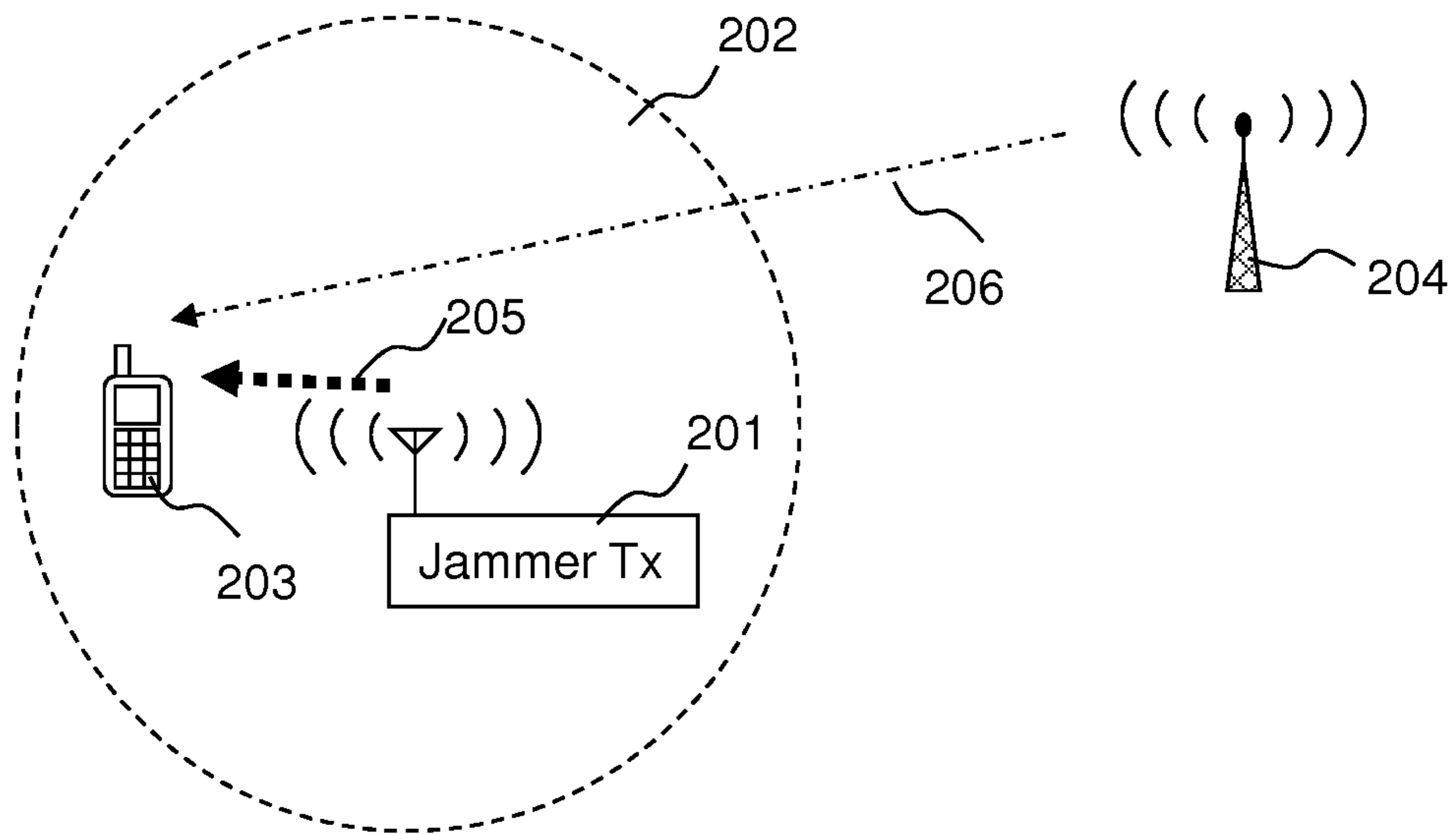
FIG. 2 (Prior Art)
