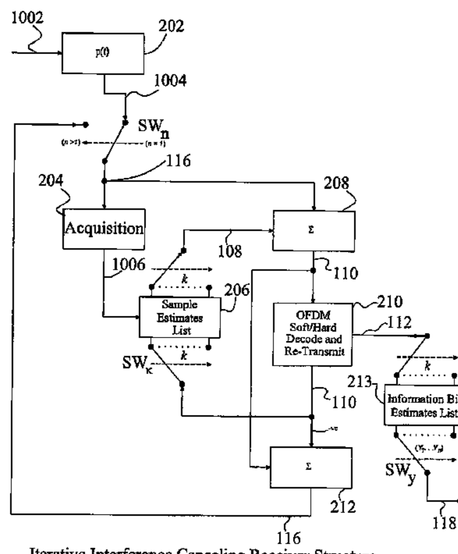
Iterative Interference Canceling Receiver Structure
