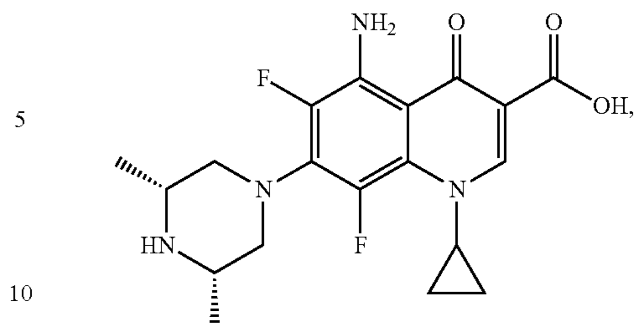
Sparfloxacin
