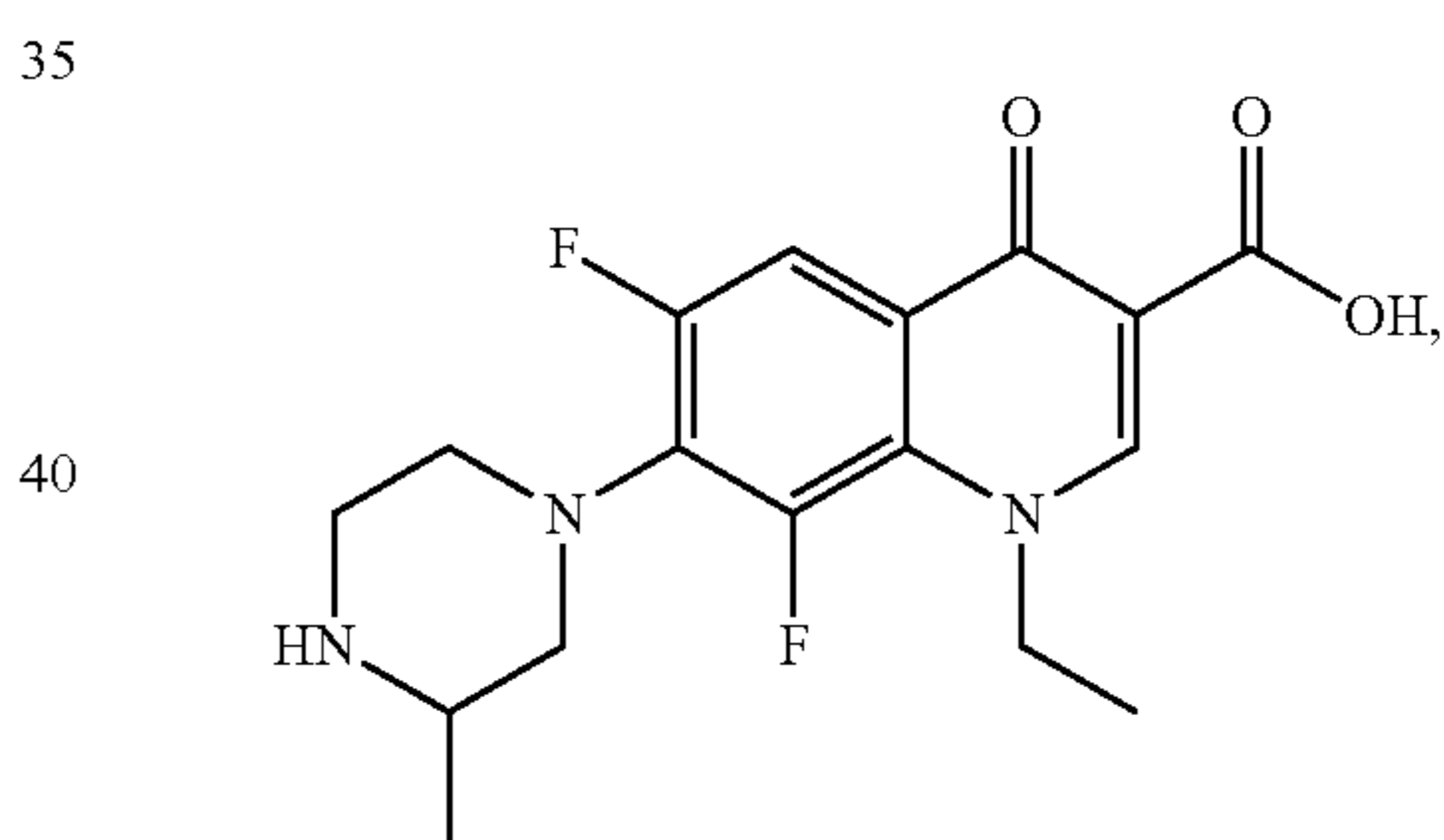
Lomefloxacina
