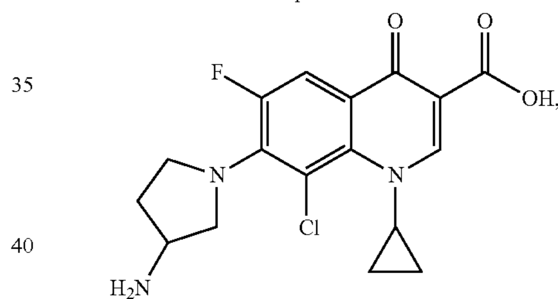
Clinafloxacin
