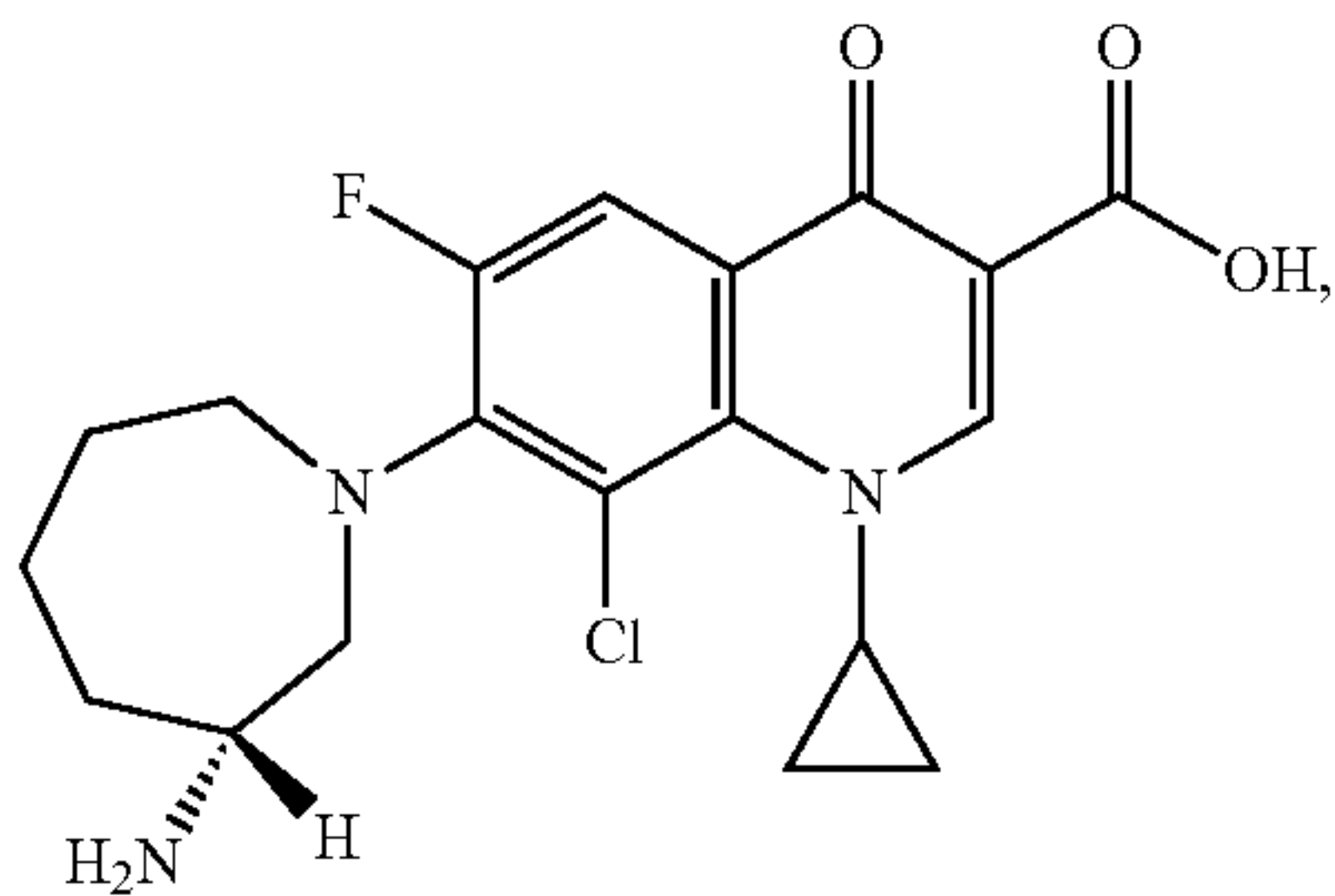
Besifloxacin
