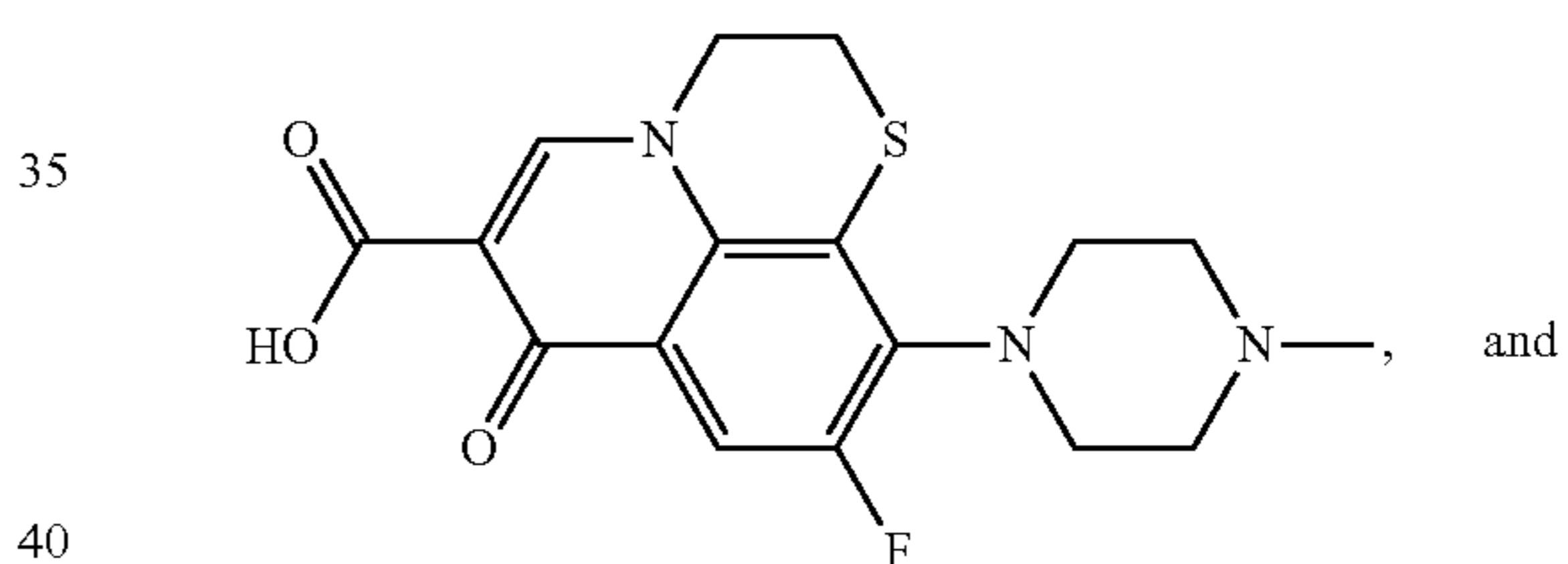
Rufloxacin
