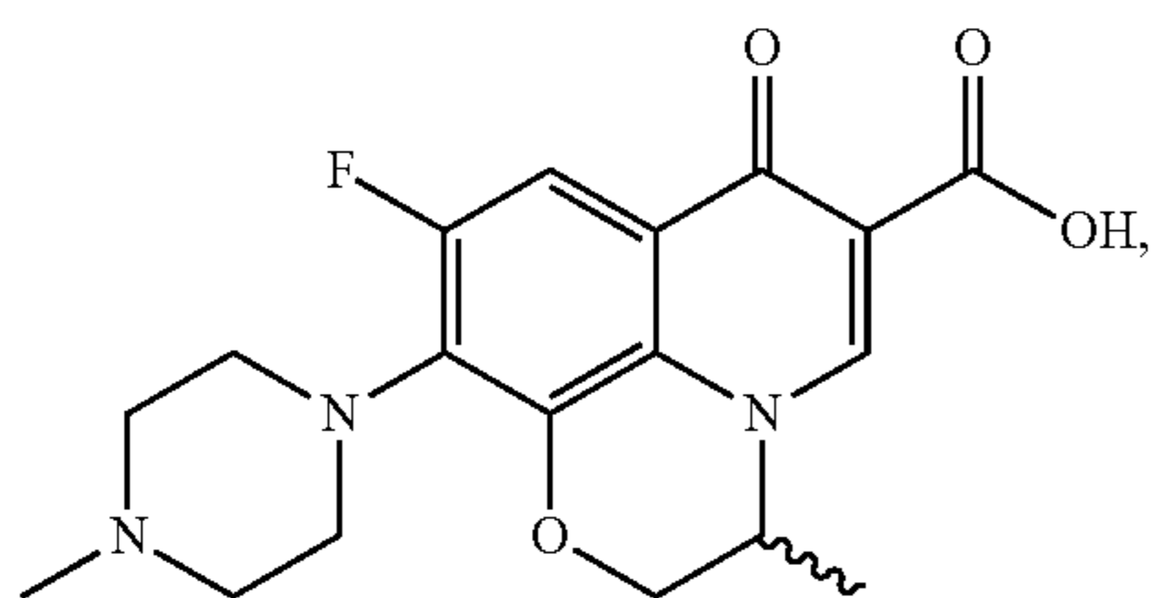
Ofloxacin
