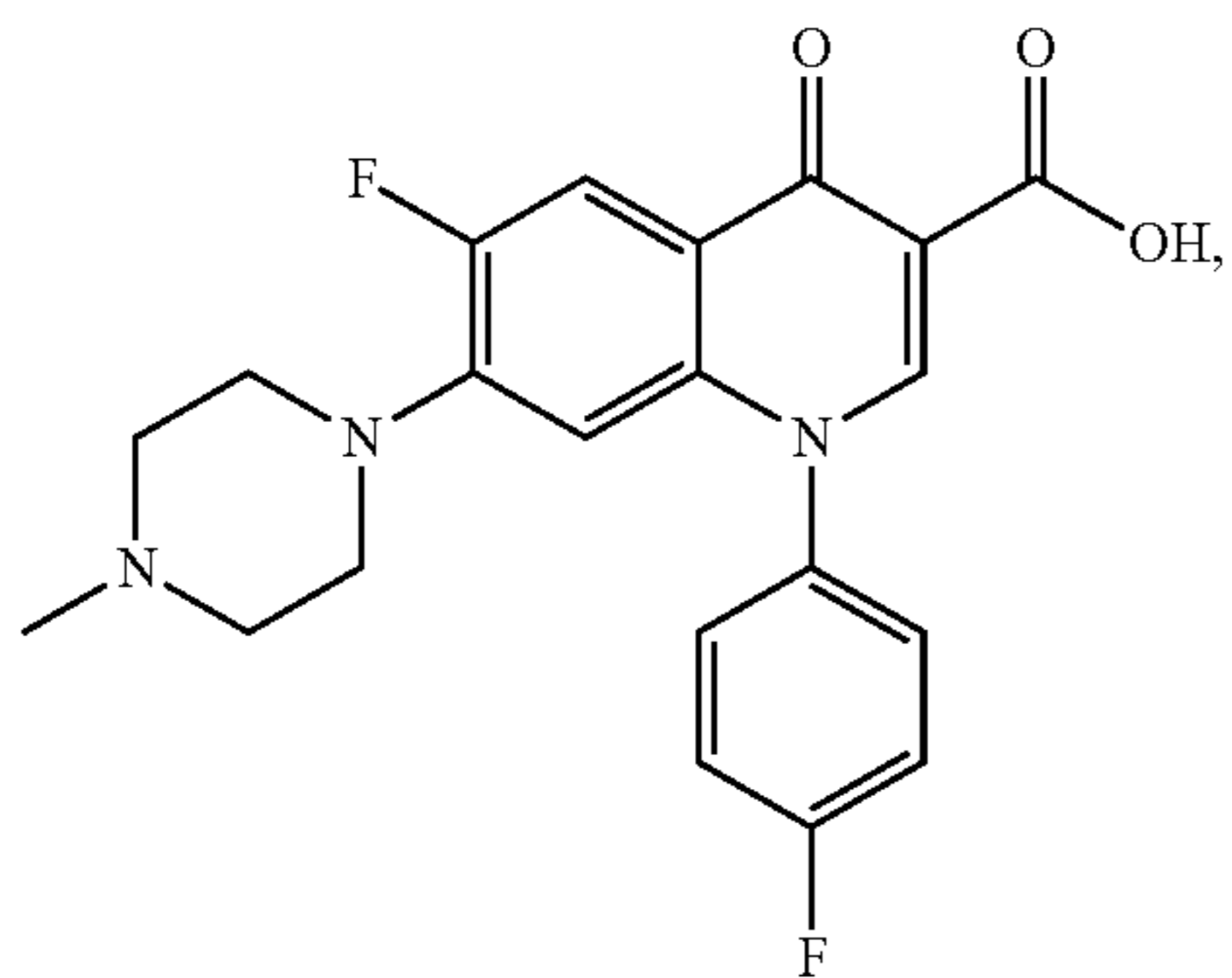
Difloxacina
