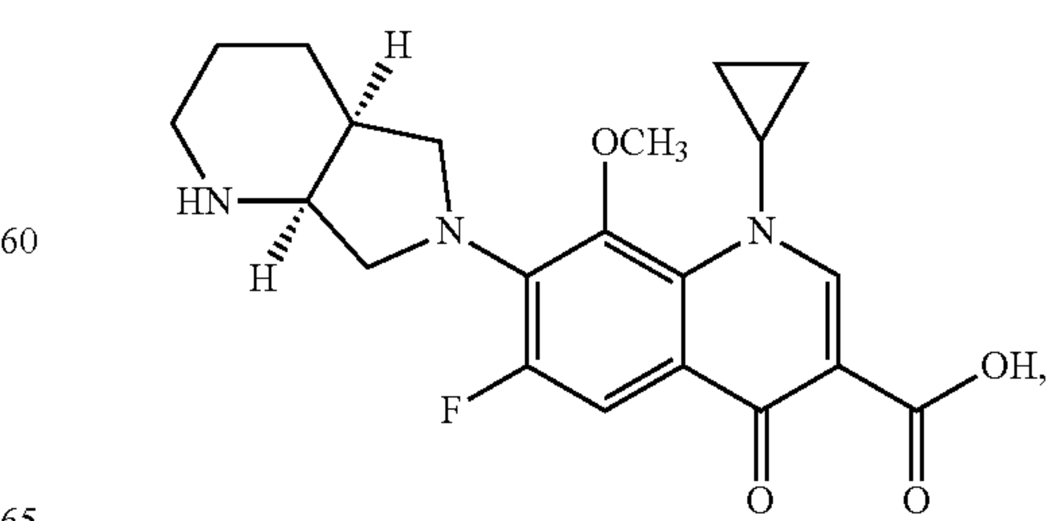
Moxifloxacin
