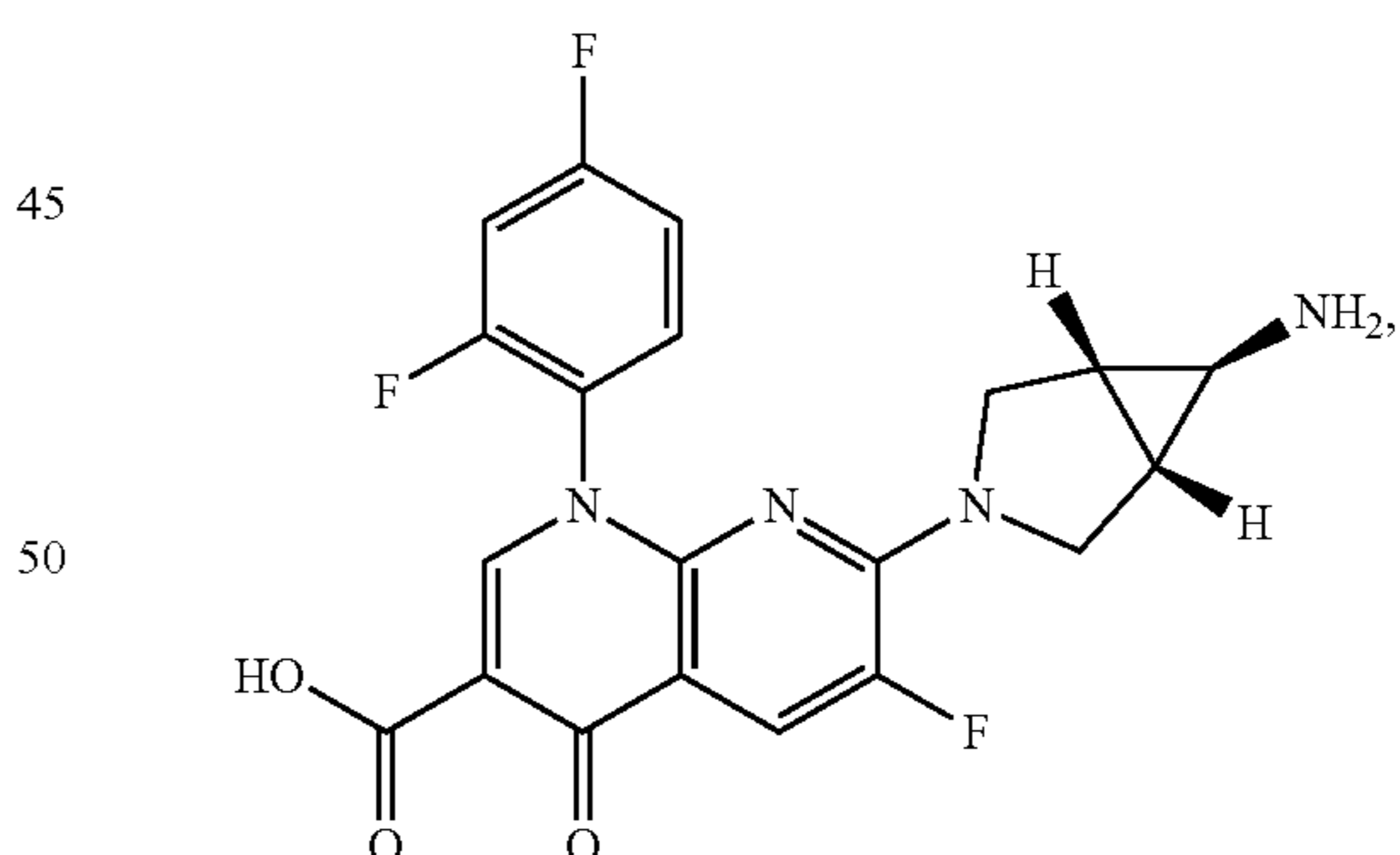
Trovafloxacin
