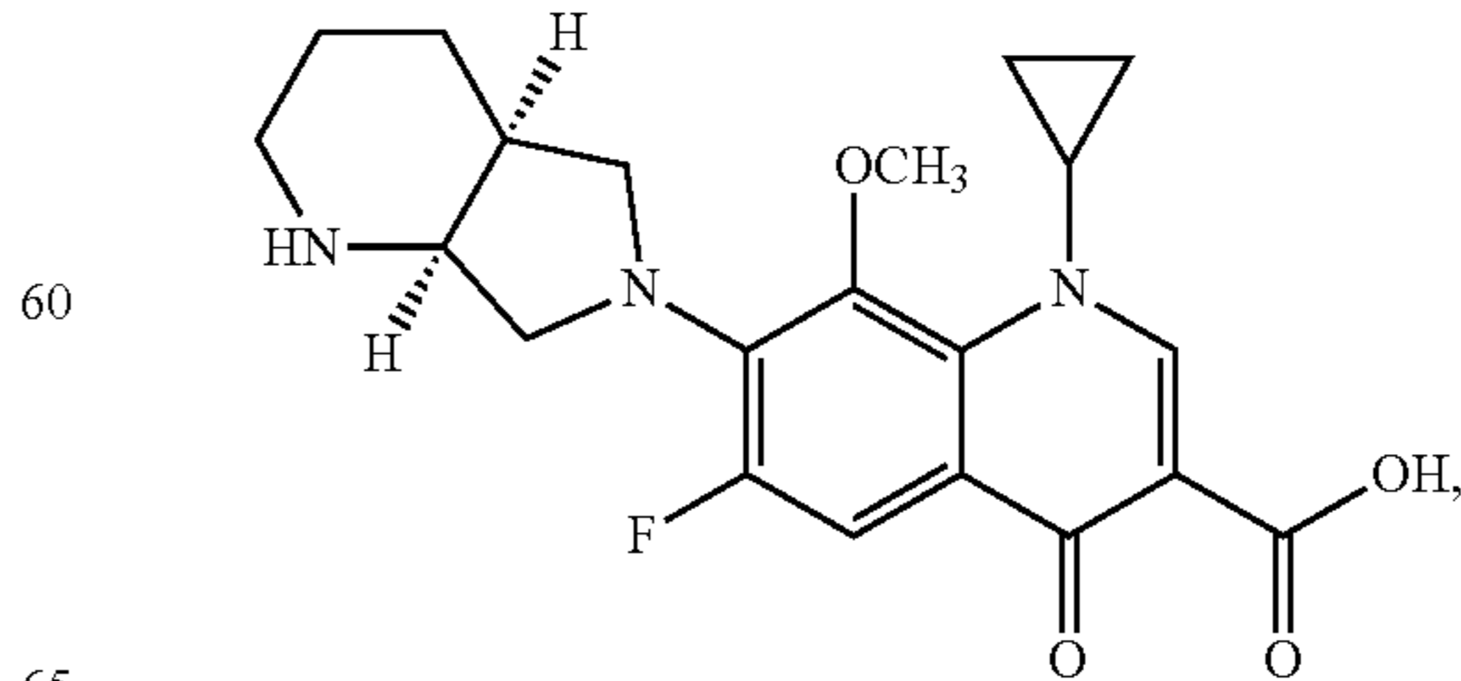
Moxifloxacina
