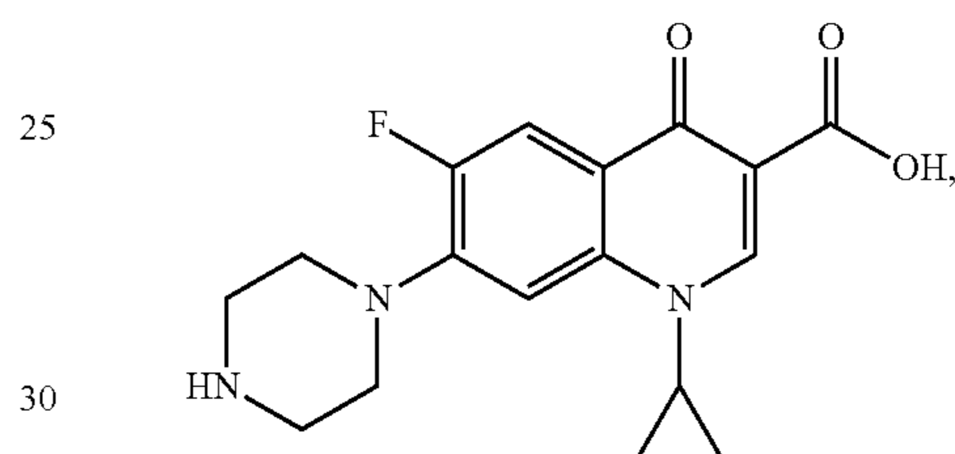
Ciprofloxacin
