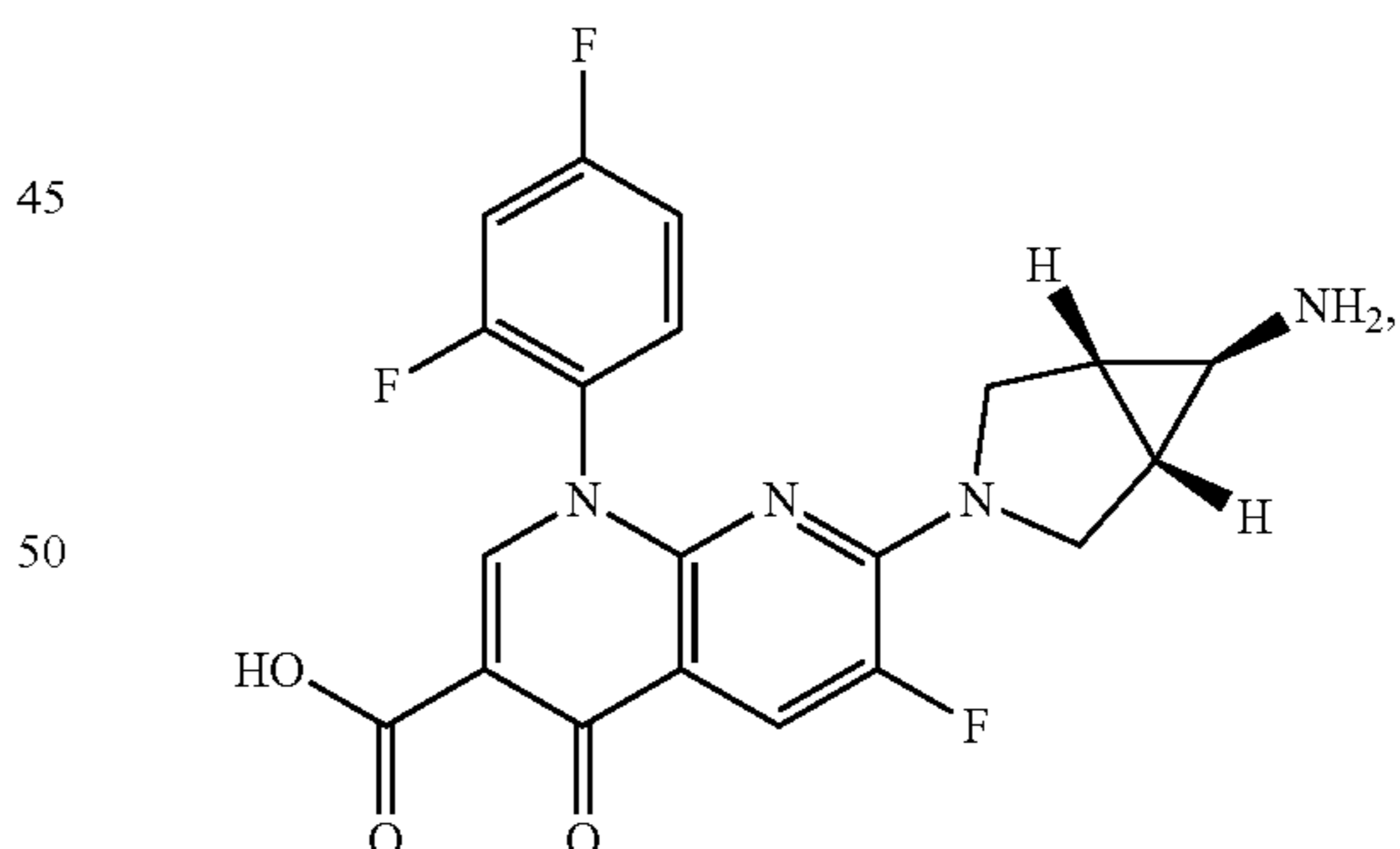
Trovafloxacin
