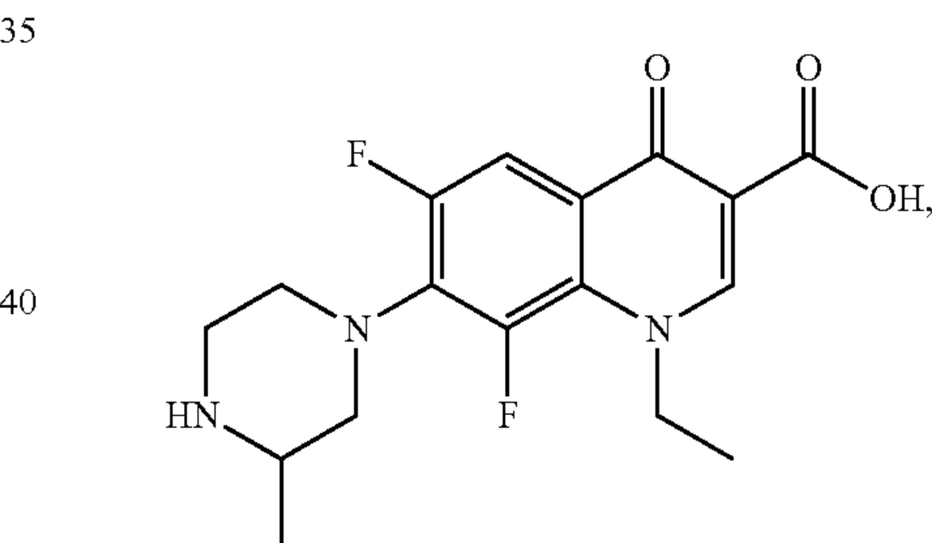
Lomefloxacin
