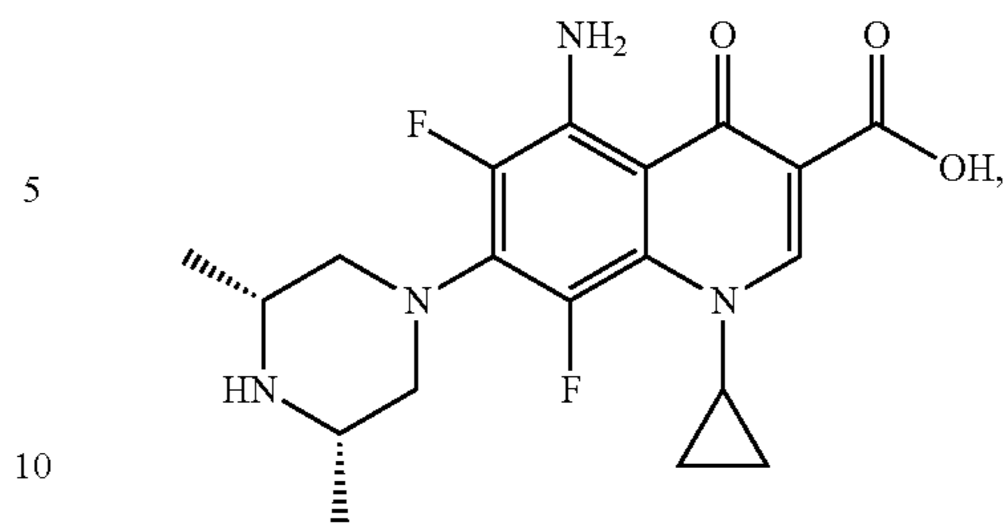
Sparfloxacin
