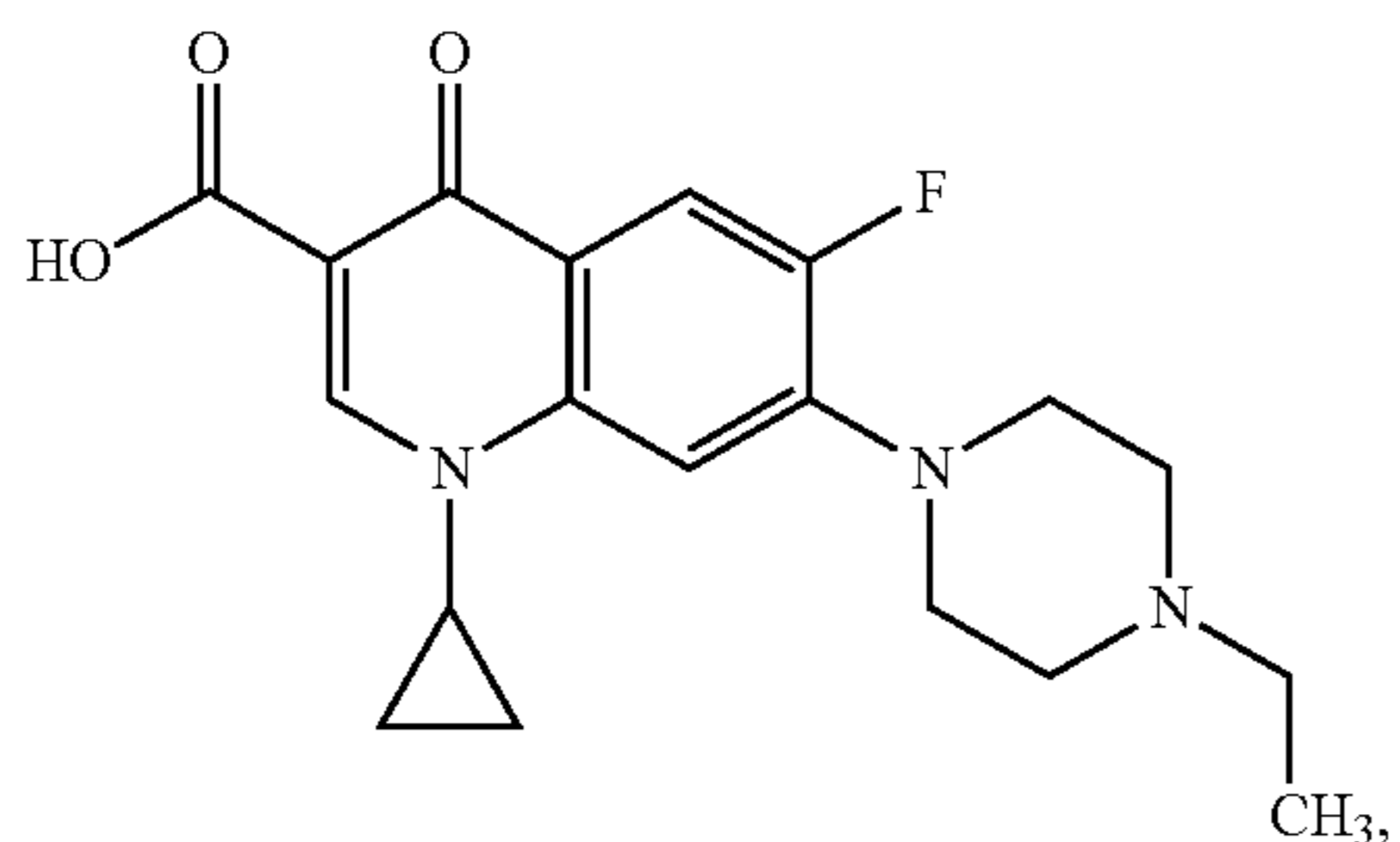
Enrofloxacin
