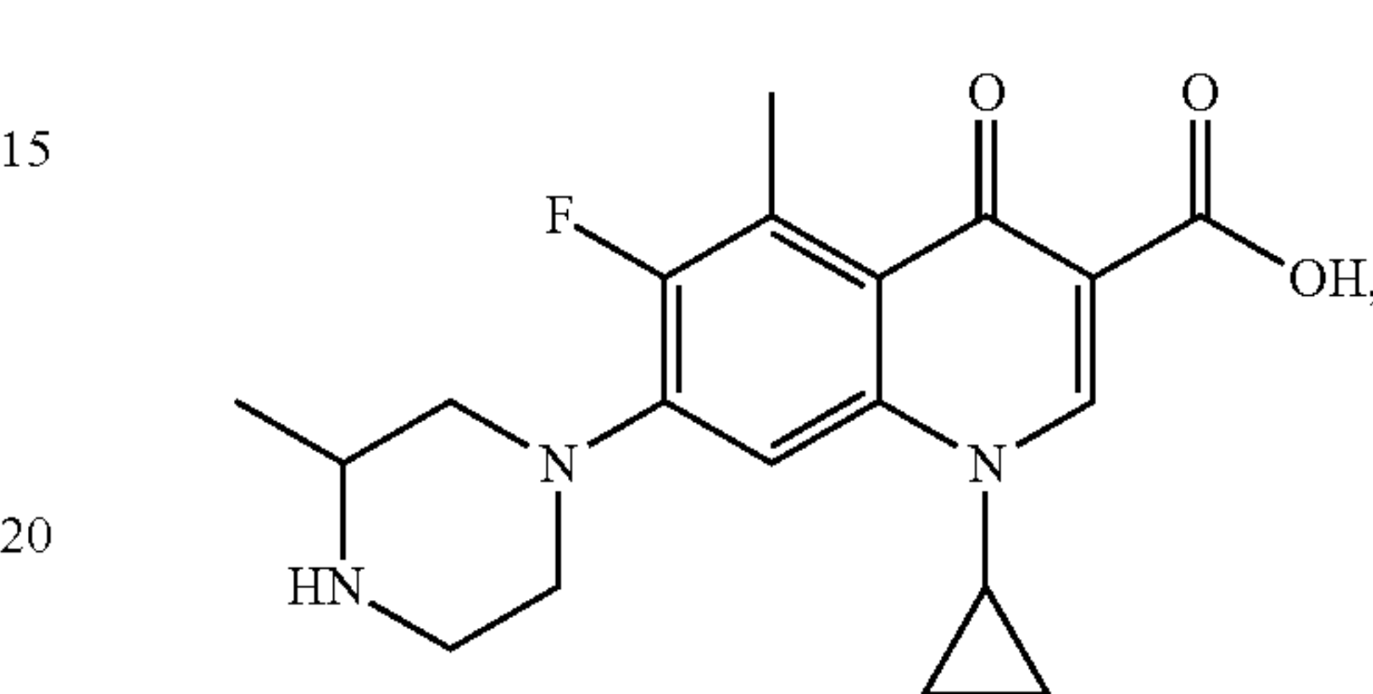
Grepafloxacin
