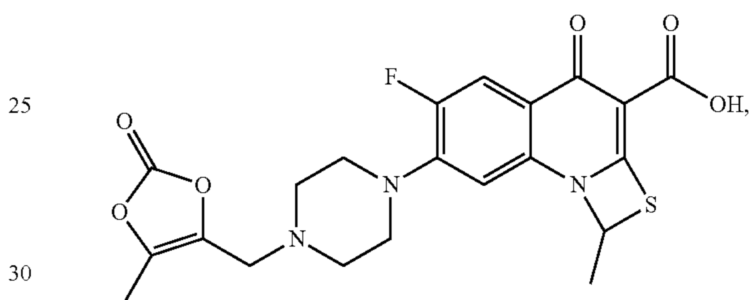
Prulifloxacin
