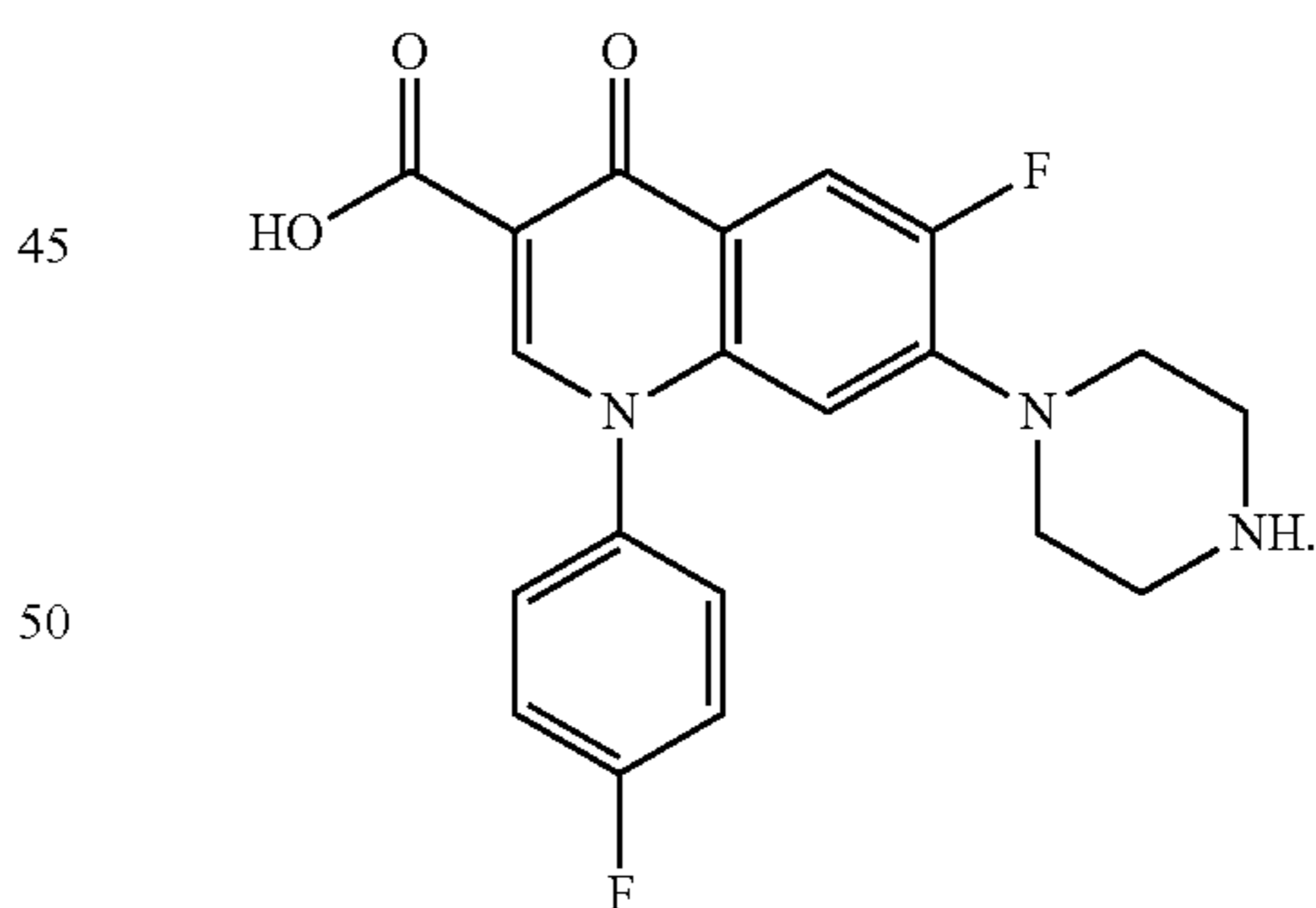
Sarafloxacin
