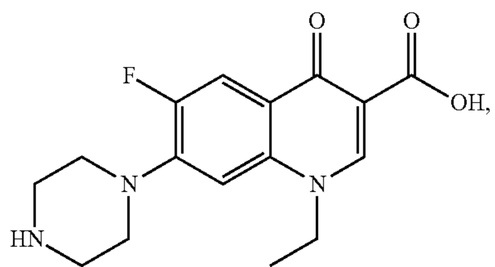
Norfloxacin
