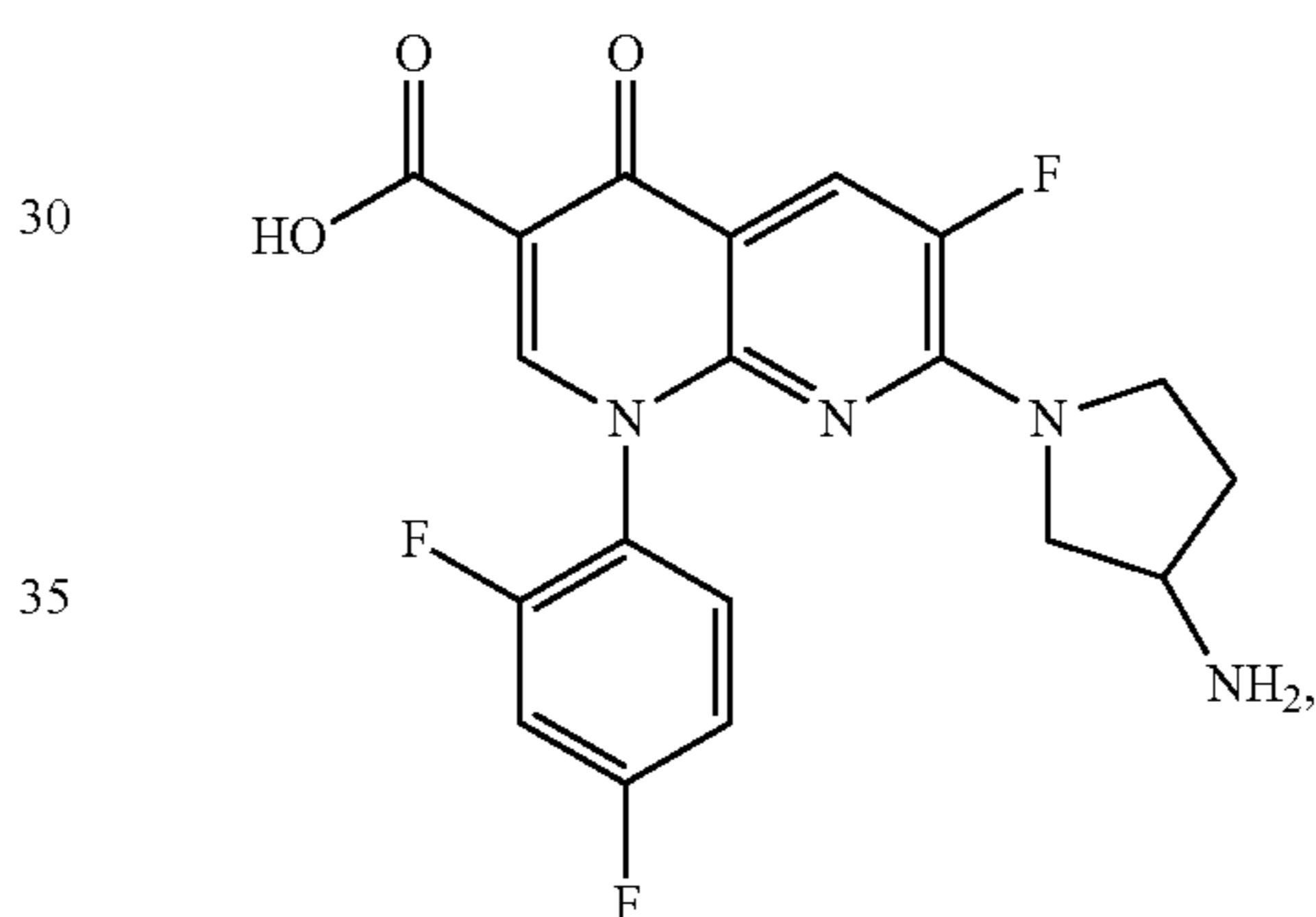
Tosufloxacin
