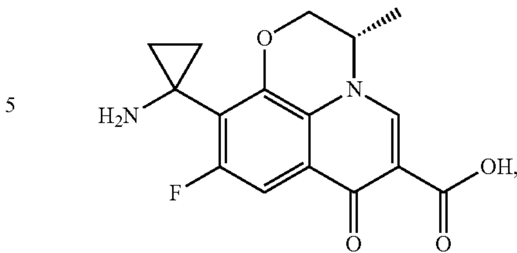
Pazufloxacin
