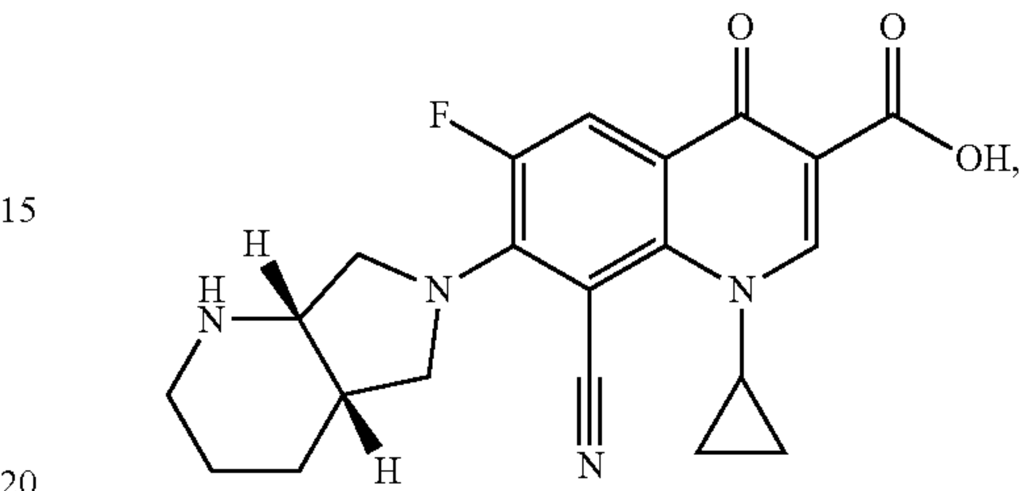
Pradofloxacin
