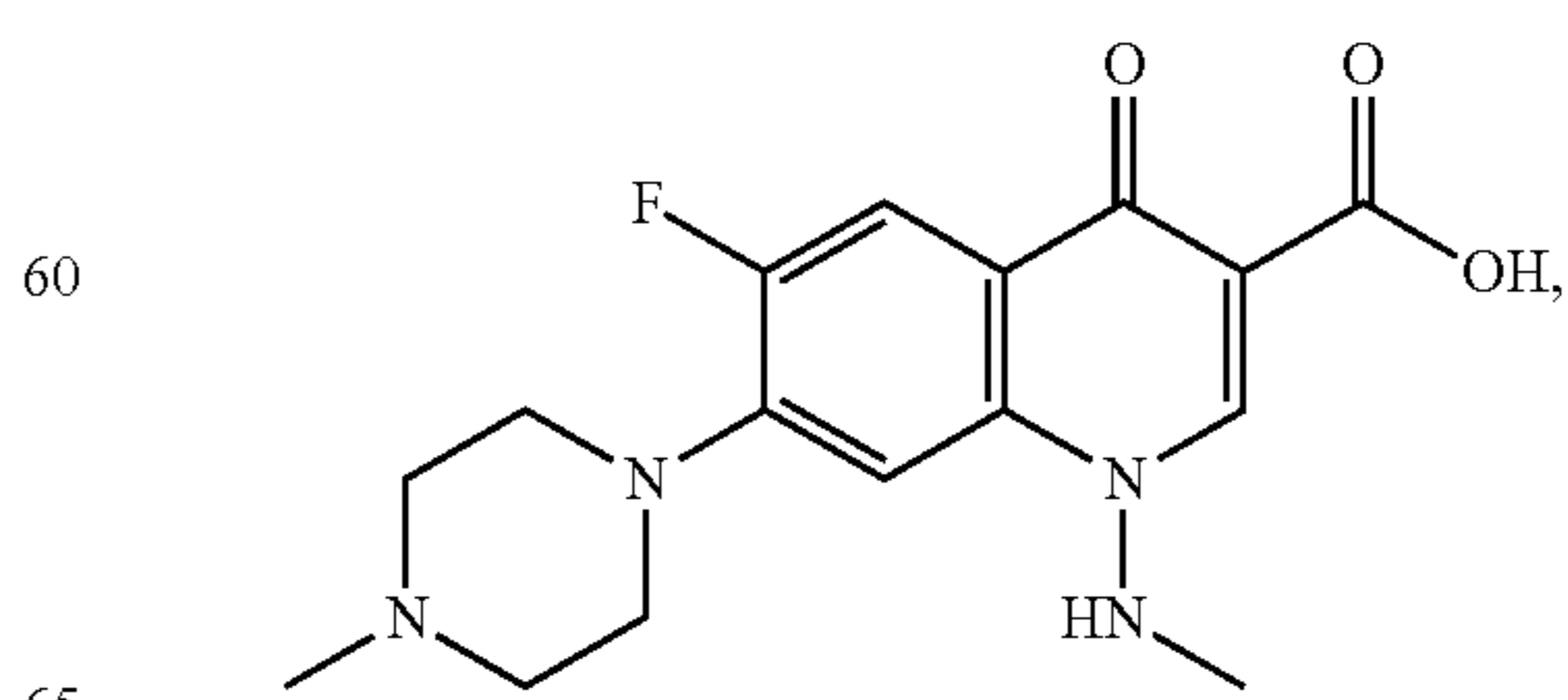
Amifloxacin
