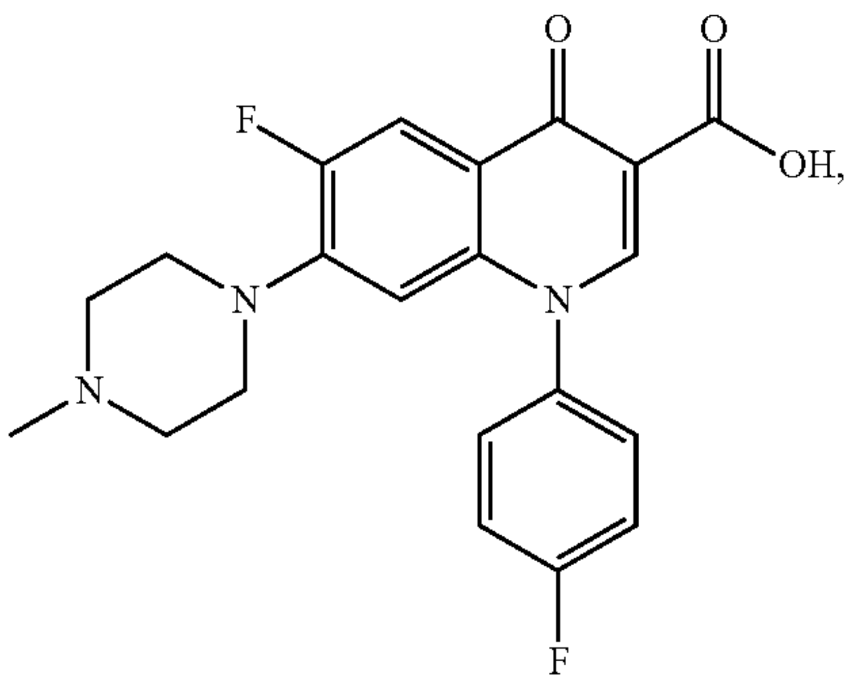
Difloxacin
