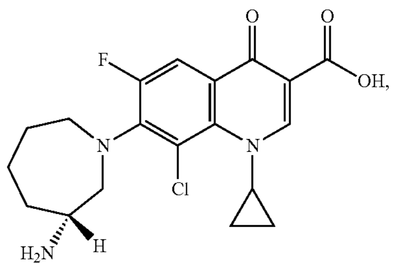
Besifloxacin
