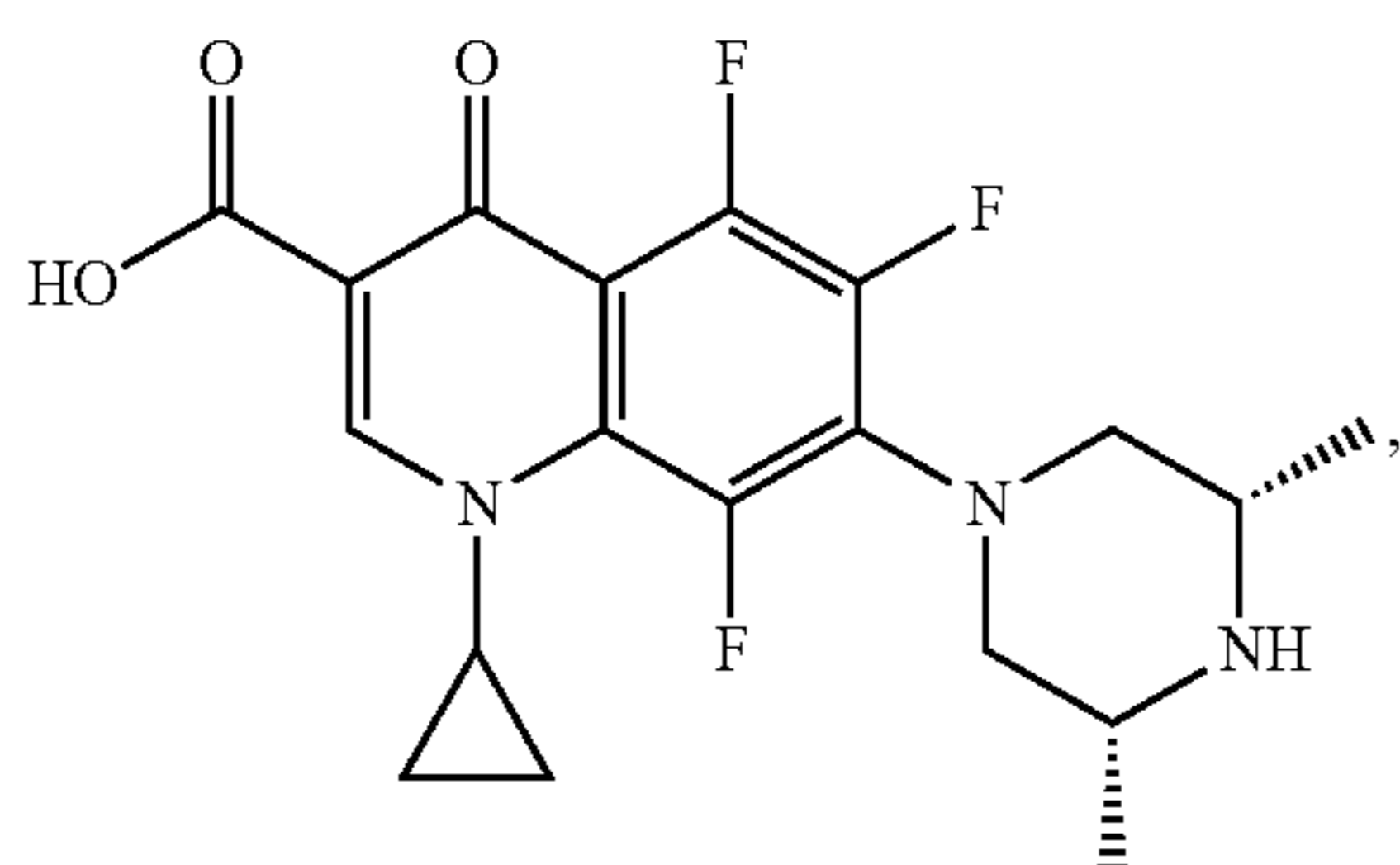
Orbifloxacin
