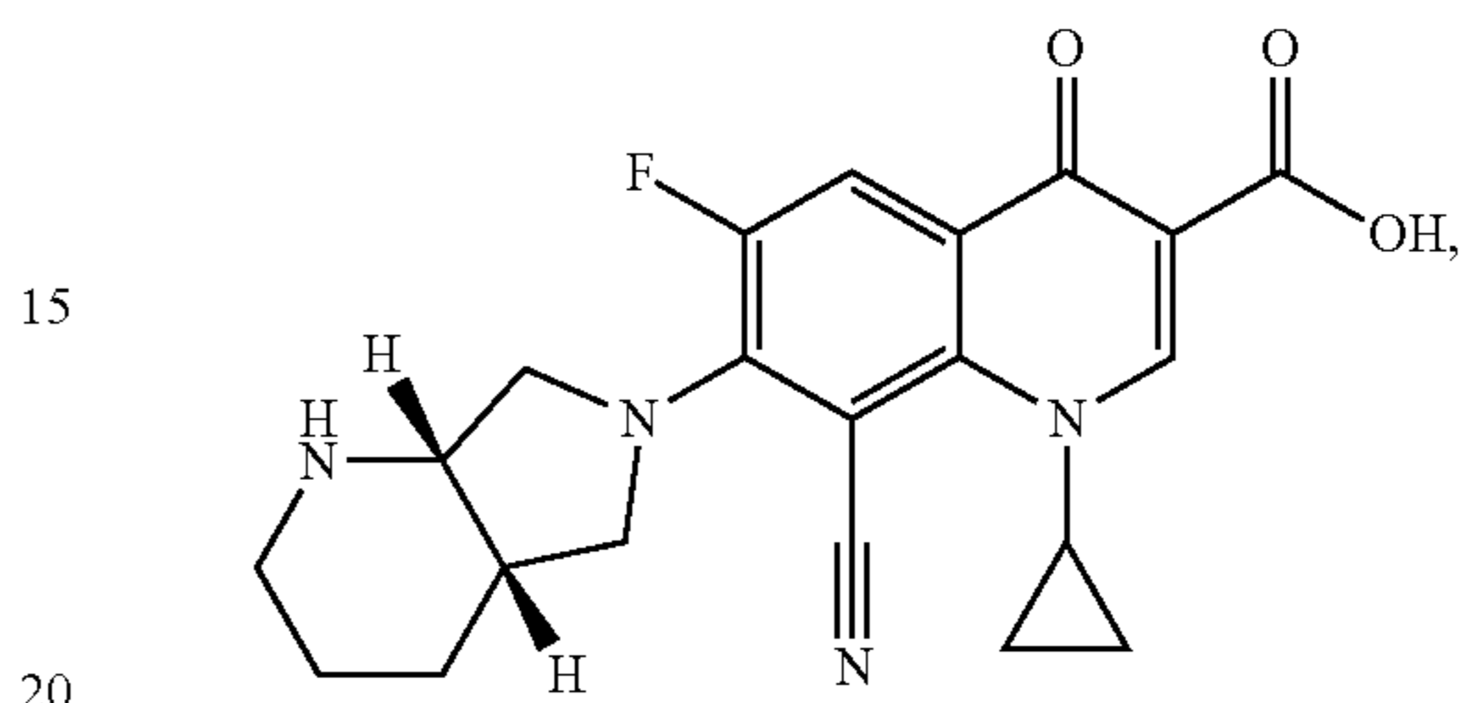
Pradofloxacin
