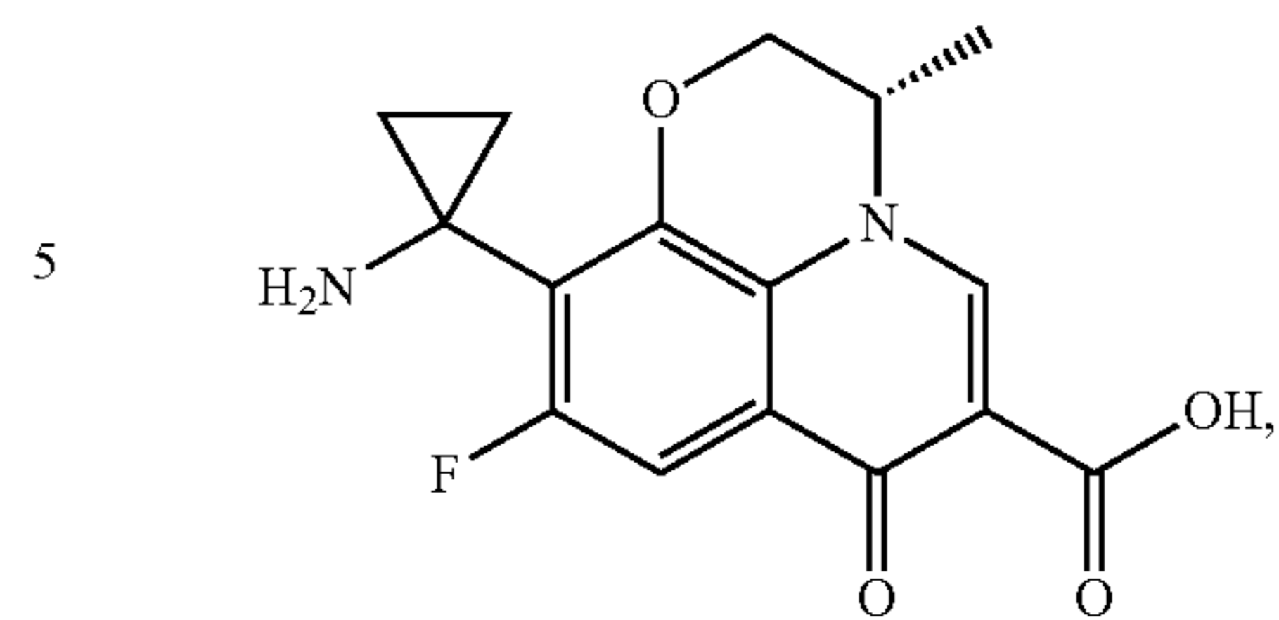
Pazufloxacin
