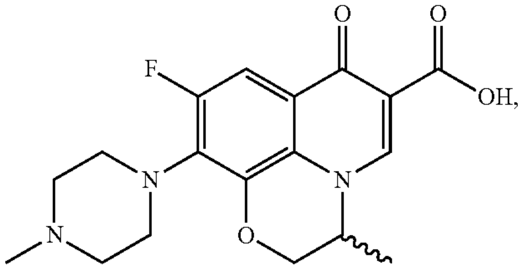
Dextrofloxacine
