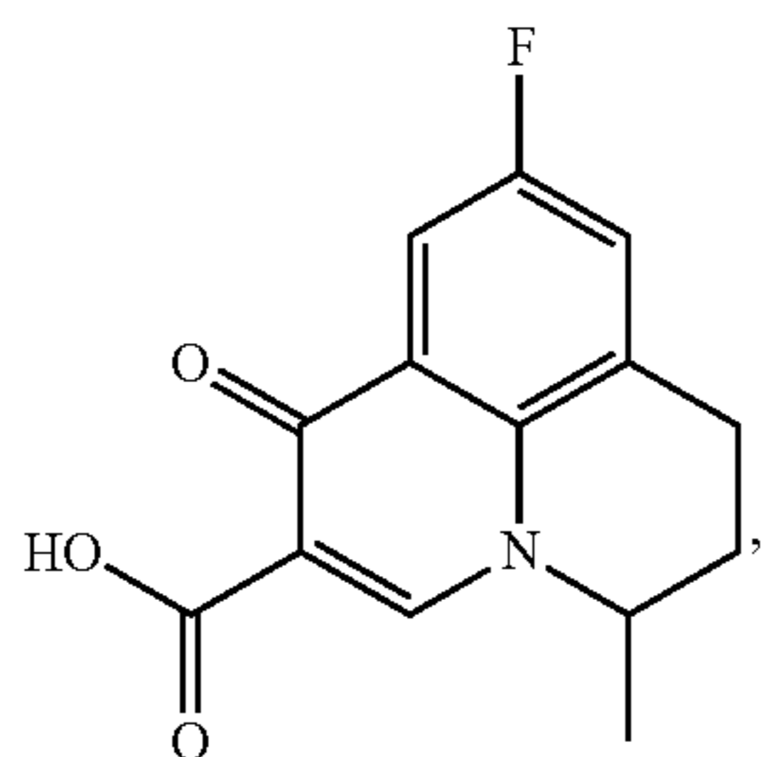
Flumequine
