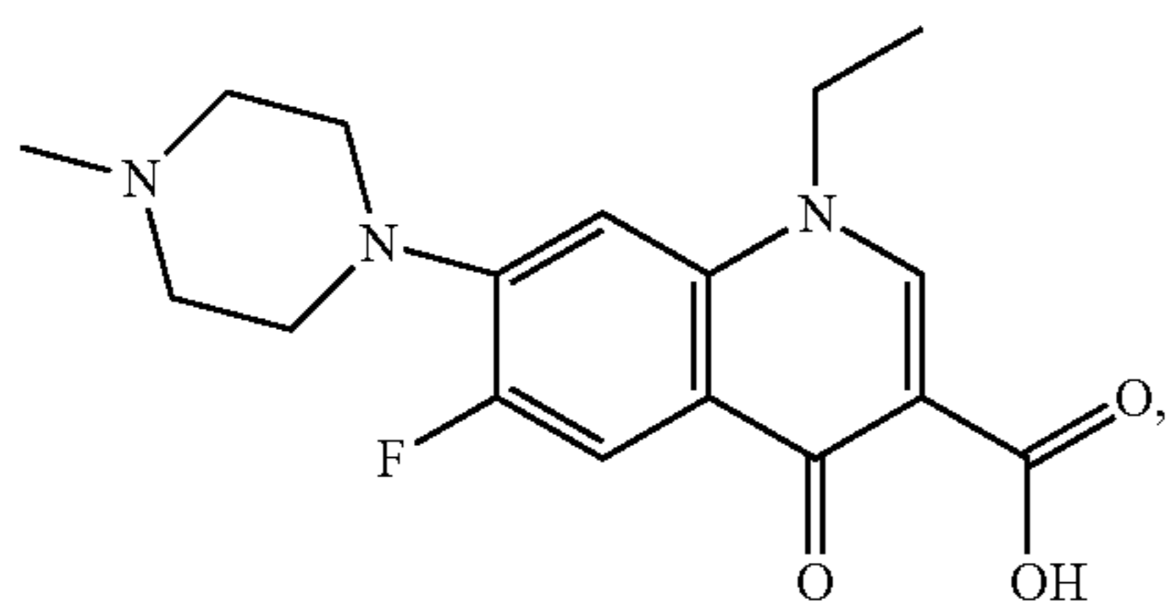
Pefloxacin
