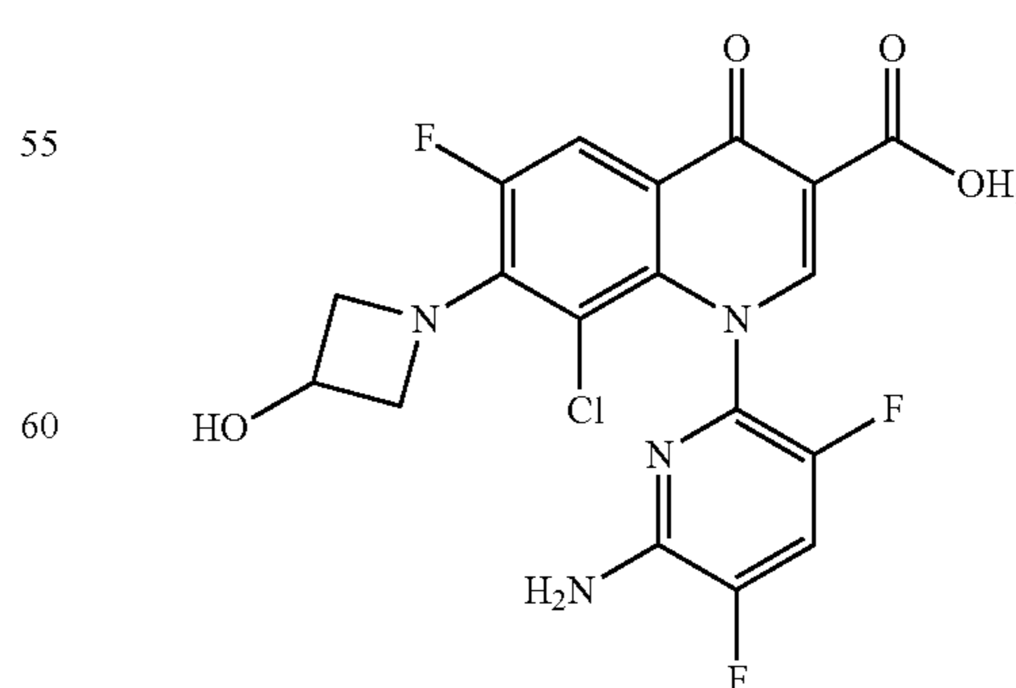
Delafloxacin
