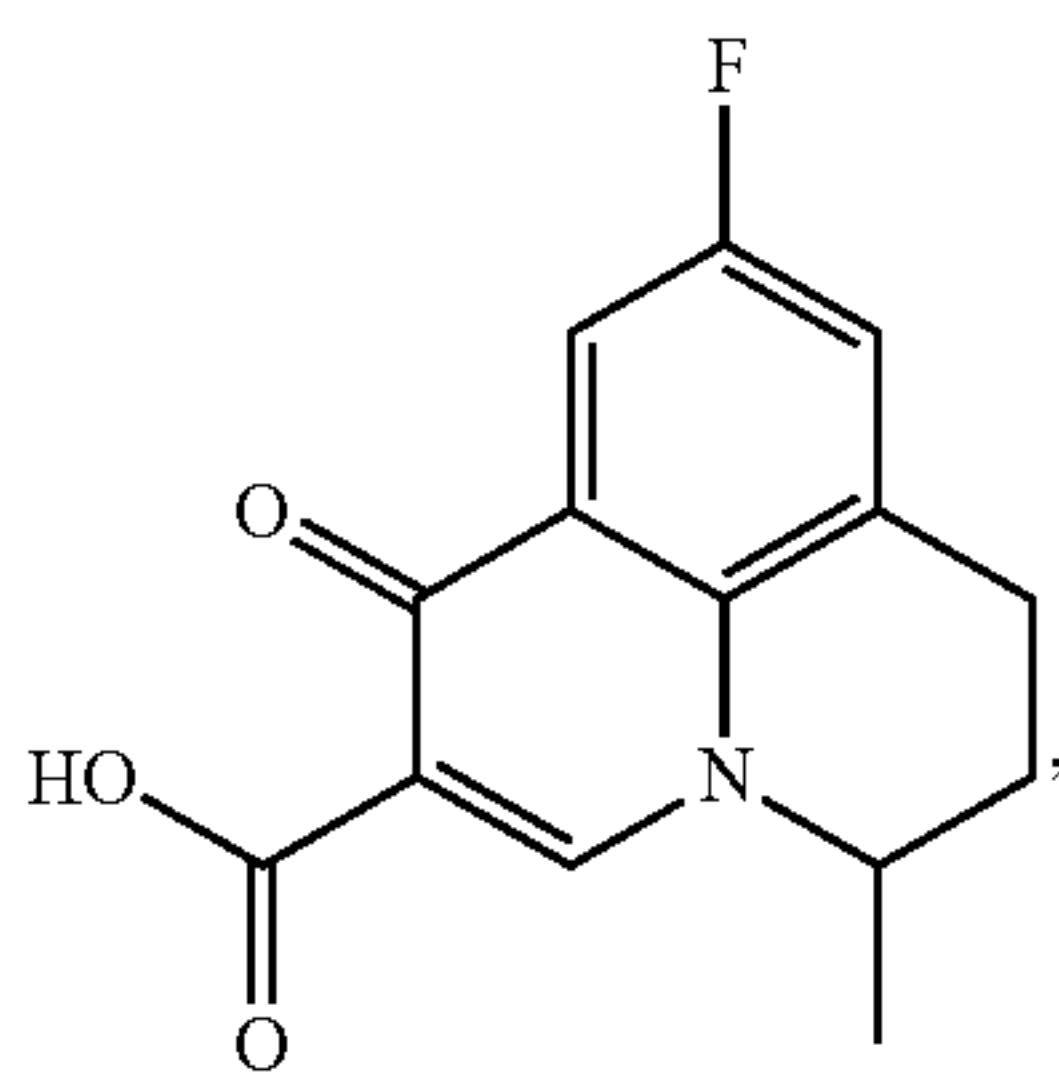
Flumequine
