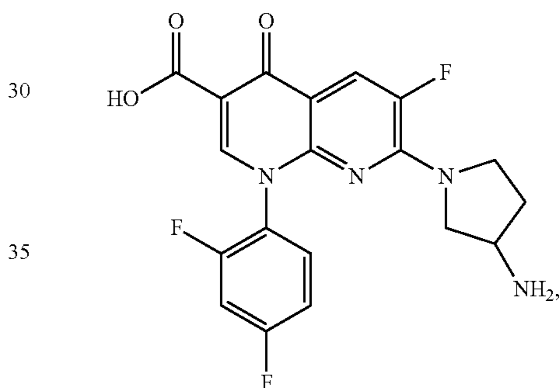
Tosufloxacin
