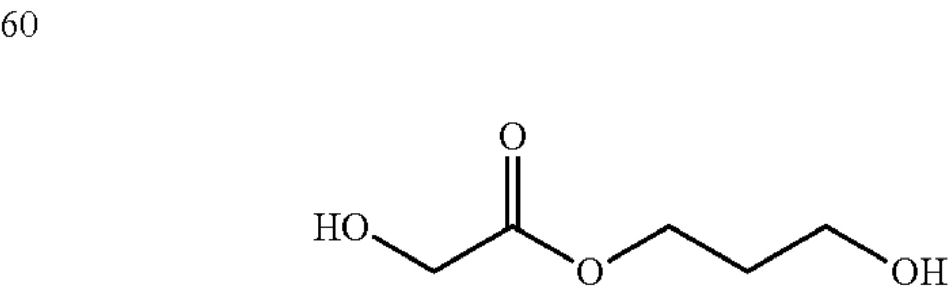
Hydroxy-acetic acid 3-hydroxy-propyl ester (GA-1,3-PD)
