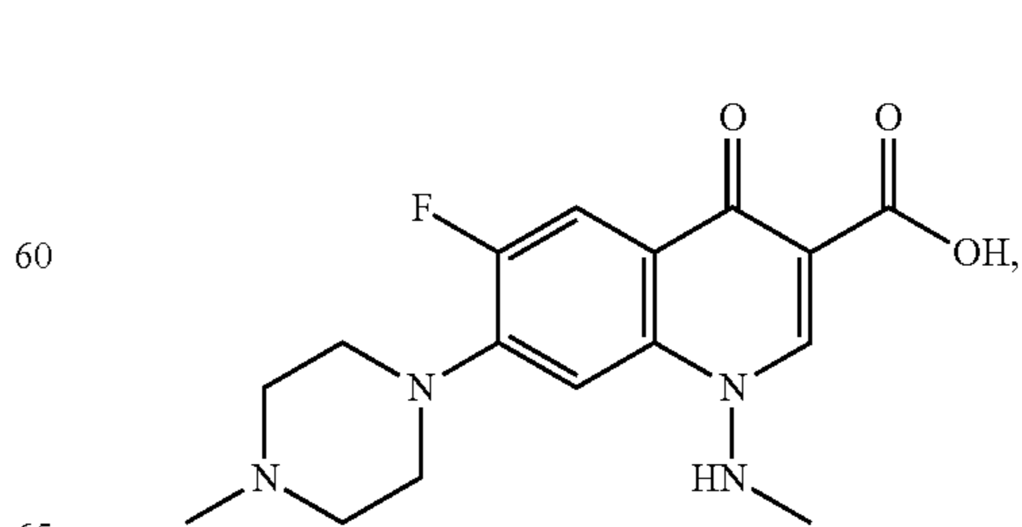
Amifloxacin
