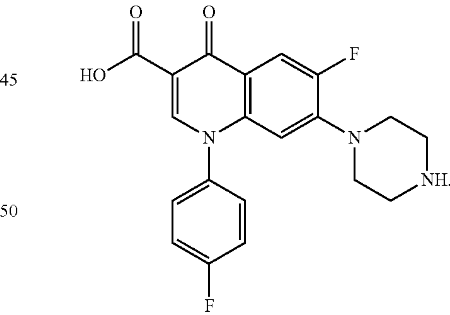
Sarafloxacin
