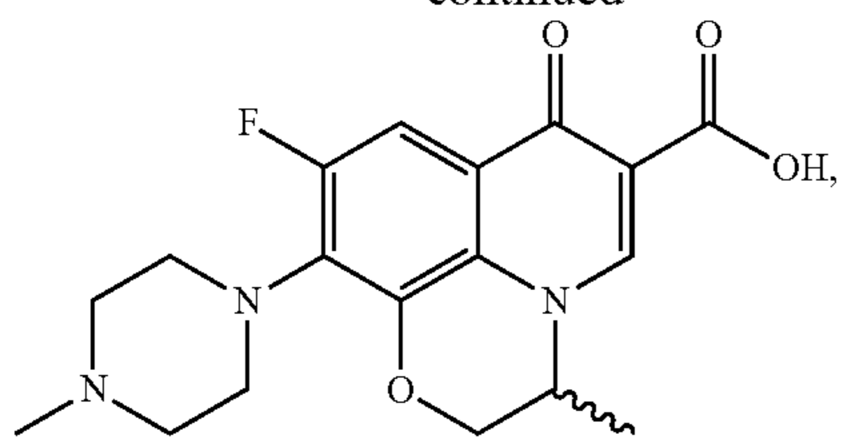
Dextrofloxacina
