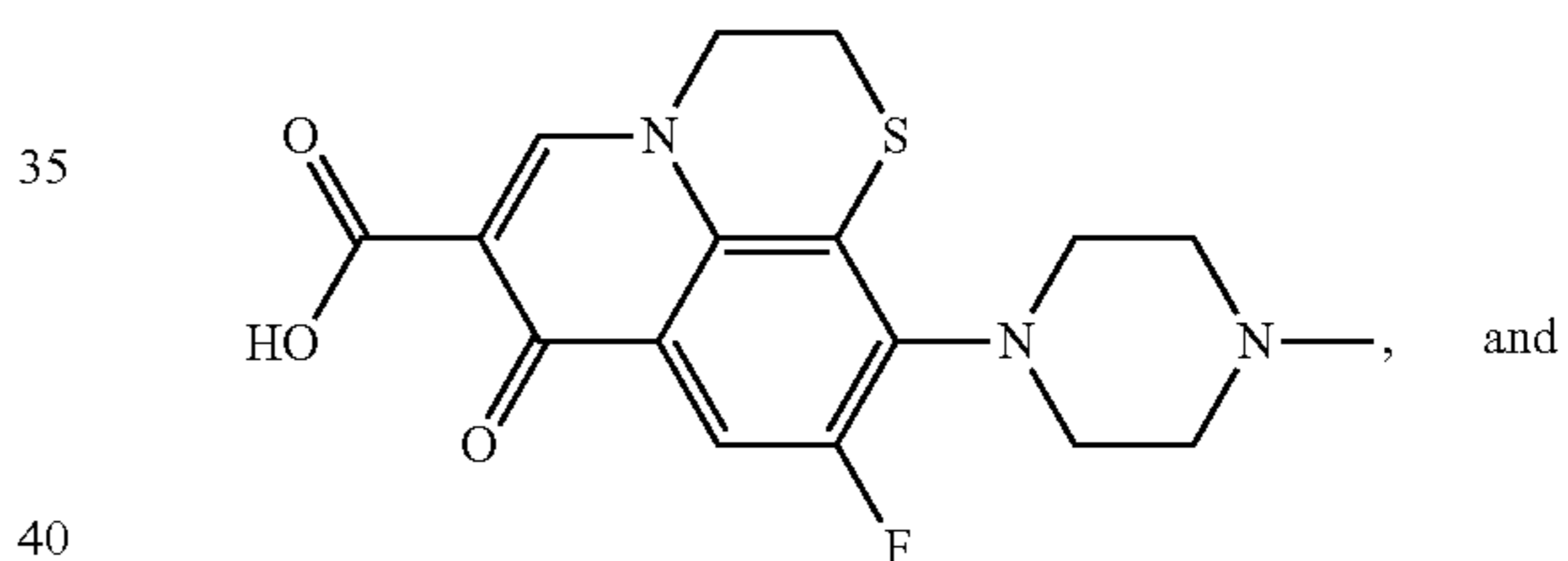
Rufloxacin
