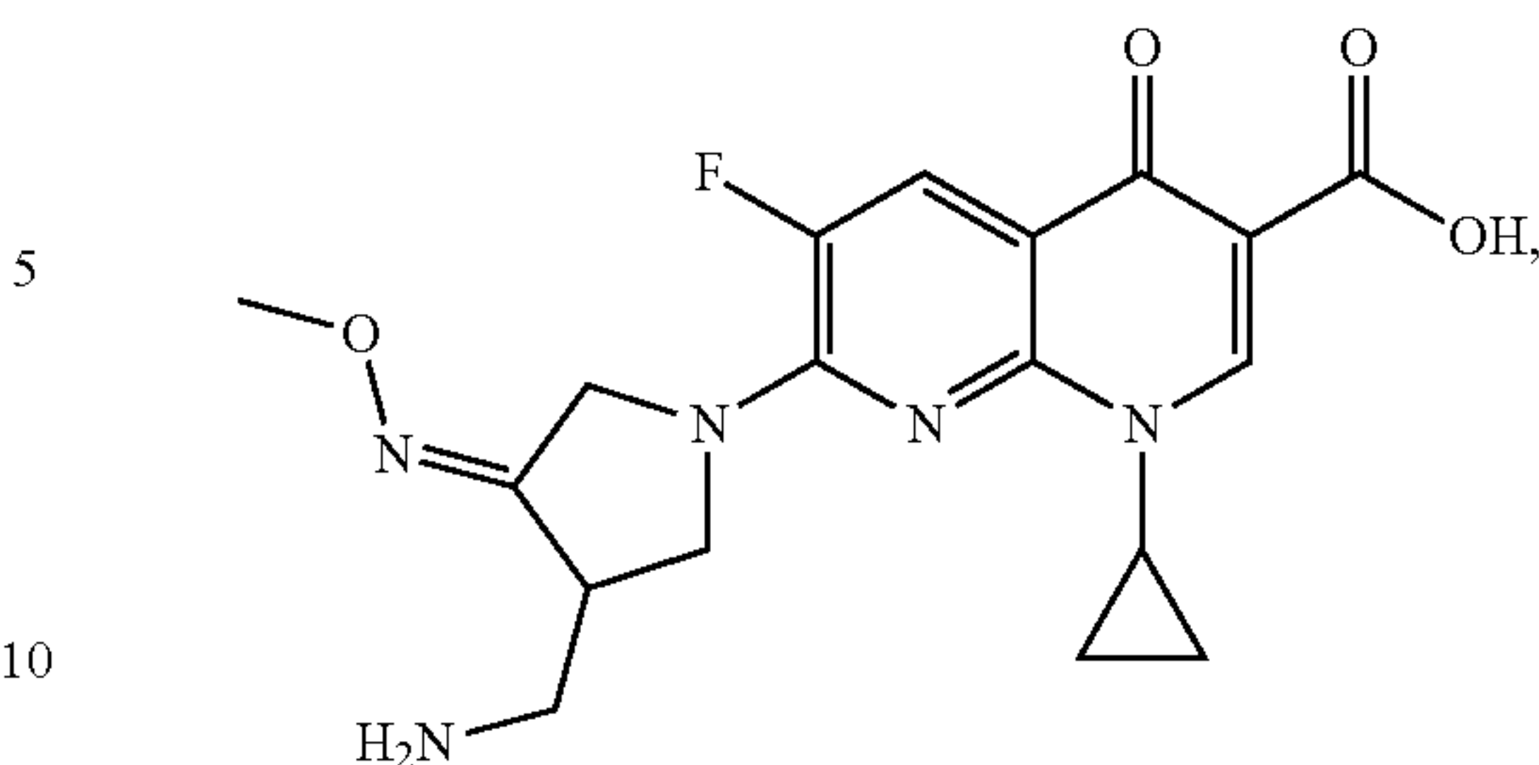
Gemifloxacin
