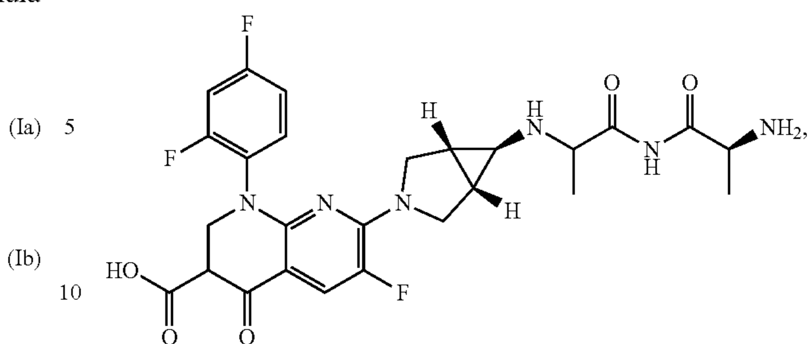
Alatrofloxacin
