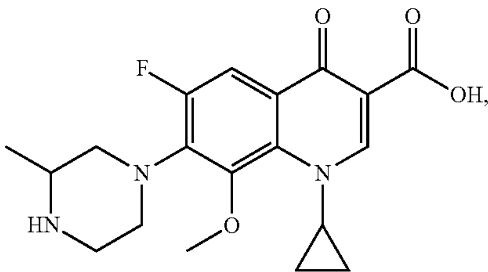
Gatifloxacin
