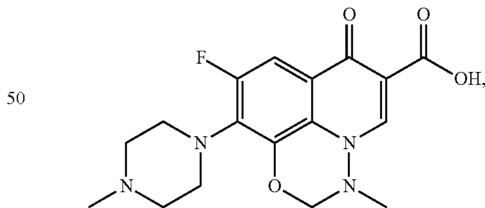
Marbofloxacina
