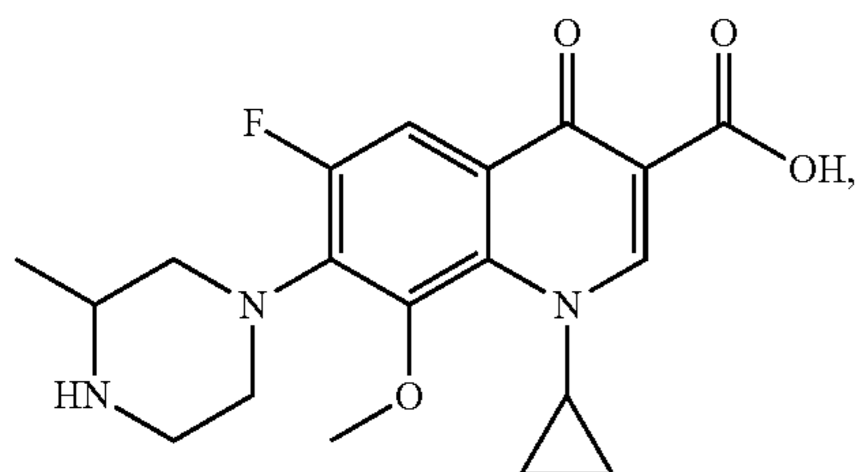
Gatifloxacin
