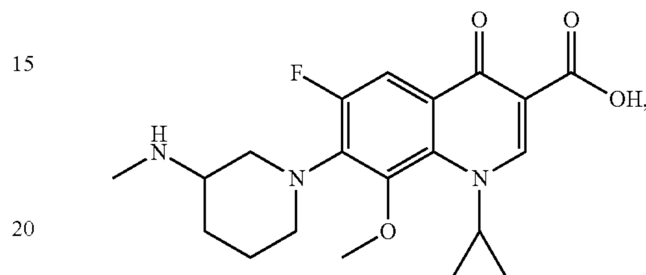
Balofloxacin
