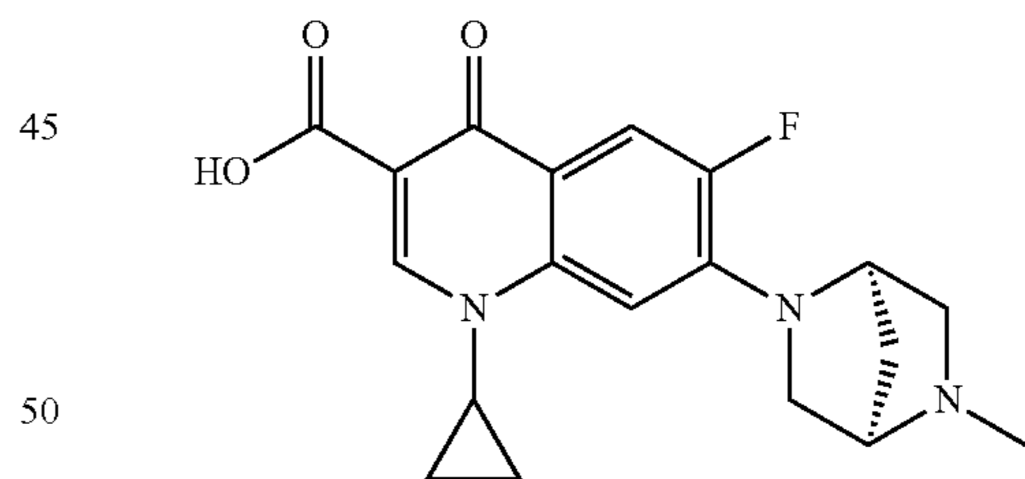
Danofloxacin
