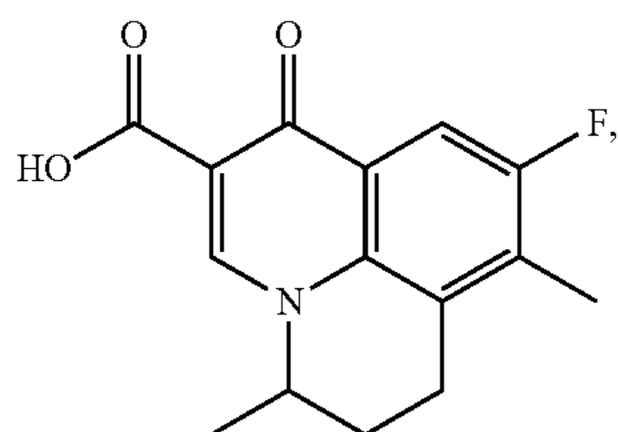
Ibafloxacin
