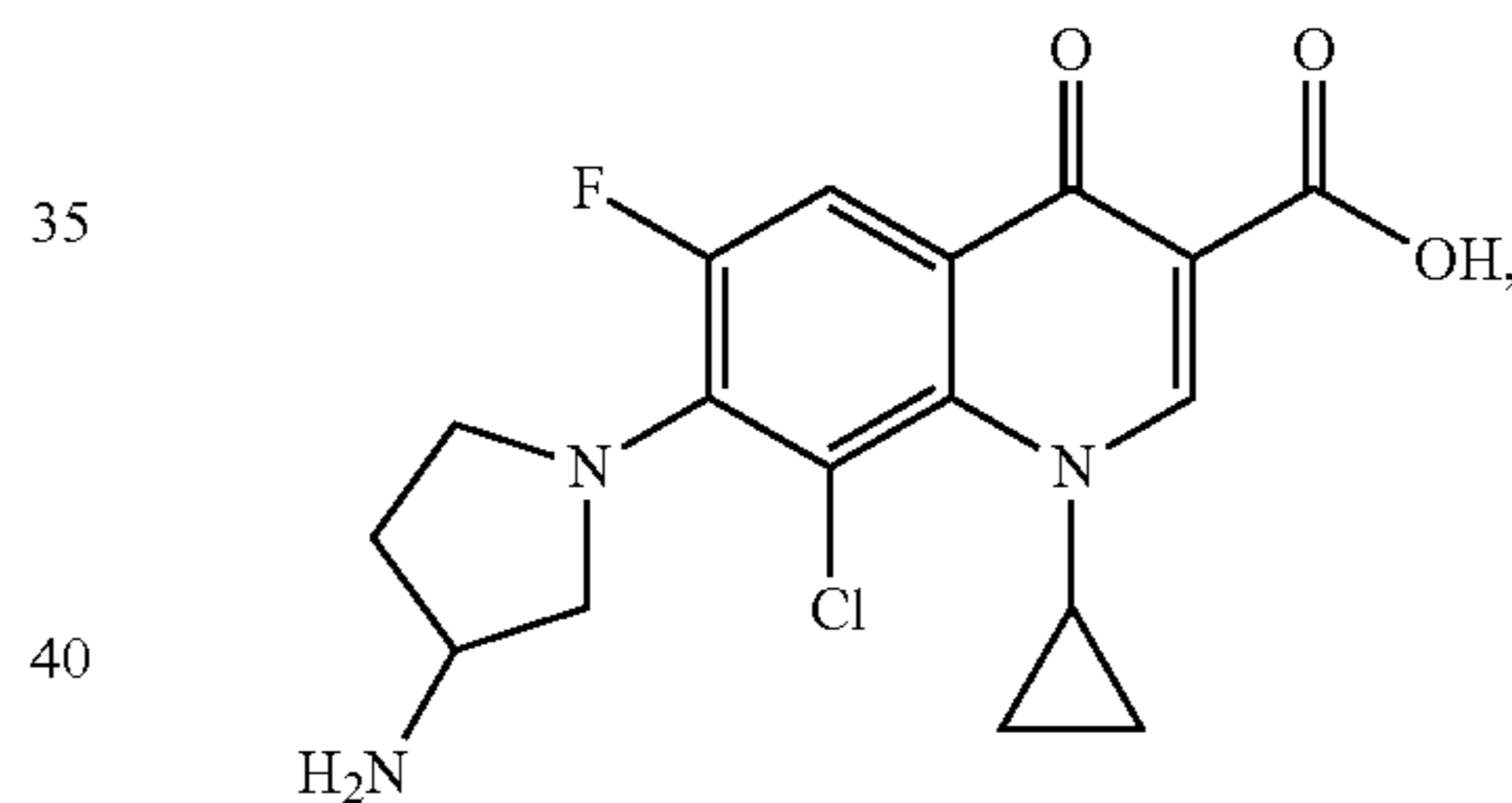
Clinafloxacin
