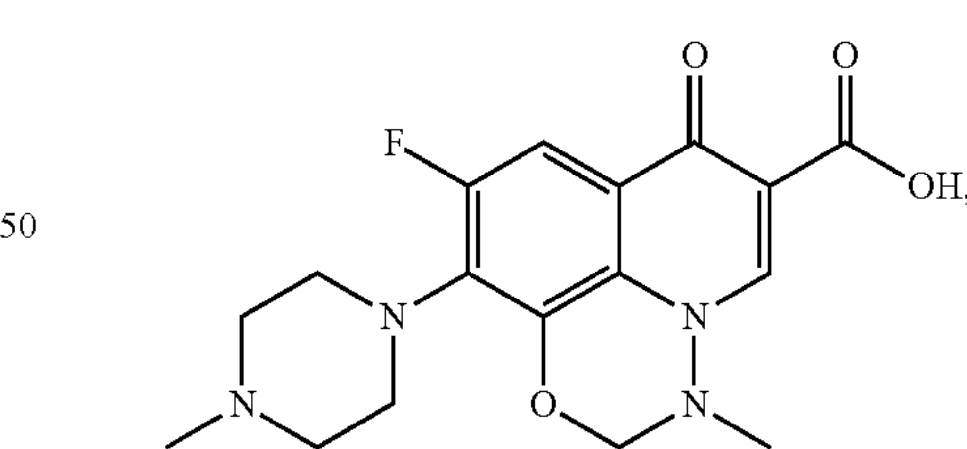
Marbofloxacin
