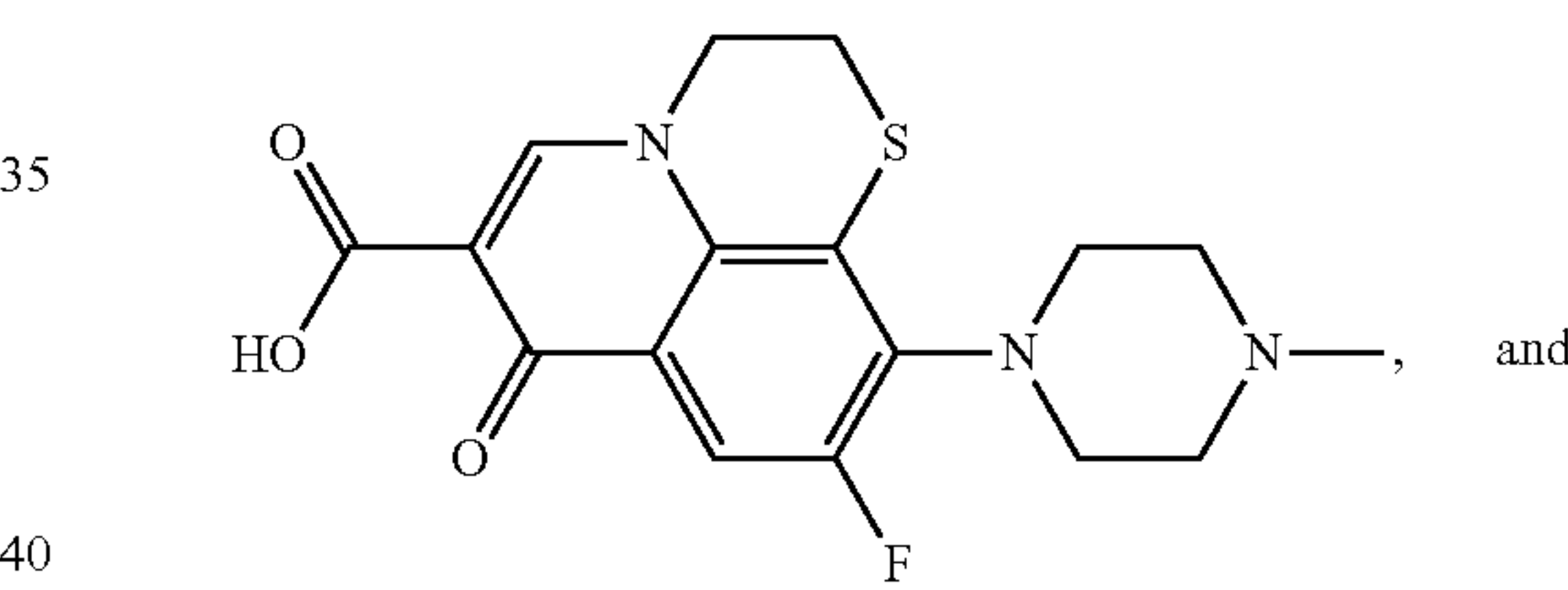
Rufloxacin
