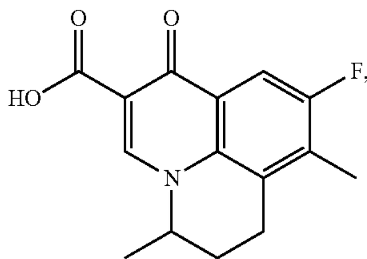
Ibafoxacin
