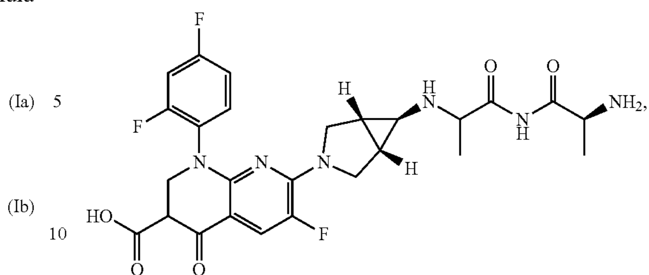
Alatrofloxacin
