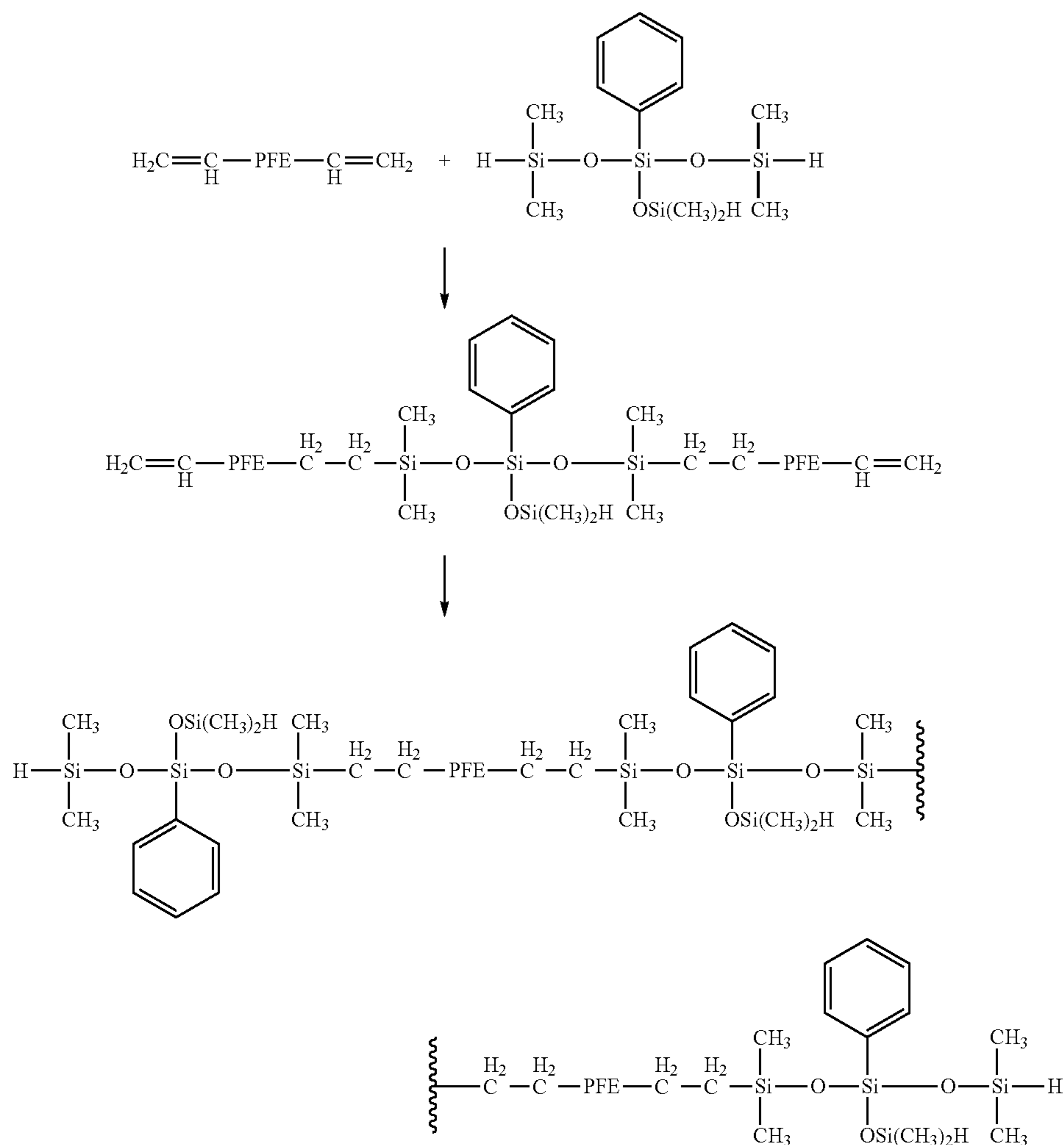
Scheme 3
