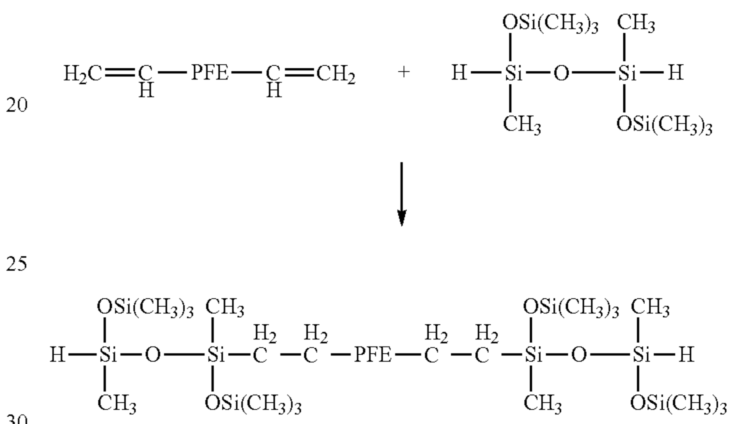
Scheme 1
