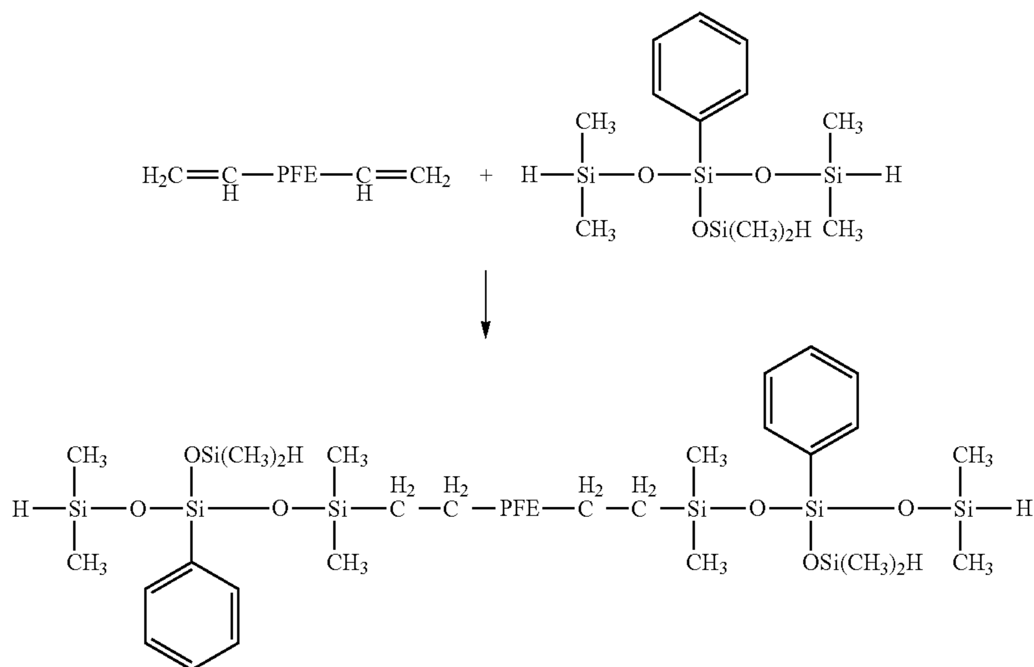
Scheme 2
